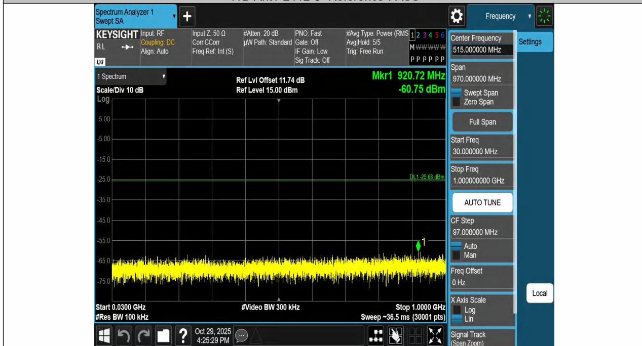
11B-Ant1-2412-30~1000-PASS
