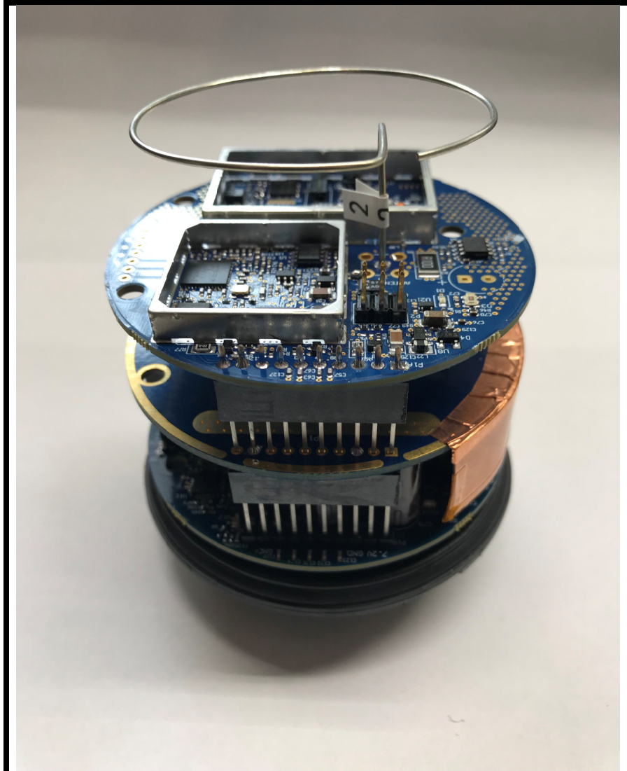
External Photo # 2 – Assembly View
