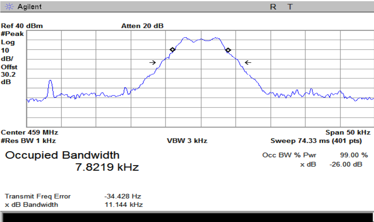
Plot 6 – High Band
