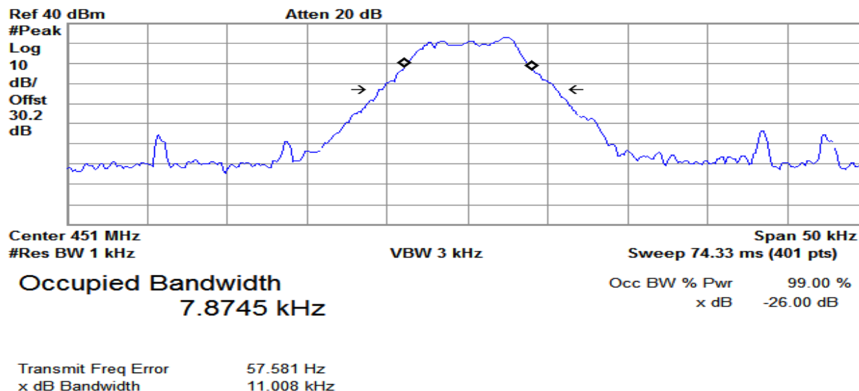
Plot 4 – Low Band
