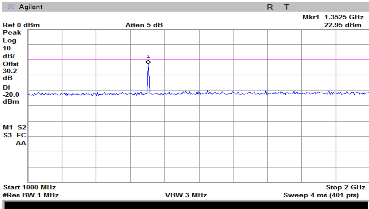
Plot 11 – Low Band
