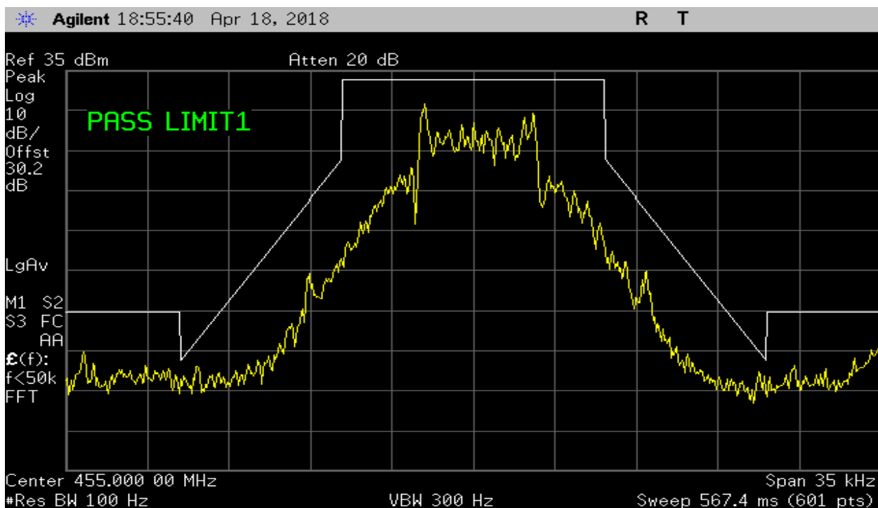
Plot 8 – Mid Chanel at Narrow Band 12.5 kHz Spacing – Mask D
