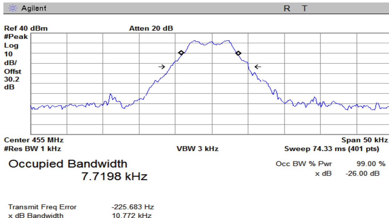
Plot 5 – Mid Band
