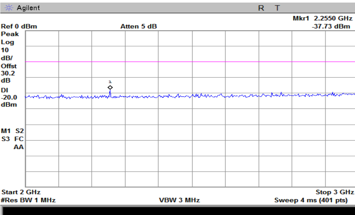
Plot 12 – Low Band
