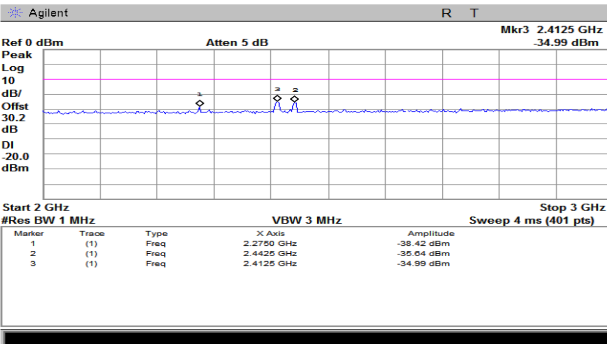
Plot 16 – Mid Band
