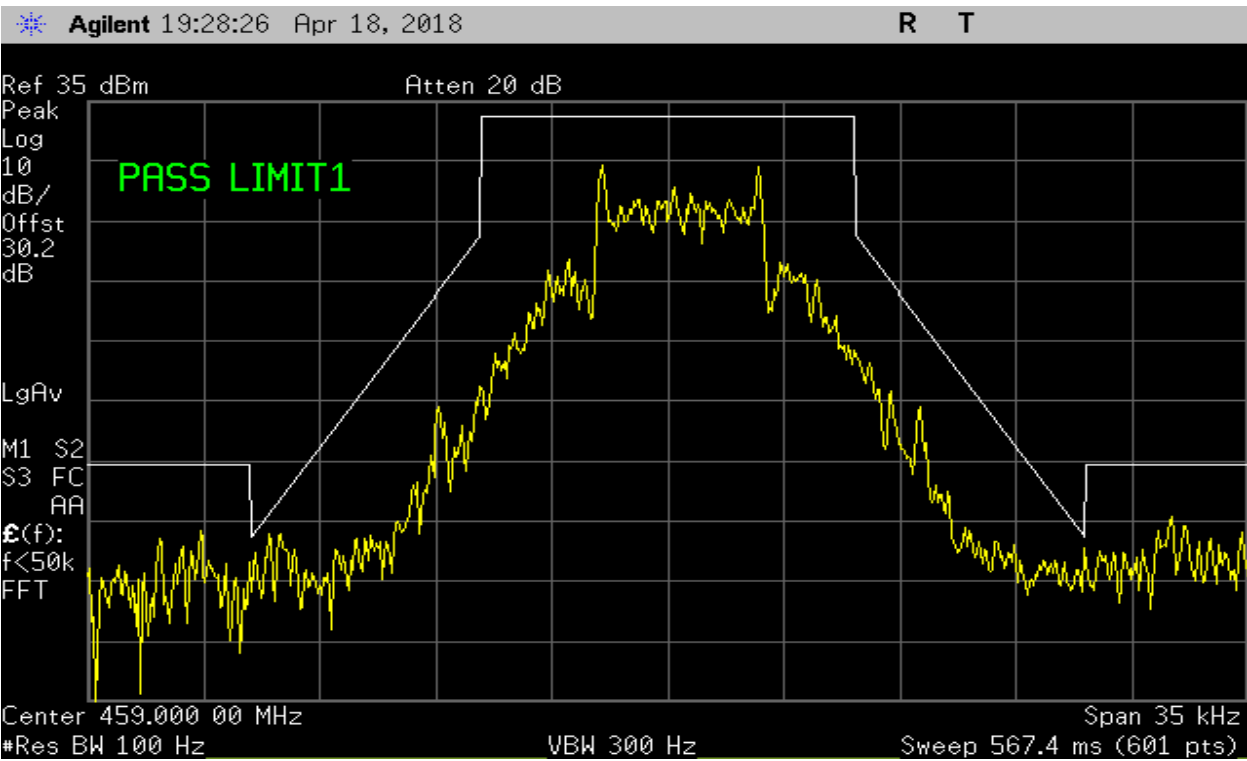
Plot 9 – High Channel at Narrow Band 12.5 kHz Spacing – Mask D
