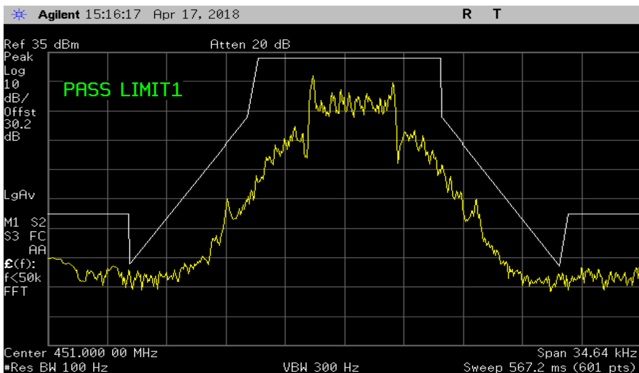
Plot 7 – Low Chanel 12.5 kHz Spacing – Mask D
