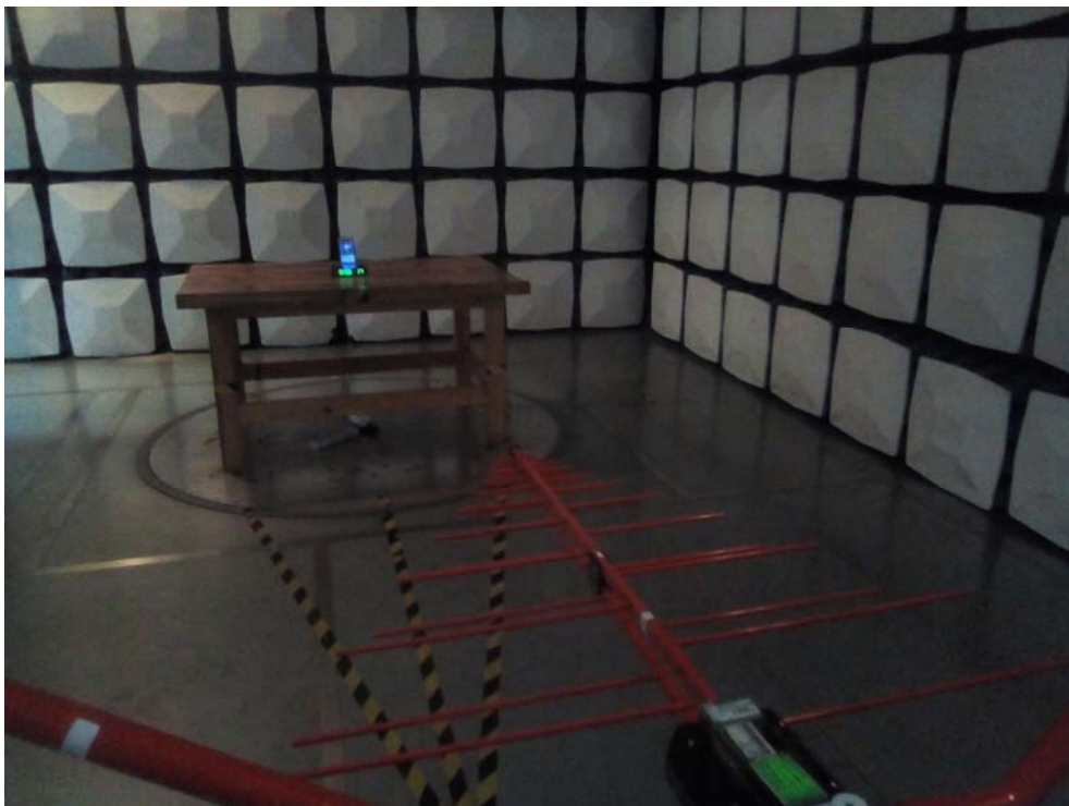
Radiated Emission View (30 MHz ~1 GHz)
