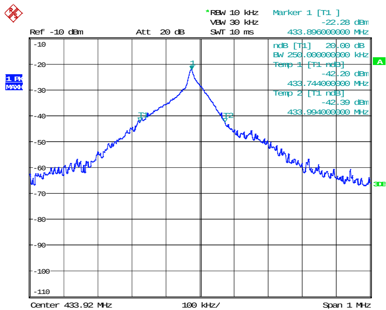
20dB Bandwidth Test Plot
