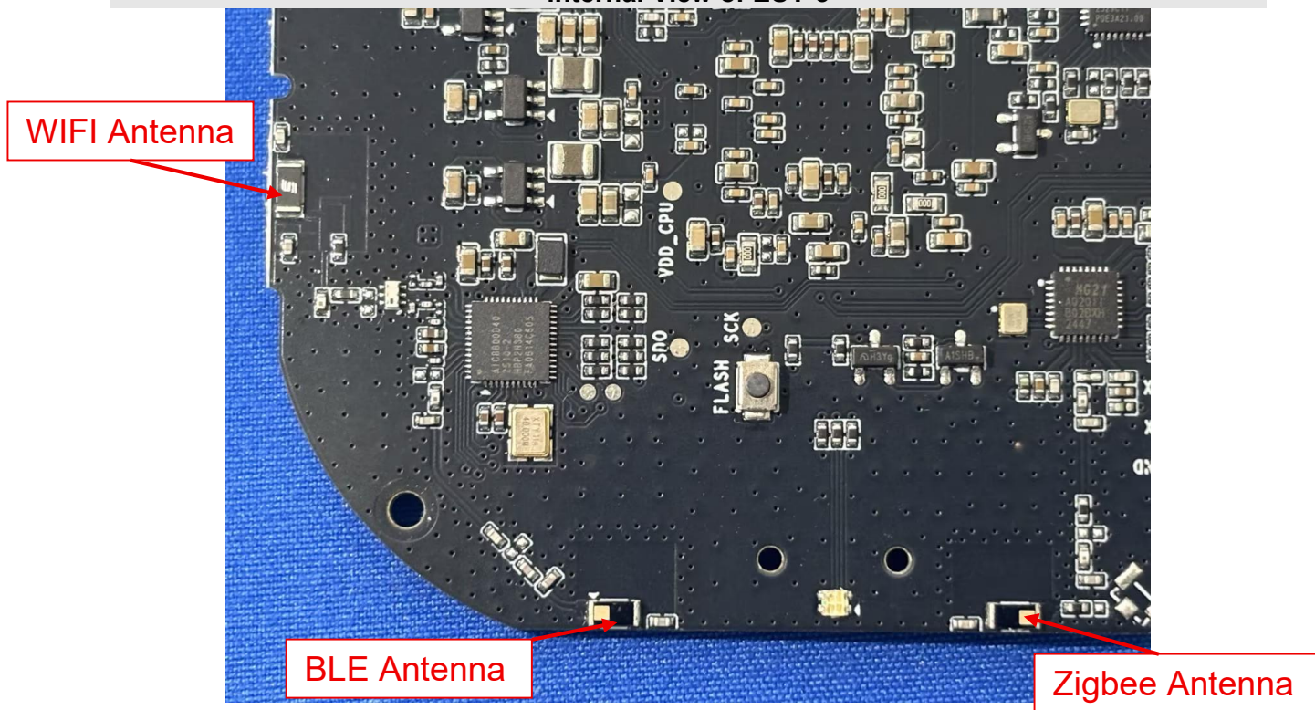
Internal View of EUT-4
