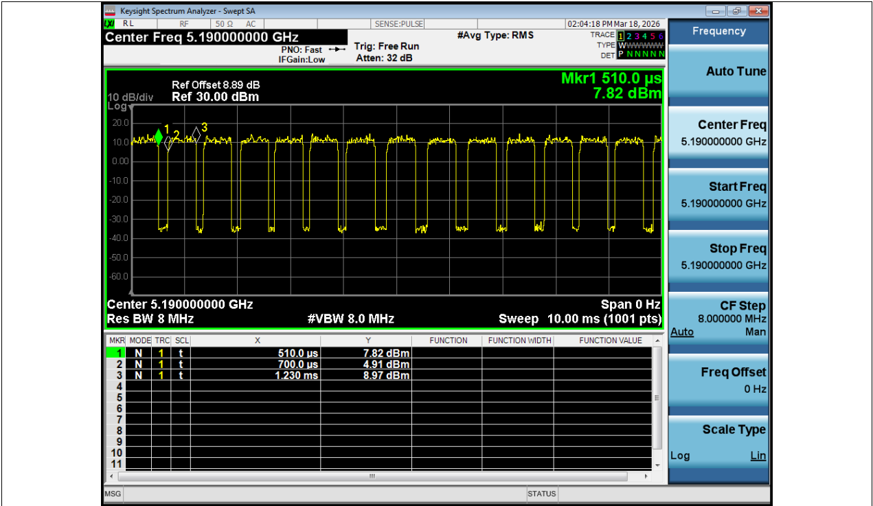
Duty Cycle NVNT ax40 5190MHz Ant1
