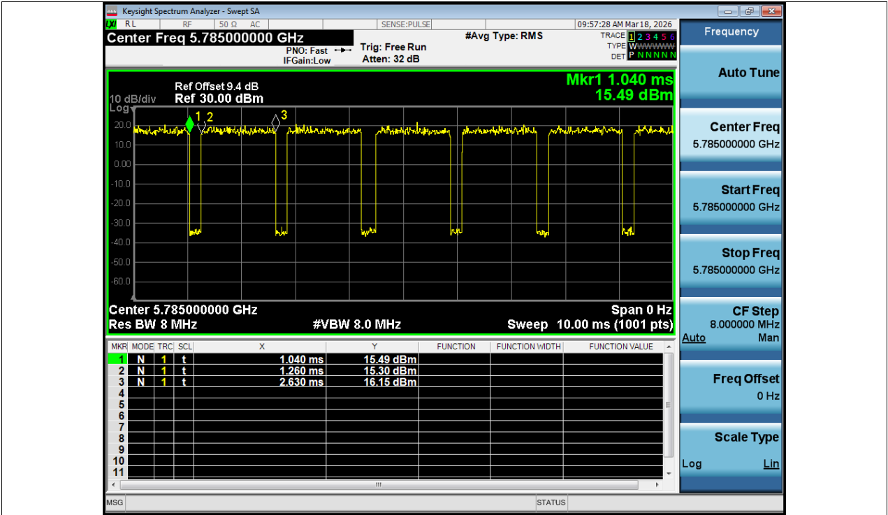
Duty Cycle NVNT a 5785MHz Ant1
