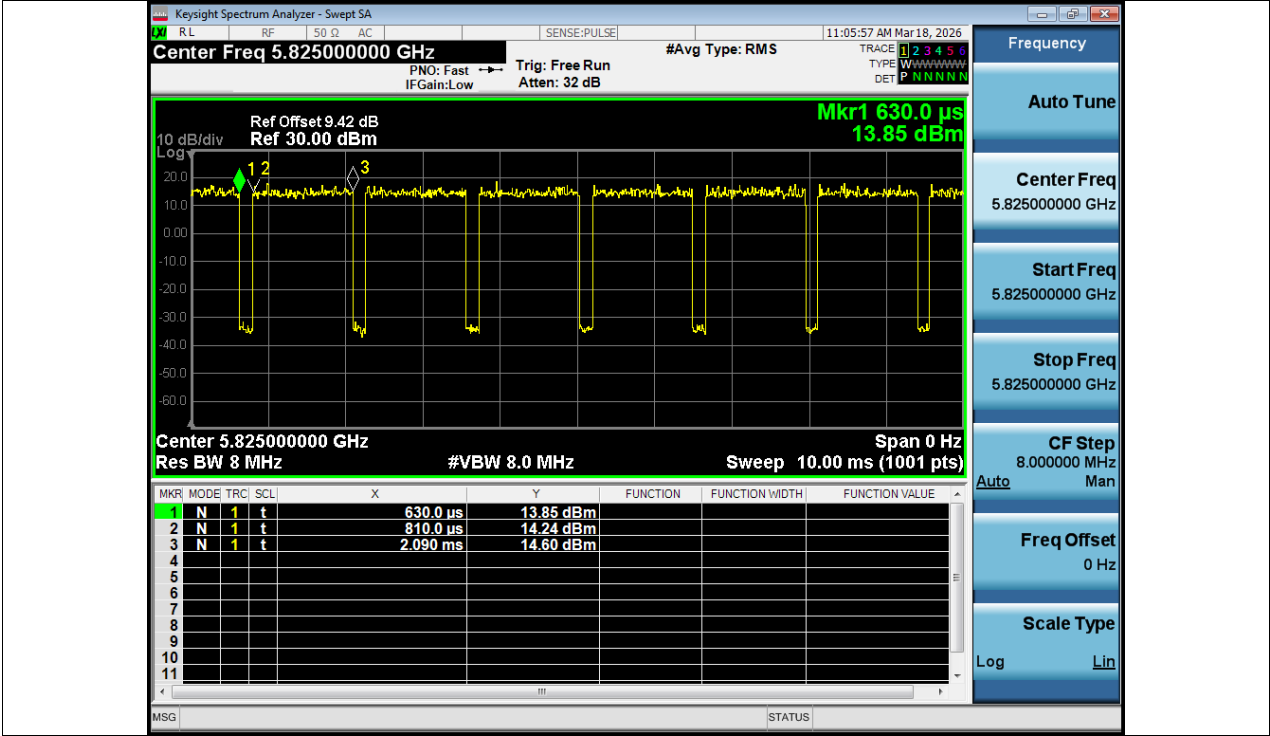
Duty Cycle NVNT ac20 5825MHz Ant1
