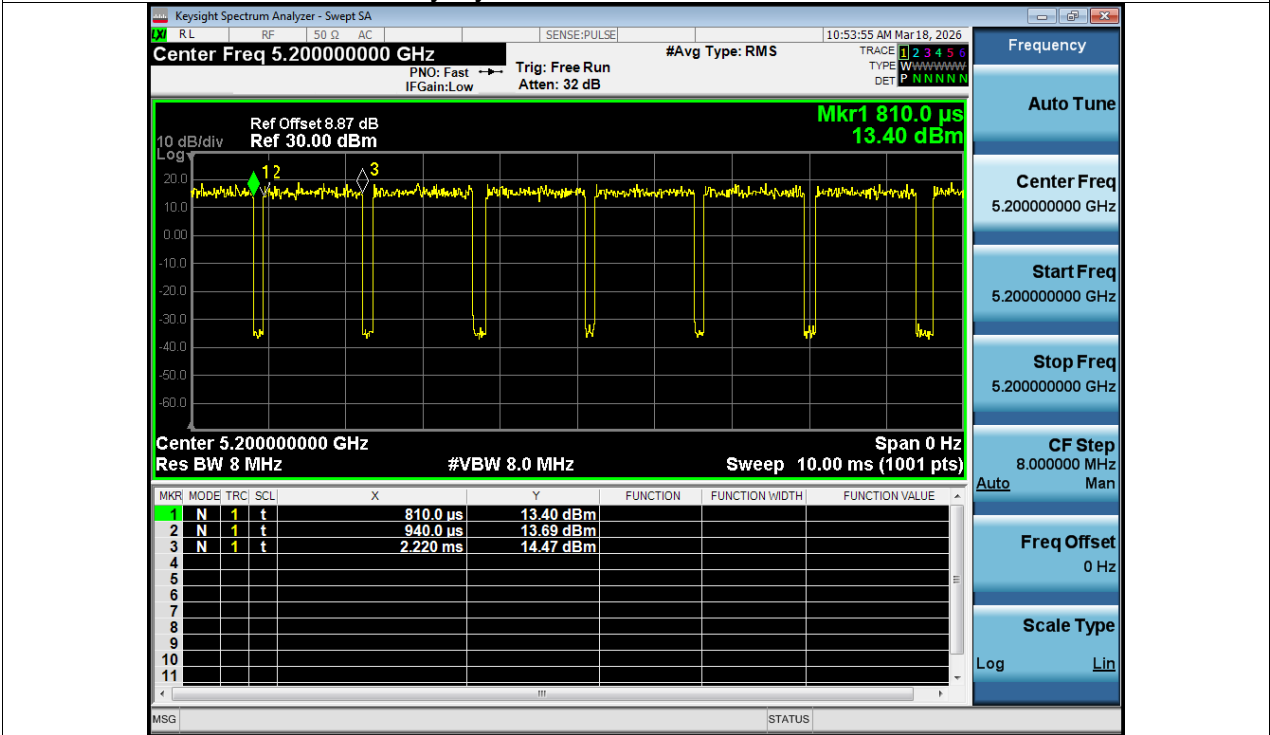
Duty Cycle NVNT ac20 5200MHz Ant1
