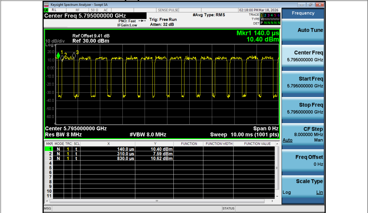
Duty Cycle NVNT ax40 5795MHz Ant1
