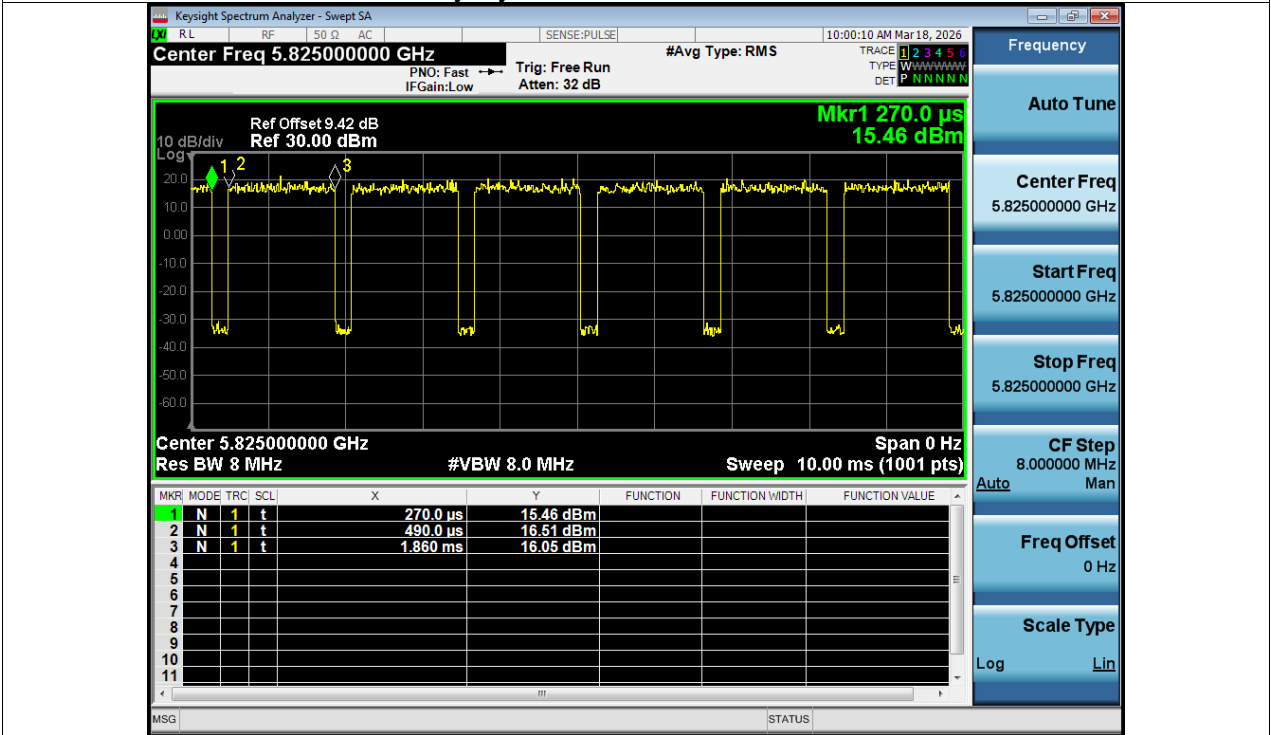
Duty Cycle NVNT a 5825MHz Ant1
