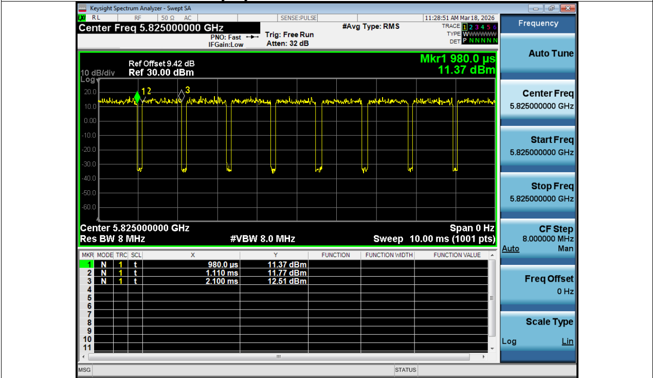
Duty Cycle NVNT ax20 5825MHz Ant1
