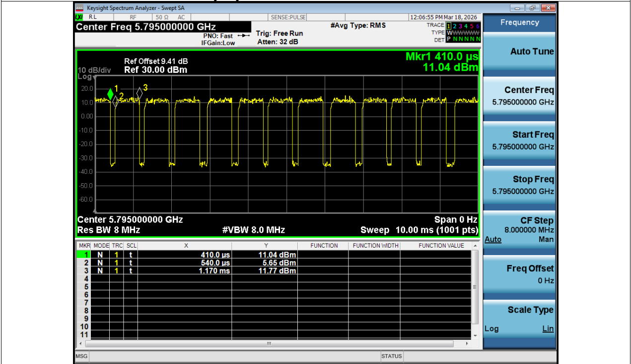
Duty Cycle NVNT ac40 5795MHz Ant1
