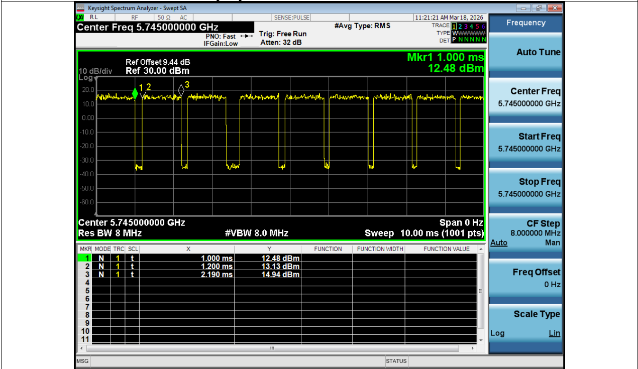
Duty Cycle NVNT ax20 5745MHz Ant1
