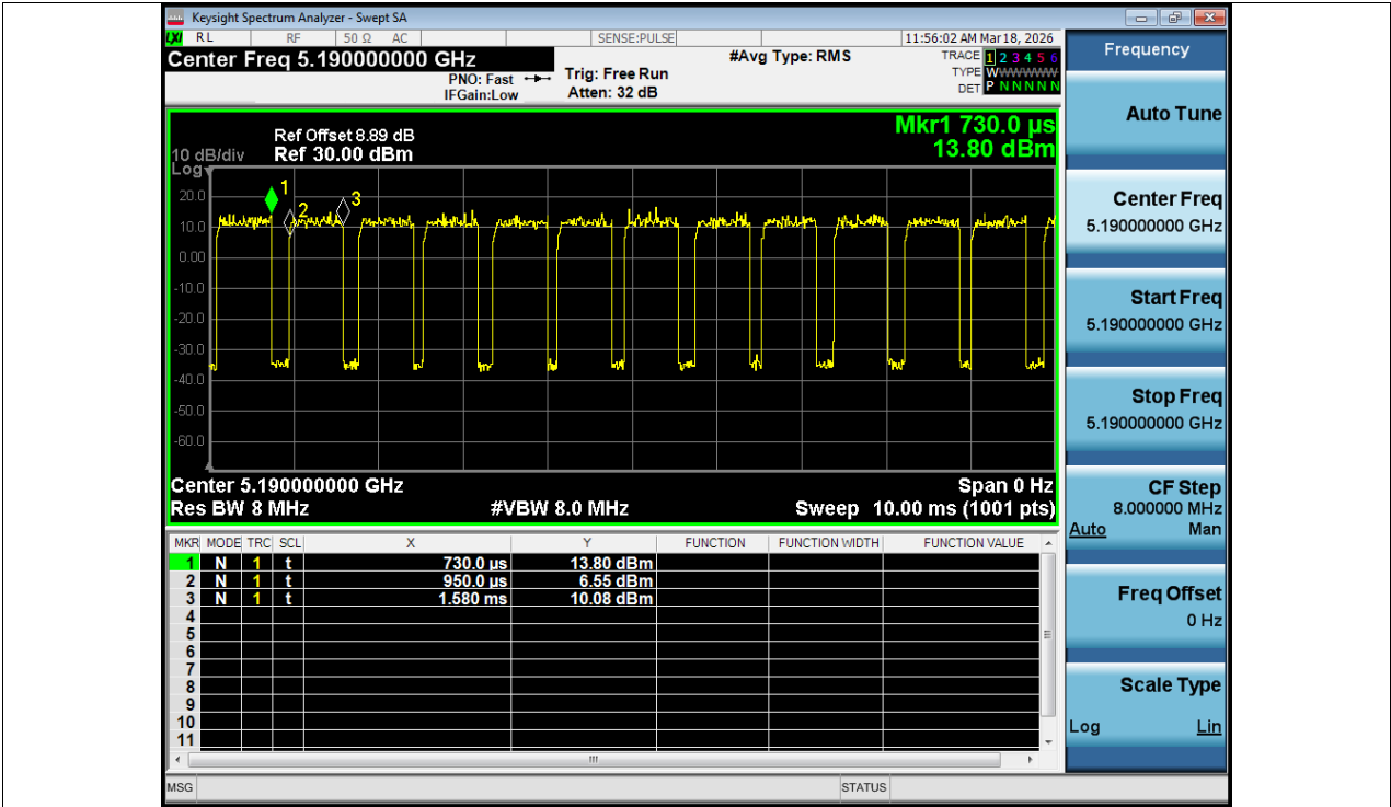
Duty Cycle NVNT ac40 5190MHz Ant1
