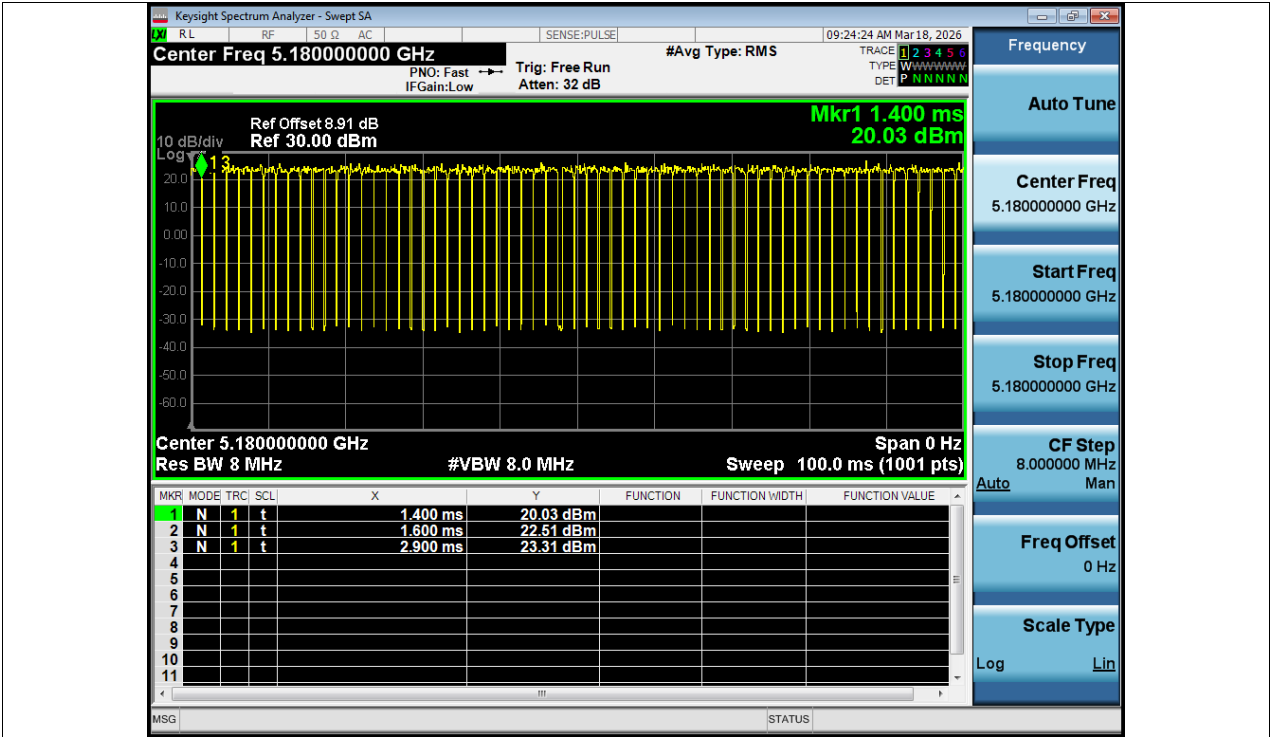
Duty Cycle NVNT a 5180MHz Ant1
