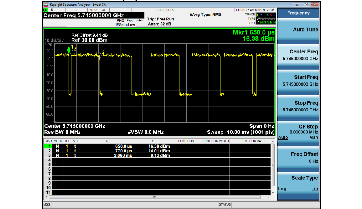
Duty Cycle NVNT ac20 5745MHz Ant1
