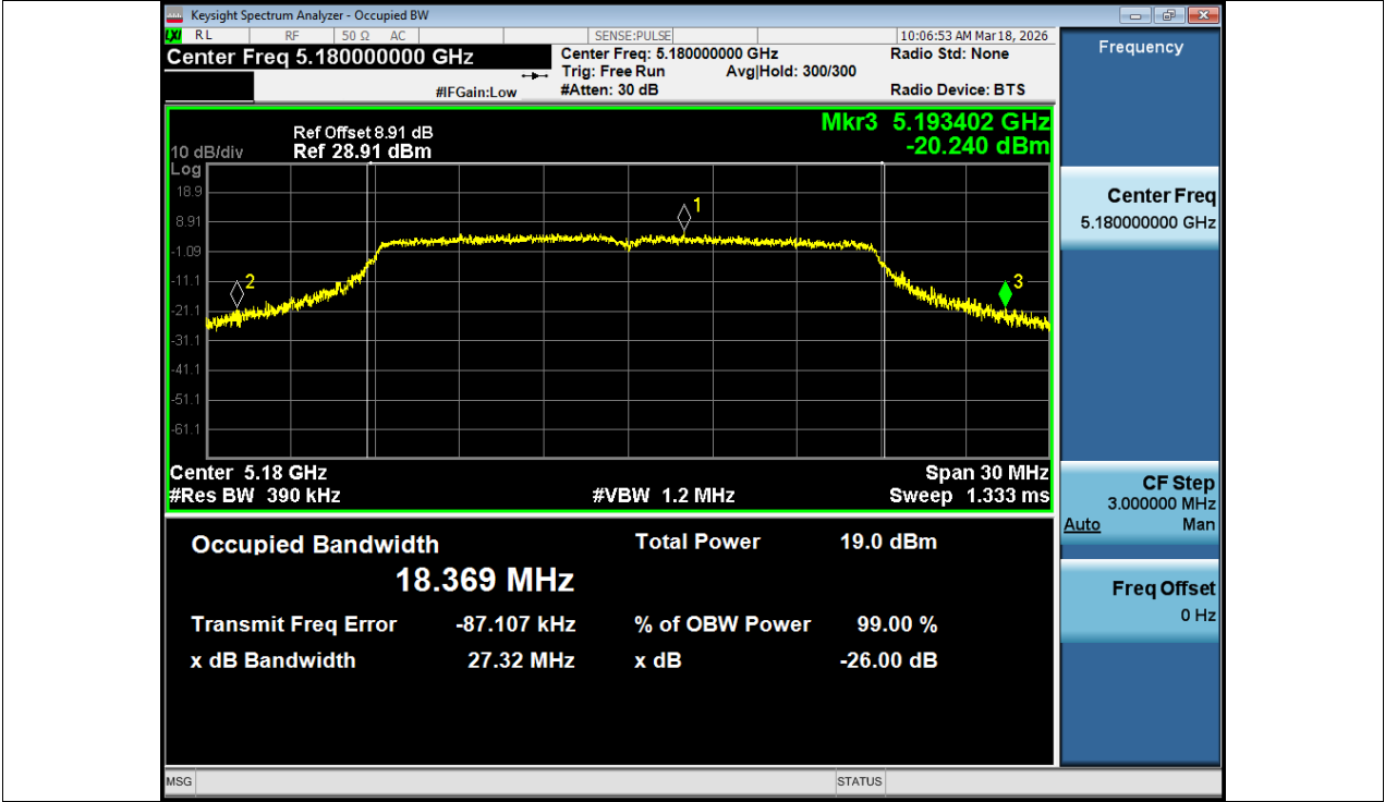
-26dB Bandwidth NVNT n20 5180MHz Ant1
