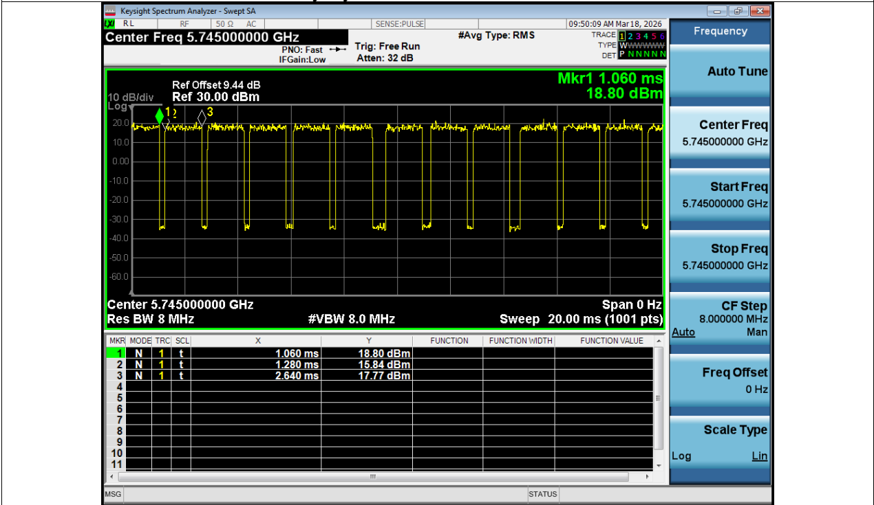
Duty Cycle NVNT a 5745MHz Ant1
