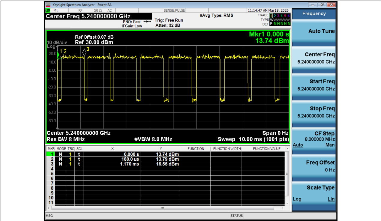
Duty Cycle NVNT ax20 5240MHz Ant1
