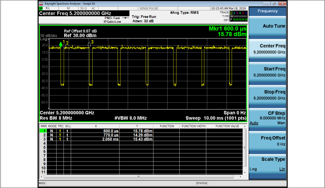
Duty Cycle NVNT n20 5200MHz Ant1
