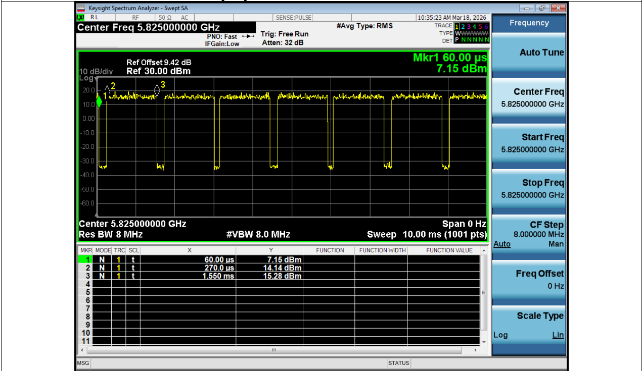
Duty Cycle NVNT n20 5825MHz Ant1
