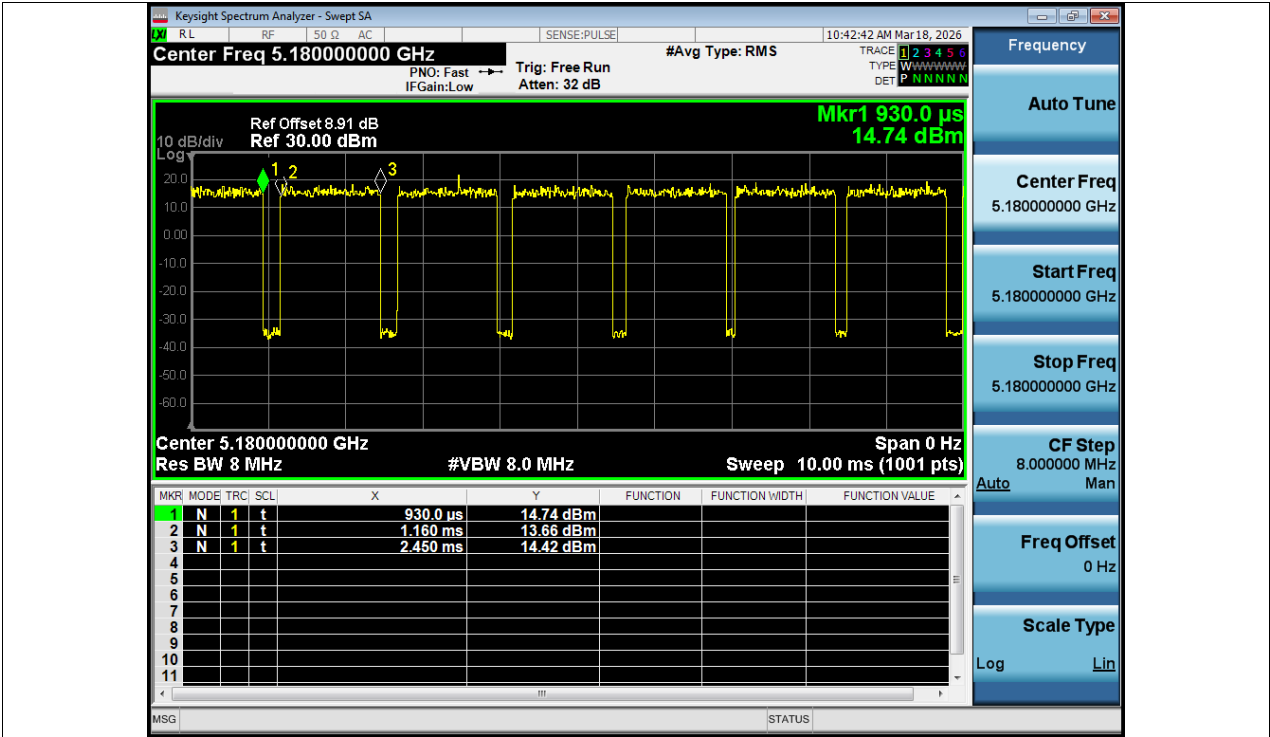
Duty Cycle NVNT ac20 5180MHz Ant1
