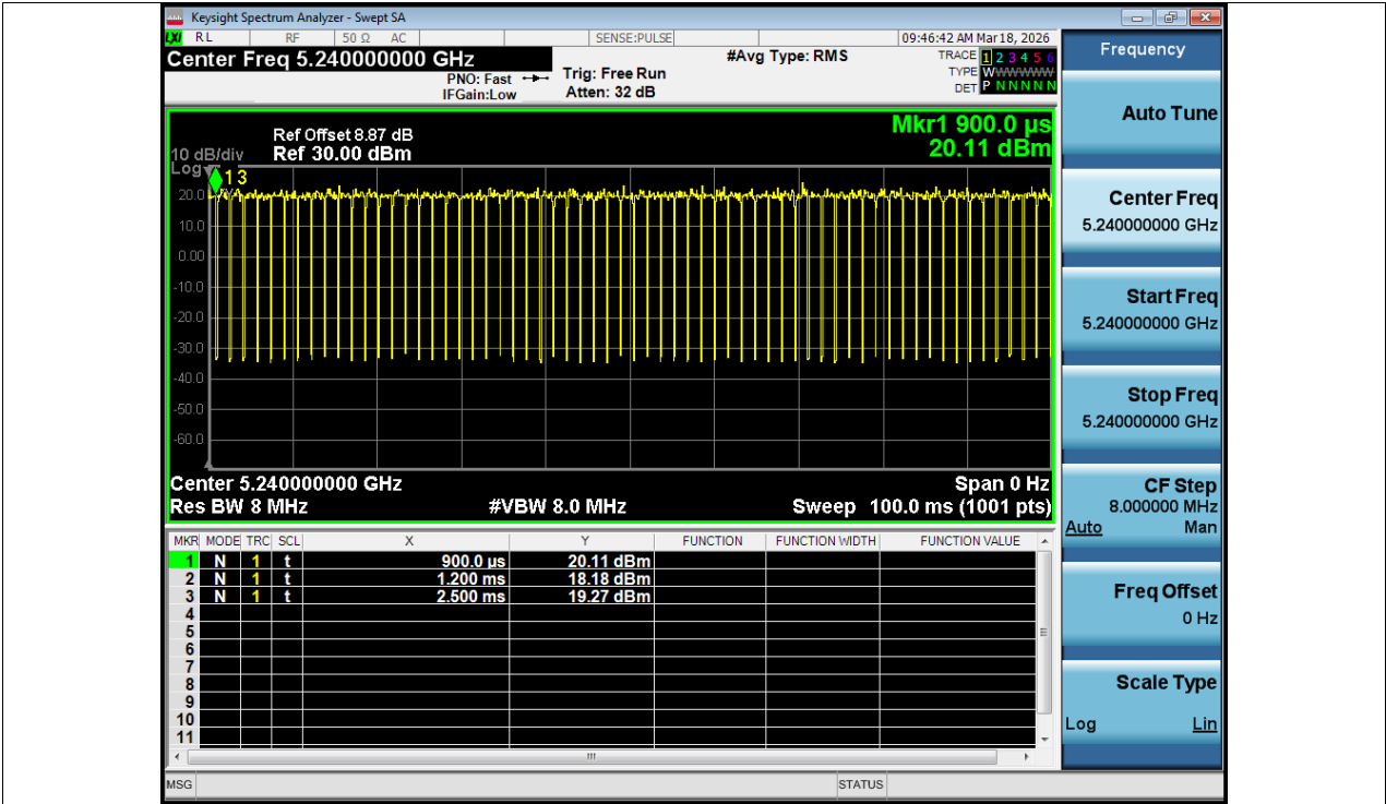
Duty Cycle NVNT a 5240MHz Ant1
