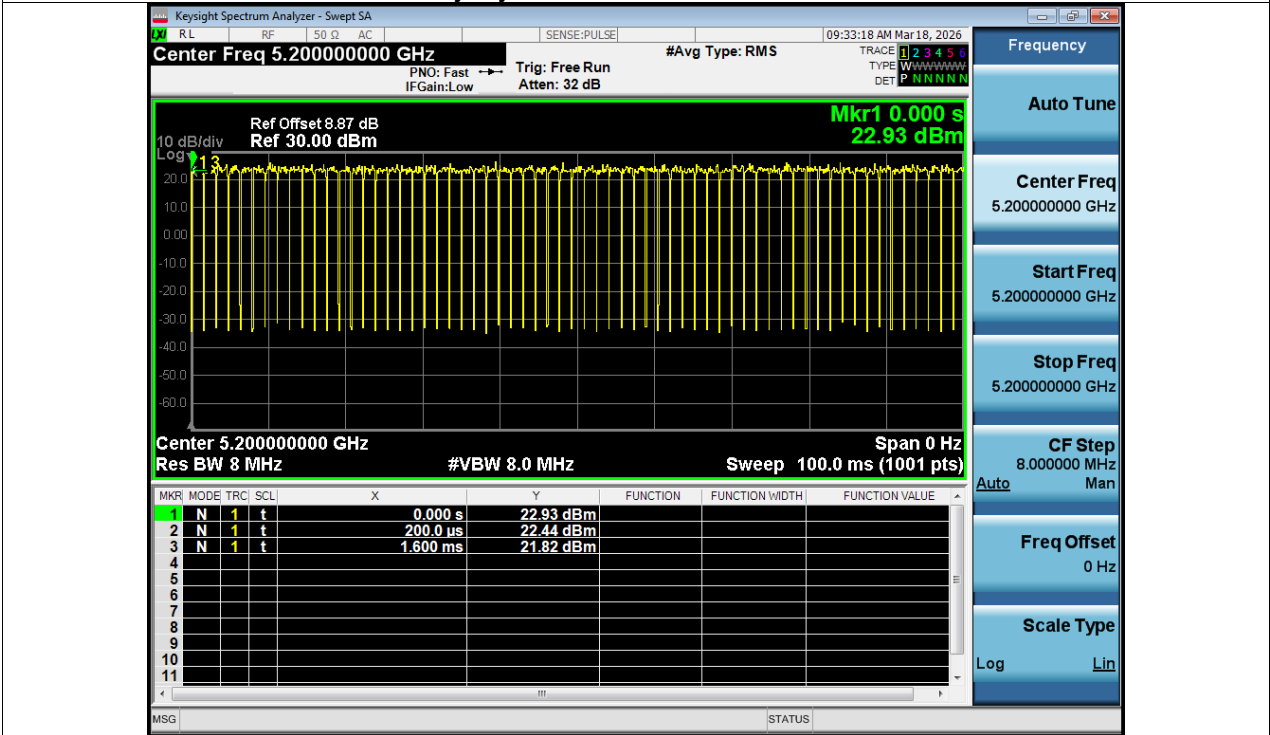
Duty Cycle NVNT a 5200MHz Ant1
