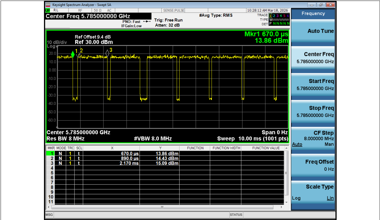
Duty Cycle NVNT n20 5785MHz Ant1
