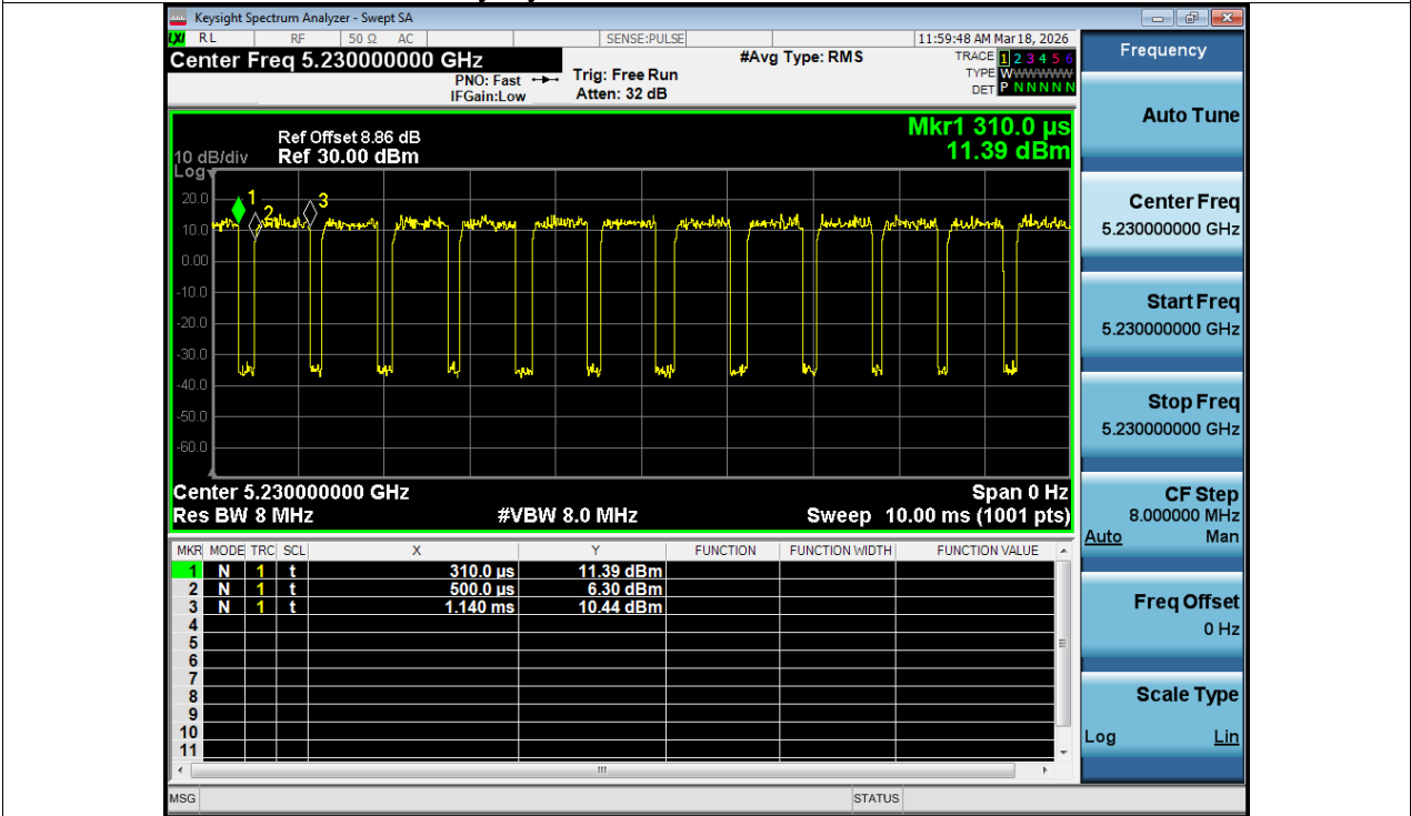
Duty Cycle NVNT ac40 5230MHz Ant1
