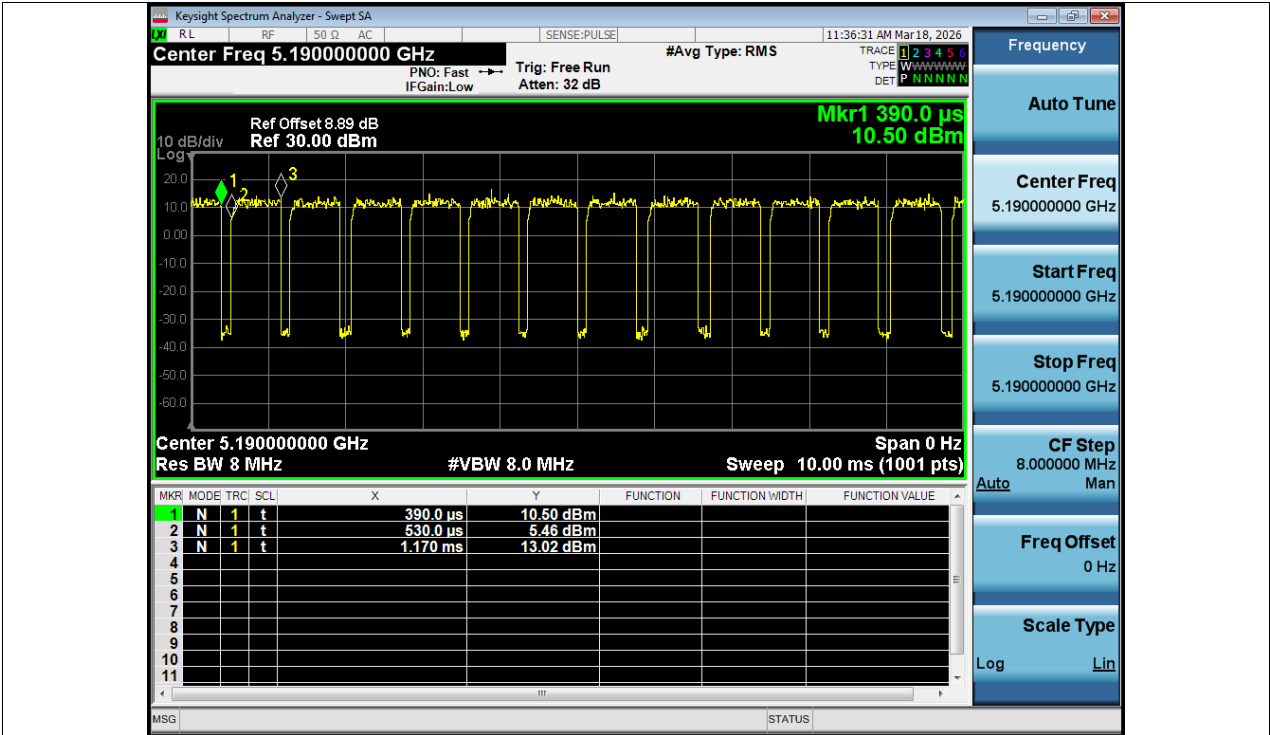
Duty Cycle NVNT n40 5190MHz Ant1
