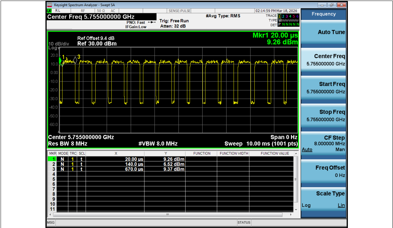
Duty Cycle NVNT ax40 5755MHz Ant1
