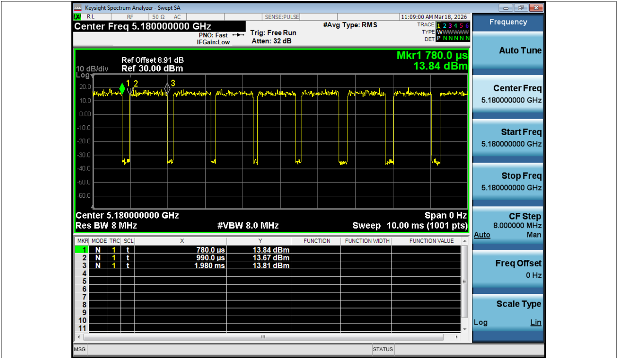
Duty Cycle NVNT ax20 5180MHz Ant1
