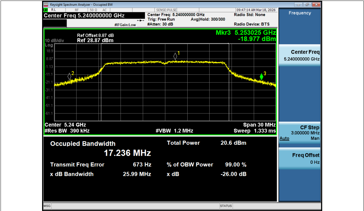
-26dB Bandwidth NVNT a 5240MHz Ant1
