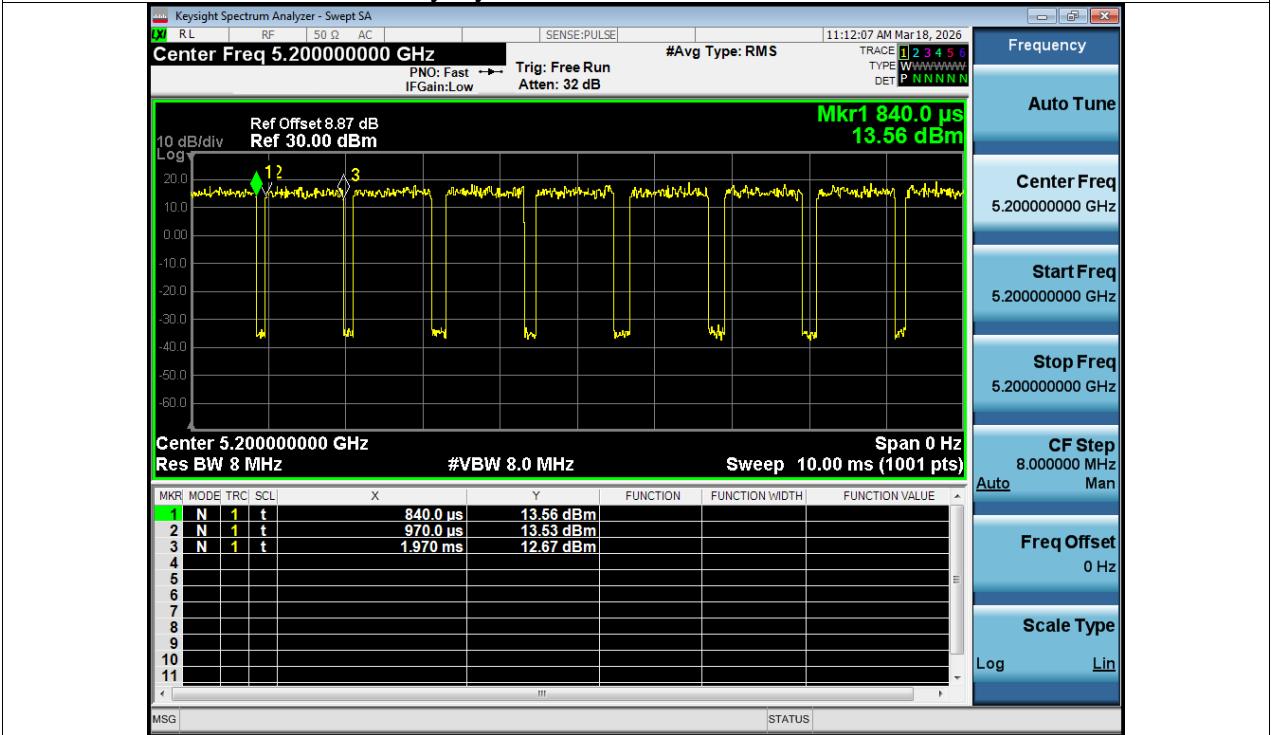
Duty Cycle NVNT ax20 5200MHz Ant1
