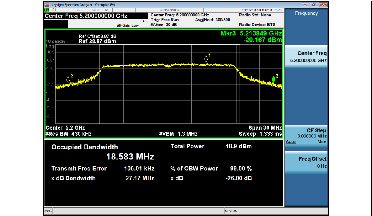
-26dB Bandwidth NVNT n20 5200MHz Ant1
