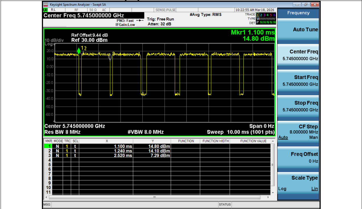
Duty Cycle NVNT n20 5745MHz Ant1
