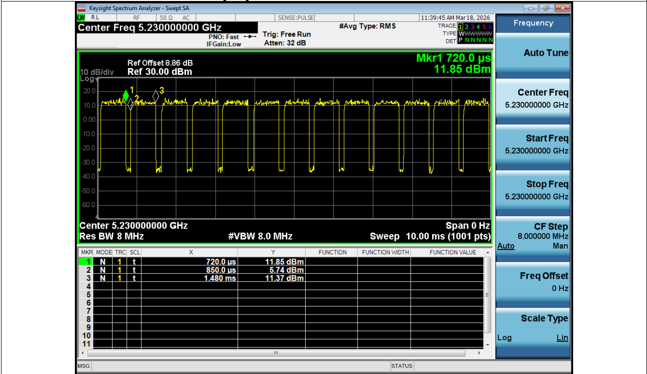
Duty Cycle NVNT n40 5230MHz Ant1
