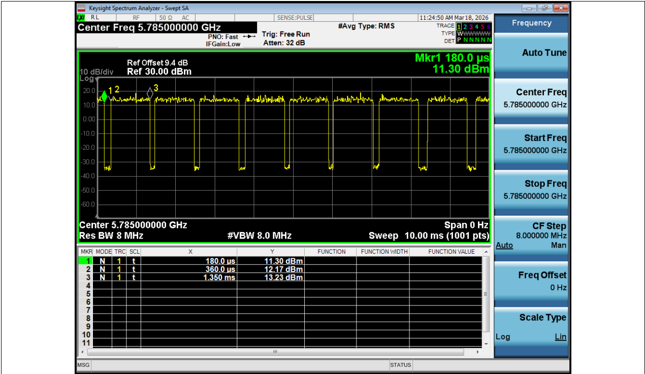
Duty Cycle NVNT ax20 5785MHz Ant1
