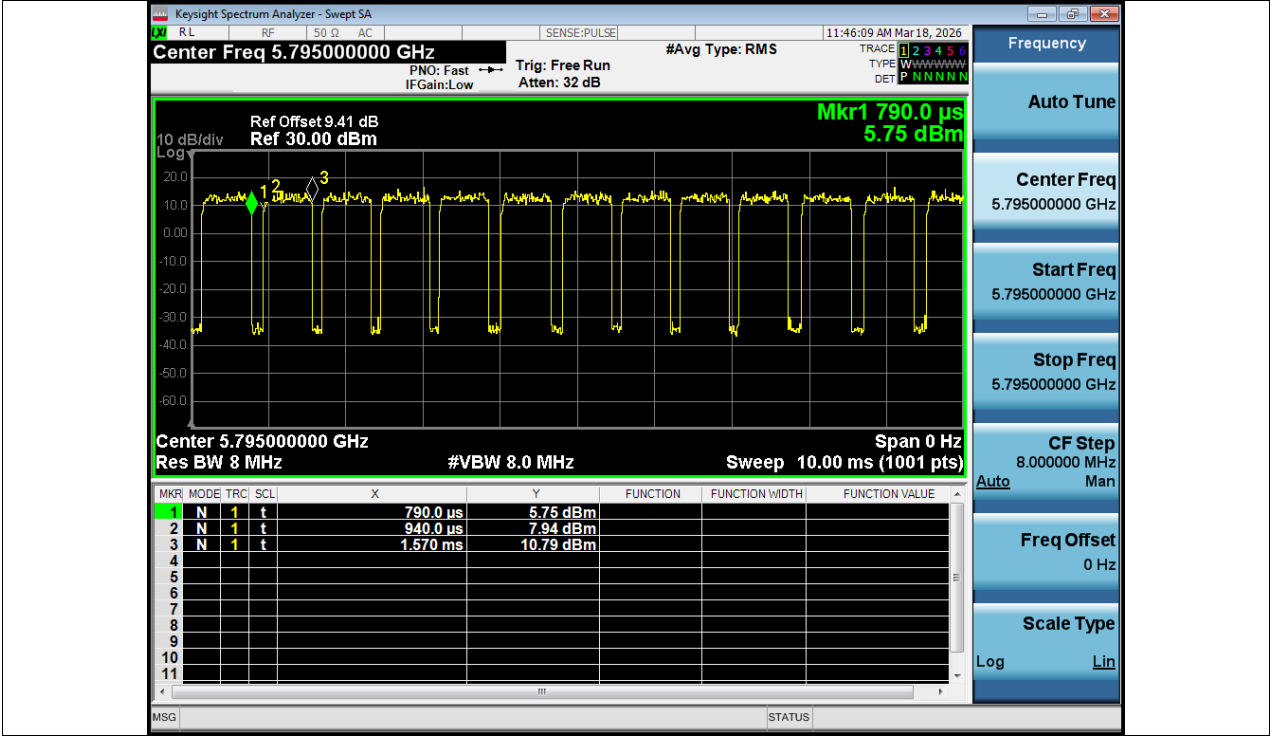
Duty Cycle NVNT n40 5795MHz Ant1
