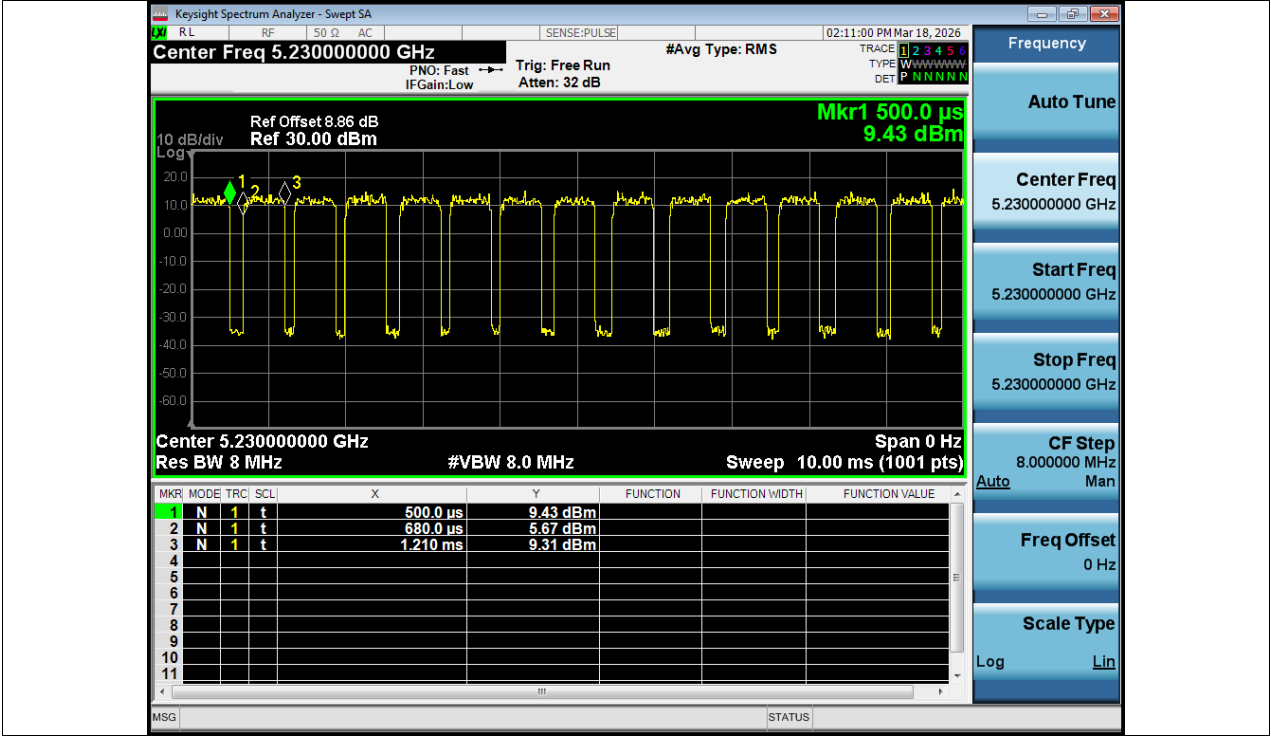
Duty Cycle NVNT ax40 5230MHz Ant1
