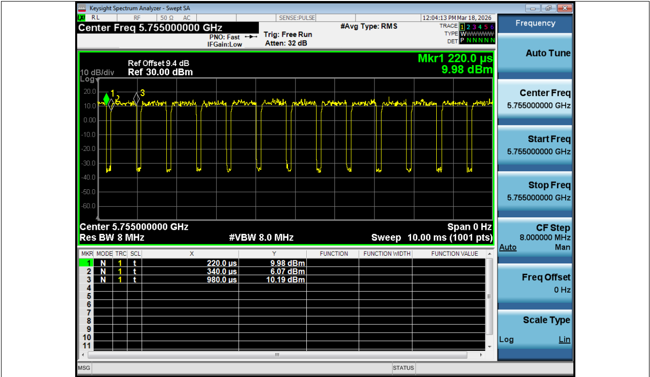
Duty Cycle NVNT ac40 5755MHz Ant1
