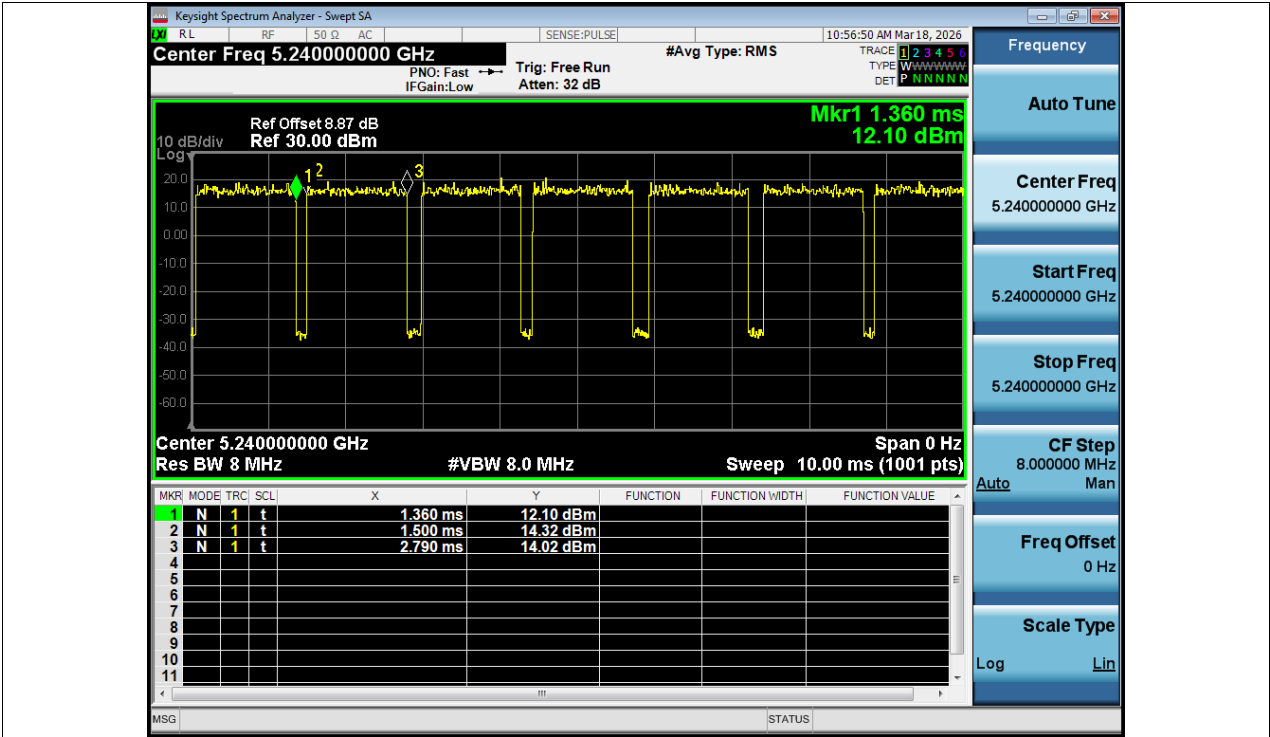
Duty Cycle NVNT ac20 5240MHz Ant1
