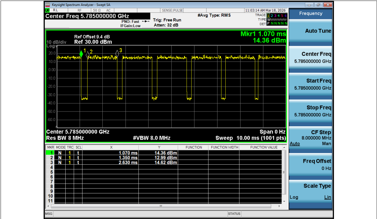
Duty Cycle NVNT ac20 5785MHz Ant1
