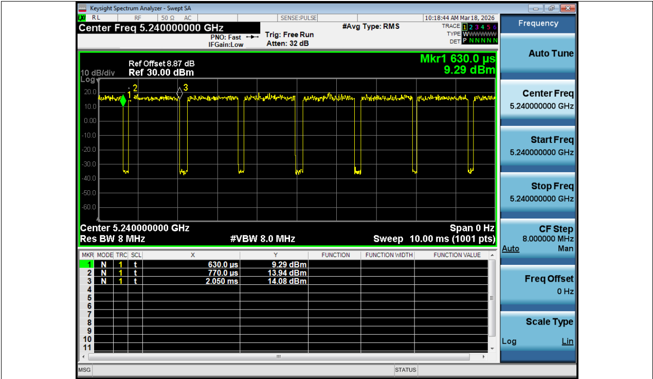
Duty Cycle NVNT n20 5240MHz Ant1
