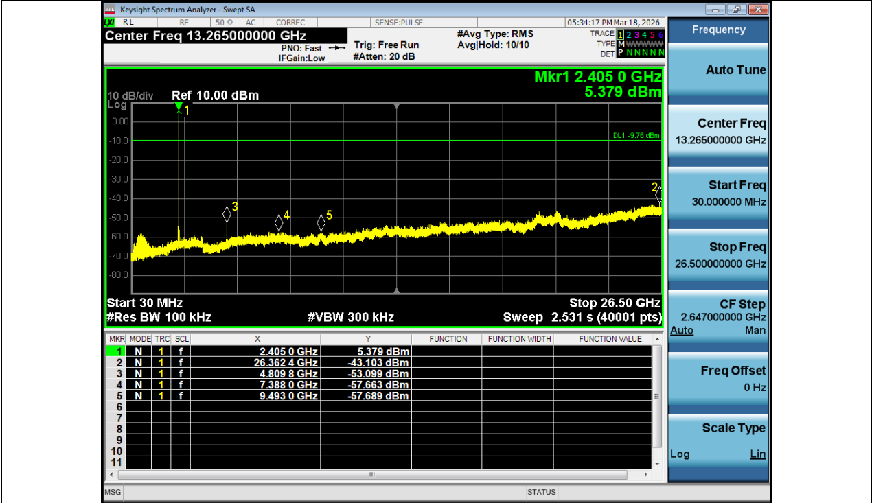
Tx. Spurious NVNT Zigbee 2405MHz Ant1 Emission
