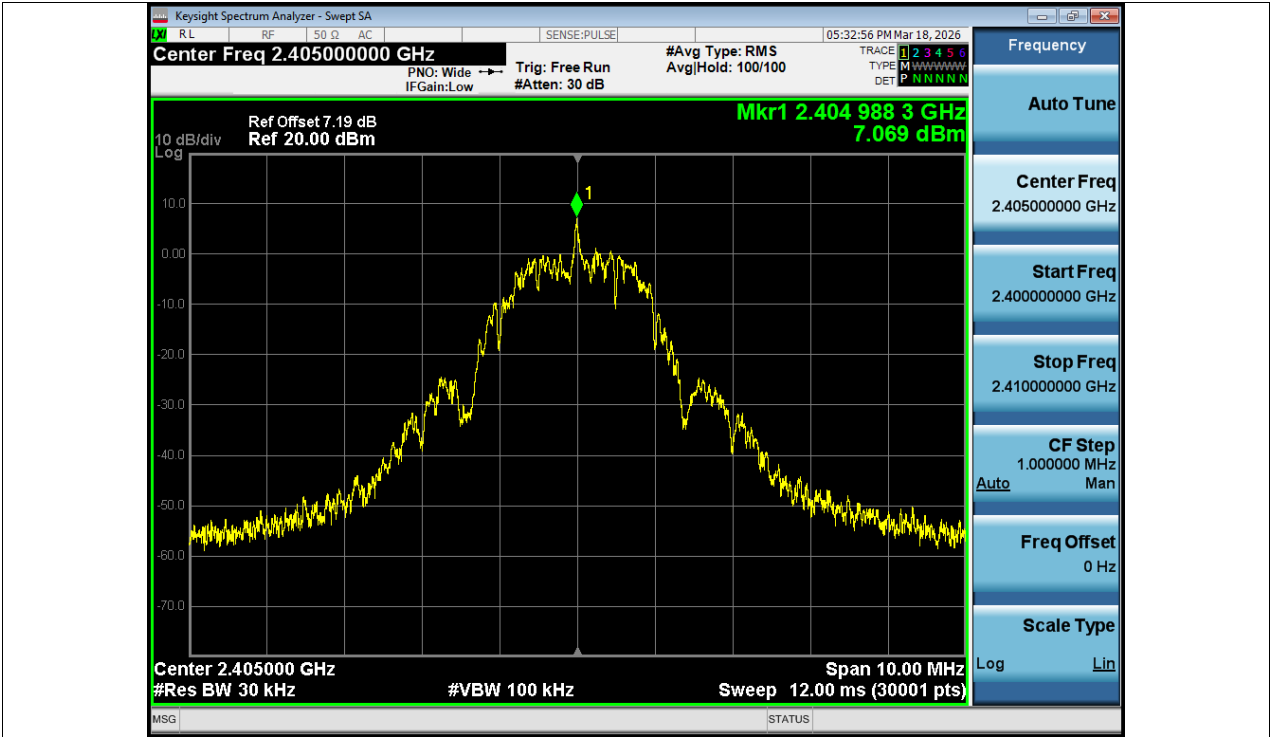
PSD NVNT Zigbee 2405MHz Ant1
