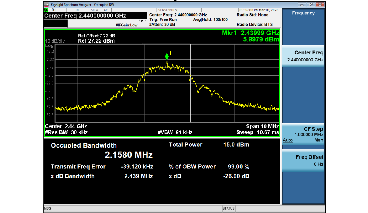
OBW NVNT Zigbee 2440MHz Ant1
