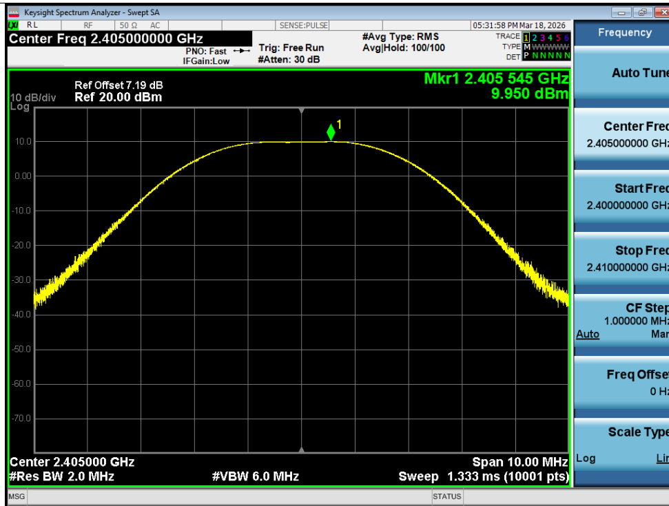
Peak Power NVNT Zigbee 2405MHz Ant1
