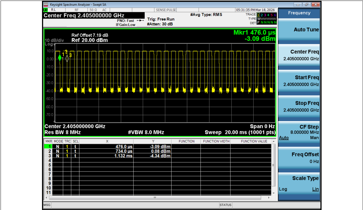
Duty Cycle NVNT Zigbee 2405MHz Ant1
