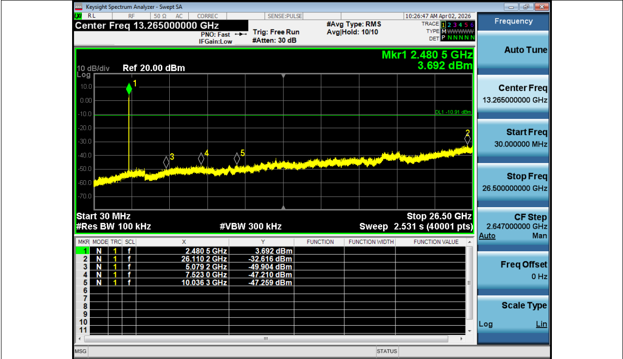
Tx. Spurious NVNT Zigbee 2480MHz Ant1 Emission
