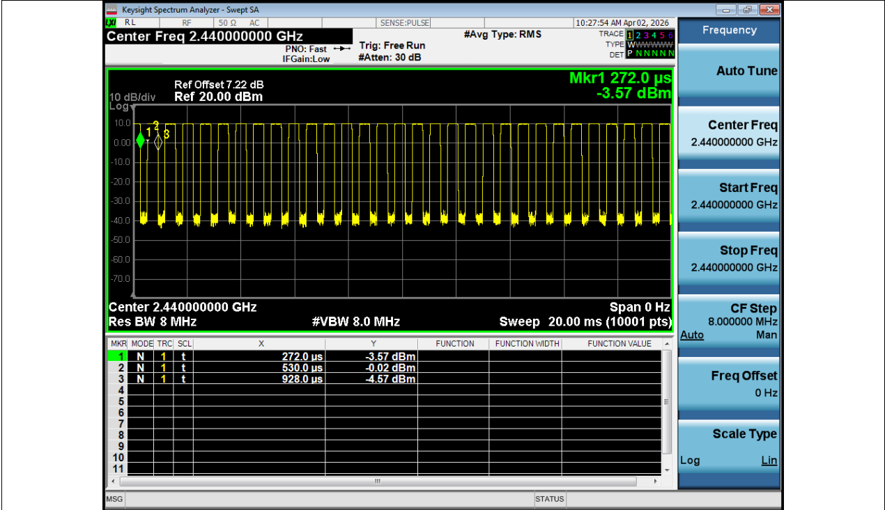
Duty Cycle NVNT Zigbee 2440MHz Ant1
