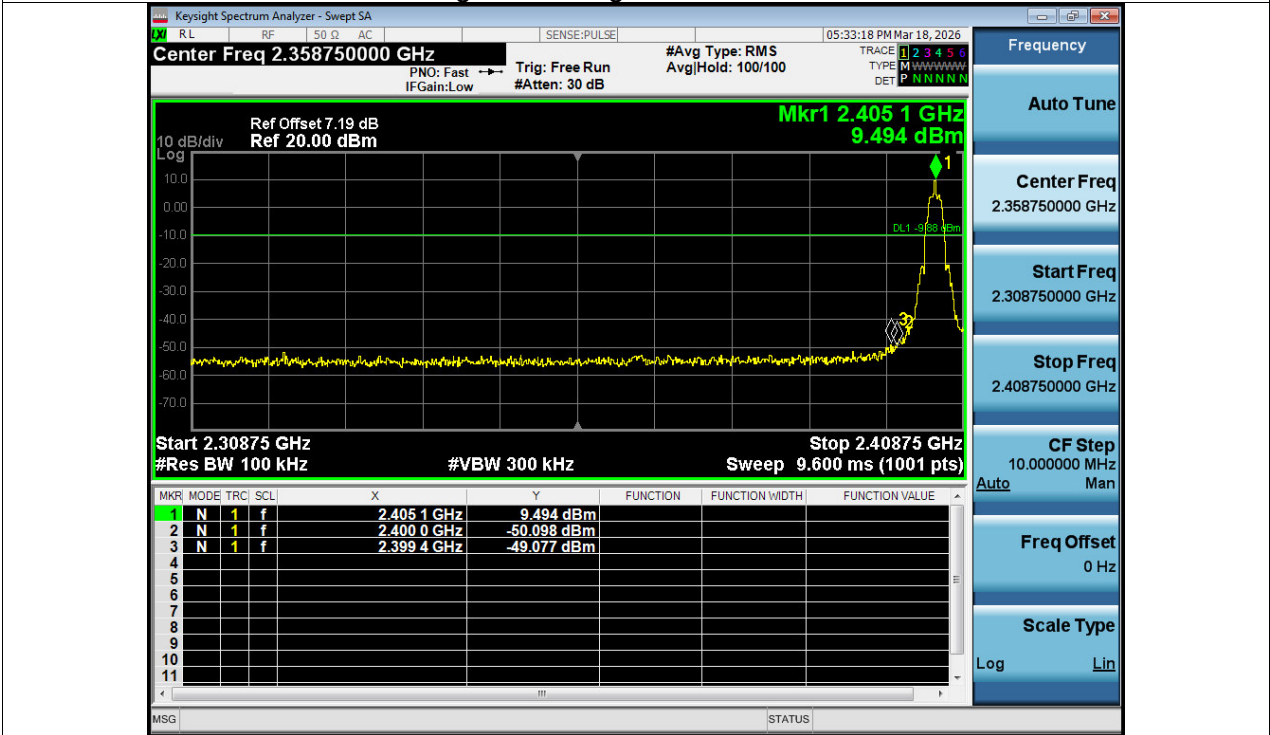
Band Edge NVNT Zigbee 2405MHz Ant1 Emission
