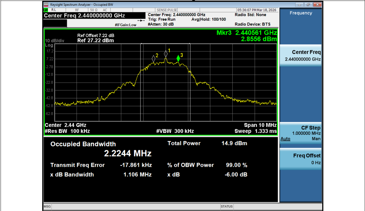
-6dB Bandwidth NVNT Zigbee 2440MHz Ant1
