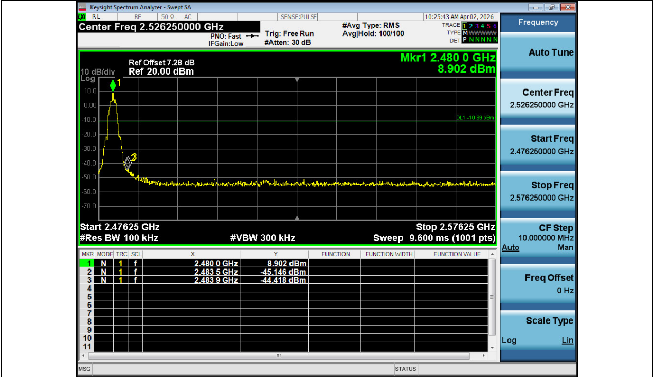
Band Edge NVNT Zigbee 2480MHz Ant1 Emission
