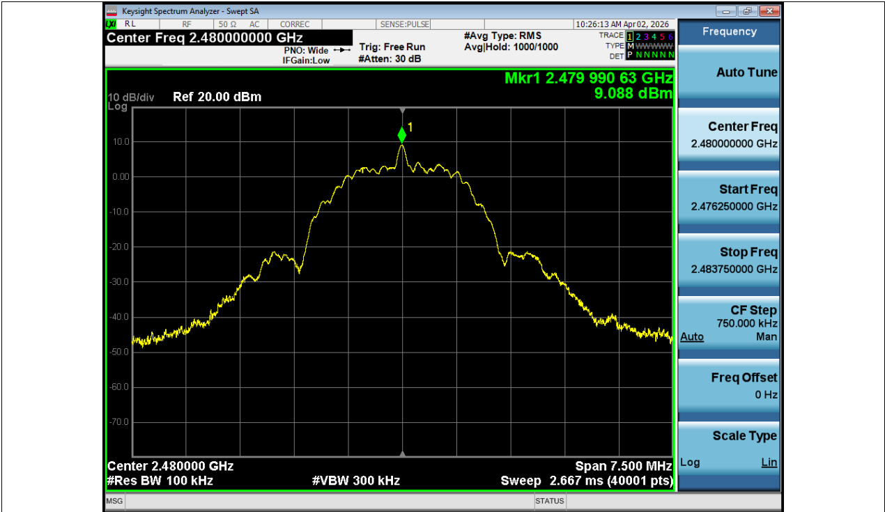
Tx. Spurious NVNT Zigbee 2480MHz Ant1 Ref
