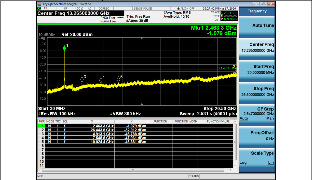
Tx. Spurious NVNT ax20 2462MHz Ant1 Emission
