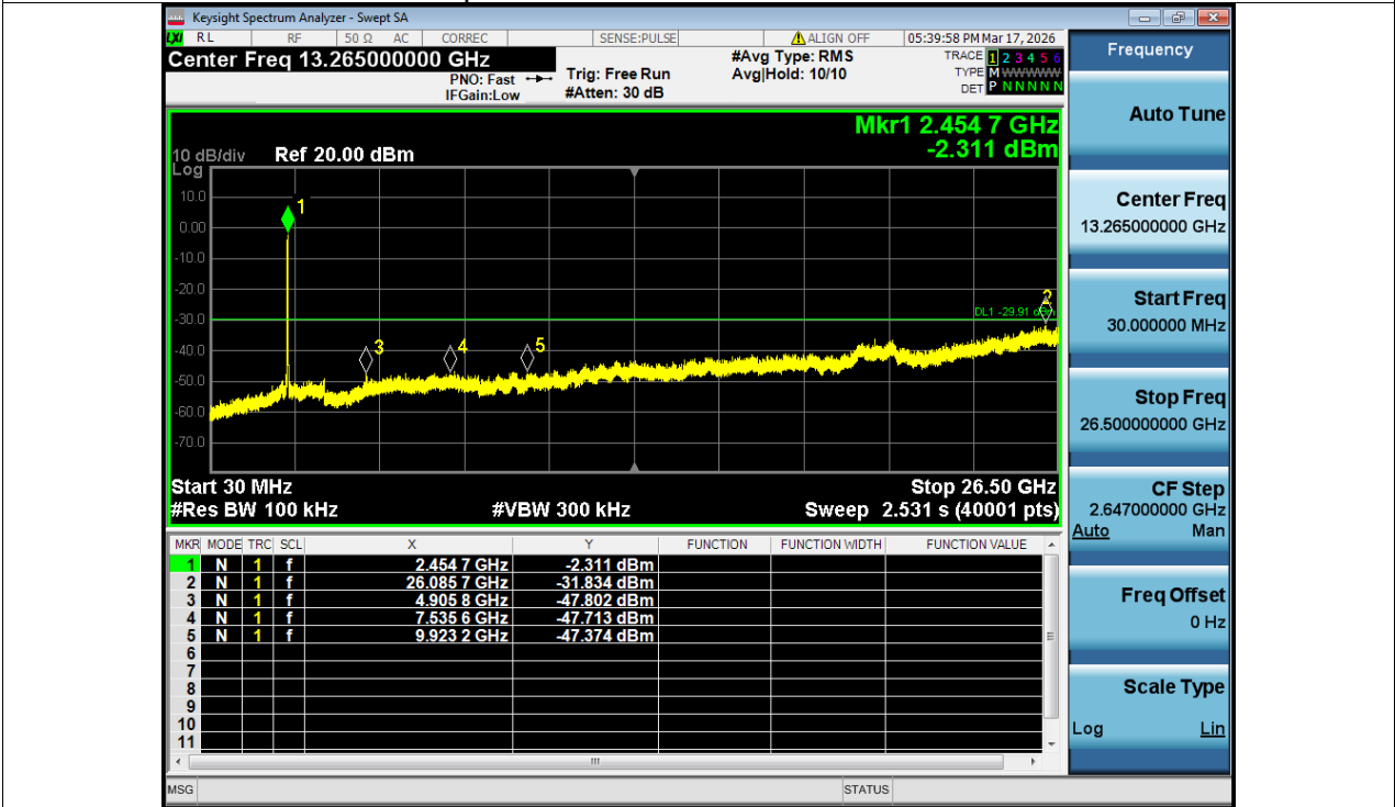
Tx. Spurious NVNT n40 2452MHz Ant1 Emission
