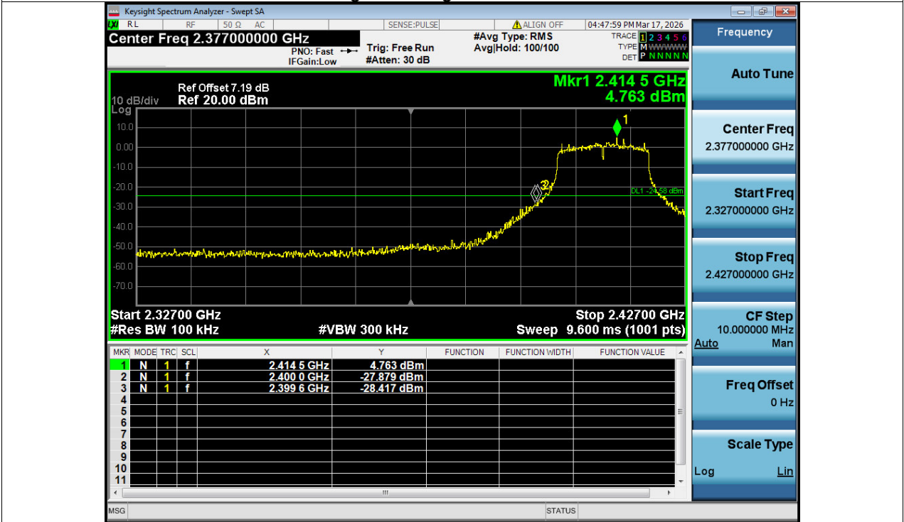
Band Edge NVNT g 2412MHz Ant1 Emission
