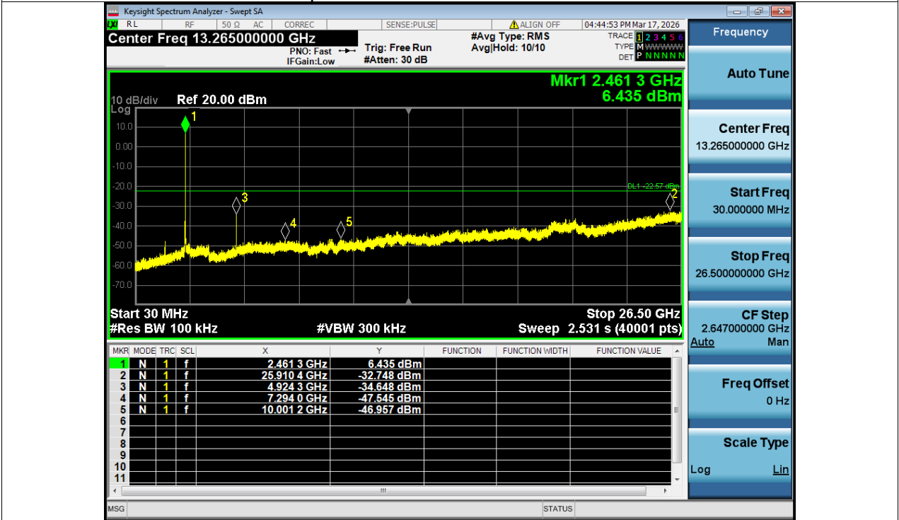
Tx. Spurious NVNT b 2462MHz Ant1 Emission
