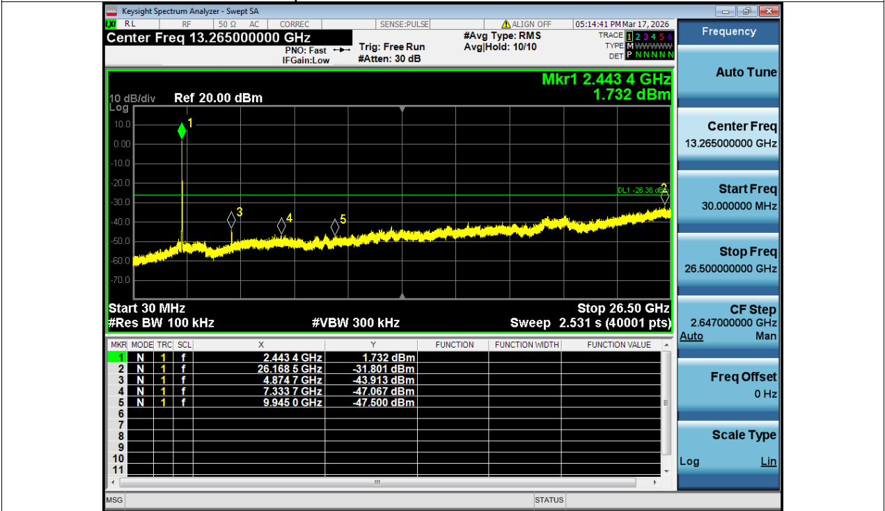
Tx. Spurious NVNT n20 2437MHz Ant1 Emission
