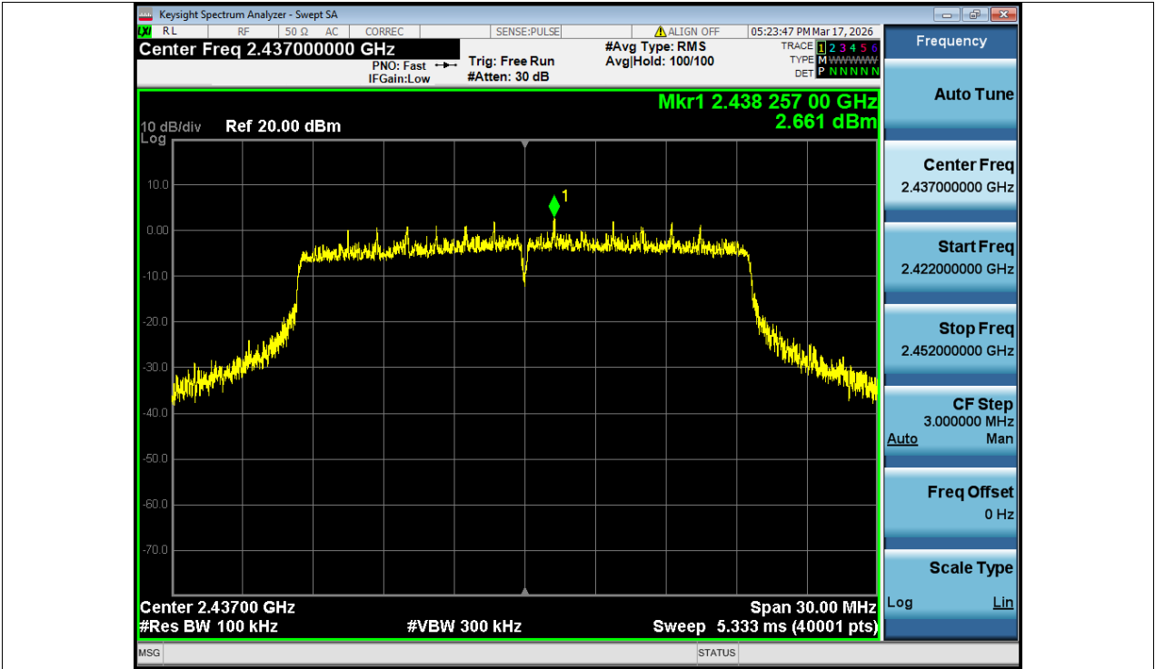
Tx. Spurious NVNT ax20 2437MHz Ant1 Ref
