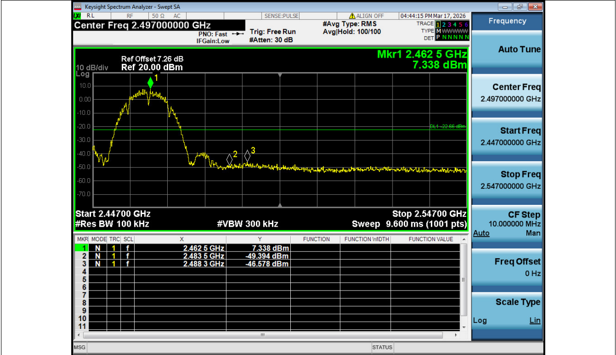
Band Edge NVNT b 2462MHz Ant1 Emission
