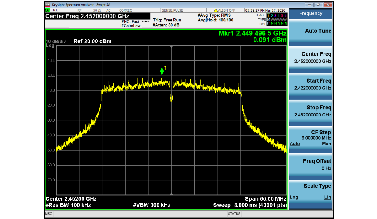
Tx. Spurious NVNT n40 2452MHz Ant1 Ref
