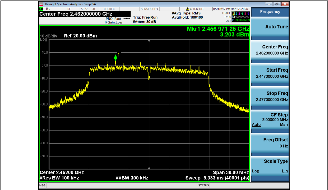
Tx. Spurious NVNT n20 2462MHz Ant1 Ref
