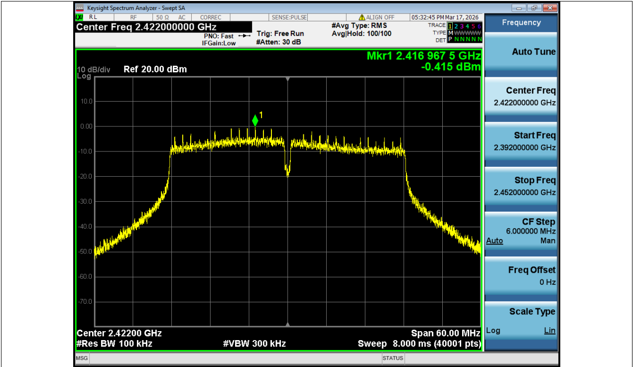
Tx. Spurious NVNT n40 2422MHz Ant1 Ref
