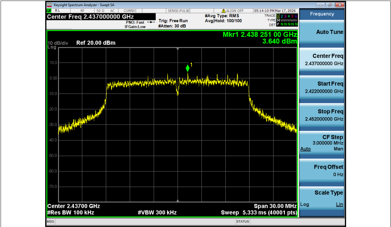
Tx. Spurious NVNT n20 2437MHz Ant1 Ref
