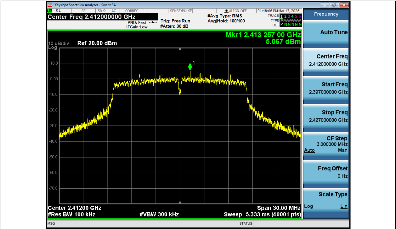
Tx. Spurious NVNT g 2412MHz Ant1 Ref
