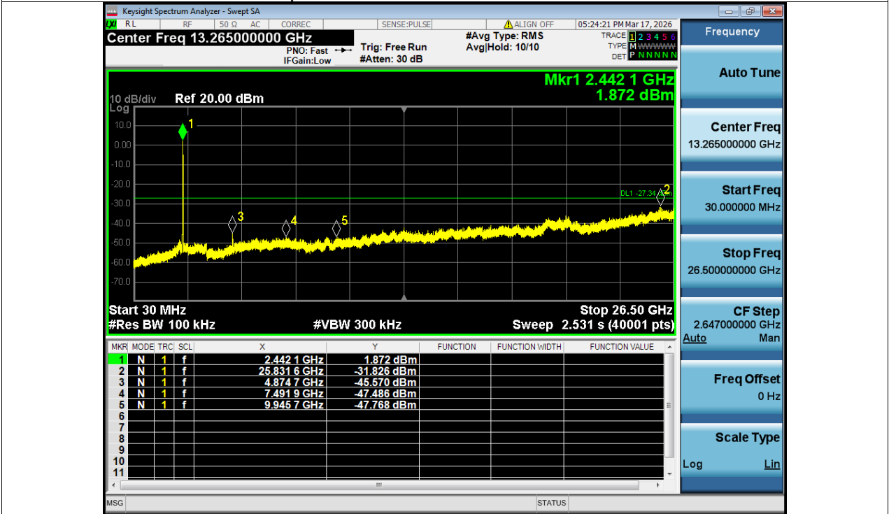
Tx. Spurious NVNT ax20 2437MHz Ant1 Emission
