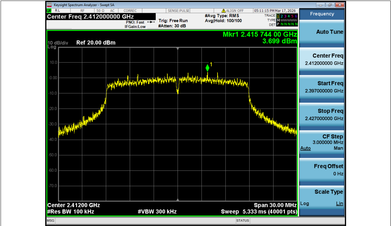
Tx. Spurious NVNT n20 2412MHz Ant1 Ref
