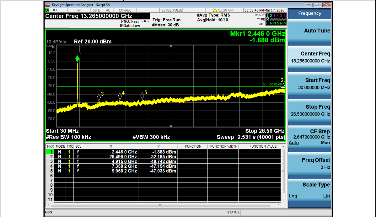
Tx. Spurious NVNT ax40 2452MHz Ant1 Emission
