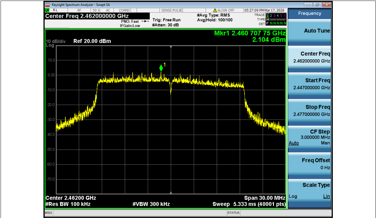
Tx. Spurious NVNT ax20 2462MHz Ant1 Ref
