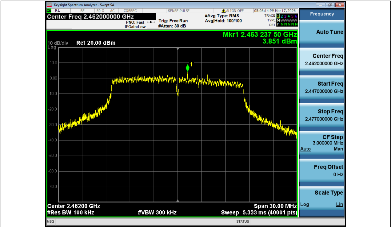
Tx. Spurious NVNT g 2462MHz Ant1 Ref
