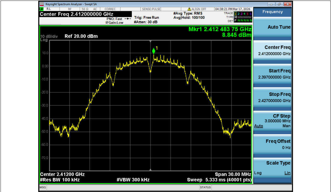
Tx. Spurious NVNT b 2412MHz Ant1 Ref
