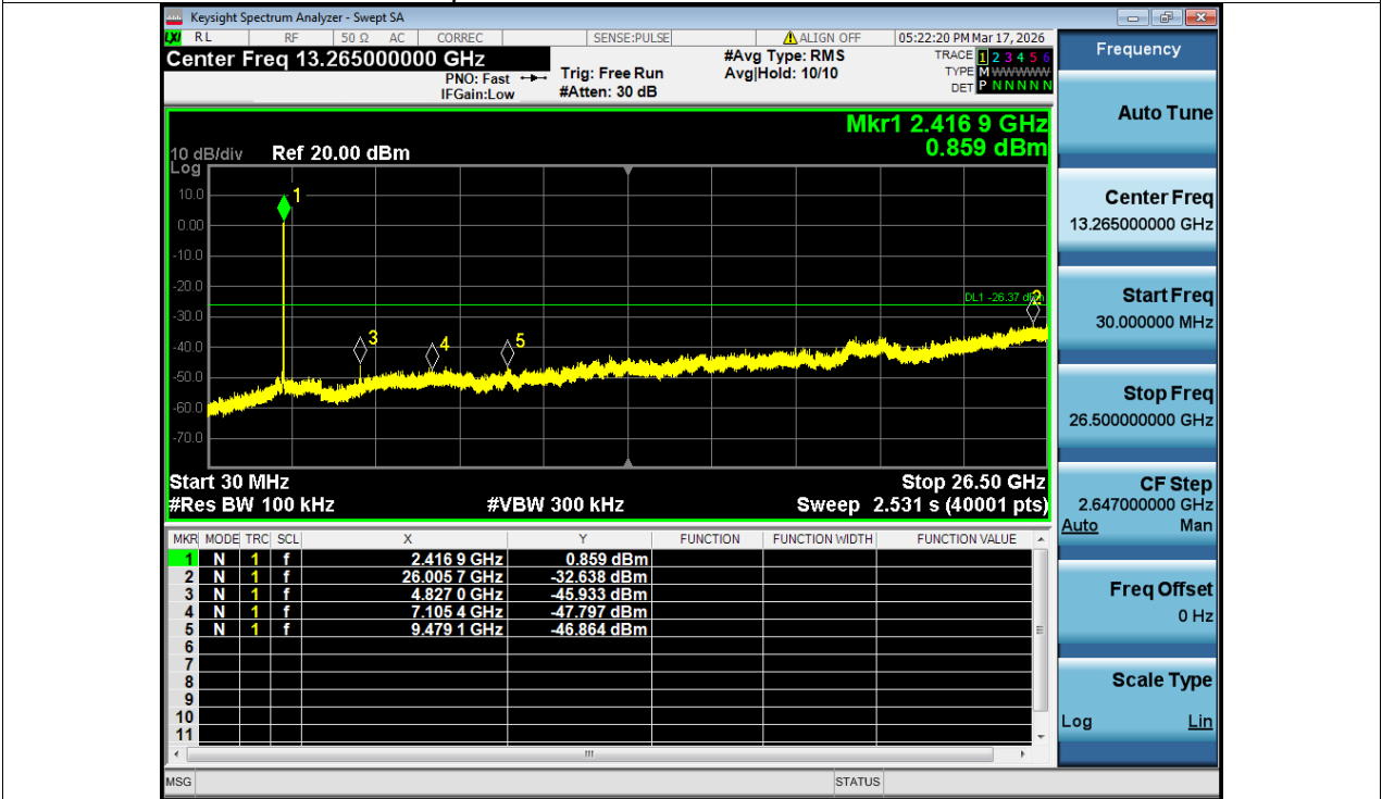
Tx. Spurious NVNT ax20 2412MHz Ant1 Emission
