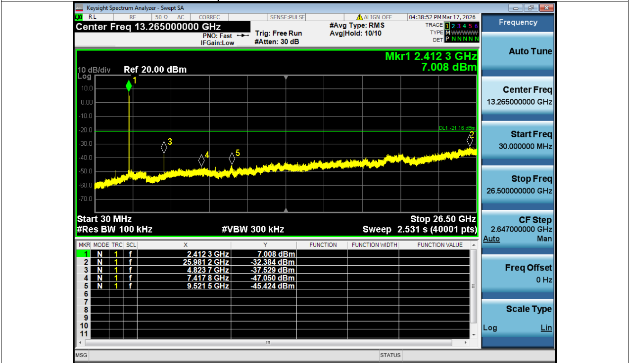
Tx. Spurious NVNT b 2412MHz Ant1 Emission
