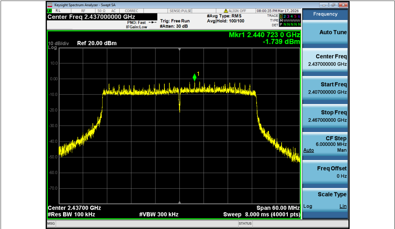
Tx. Spurious NVNT ax40 2437MHz Ant1 Ref
