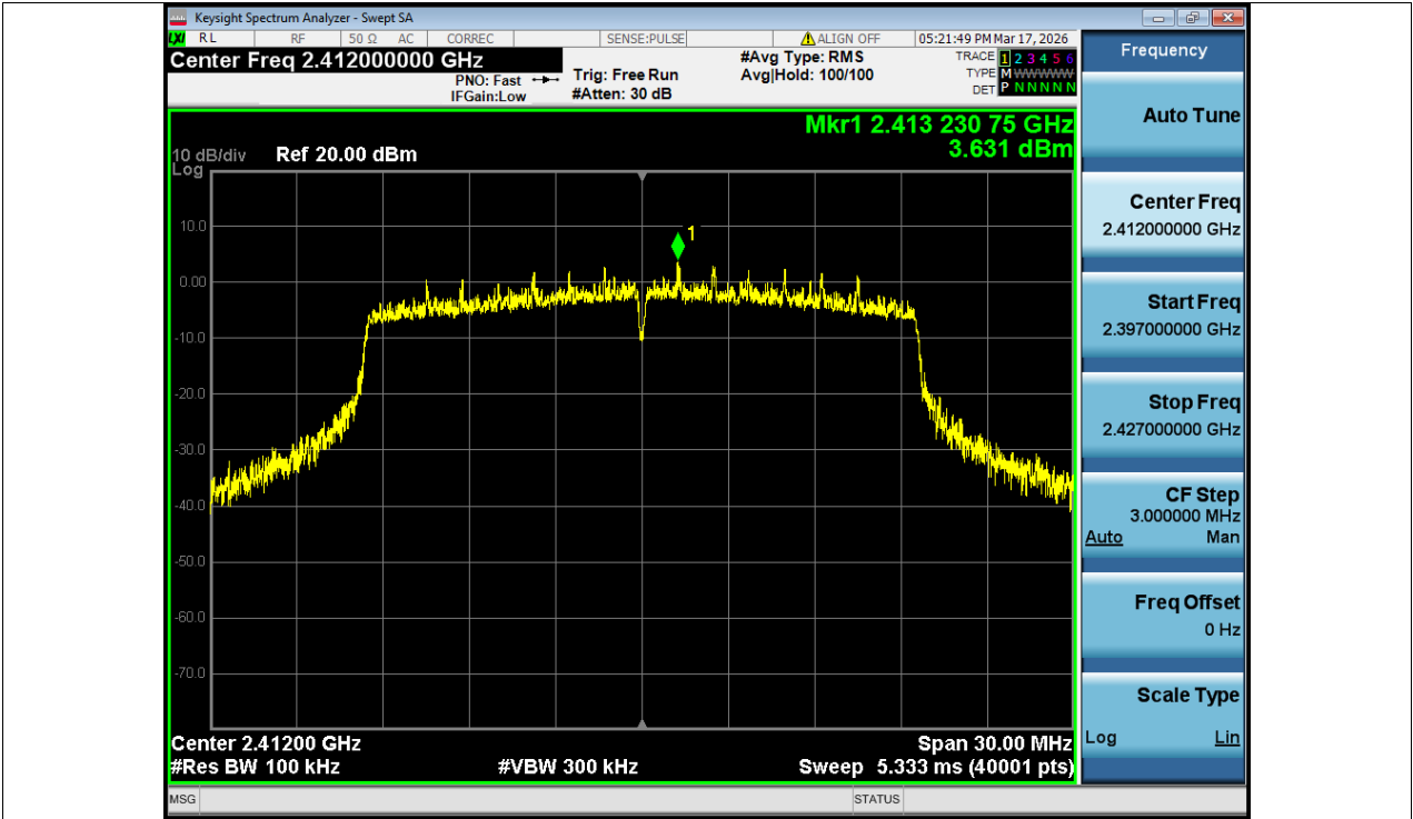
Tx. Spurious NVNT ax20 2412MHz Ant1 Ref
