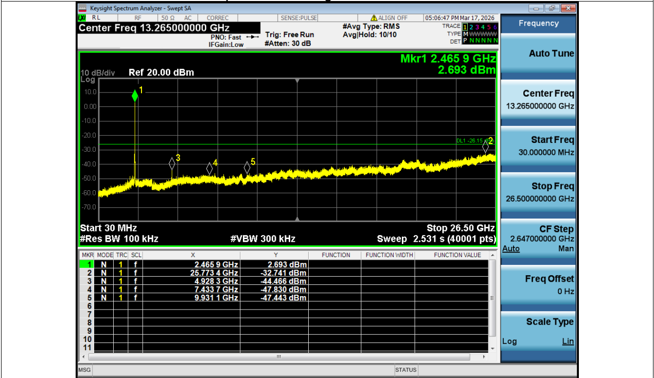
Tx. Spurious NVNT g 2462MHz Ant1 Emission
