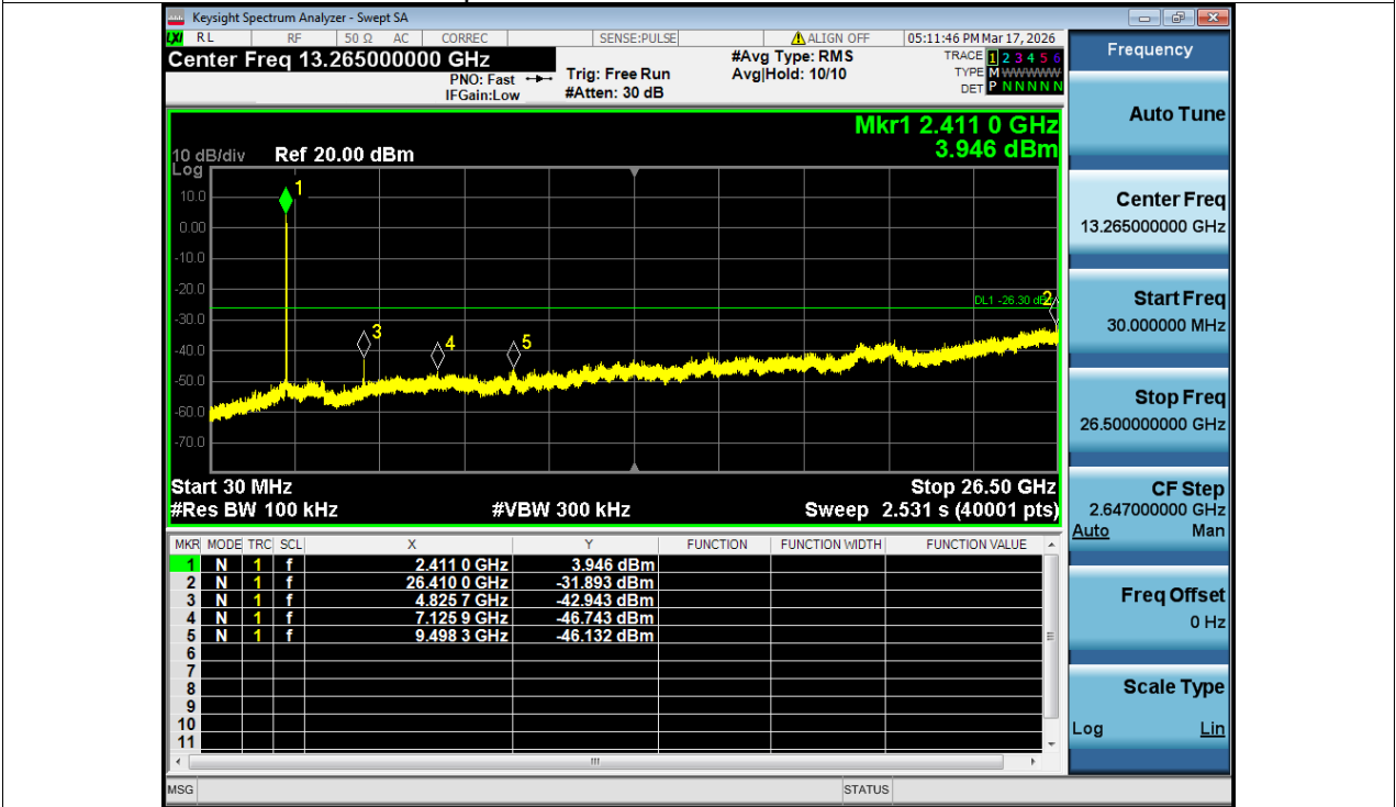
Tx. Spurious NVNT n20 2412MHz Ant1 Emission
