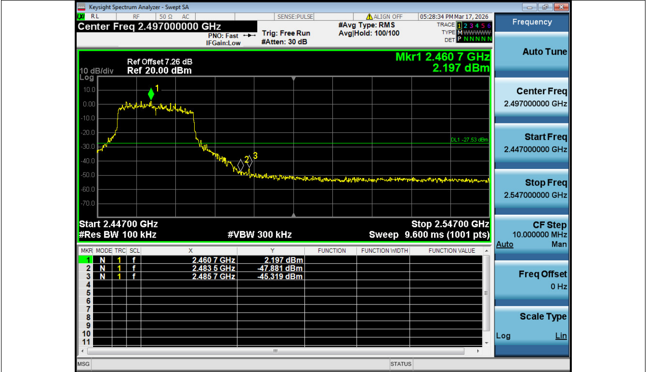
Band Edge NVNT ax20 2462MHz Ant1 Emission
