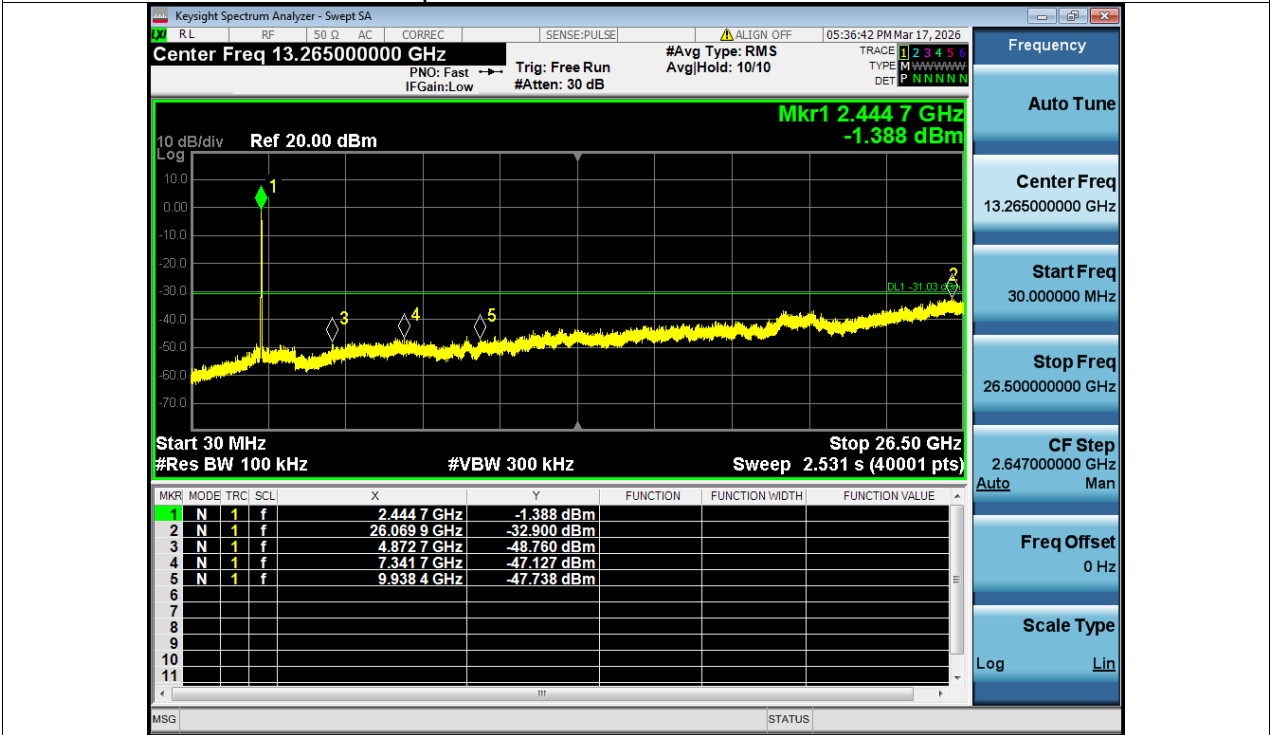
Tx. Spurious NVNT n40 2437MHz Ant1 Emission
