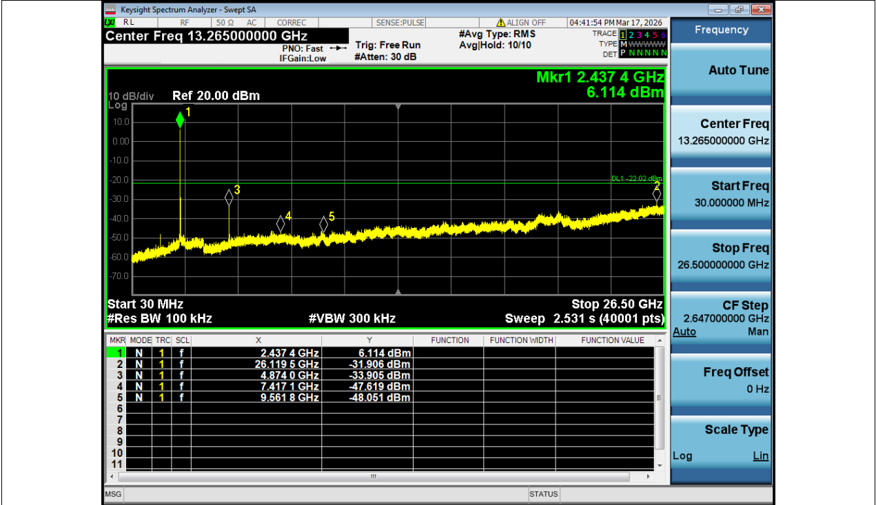
Tx. Spurious NVNT b 2437MHz Ant1 Emission
