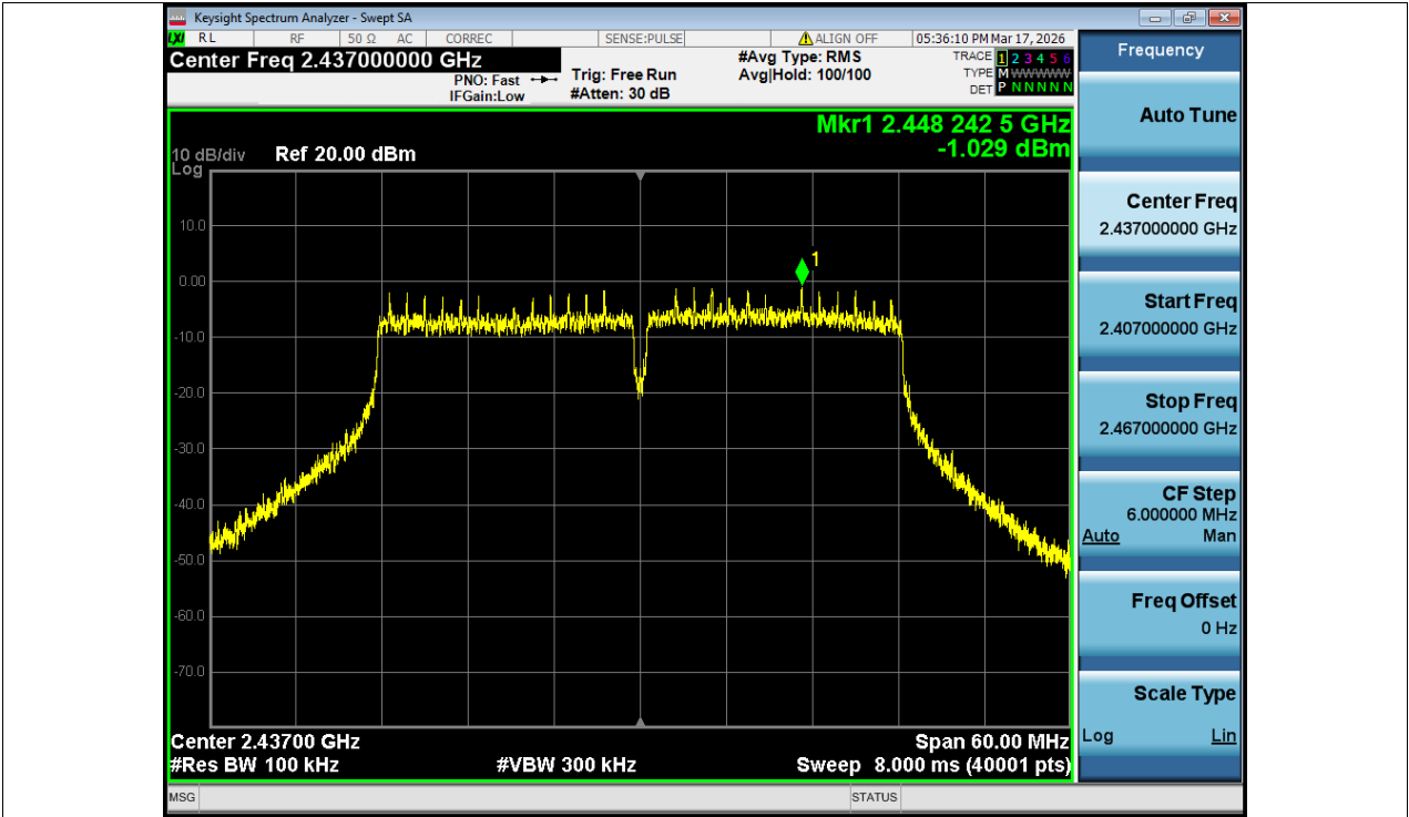
Tx. Spurious NVNT n40 2437MHz Ant1 Ref
