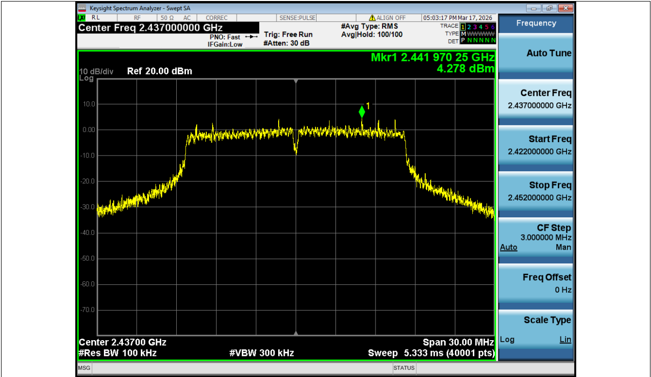
Tx. Spurious NVNT g 2437MHz Ant1 Ref
