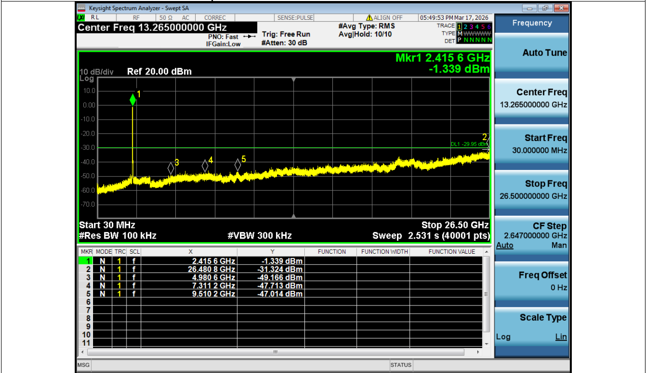
Tx. Spurious NVNT ax40 2422MHz Ant1 Emission
