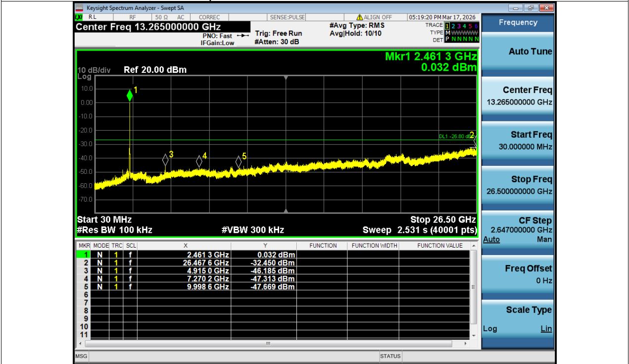
Tx. Spurious NVNT n20 2462MHz Ant1 Emission
