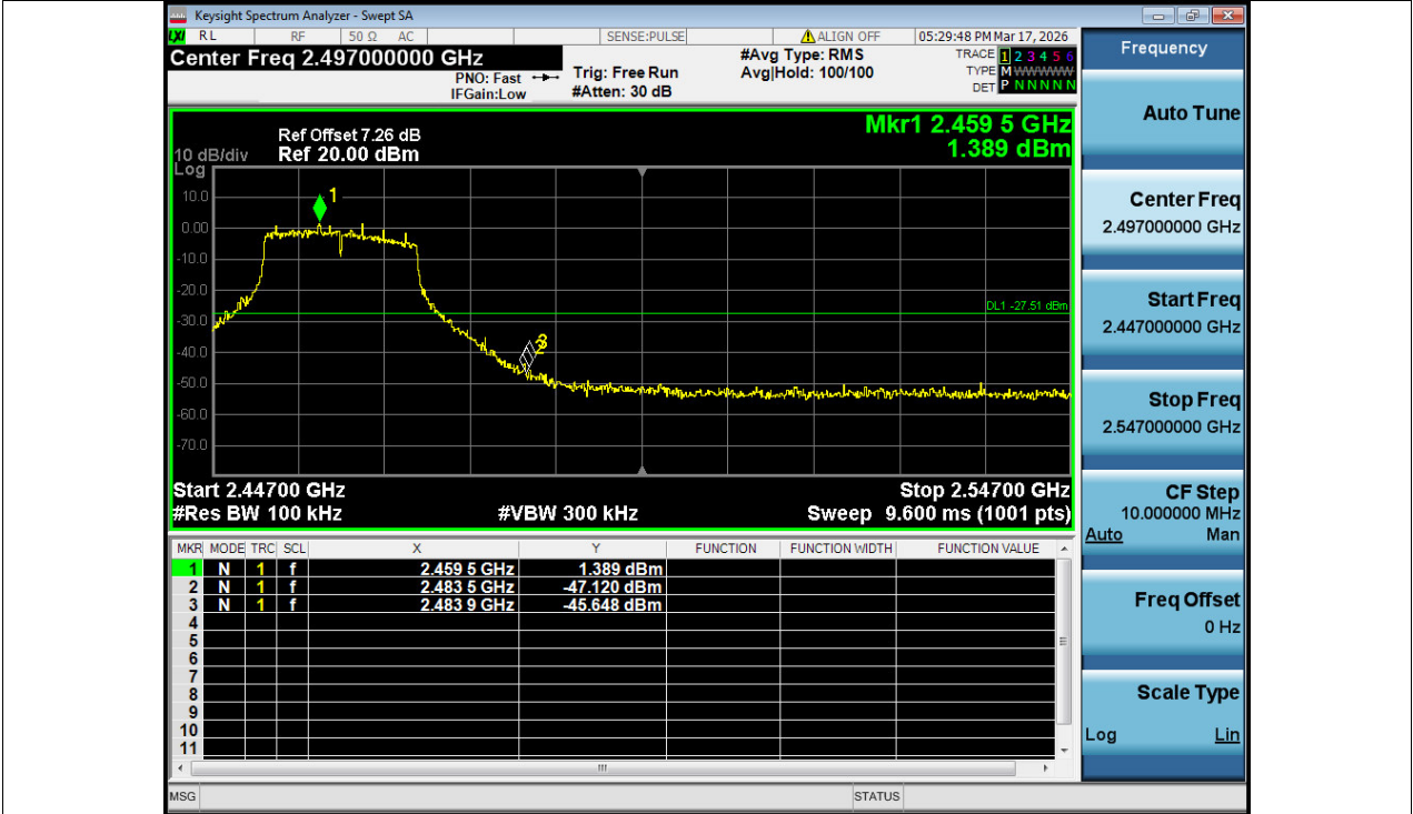
Band Edge NVNT n20 2462MHz Ant1 Emission
