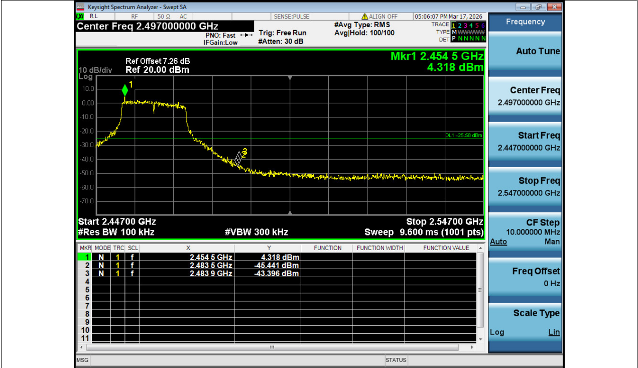
Band Edge NVNT g 2462MHz Ant1 Emission
