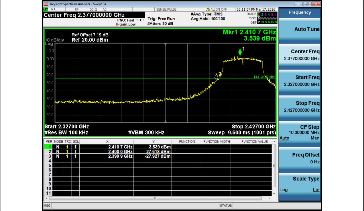
Band Edge NVNT n20 2412MHz Ant1 Emission
