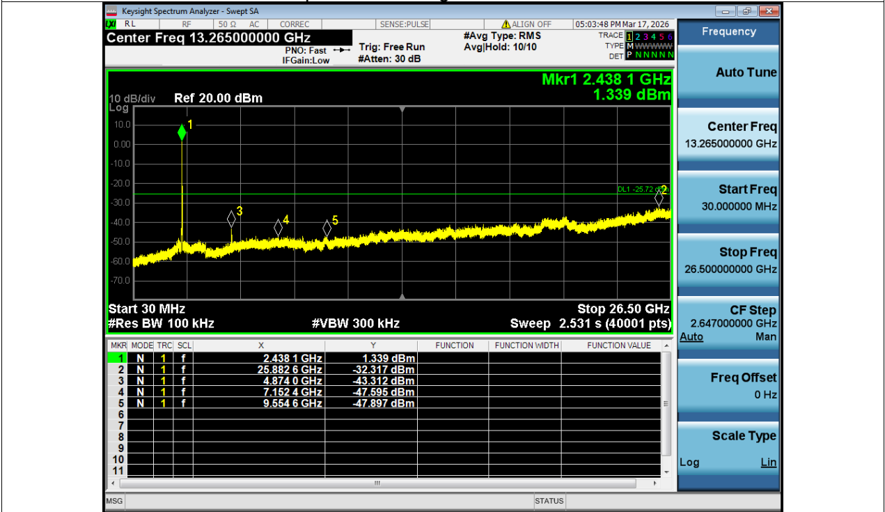
Tx. Spurious NVNT g 2437MHz Ant1 Emission
