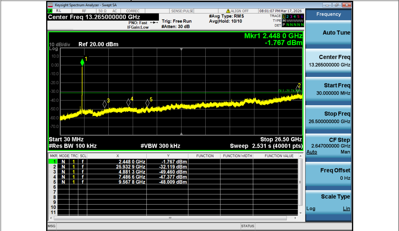
Tx. Spurious NVNT ax40 2437MHz Ant1 Emission
