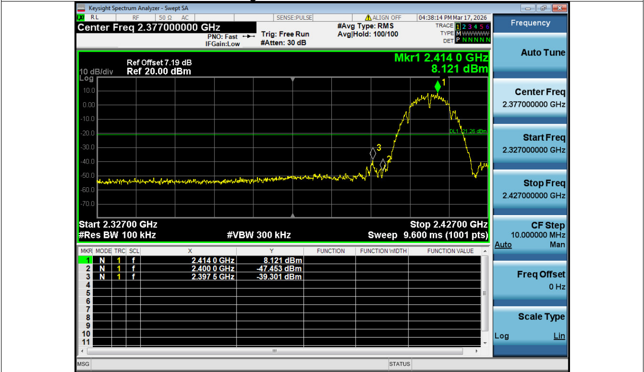
Band Edge NVNT b 2412MHz Ant1 Emission
