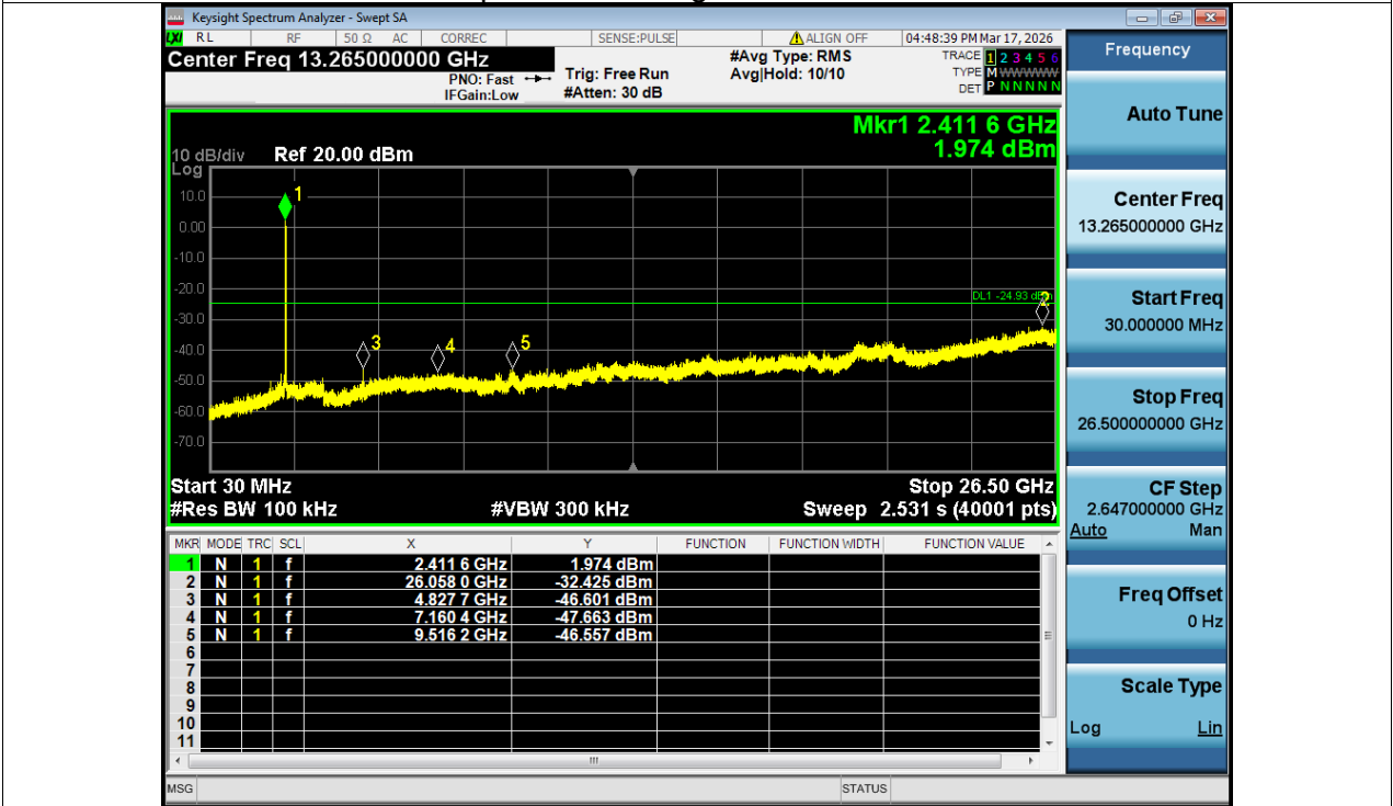
Tx. Spurious NVNT g 2412MHz Ant1 Emission
