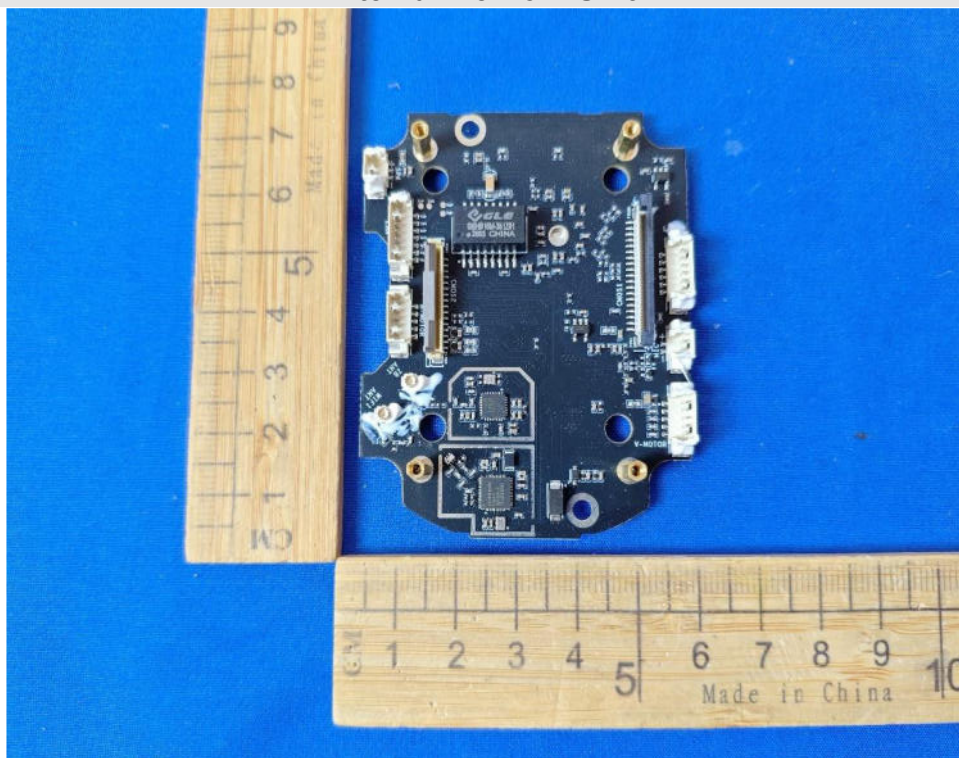
Internal View of EUT-9
