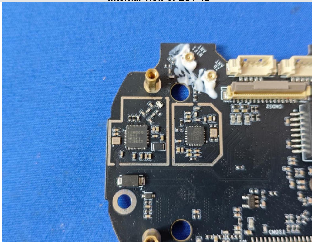
Internal View of EUT-12
