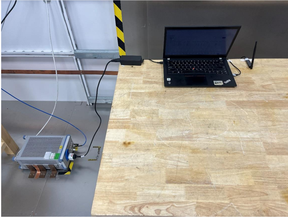
Conducted emissions
