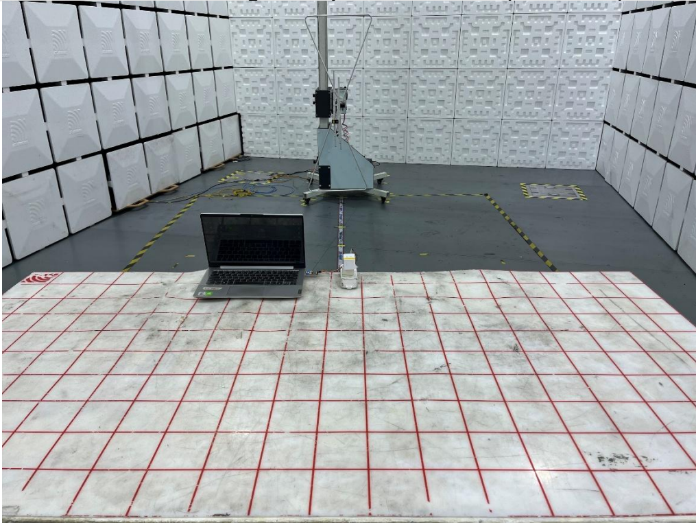
Radiated Band edge and Spurious Emission (BLE + WIFI)
