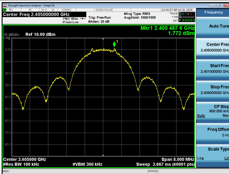
Tx. Spurious NVNT Zigbee 2405MHz Ant1 Ref
