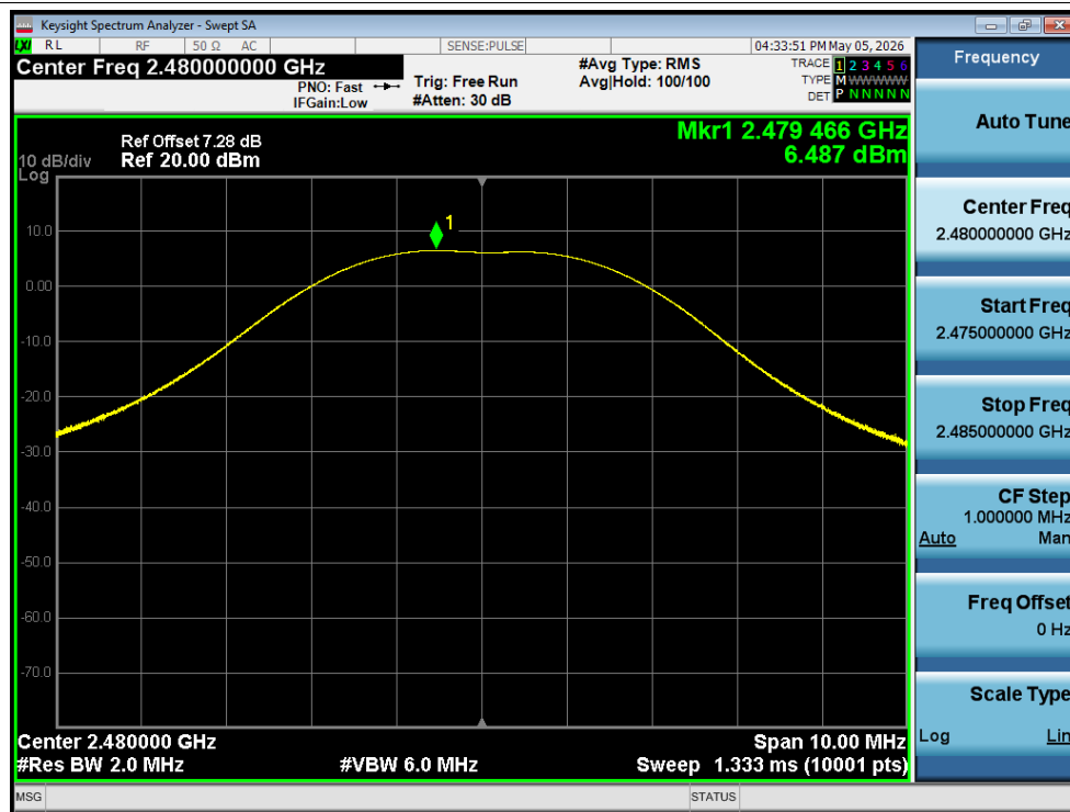
Peak Power NVNT Zigbee 2480MHz Ant1
