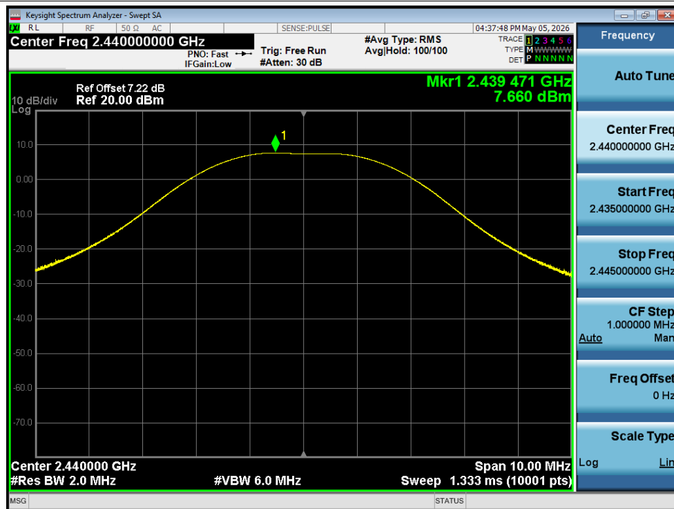
Peak Power NVNT Zigbee 2440MHz Ant1
