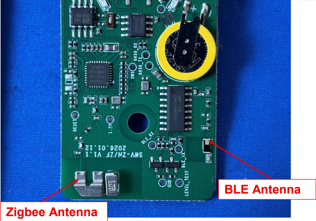
Internal View of EUT-18
