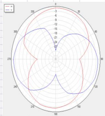
2450P0 Total
