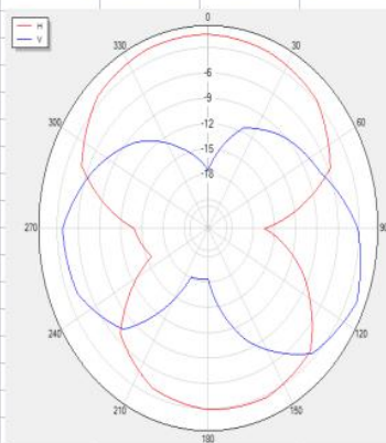
2500T90 Polar
