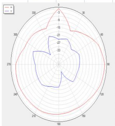
2450P0 Polar
