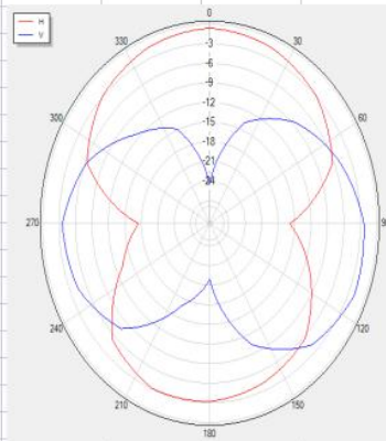
2500P0 Total
