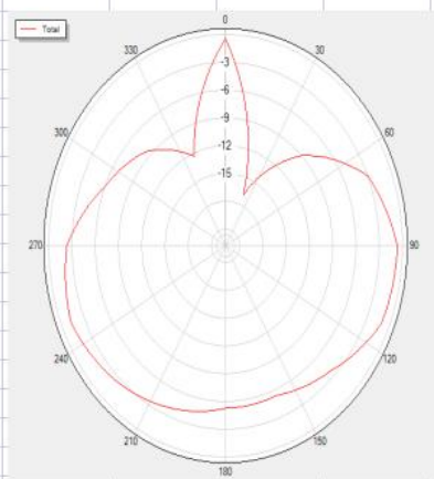
2400T90 Polar
