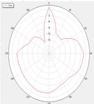
2500T90 Polar
