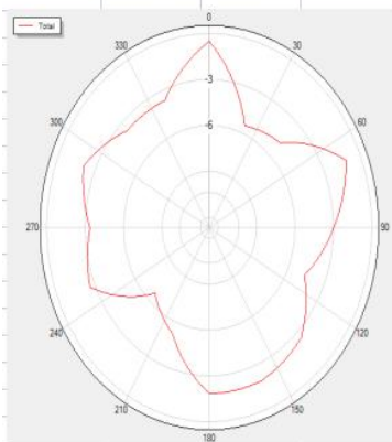
2500P90 Total
