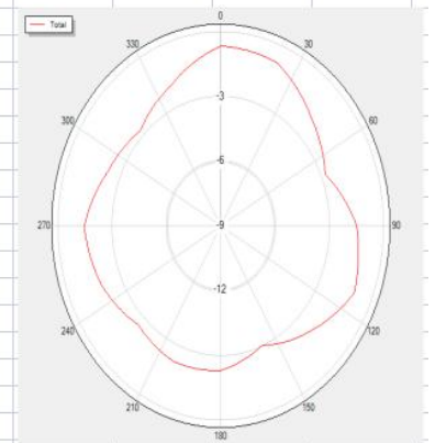
2450P90 Polar
