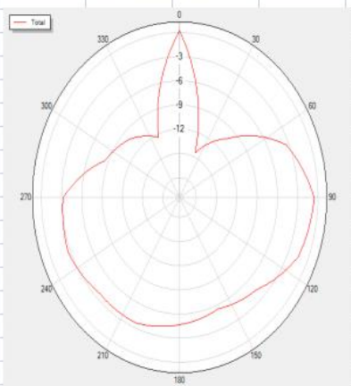
2450P0 Total
