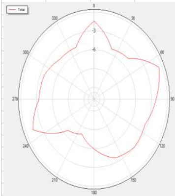
2500P0 Polar
