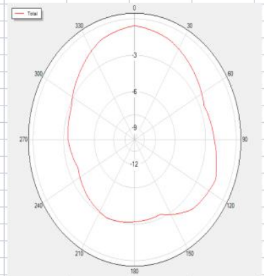
2500P90 Polar
