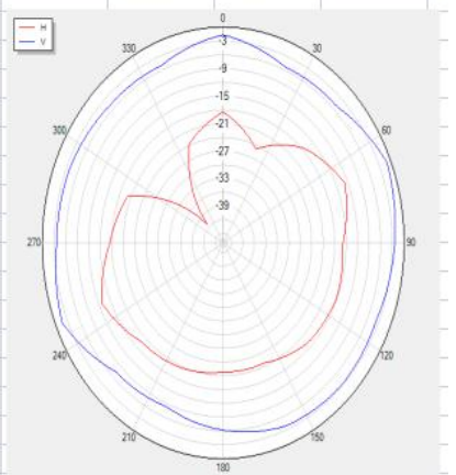
2450P90 Polar
