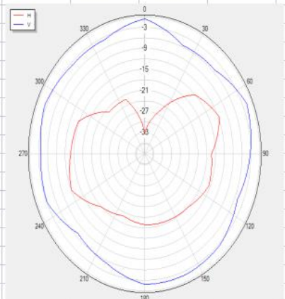
2500T90 Total
