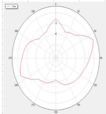
2450P0 Polar
