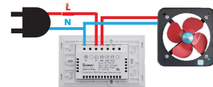
4.2 Control the appliance lower than 600W (Eg:1CH).
