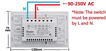
4.1 Lights wiring instruction (Eg:3CH).
