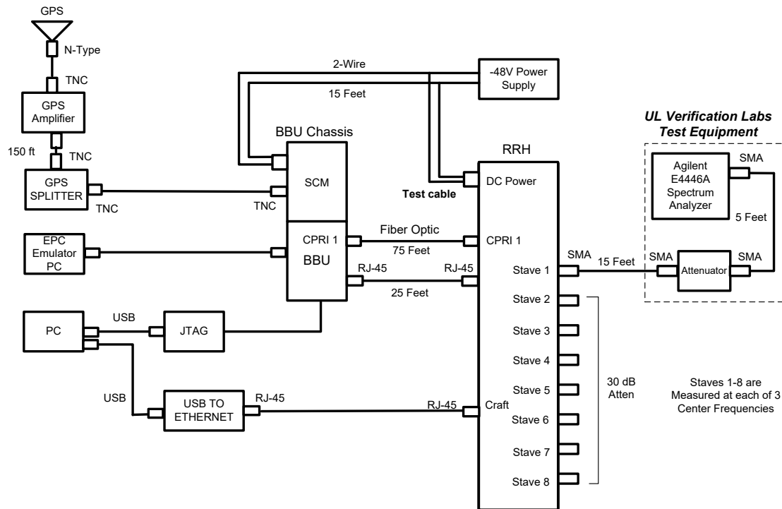
Conducted Emissions Tests Configuration - RRH to Spectrum Analyzer
