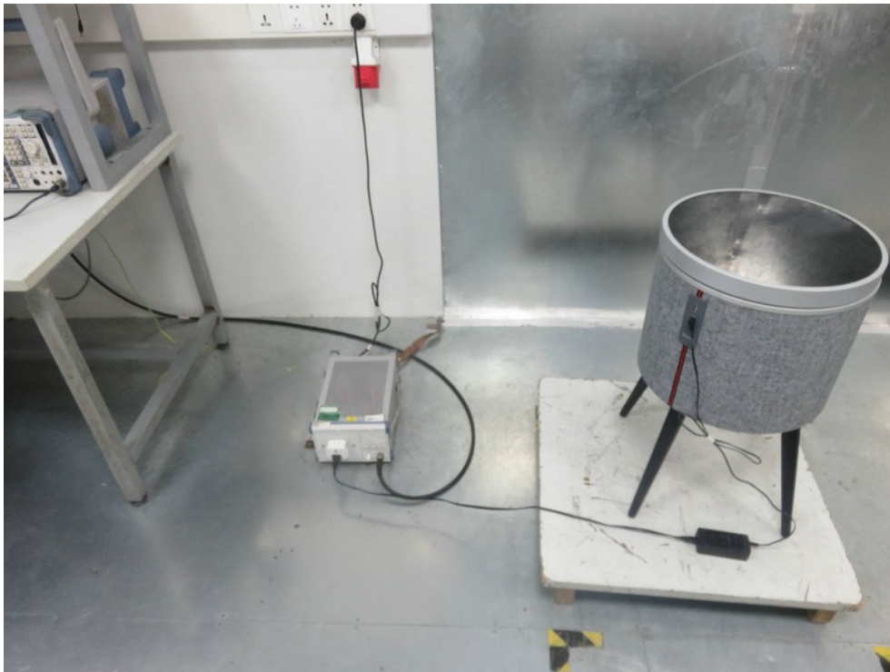
FCC ID: 2APNM-STSW Photo of Conducted Emission Measurement
