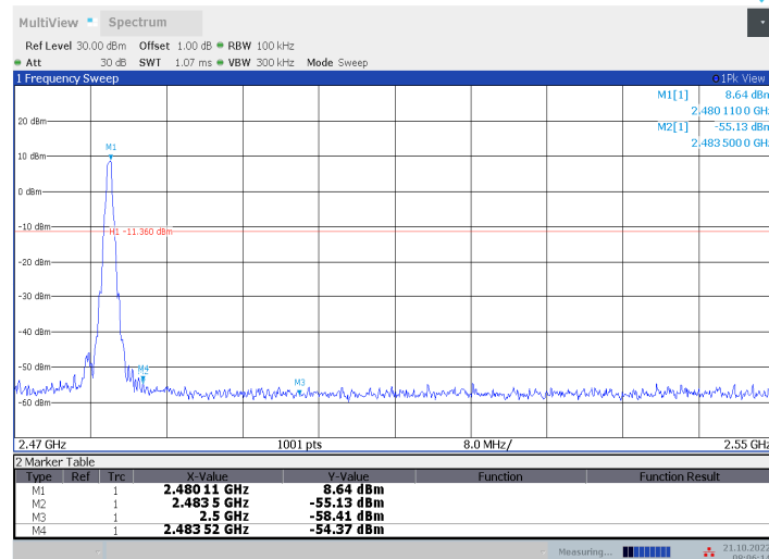
DH5_Ant2_High_2480
