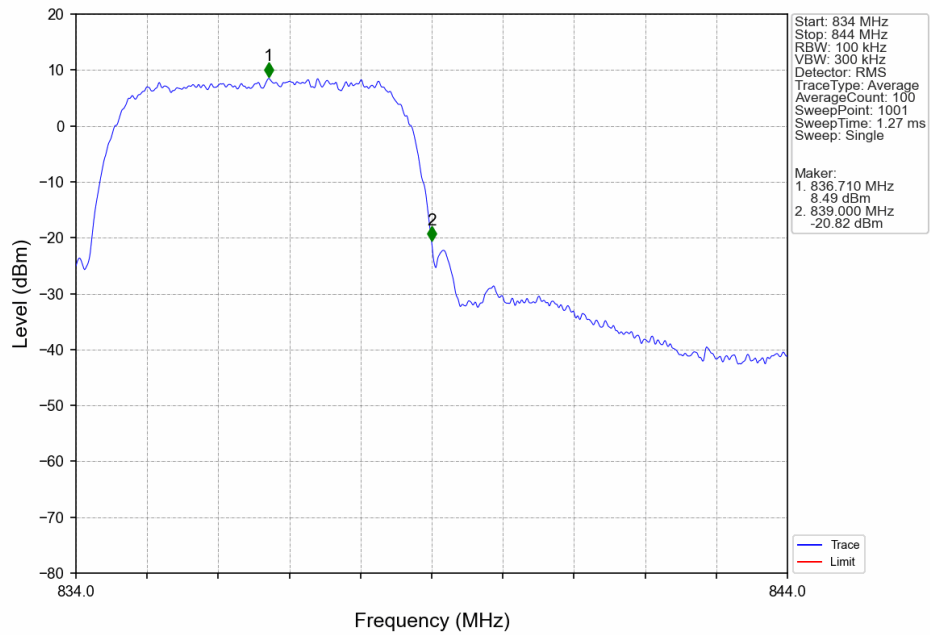
BandV_RMC_MCH_836.6MHz_12.2kbps_RMC_NTNV
