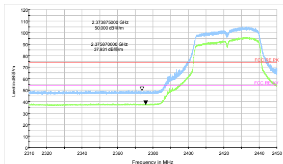
802.11ax HE40-Channel 3 Peak+ Average
