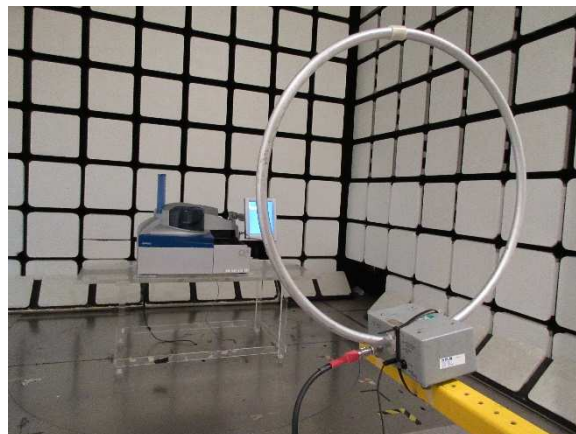
Radio-frequency radiated emissions (9k-30MHz)
