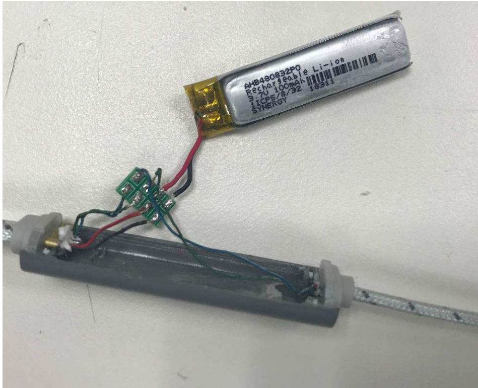
Internal View
