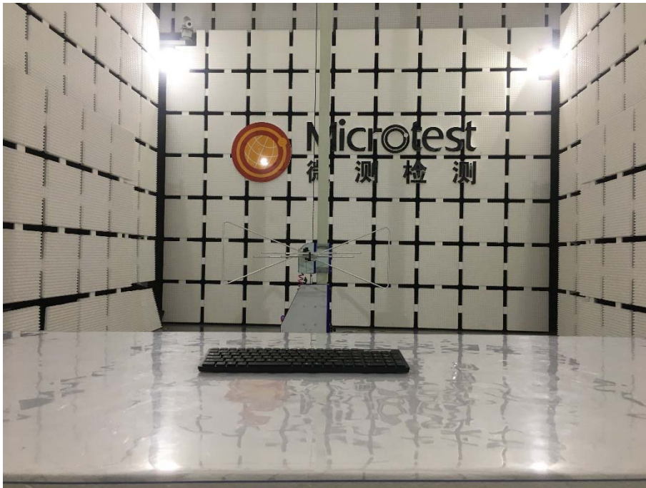
Keyboard
