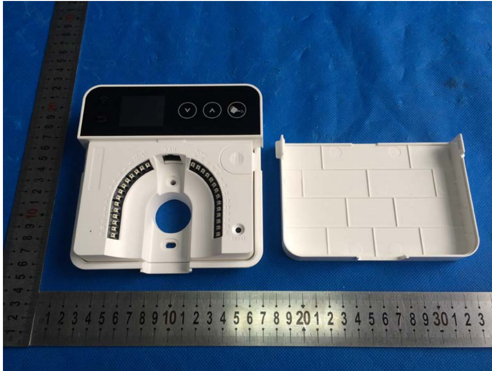
EUT - Open View 1
