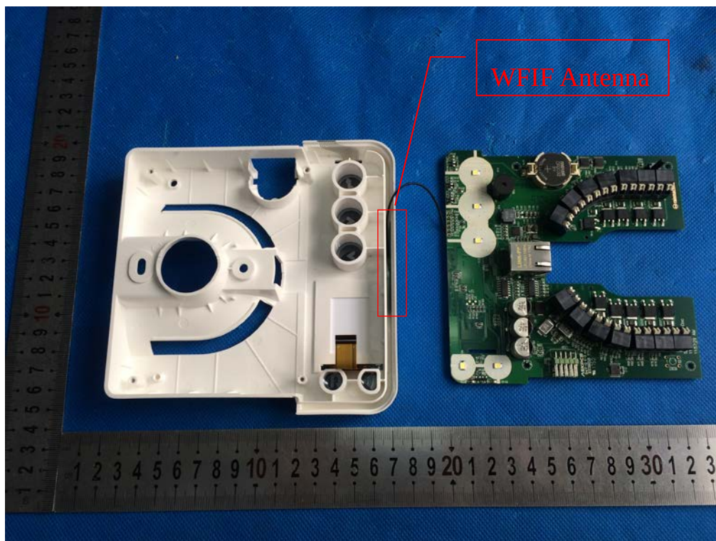
EUT - Open View 3
