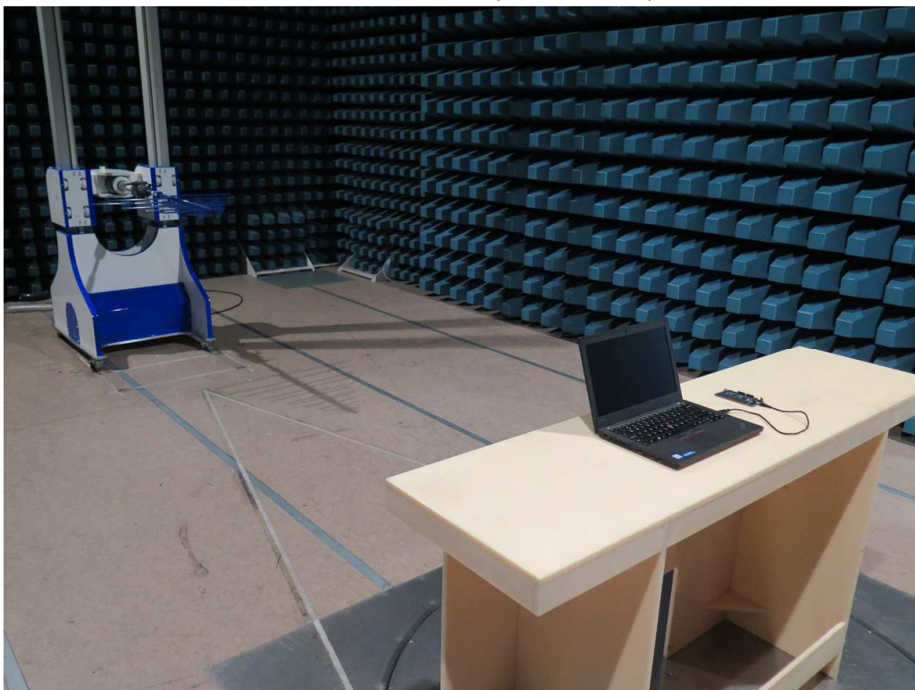
200Mz – 1GHz (Data transfer)
