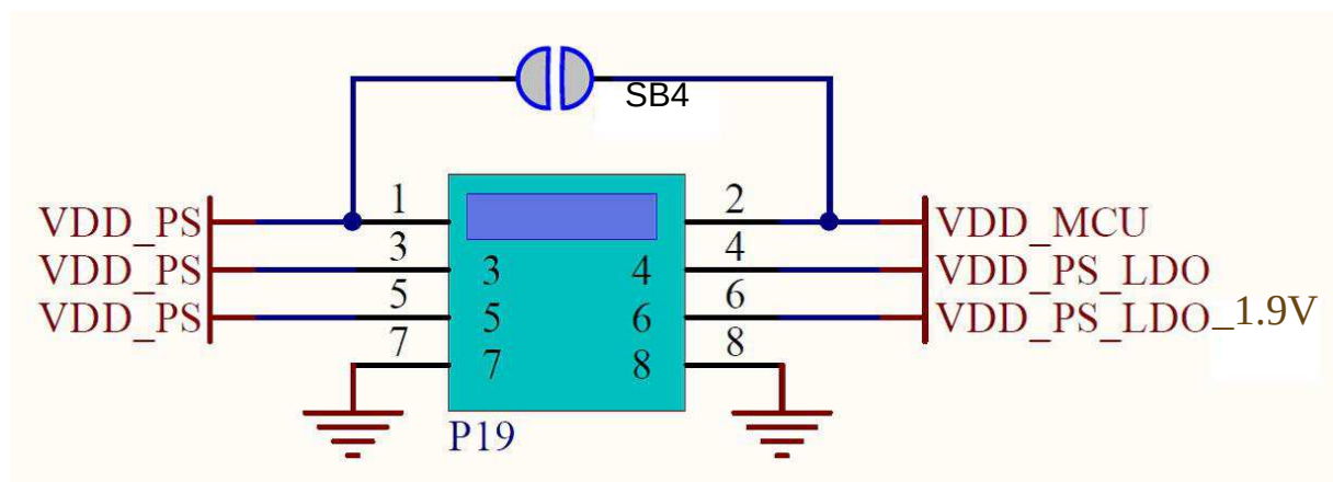
Figure 6. Voltage Selection on Header P19
