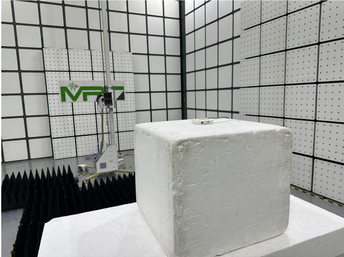
Description: Duty Cycle Test Setup
