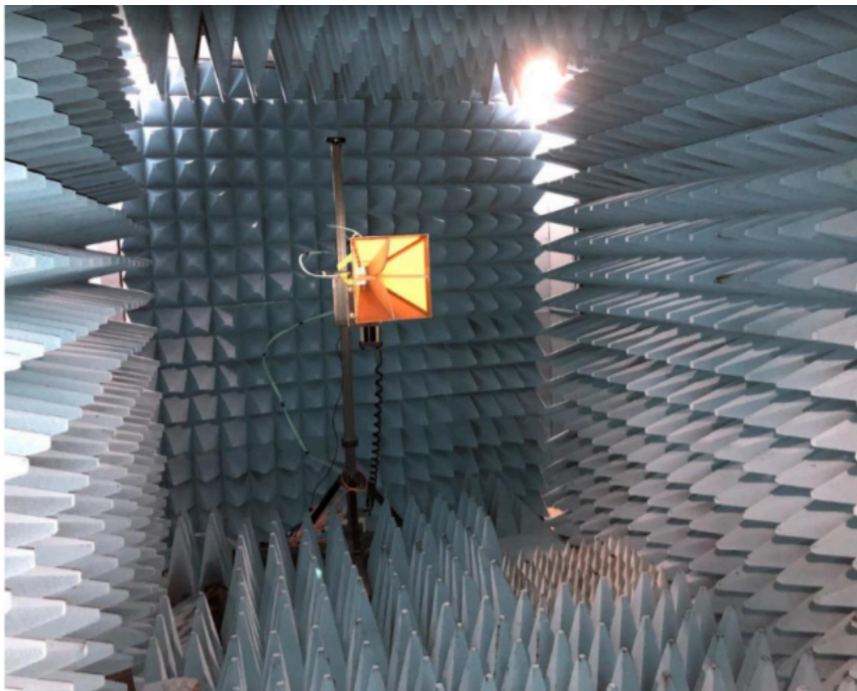
Figure 2: Receiving antenna in chamber
