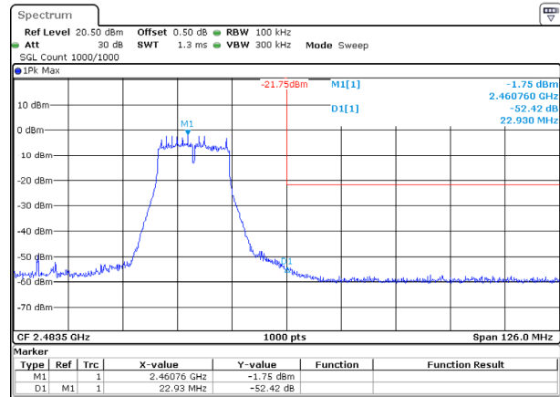
802.11g_2462MHz
