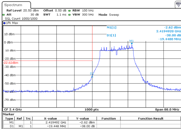
802.11g_2412MHz
