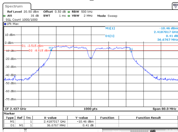
802.11n40_2437MHz
