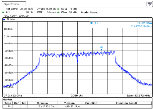
802.11g_2412MHz
