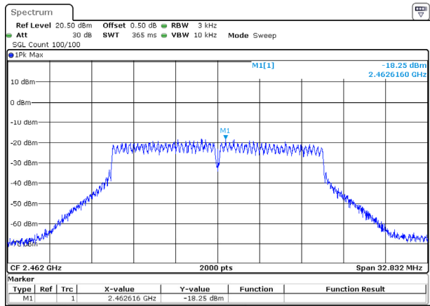
802.11g_2462MHz
