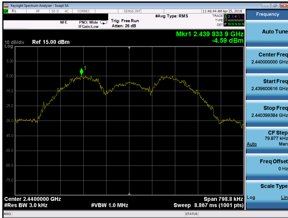
Plot 7-20. Power Spectral Density Plot (Bluetooth (LE), 250kbps – Ch. 19)
