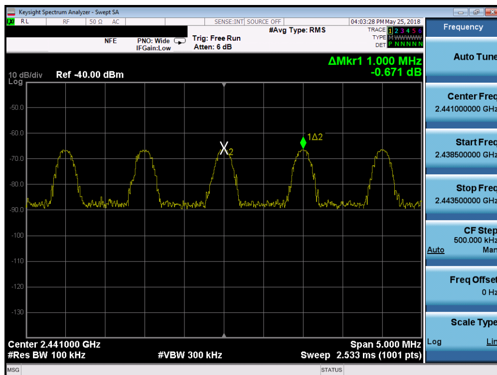
Plot 7-34. Channel Spacing Plot (Bluetooth)
