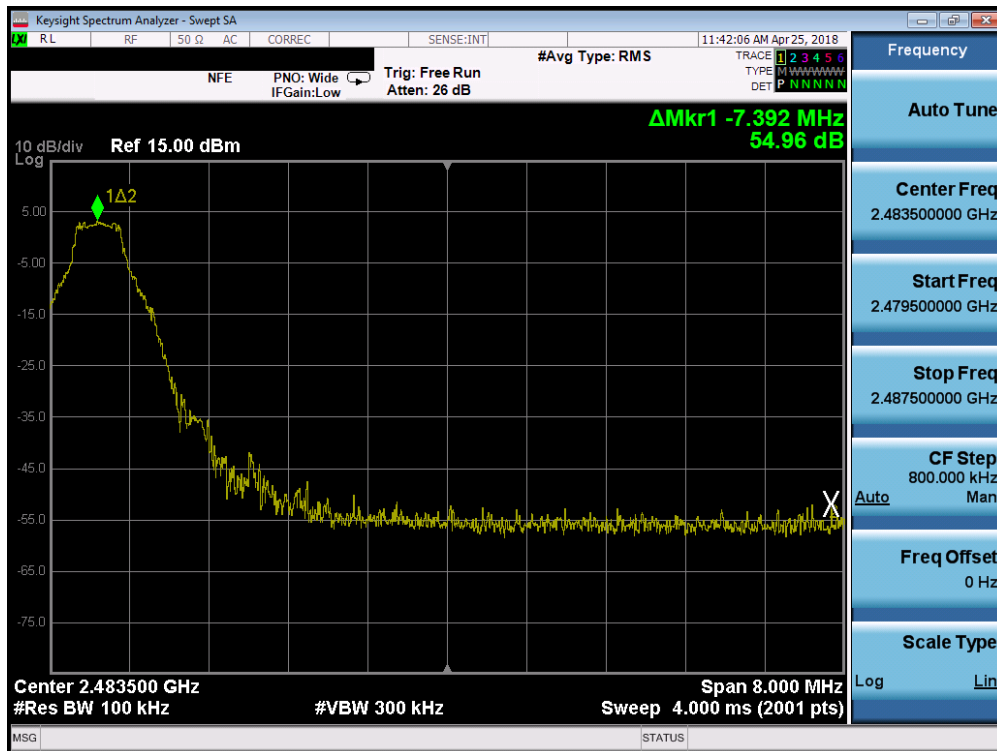
Plot 7-31. Band Edge Plot (Bluetooth (LE), 1Mbps – Ch. 39)
