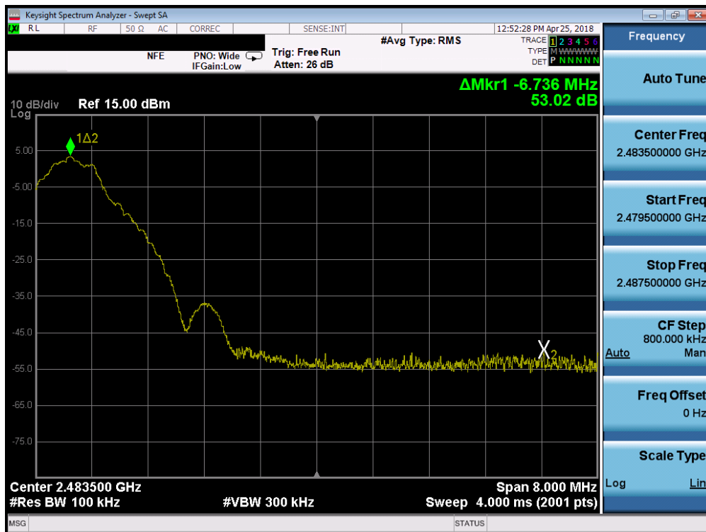
Plot 7-33. Band Edge Plot (Bluetooth (LE), 2Mbps – Ch. 39)
