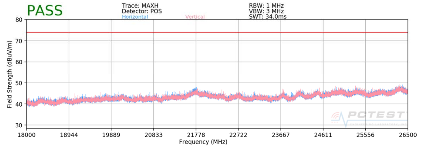
Plot 7-58. Radiated Spurious Plot above 18GHz
