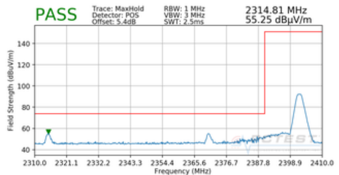
Plot 7-60. Radiated Restricted Lower Band Edge Measurement (Peak)
