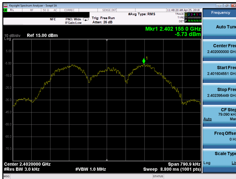
Plot 7-19. Power Spectral Density Plot (Bluetooth (LE), 250kbps – Ch. 0)
