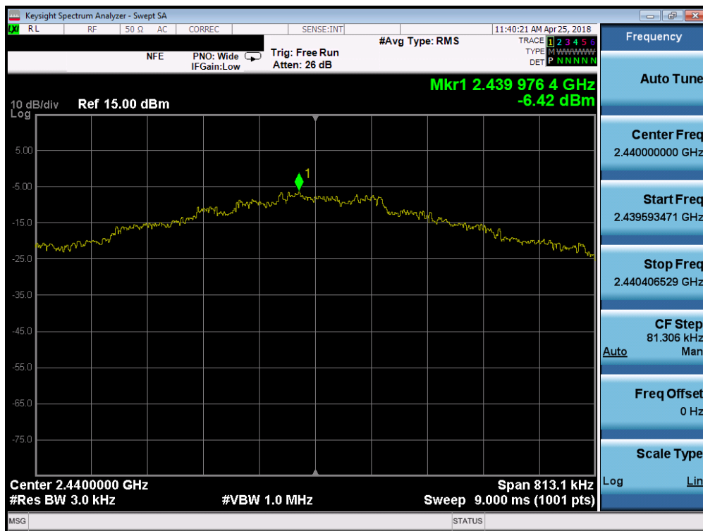
Plot 7-23. Power Spectral Density Plot (Bluetooth (LE), 1Mbps – Ch. 19)
