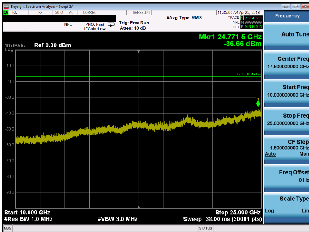
Plot 7-54. Conducted Spurious Plot (Bluetooth (LE), 2Mbps – Ch. 39)
