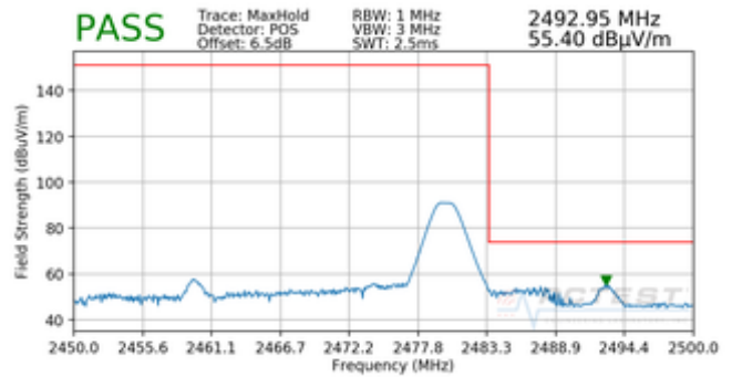
Plot 7-62. Radiated Restricted Upper Band Edge Measurement (Peak)
