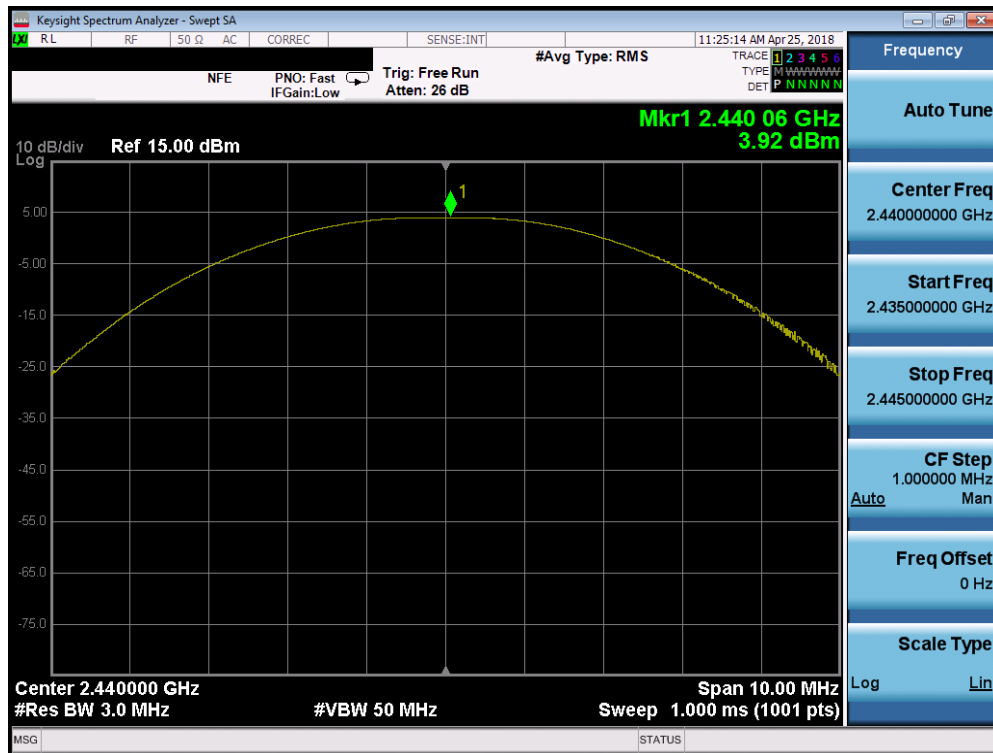
Plot 7-17. Peak Power Plot (Bluetooth (LE), 2Mbps – Ch. 19)
