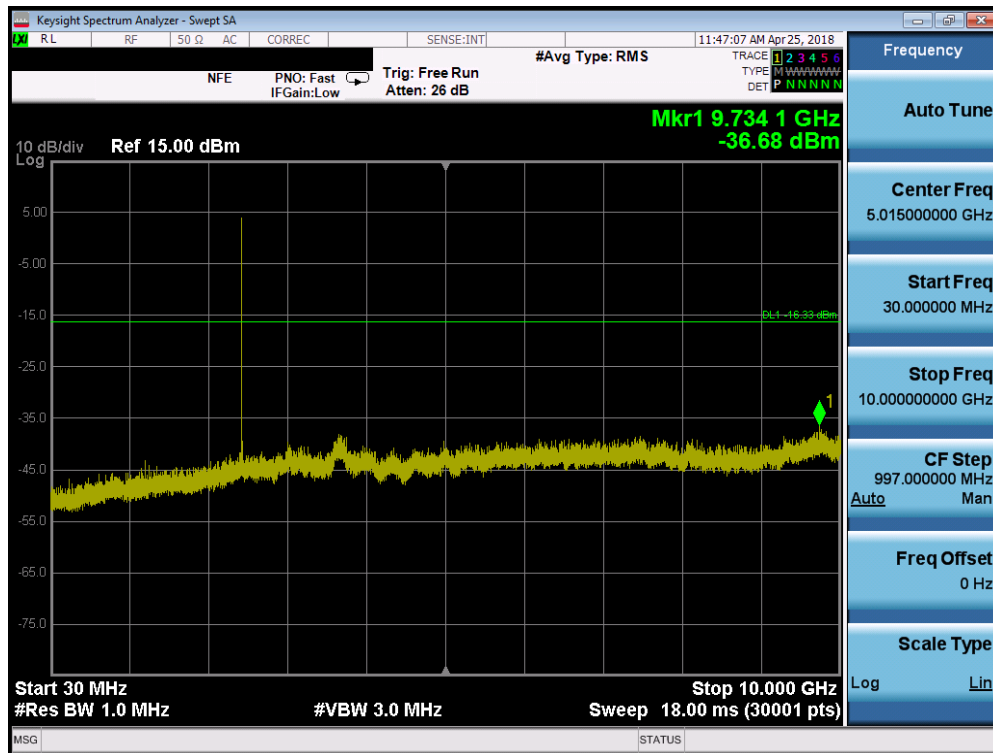
Plot 7-39. Conducted Spurious Plot (Bluetooth (LE), 250kbps – Ch. 19)
