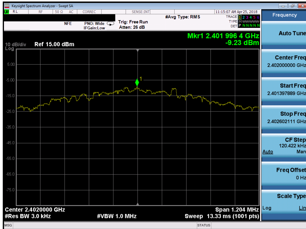
Plot 7-25. Power Spectral Density Plot (Bluetooth (LE), 2Mbps – Ch. 0)
