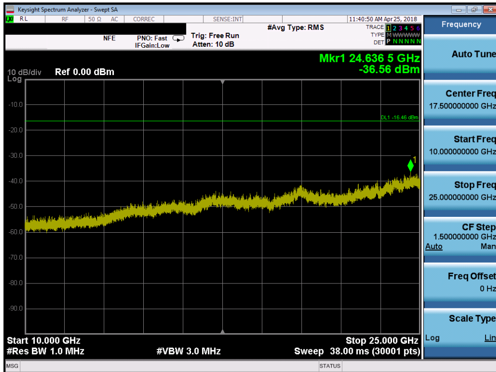
Plot 7-46. Conducted Spurious Plot (Bluetooth (LE), 1Mbps – Ch. 19)
