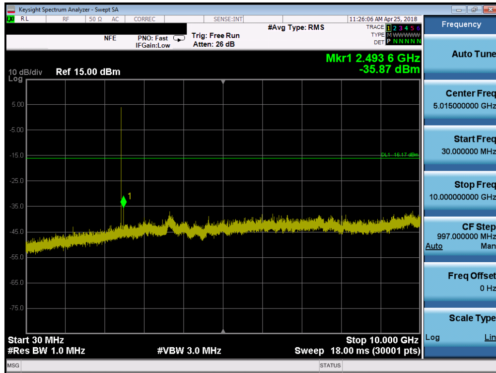
Plot 7-51. Conducted Spurious Plot (Bluetooth (LE), 2Mbps - Ch. 19)
