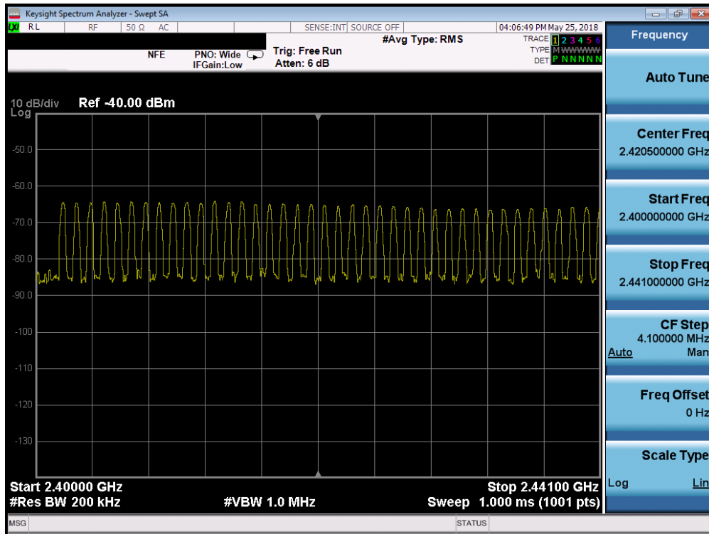
Plot 7-35. Low End Spectrum Channel Hopping Plot (Bluetooth)
