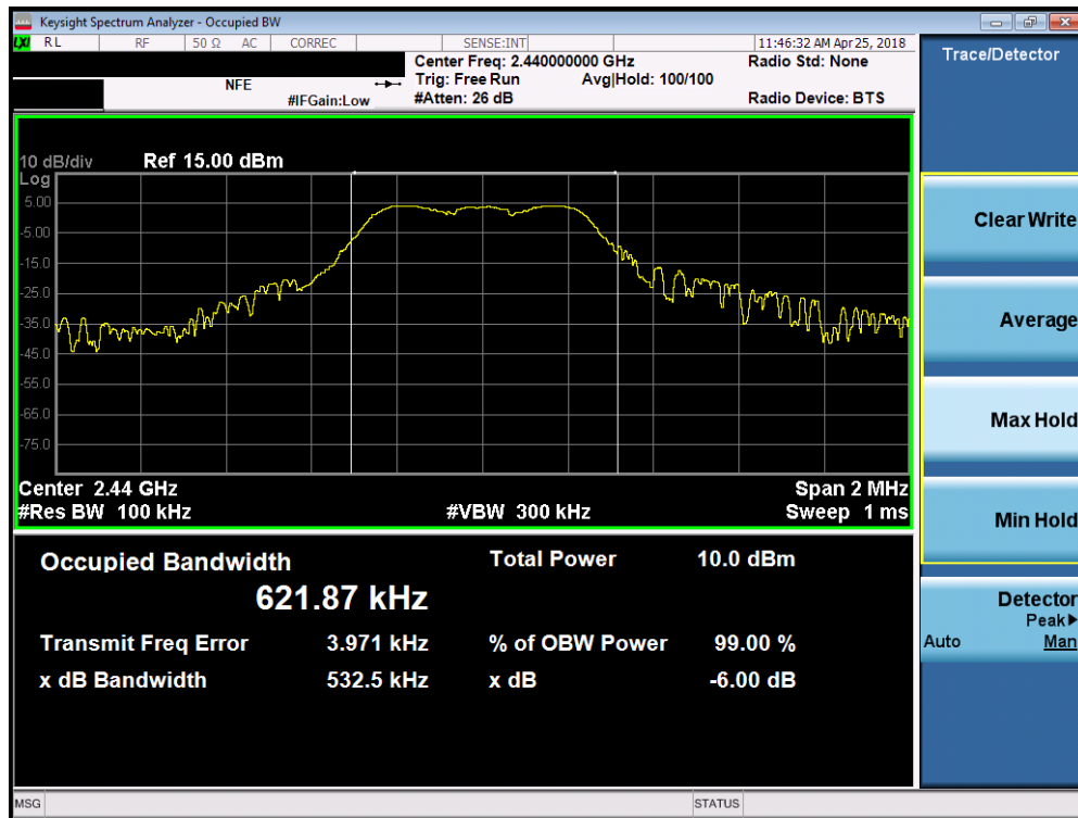
Plot 7-2. 6dB Bandwidth Plot (Bluetooth (LE), 250kbps – Ch. 19)
