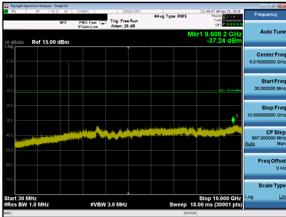
Plot 7-37. Conducted Spurious Plot (Bluetooth (LE), 250kbps – Ch. 0)
