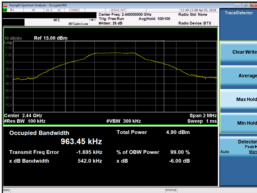
Plot 7-5. 6dB Bandwidth Plot (Bluetooth (LE), 1Mbps – Ch. 19)
