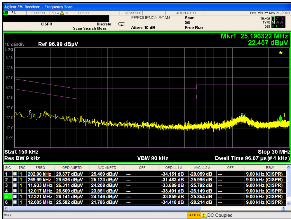
Plot 7-65. Line Conducted Plot with Bluetooth LE (N)
