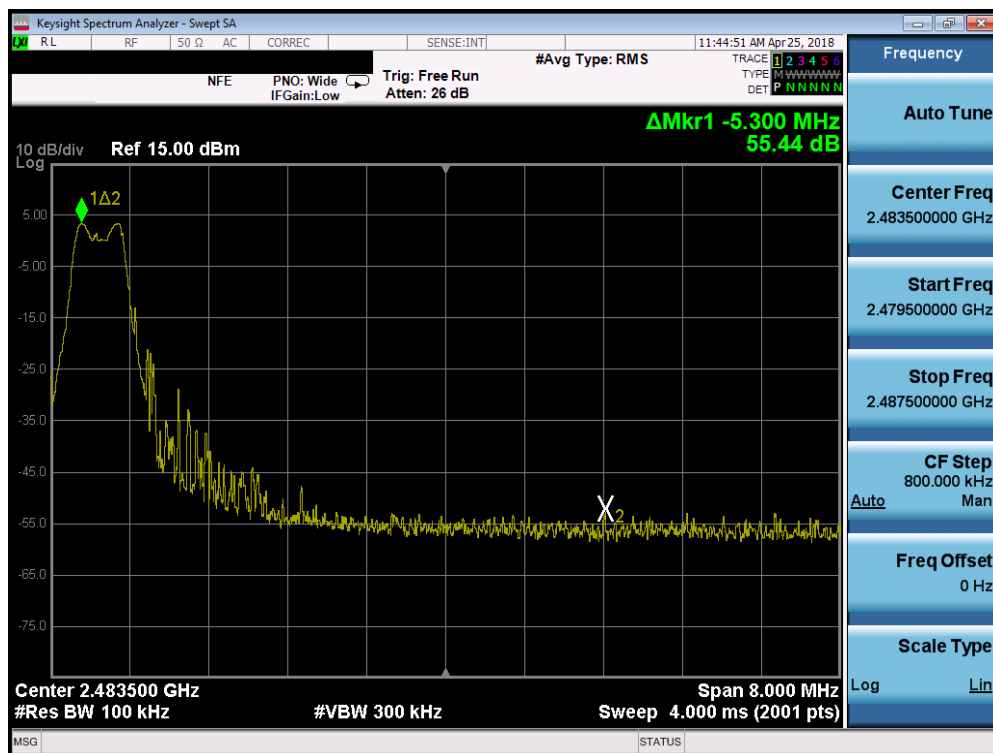
Plot 7-29. Band Edge Plot (Bluetooth (LE), 250kbps – Ch. 39)
