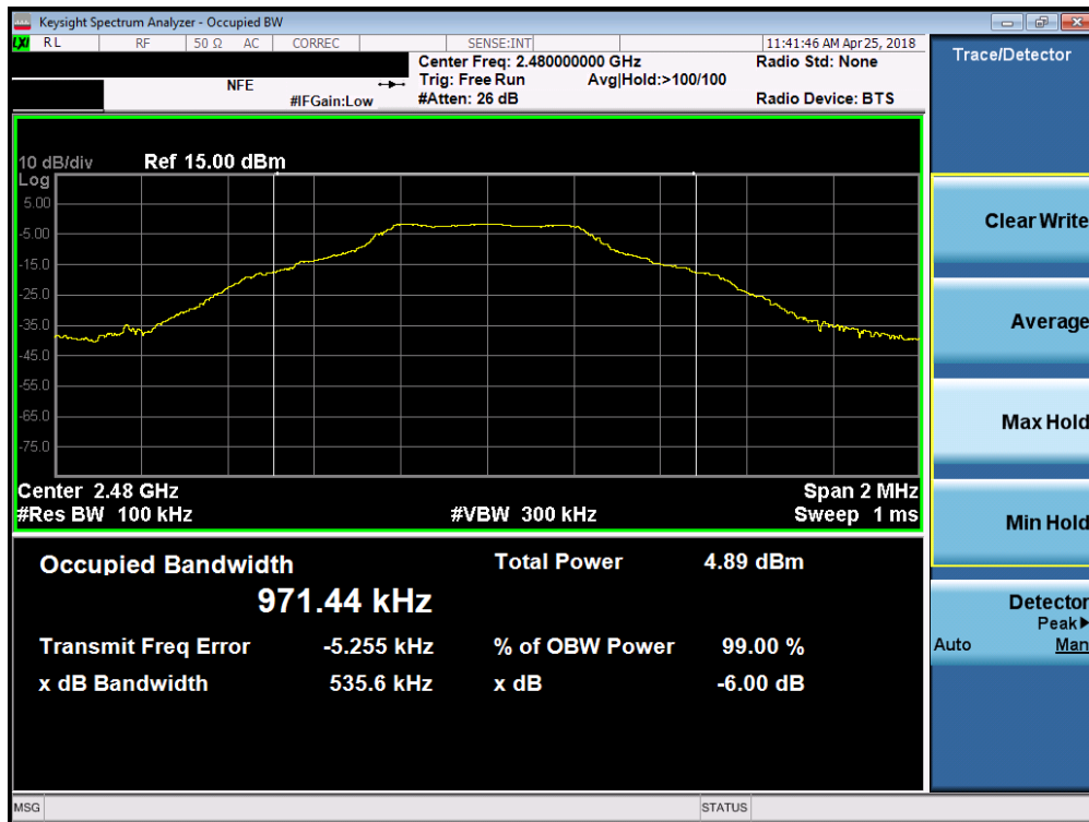
Plot 7-6. 6dB Bandwidth Plot (Bluetooth (LE), 1Mbps – Ch. 39)
