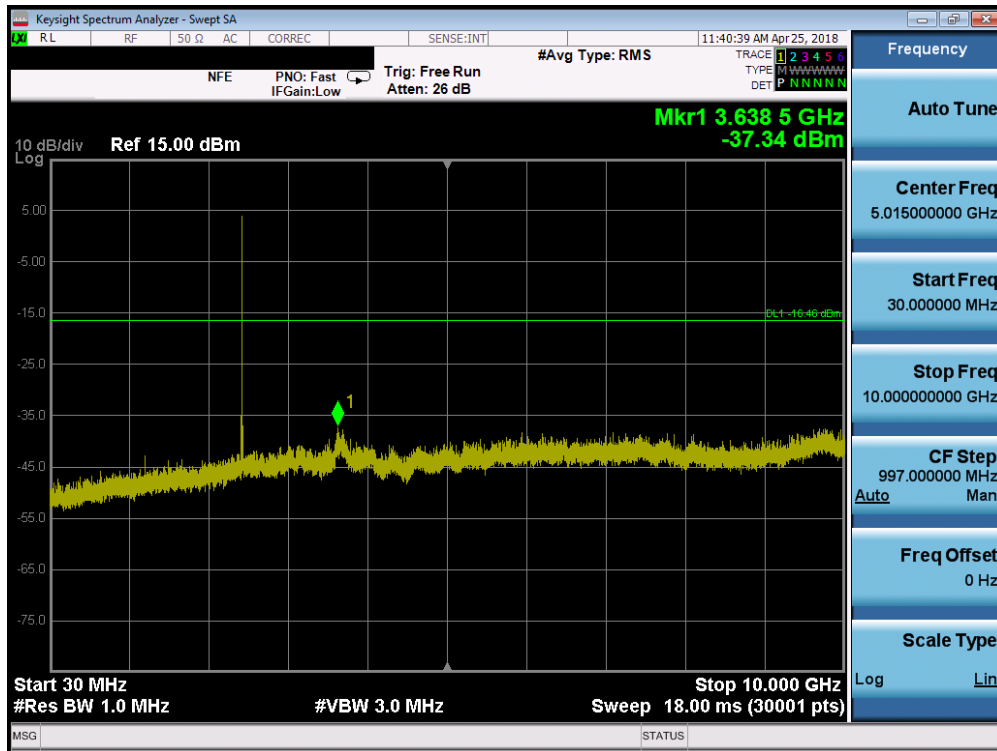
Plot 7-45. Conducted Spurious Plot (Bluetooth (LE), 1Mbps – Ch. 19)
