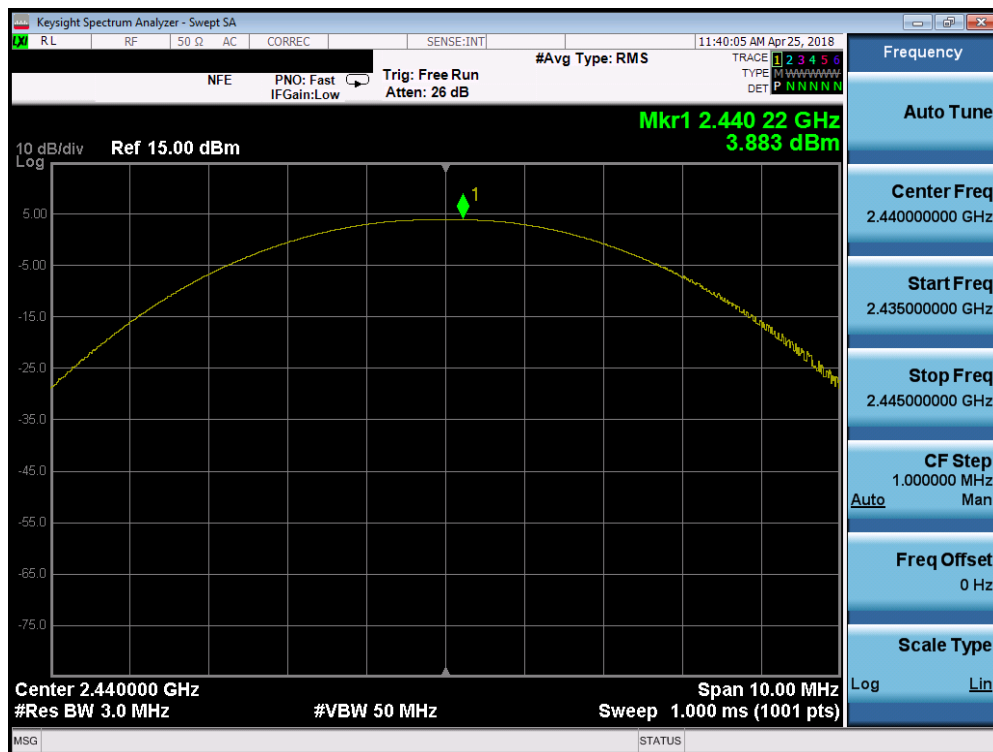
Plot 7-14. Peak Power Plot (Bluetooth (LE), 1Mbps – Ch. 19)
