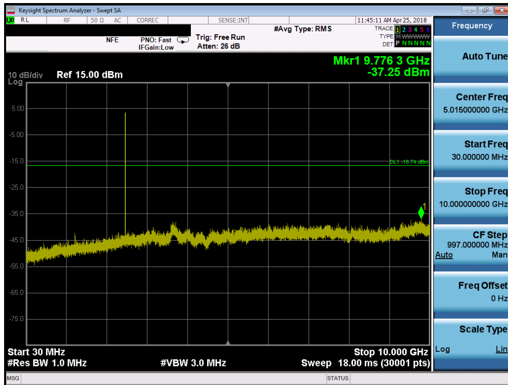
Plot 7-41. Conducted Spurious Plot (Bluetooth (LE), 250kbps – Ch. 39)
