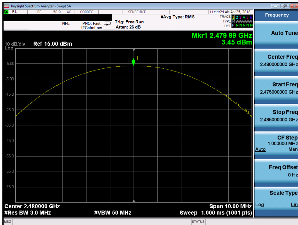
Plot 7-12. Peak Power Plot (Bluetooth (LE), 250kbps – Ch. 39)
