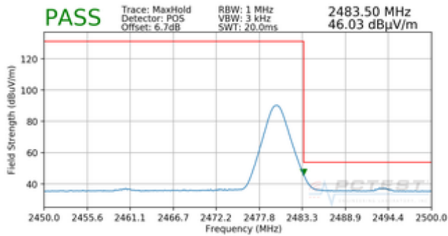
Plot 7-61. Radiated Restricted Upper Band Edge Measurement (Average)
