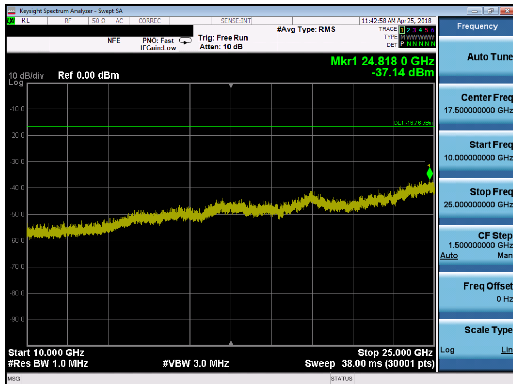
Plot 7-48. Conducted Spurious Plot (Bluetooth (LE), 1Mbps – Ch. 39)
