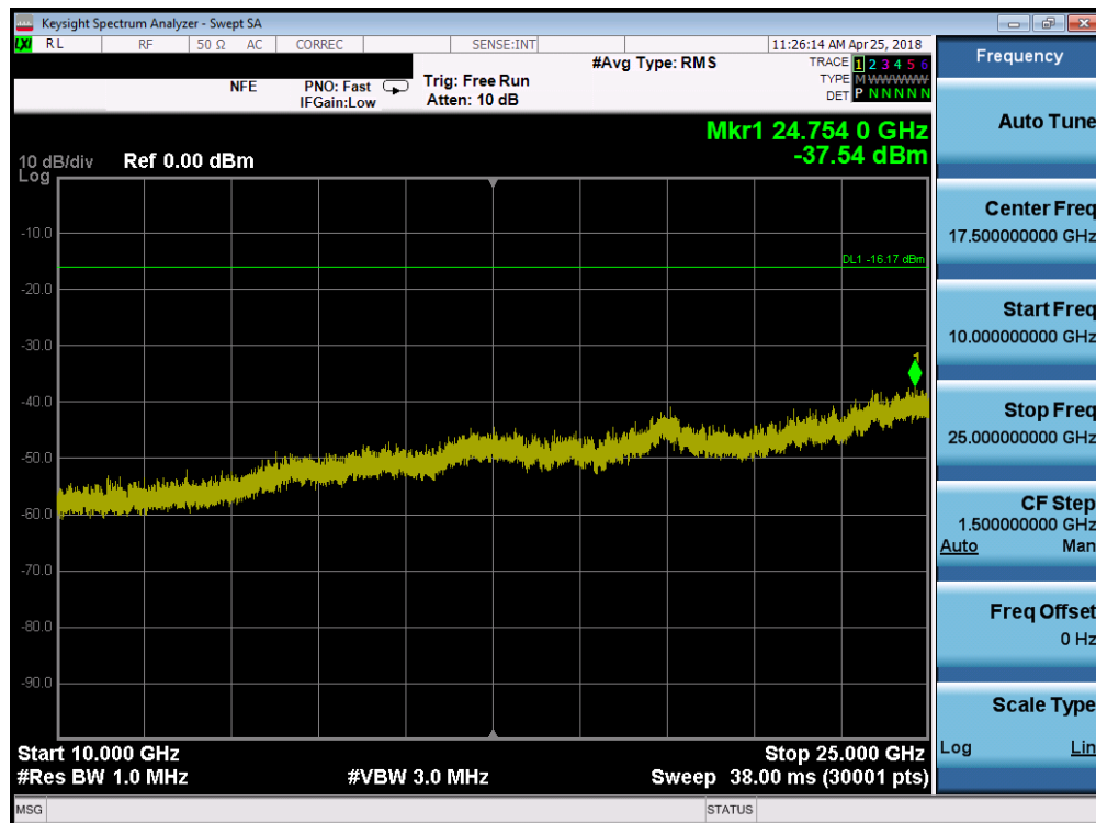
Plot 7-52. Conducted Spurious Plot (Bluetooth (LE), 2Mbps - Ch. 19)
