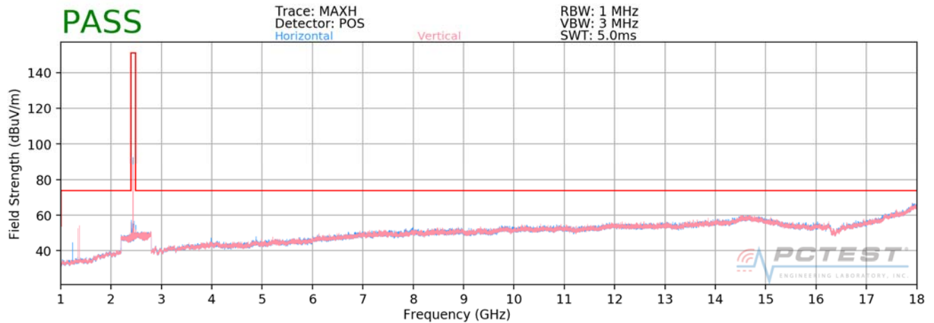
Plot 7-56. Radiated Spurious Plot above 1GHz (Bluetooth LE – Ch. 19)
