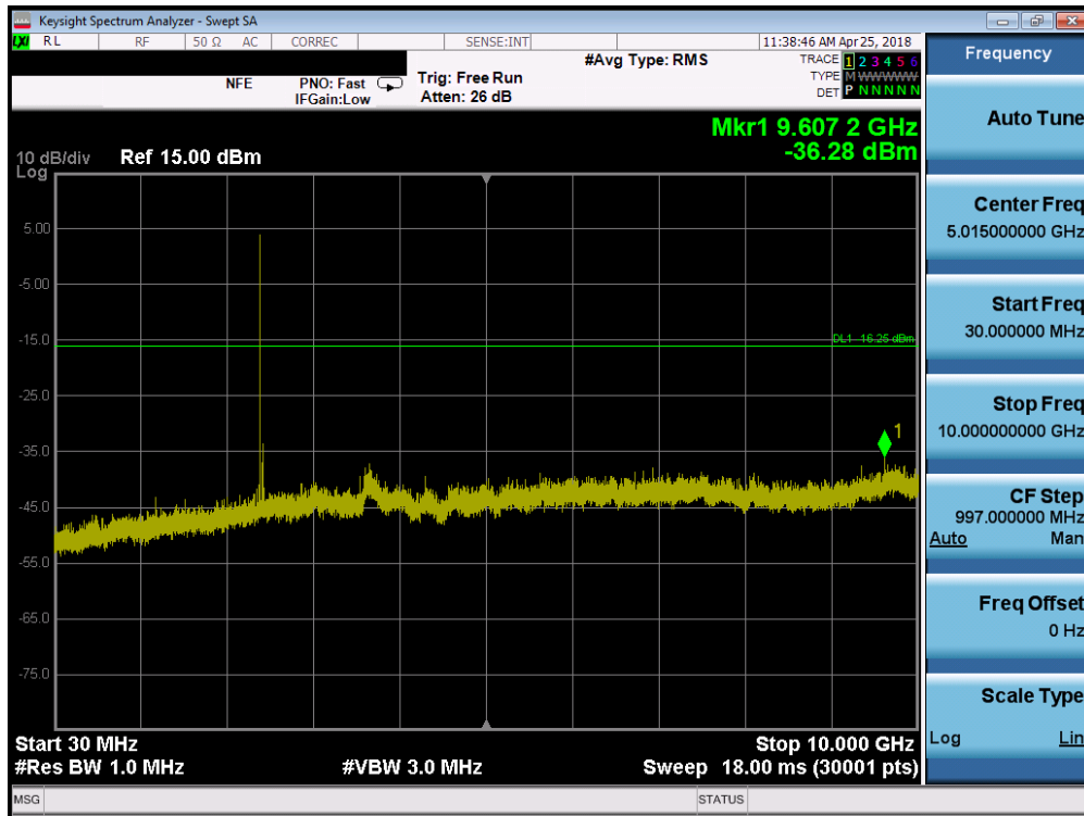
Plot 7-43. Conducted Spurious Plot (Bluetooth (LE), 1Mbps – Ch. 0)
