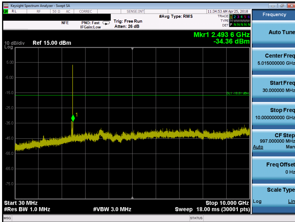
Plot 7-53. Conducted Spurious Plot (Bluetooth (LE), 2Mbps – Ch. 39)
