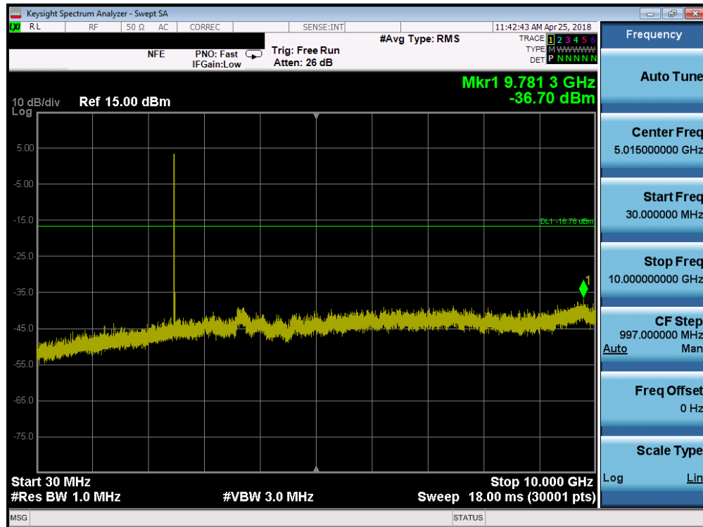
Plot 7-47. Conducted Spurious Plot (Bluetooth (LE), 1Mbps – Ch. 39)
