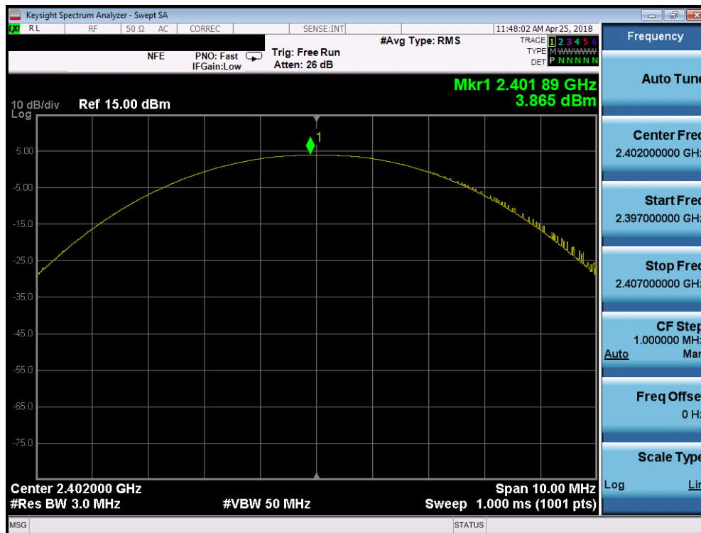
Plot 7-10. Peak Power Plot (Bluetooth (LE), 250kbps – Ch. 0)
