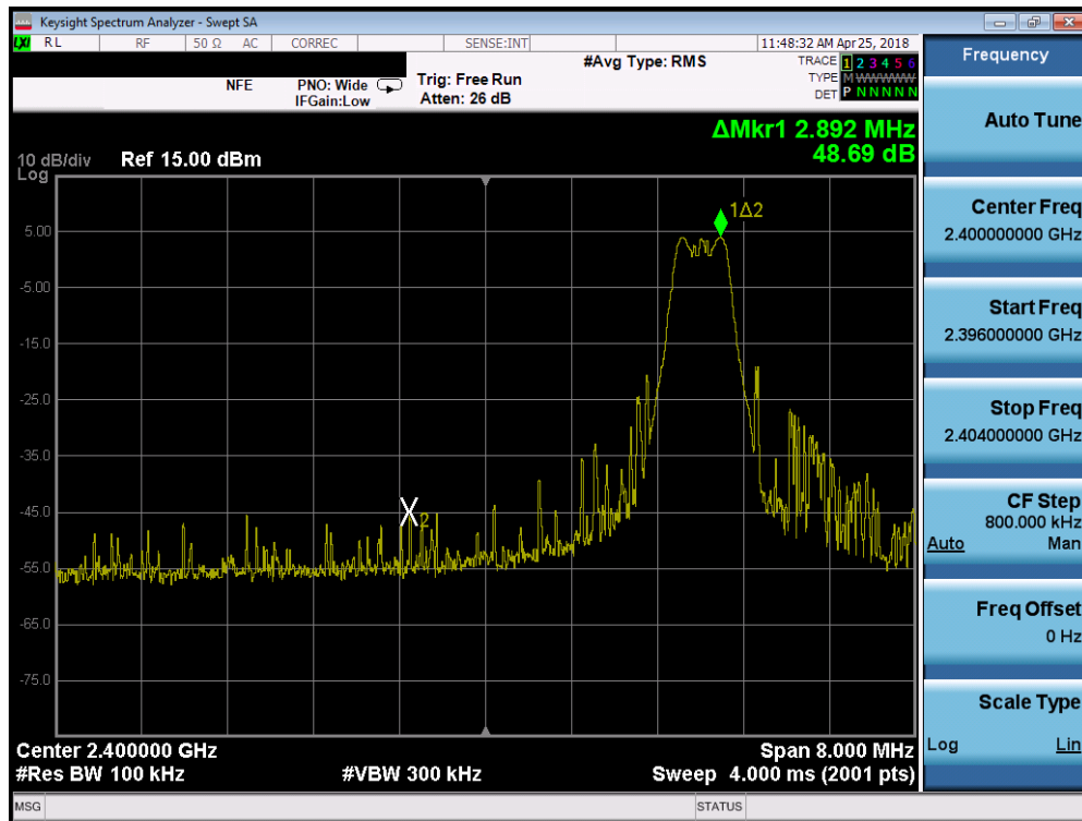
Plot 7-28. Band Edge Plot (Bluetooth (LE), 250kbps – Ch. 0)
