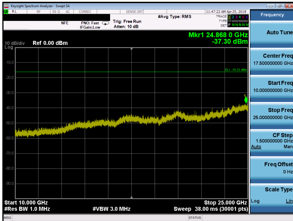
Plot 7-40. Conducted Spurious Plot (Bluetooth (LE), 250kbps – Ch. 19)
