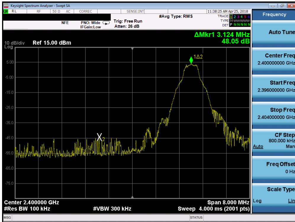
Plot 7-30. Band Edge Plot (Bluetooth (LE), 1Mbps – Ch. 0)
