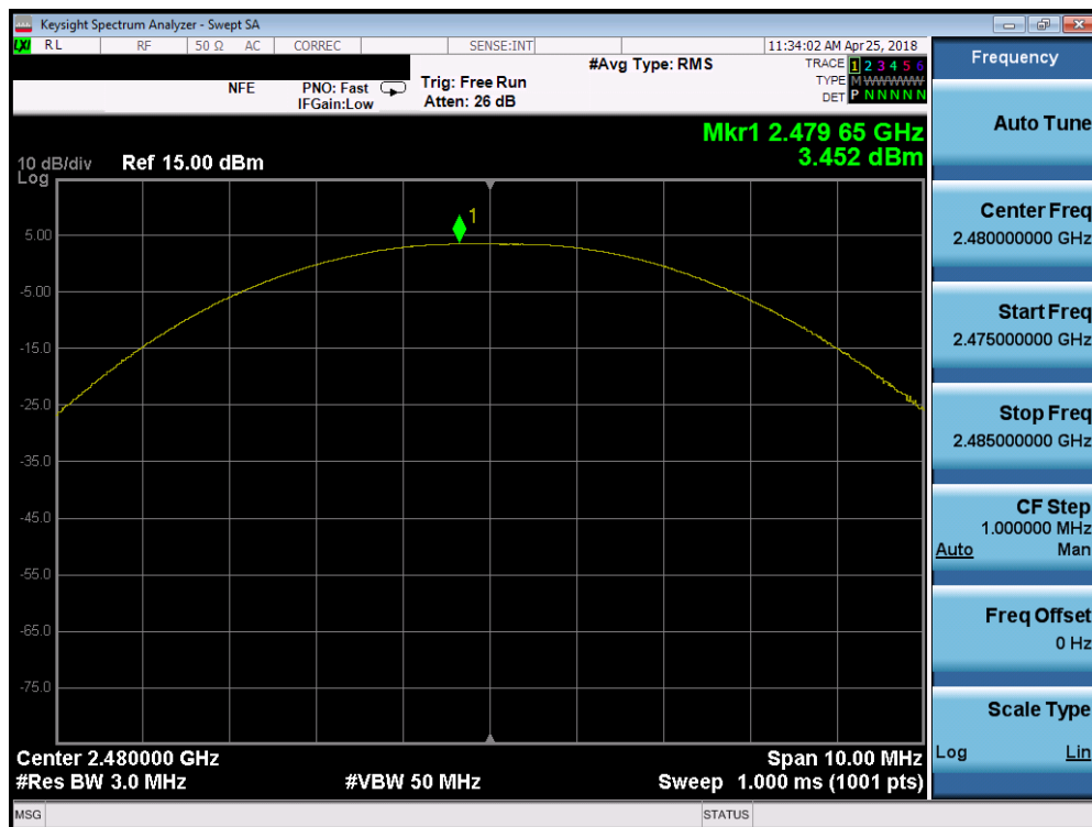
Plot 7-18. Peak Power Plot (Bluetooth (LE), 2Mbps – Ch. 39)
