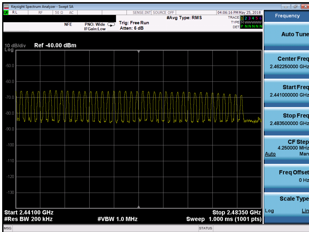
Plot 7-36. High End Spectrum Channel Hopping Plot (Bluetooth)
