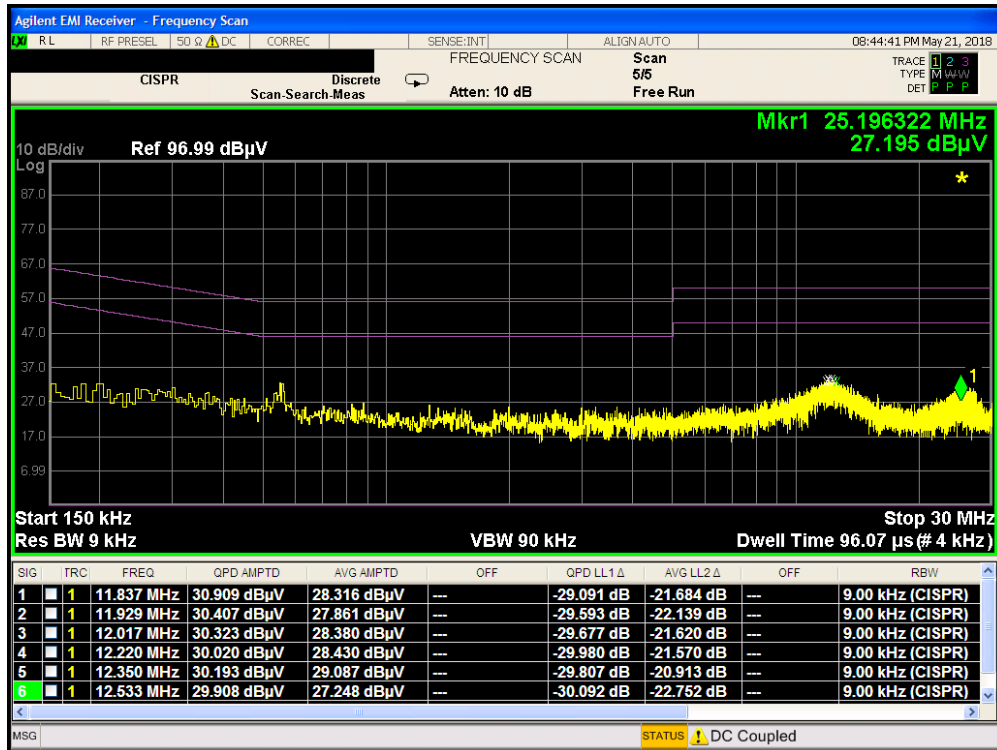
Plot 7-64. Line Conducted Plot with Bluetooth LE (L1)
