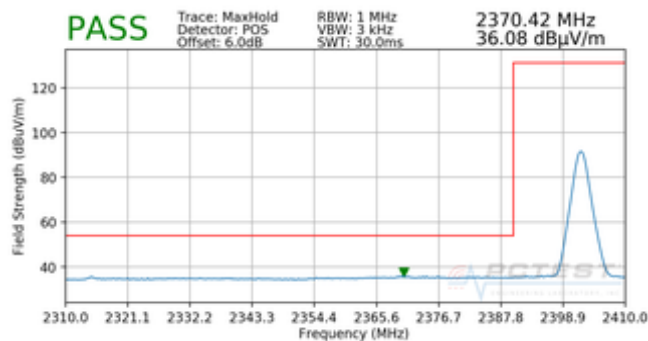
Plot 7-59. Radiated Restricted Lower Band Edge Measurement (Average)
