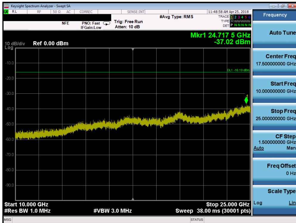
Plot 7-38. Conducted Spurious Plot (Bluetooth (LE), 250kbps – Ch. 0)
