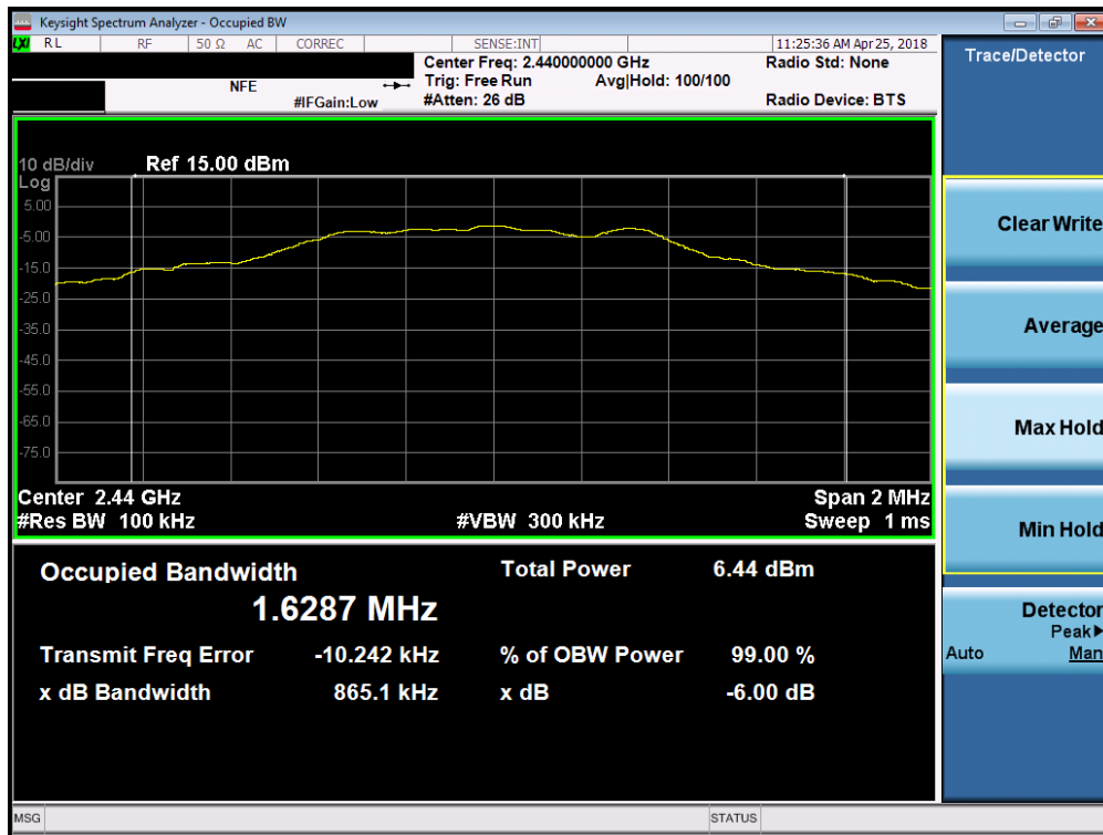
Plot 7-8. 6dB Bandwidth Plot (Bluetooth (LE), 2Mbps – Ch. 19)
