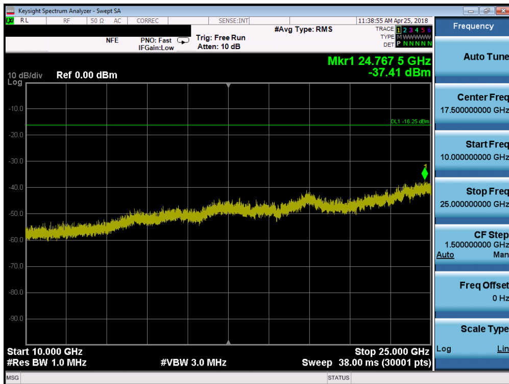
Plot 7-44. Conducted Spurious Plot (Bluetooth (LE), 1Mbps – Ch. 0)
