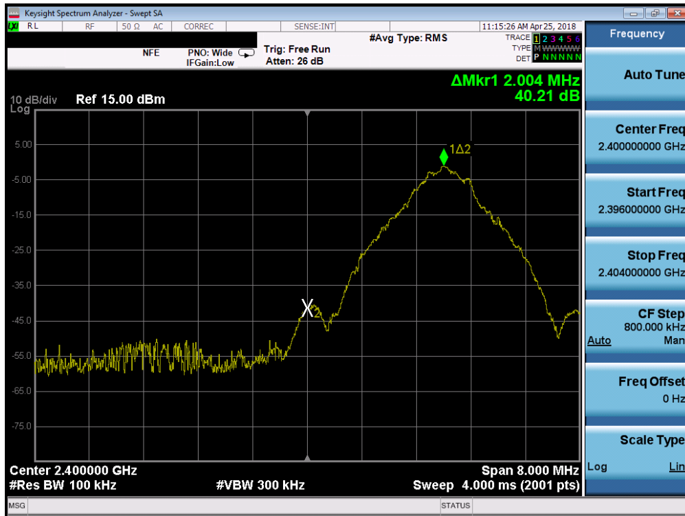
Plot 7-32. Band Edge Plot (Bluetooth (LE), 2Mbps – Ch. 0)
