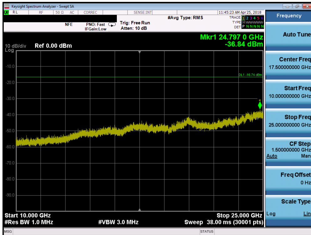
Plot 7-42. Conducted Spurious Plot (Bluetooth (LE), 250kbps – Ch. 39)
