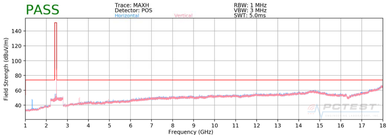
Plot 7-57. Radiated Spurious Plot above 1GHz (Bluetooth LE – Ch. 39)
