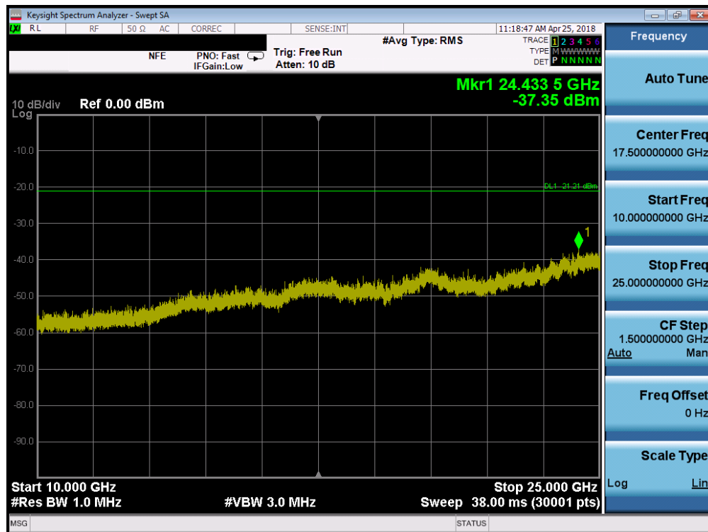
Plot 7-50. Conducted Spurious Plot (Bluetooth (LE), 2Mbps – Ch. 0)
