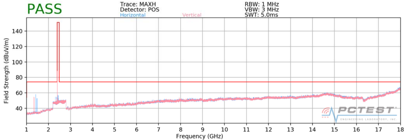
Plot 7-55. Radiated Spurious Plot above 1GHz (Bluetooth LE – Ch. 0)
