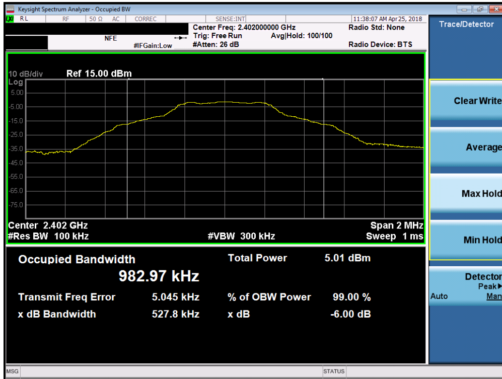
Plot 7-4. 6dB Bandwidth Plot (Bluetooth (LE), 1Mbps – Ch. 0)
