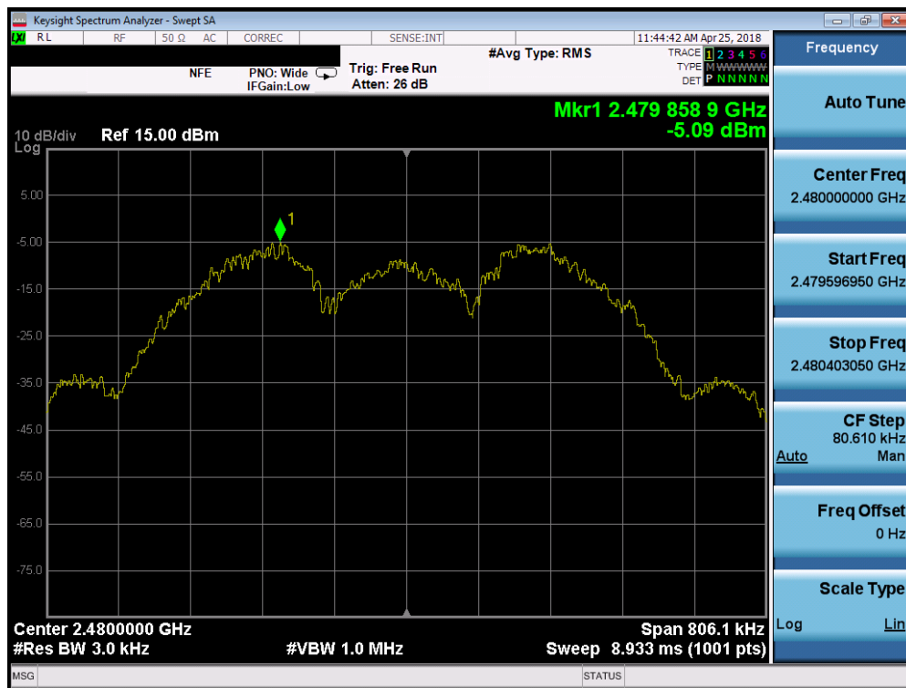
Plot 7-21. Power Spectral Density Plot (Bluetooth (LE), 250kbps – Ch. 39)
