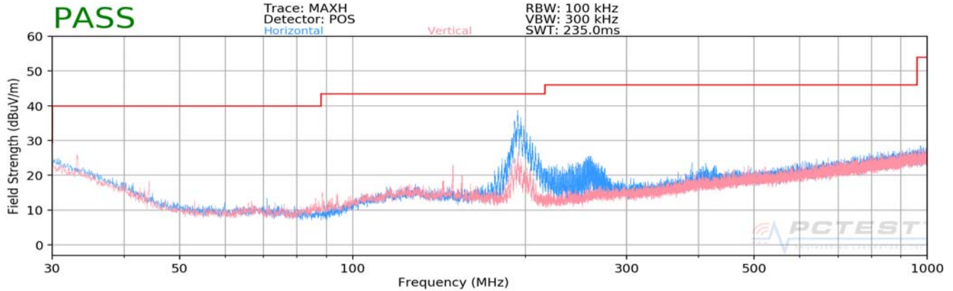
Plot 7-63. Radiated Spurious Plot below 1GHz
