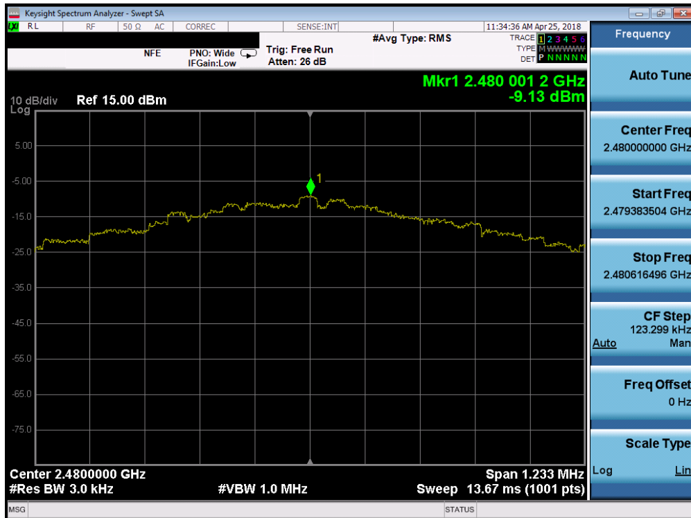
Plot 7-27. Power Spectral Density Plot (Bluetooth (LE), 2Mbps – Ch. 39)
