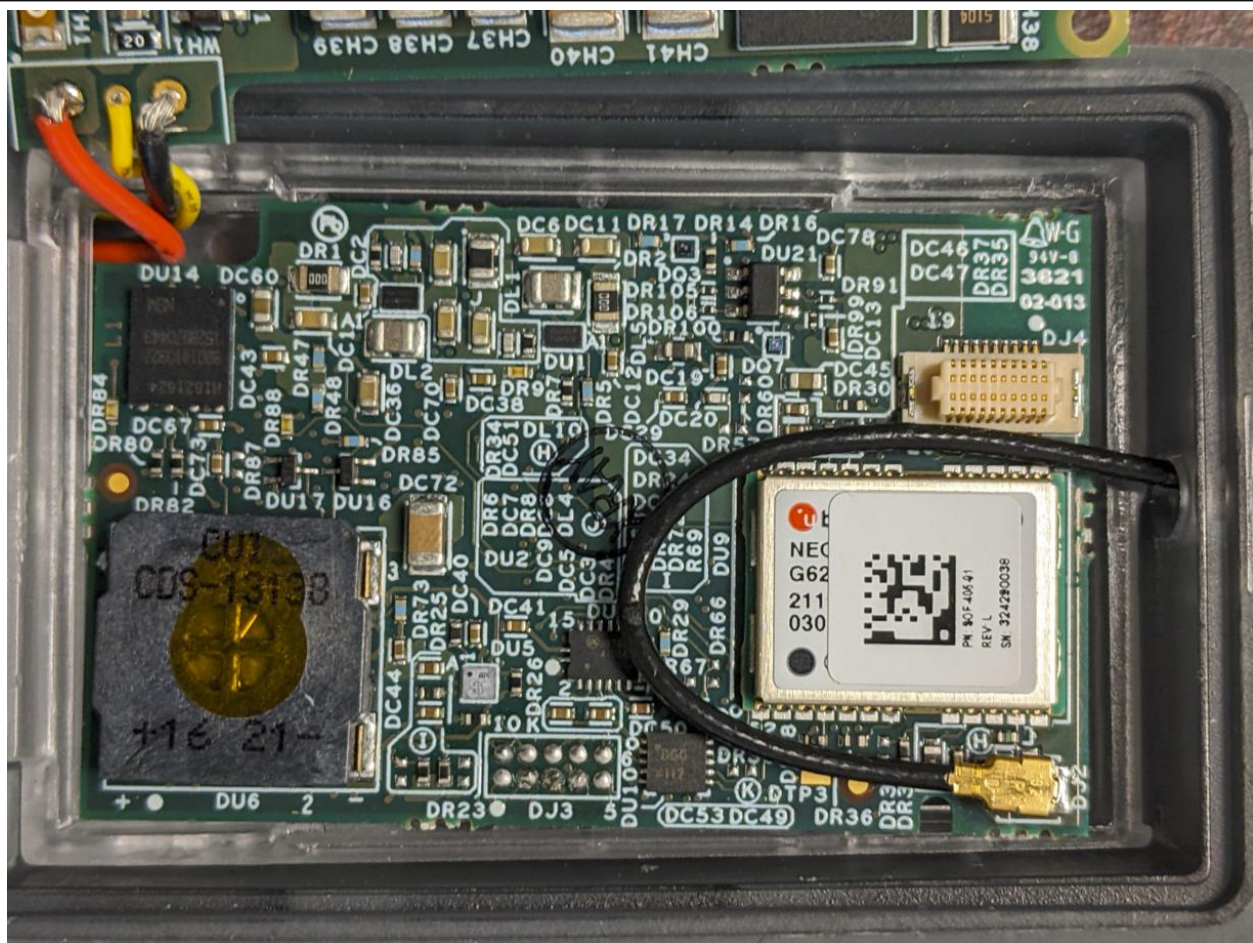
Figure 3: Digital Board – back
