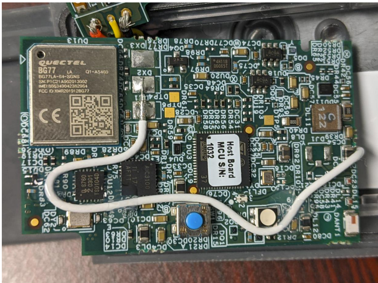
Figure 2: Digital Board – front
