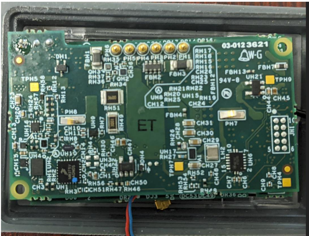
Figure 5: Analog Board – back
