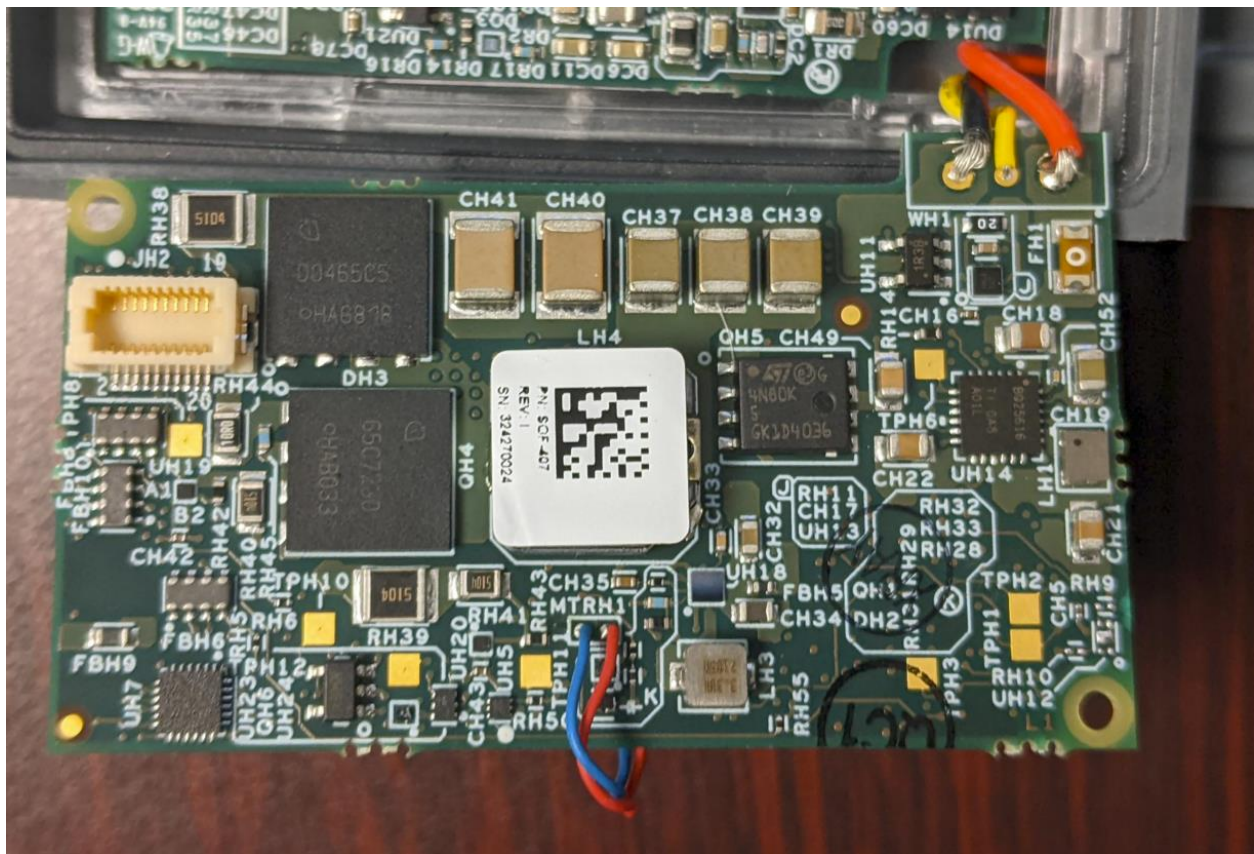
Figure 4: Analog Board – front
