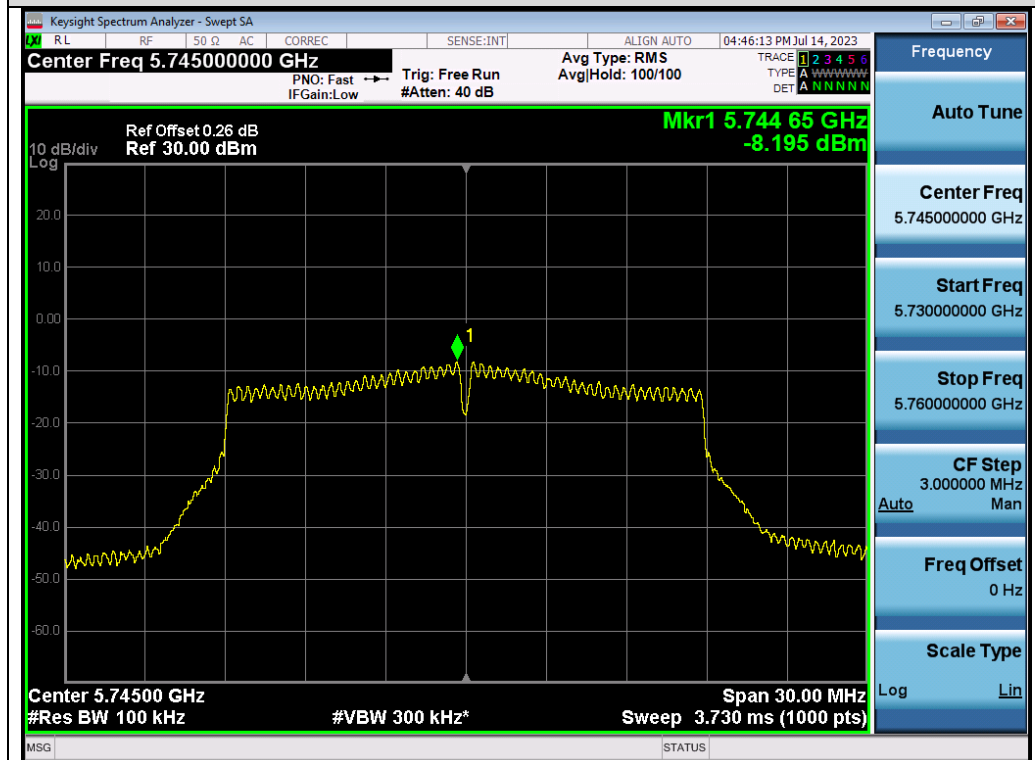
Test_Graph_802.11ac20_ANT1_5745_MCS0_PSD
