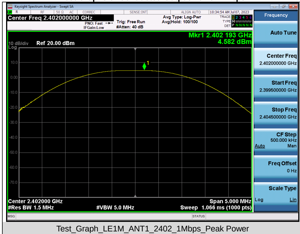
Test Graphs of Conducted Output Power-1Mbps
