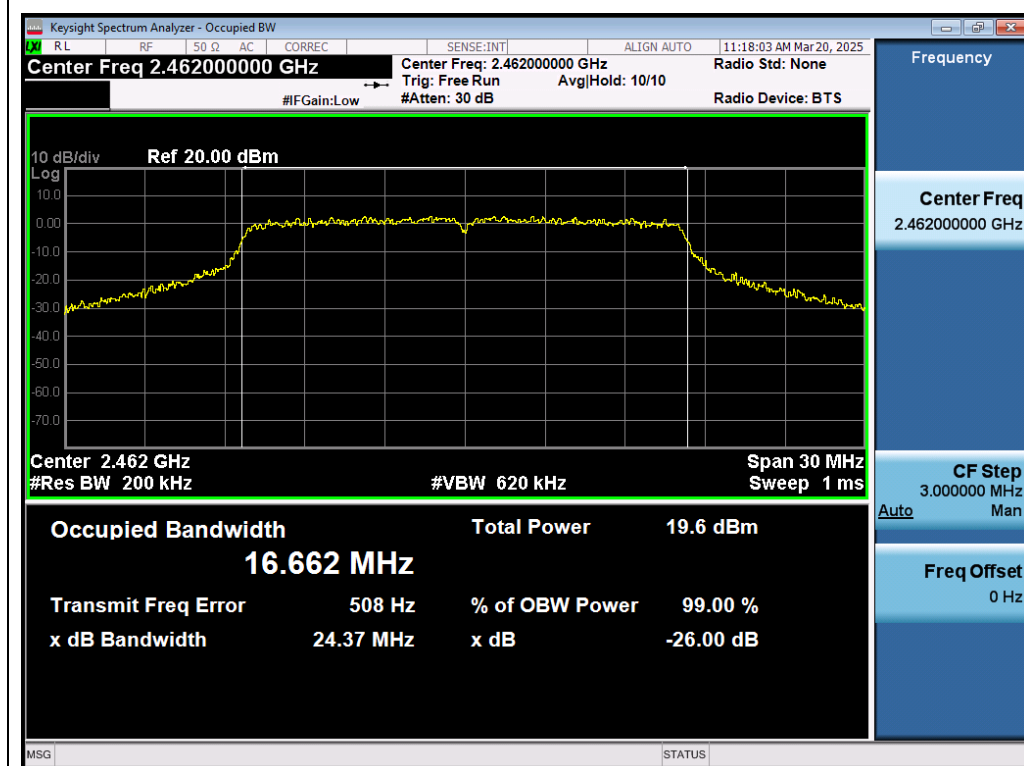
Test_Graph_802.11g_ANT1_2462_6Mbps_OBW
