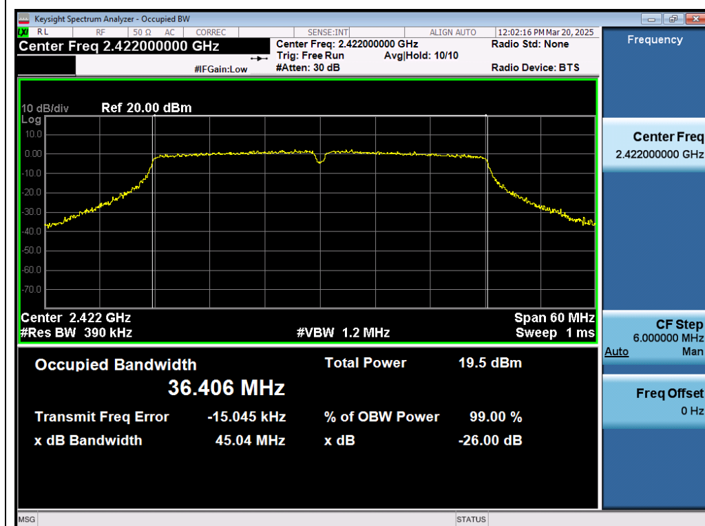
Test_Graph_802.11n40_ANT1_2422_MCS0_OBW
