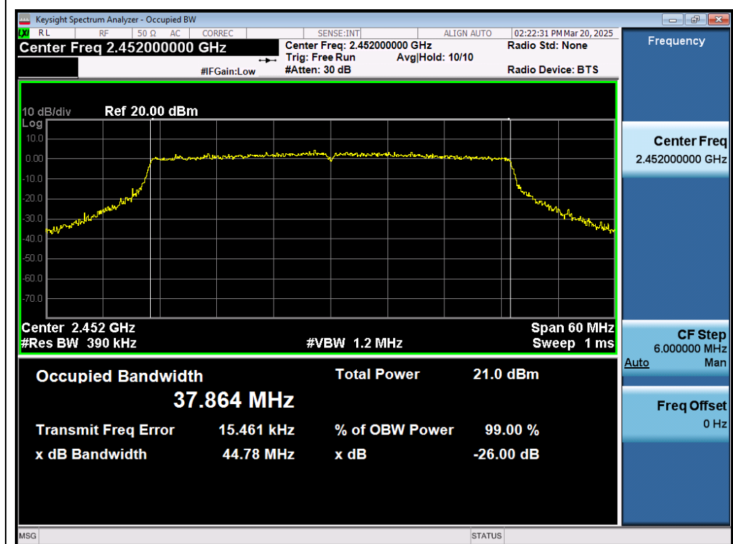
Test_Graph_802.11ax40_ANT1_2452_MCS0_OBW
