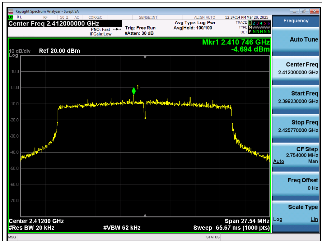
Test_Graph_802.11ax20_ANT1_2412_MCS0_PSD
