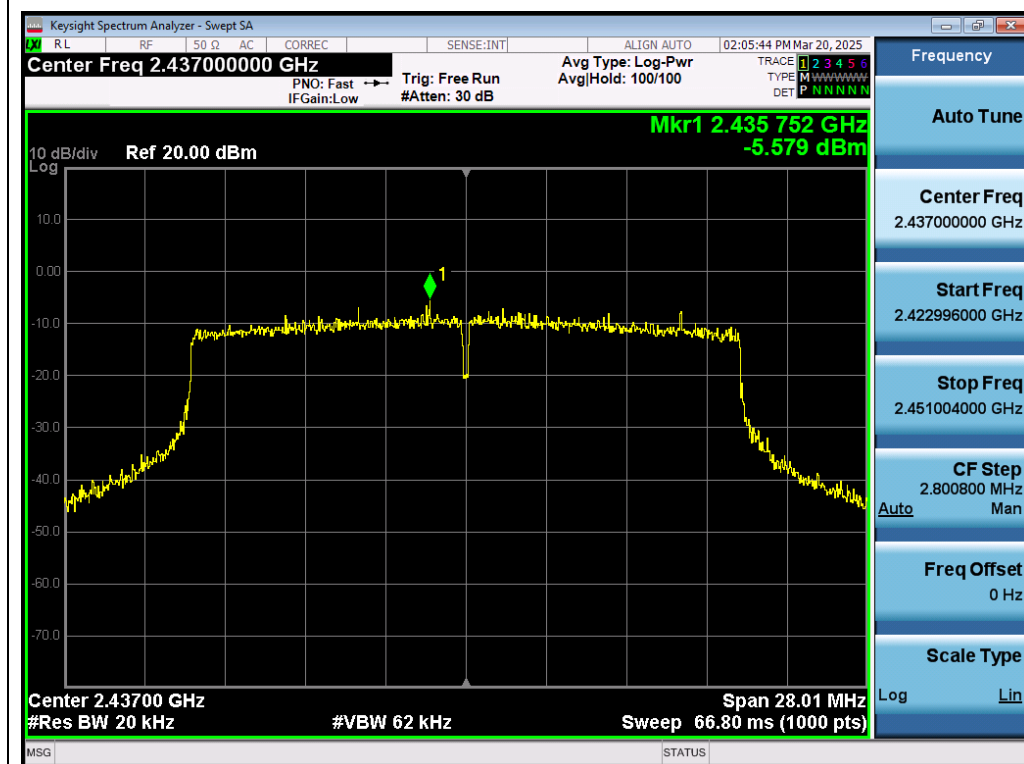
Test_Graph_802.11ax20_ANT1_2437_MCS0_PSD
