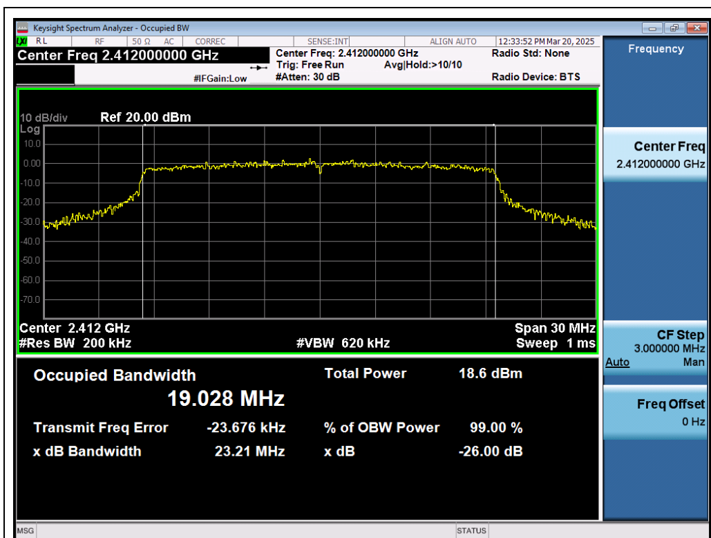
Test_Graph_802.11ax20_ANT1_2412_MCS0_OBW
