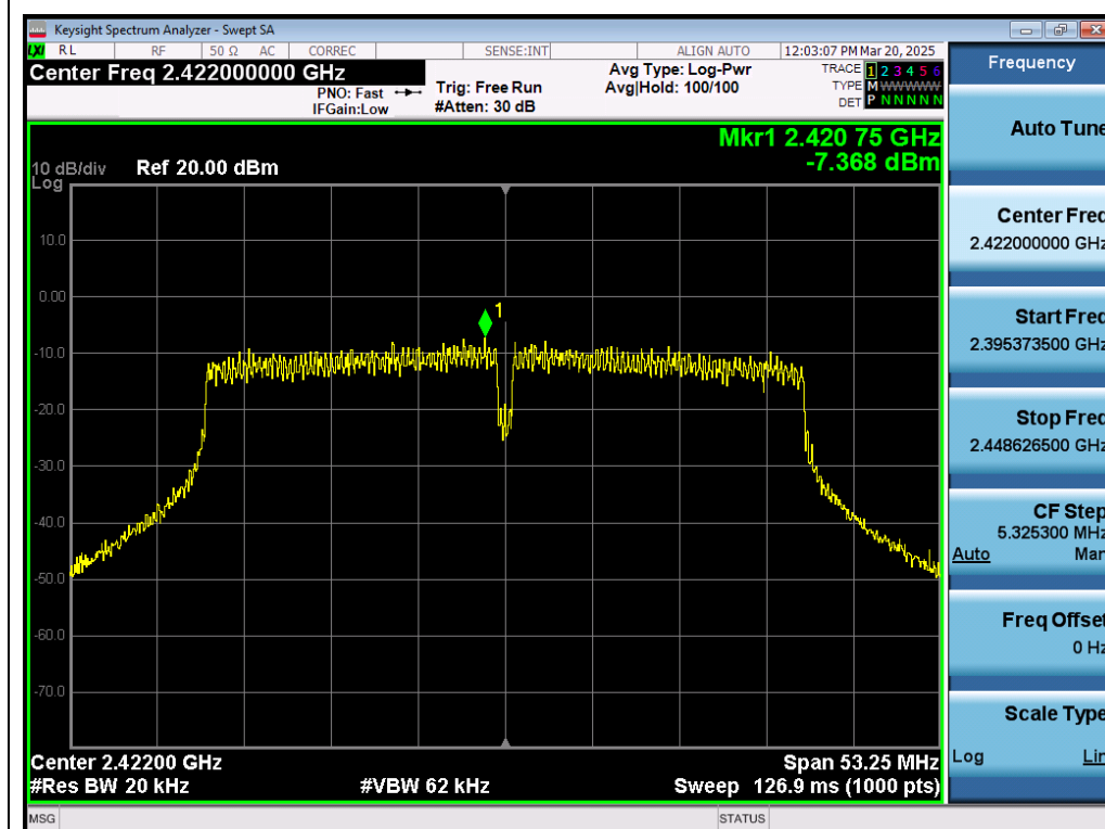
Test_Graph_802.11n40_ANT1_2422_MCS0_PSD
