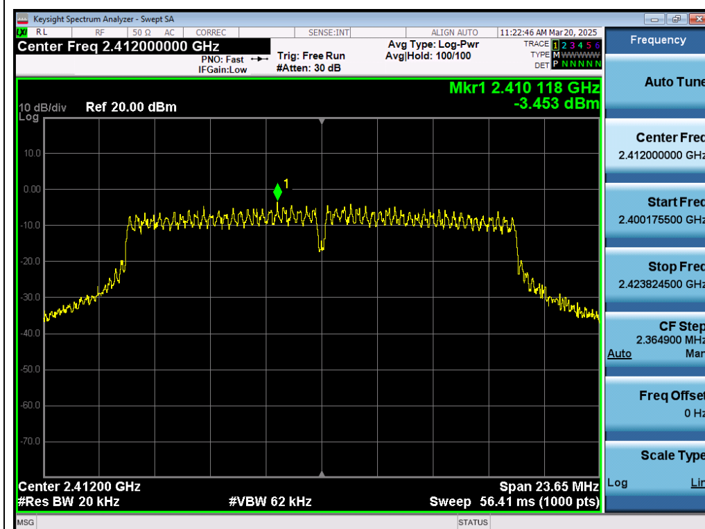
Test_Graph_802.11g_ANT1_2412_6Mbps_PSD
