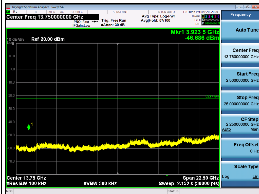
Test_Graph_802.11n40_ANT1_2452_MCS0_Higher Band Emissions
