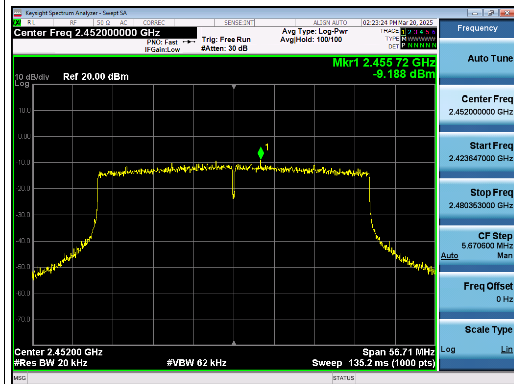
Test_Graph_802.11ax40_ANT1_2452_MCS0_PSD
