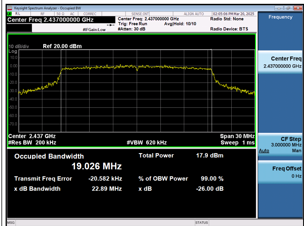
Test_Graph_802.11ax20_ANT1_2437_MCS0_OBW
