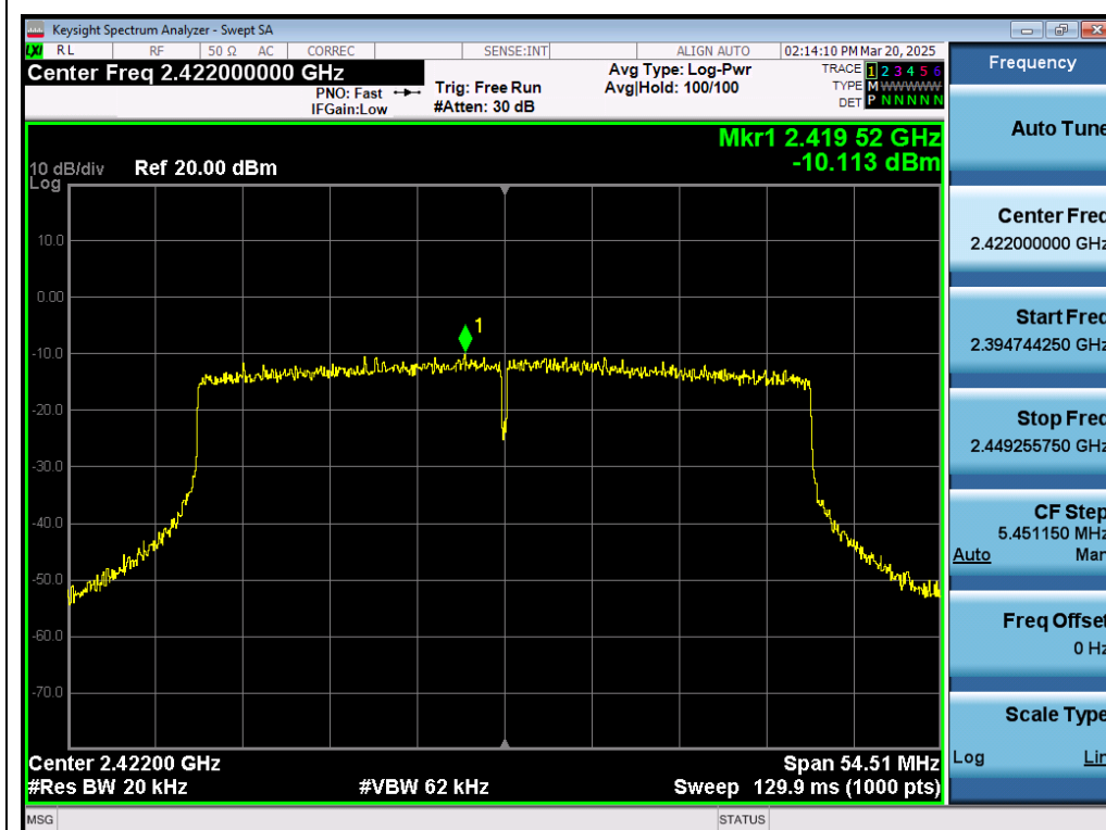
Test_Graph_802.11ax40_ANT1_2422_MCS0_PSD
