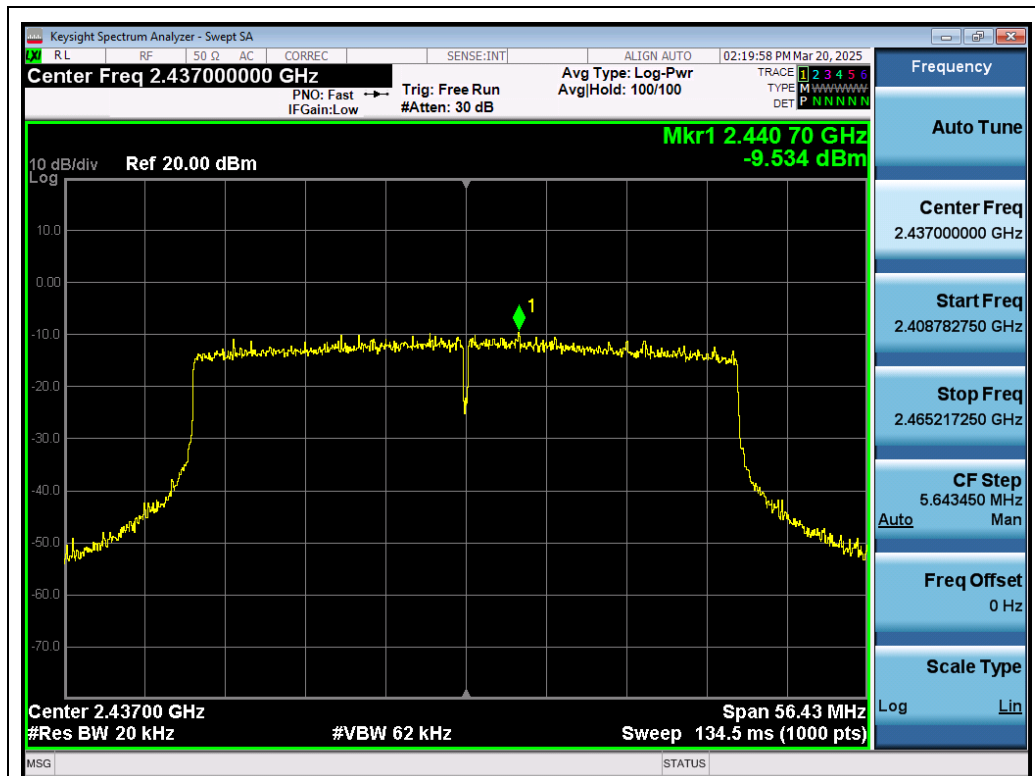
Test_Graph_802.11ax40_ANT1_2437_MCS0_PSD
