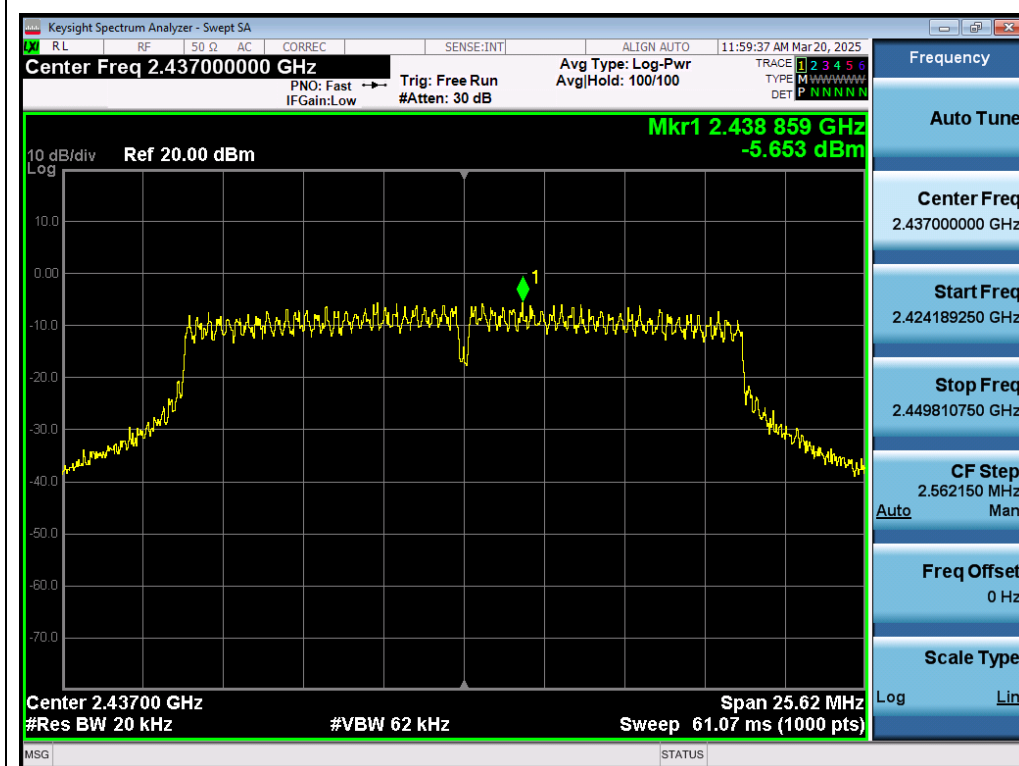
Test_Graph_802.11n20_ANT1_2437_MCS0_PSD
