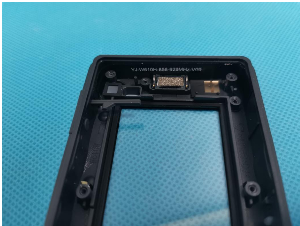
SRD ANTENNA
