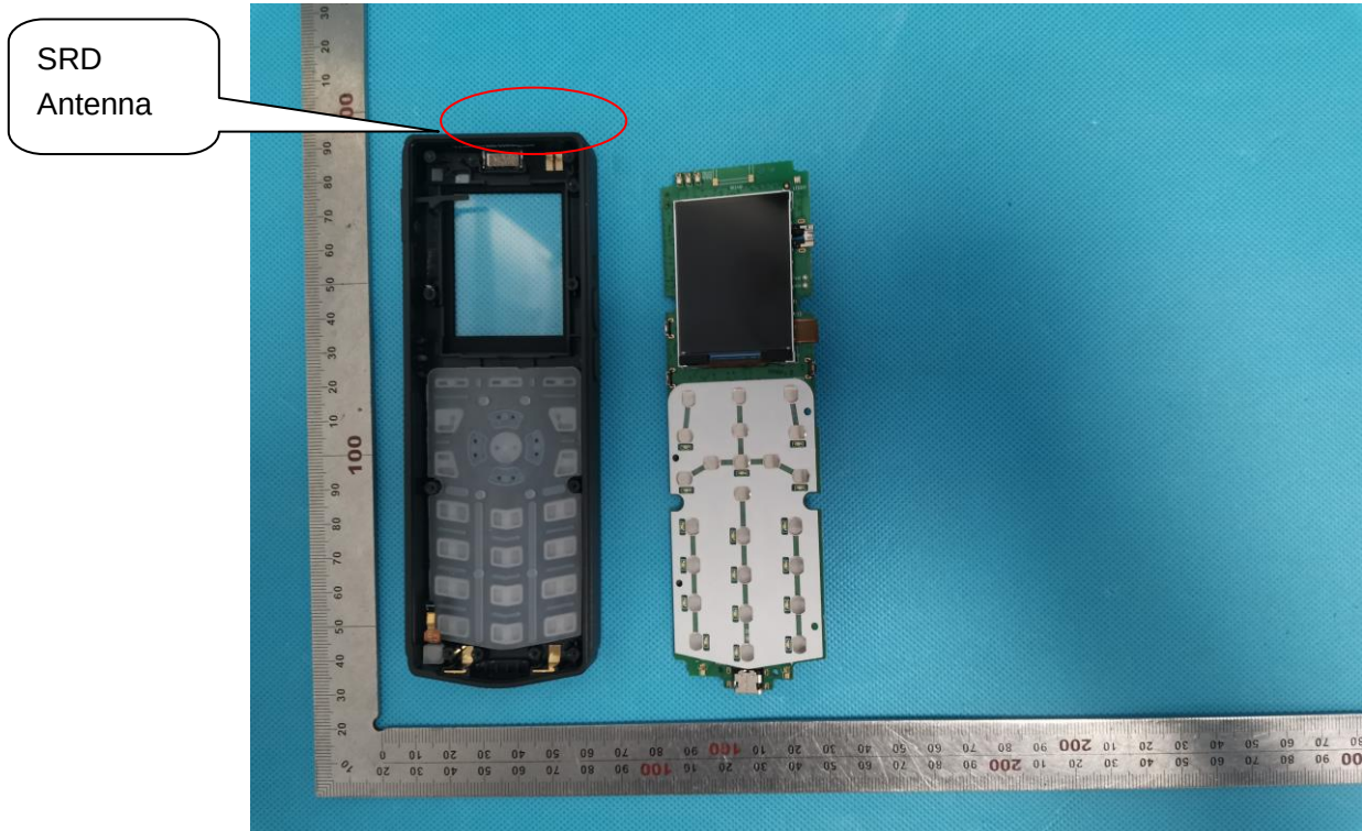
SRD ANTENNA
