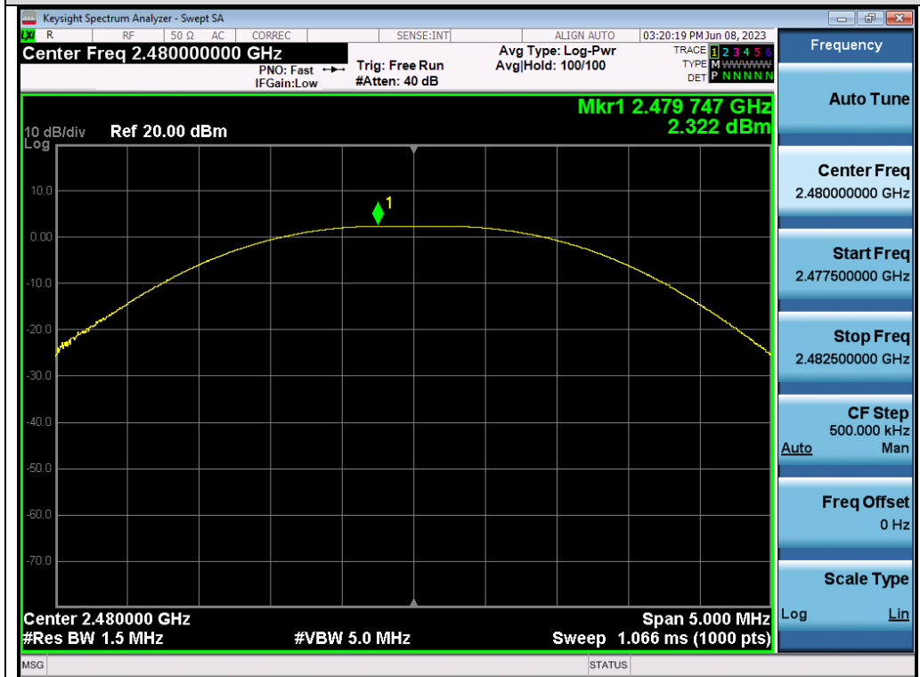
Test_Graph_LE1M_ANT1_2480_1Mbps_Peak Power
