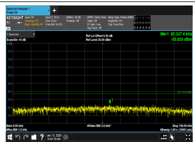
GPRS1900-512-0-0.009~0.15MHz-PASS
