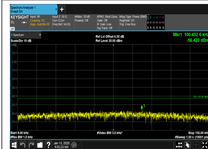
EGPRS1900-512-2-0.009~0.15MHz-PASS
