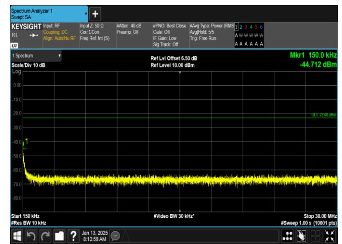
EGPRS850-251-8-0.15~30MHz-PASS
