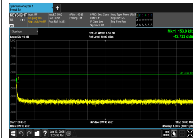
EGPRS1900-661-2-0.15~30MHz-PASS
