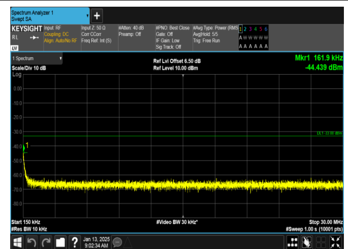
EGPRS1900-512-2-0.15~30MHz-PASS
