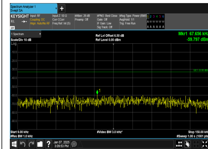
Band12-3MHz-QPSK-23025-15RB#0-0.009~0.15-PASS
