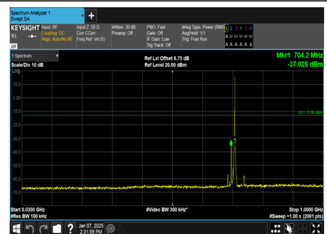
Band12-1.4MHz-QPSK-23173-1RB#5-30~1000-PASS
