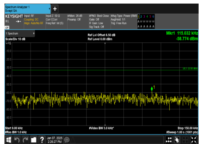
Band12-1.4MHz-16QAM-23095-1RB#5-0.009~0.15-PASS
