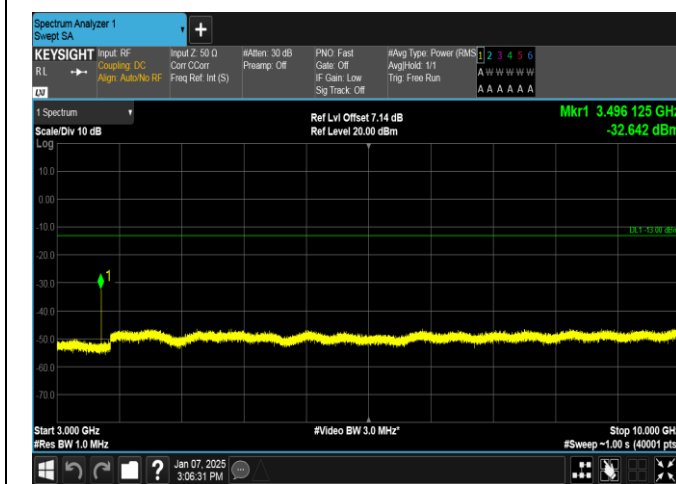
Band12-3MHz-QPSK-23025-1RB#0-3000~10000-PASS
