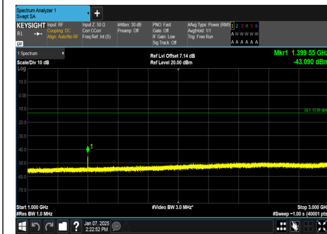
Band12-1.4MHz-16QAM-23017-6RB#0-1000~3000-PASS
