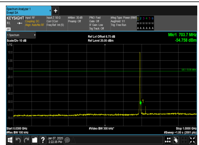
Band12-1.4MHz-16QAM-23017-6RB#0-30~1000-PASS
