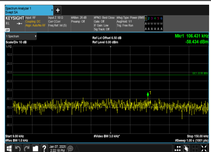
Band12-1.4MHz-16QAM-23017-6RB#0-0.009~0.15-PASS
