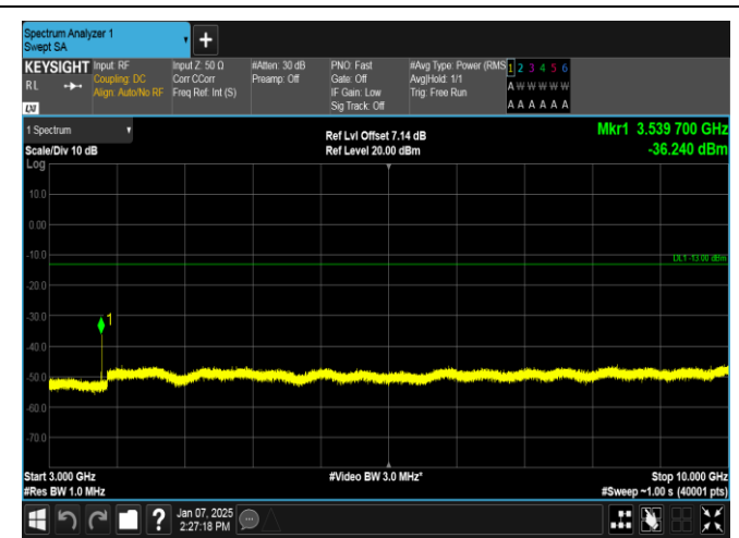
Band12-1.4MHz-16QAM-23095-1RB#5-3000~10000-PASS
