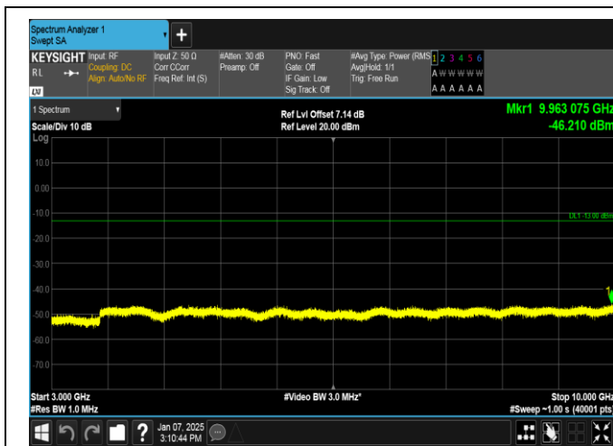
Band12-3MHz-QPSK-23025-15RB#0-3000~10000-PASS
