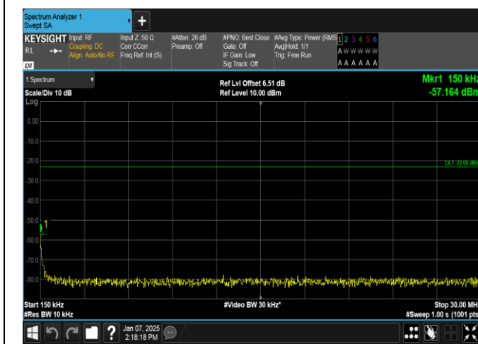
Band12-1.4MHz-16QAM-23017-1RB#0-0.15~30-PASS
