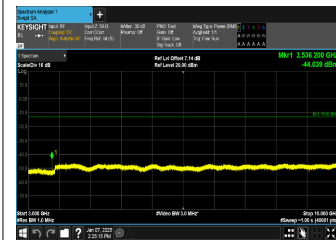
Band12-1.4MHz-16QAM-23095-1RB#0-3000~10000-PASS
