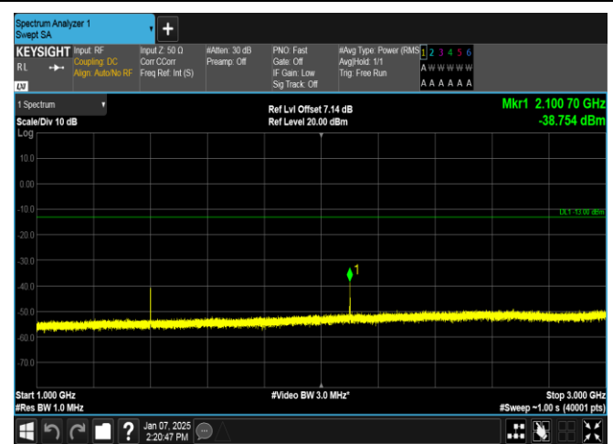
Band12-1.4MHz-16QAM-23017-1RB#5-1000~3000-PASS
