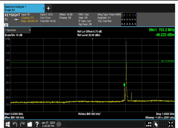
Band12-1.4MHz-16QAM-23173-1RB#0-30~1000-PASS
