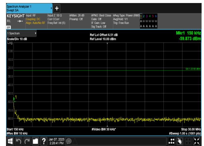
Band12-1.4MHz-16QAM-23095-6RB#0-0.15~30-PASS
