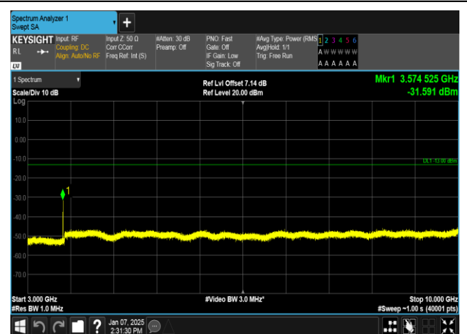
Band12-1.4MHz-16QAM-23173-1RB#0-3000~10000-PASS
