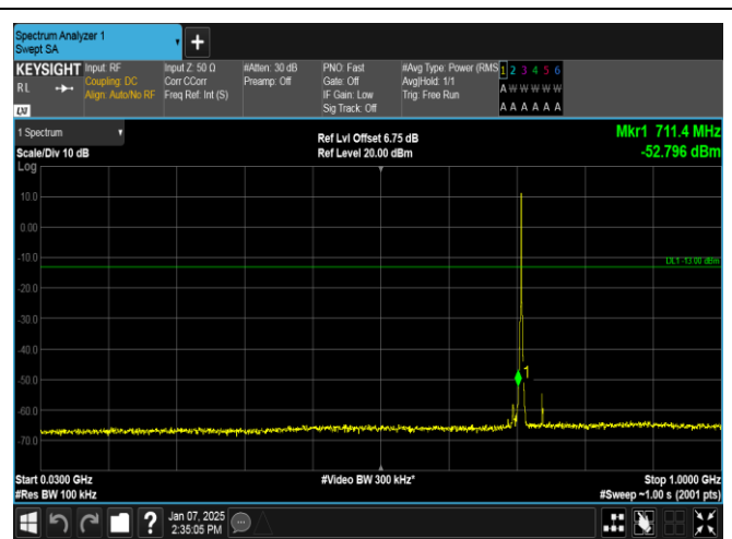
Band12-1.4MHz-16QAM-23173-6RB#0-30~1000-PASS
