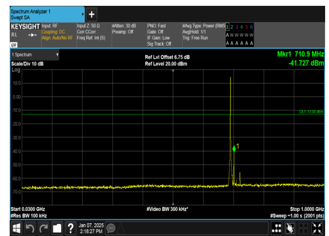
Band12-1.4MHz-16QAM-23017-1RB#0-30~1000-PASS
