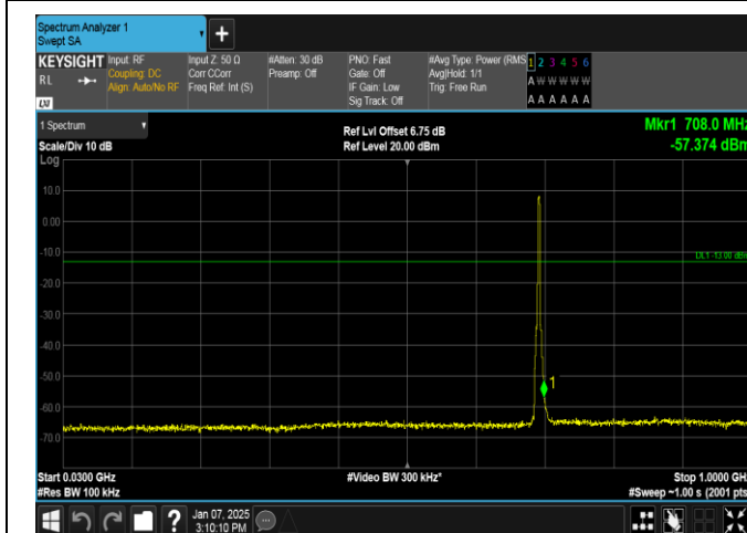
Band12-3MHz-QPSK-23025-15RB#0-30~1000-PASS
