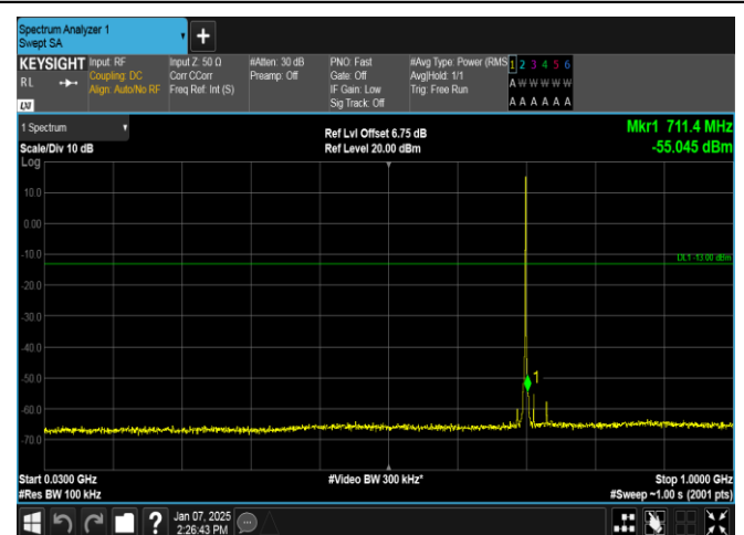
Band12-1.4MHz-16QAM-23095-1RB#5-30~1000-PASS
