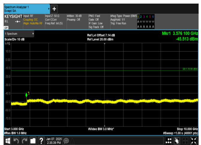
Band12-1.4MHz-16QAM-23173-6RB#0-3000~10000-PASS
