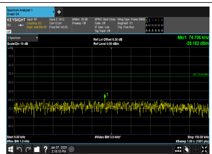
Band12-1.4MHz-16QAM-23017-1RB#0-0.009~0.15-PASS
