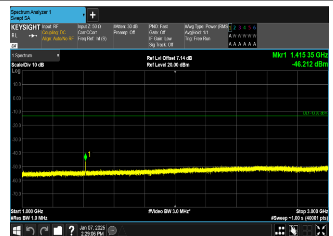
Band12-1.4MHz-16QAM-23095-6RB#0-1000~3000-PASS
