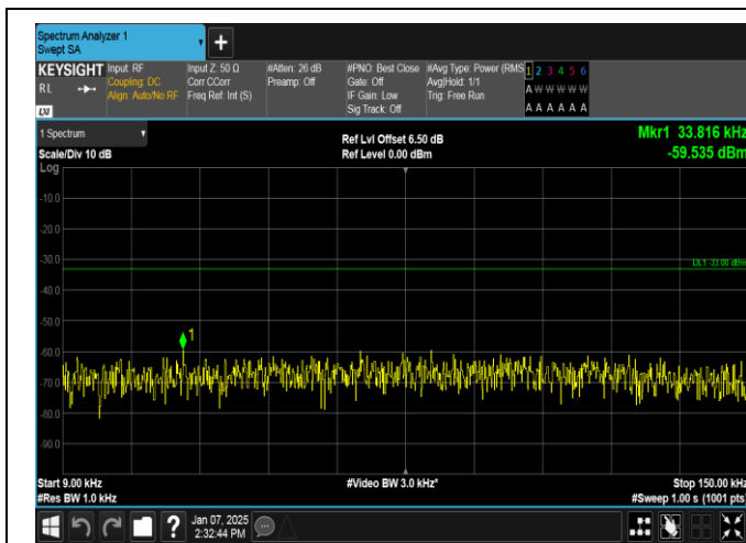
Band12-1.4MHz-16QAM-23173-1RB#5-0.009~0.15-PASS
