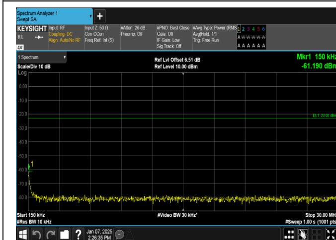
Band12-1.4MHz-16QAM-23095-1RB#5-0.15~30-PASS
