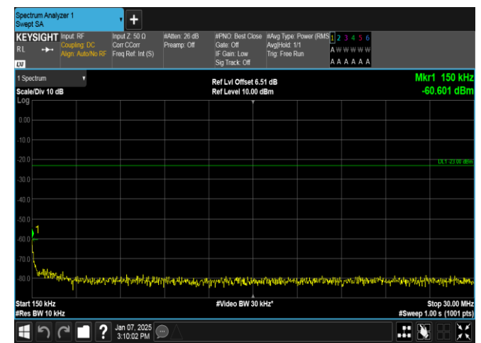
Band12-3MHz-QPSK-23025-15RB#0-0.15~30-PASS
