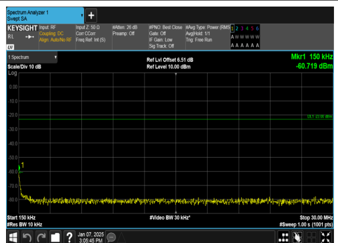
Band12-3MHz-QPSK-23025-1RB#0-0.15~30-PASS
