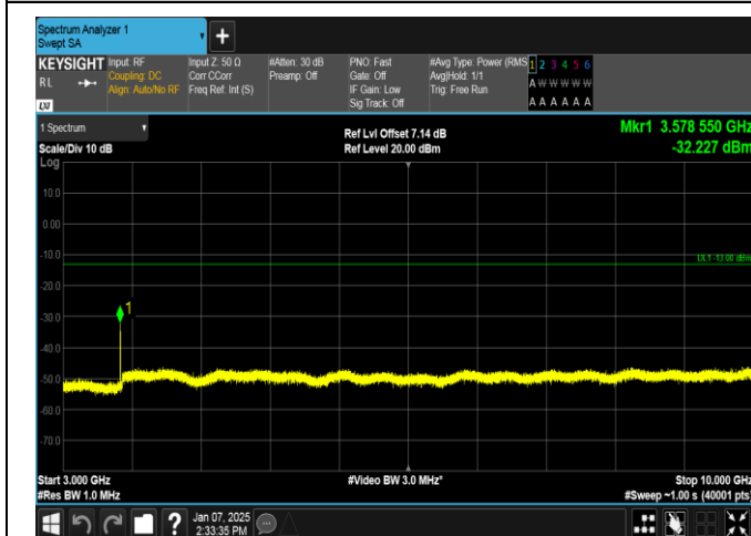
Band12-1.4MHz-16QAM-23173-1RB#5-3000~10000-PASS
