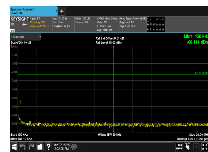
Band12-1.4MHz-16QAM-23017-6RB#0-0.15~30-PASS
