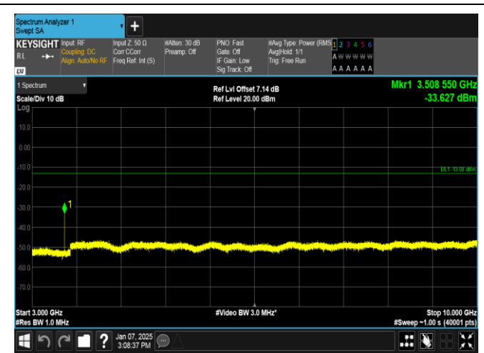
Band12-3MHz-QPSK-23025-1RB#14-3000~10000-PASS
