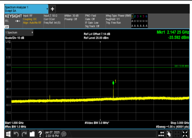
Band12-1.4MHz-16QAM-23173-1RB#5-1000~3000-PASS
