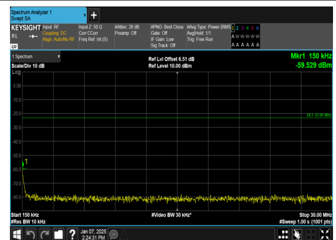
Band12-1.4MHz-16QAM-23095-1RB#0-0.15~30-PASS
