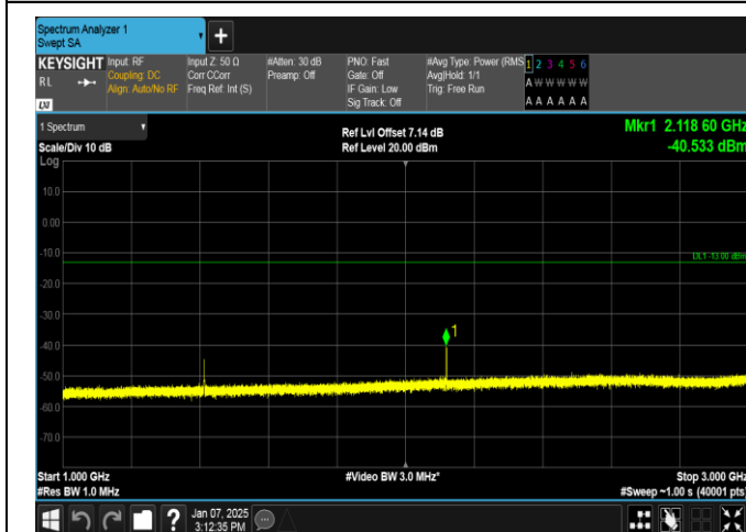
Band12-3MHz-QPSK-23095-1RB#0-1000~3000-PASS
