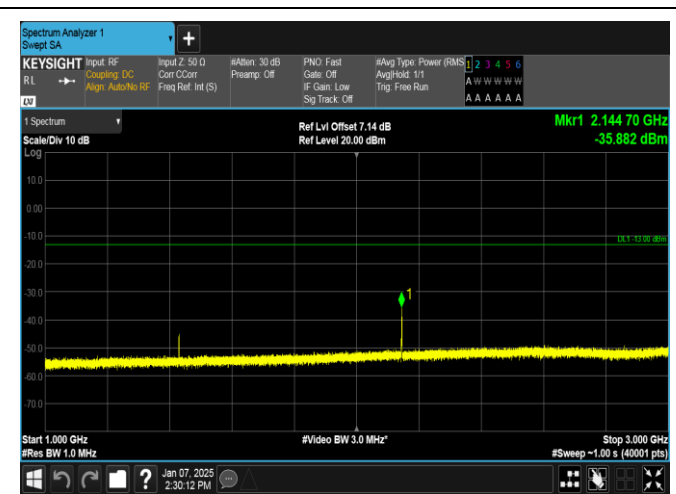
Band12-1.4MHz-QPSK-23173-1RB#0-1000~3000-PASS
