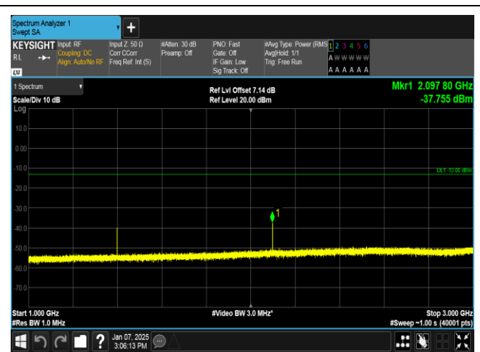
Band12-3MHz-QPSK-23025-1RB#0-1000~3000-PASS
