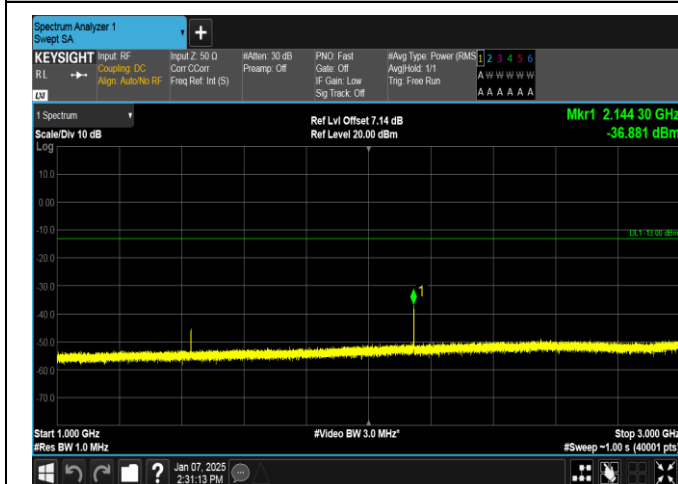
Band12-1.4MHz-16QAM-23173-1RB#0-1000~3000-PASS
