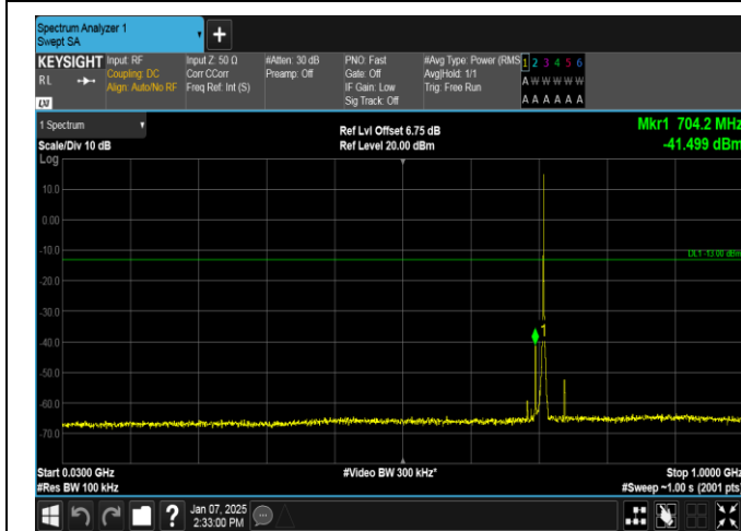
Band12-1.4MHz-16QAM-23173-1RB#5-30~1000-PASS
