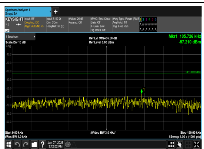
Band12-3MHz-QPSK-23095-1RB#0-0.009~0.15-PASS
