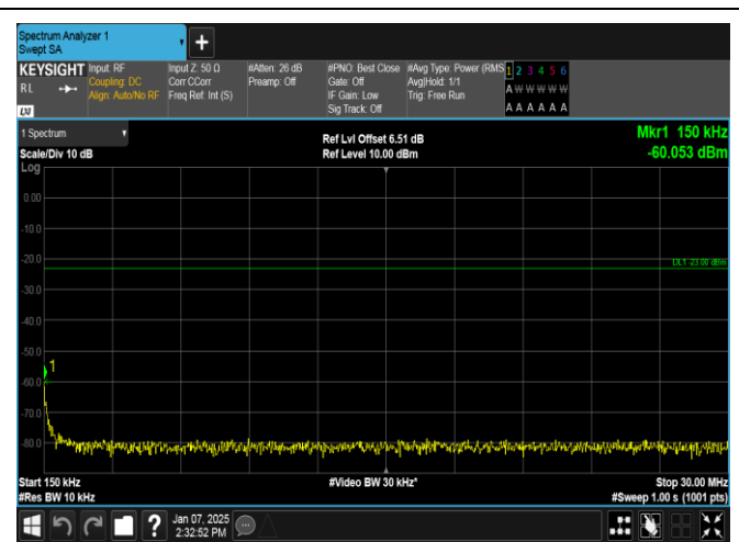
Band12-1.4MHz-16QAM-23173-1RB#5-0.15~30-PASS
