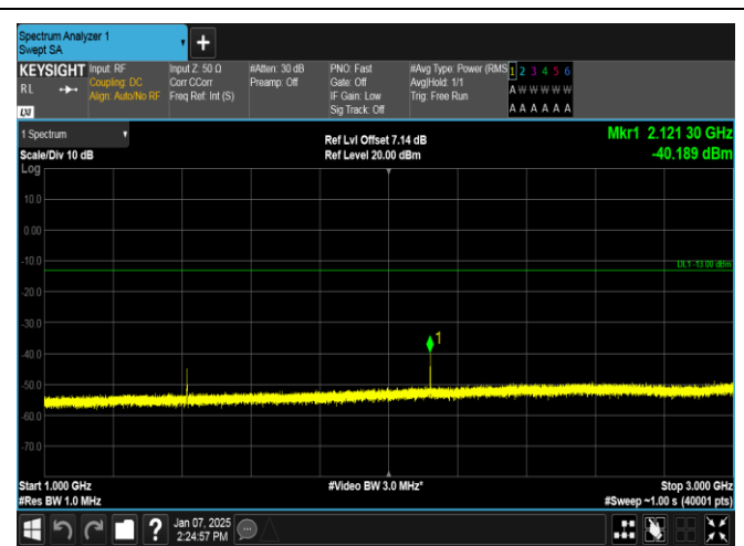
Band12-1.4MHz-16QAM-23095-1RB#0-1000~3000-PASS
