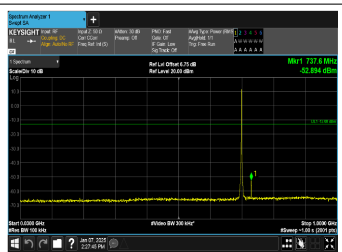
Band12-1.4MHz-QPSK-23095-6RB#0-30~1000-PASS
