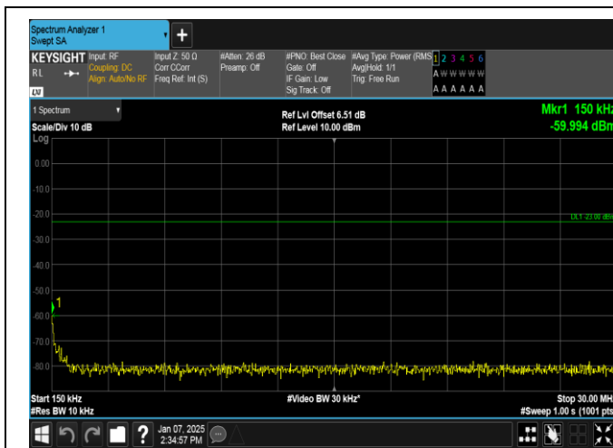
Band12-1.4MHz-16QAM-23173-6RB#0-0.15~30-PASS
