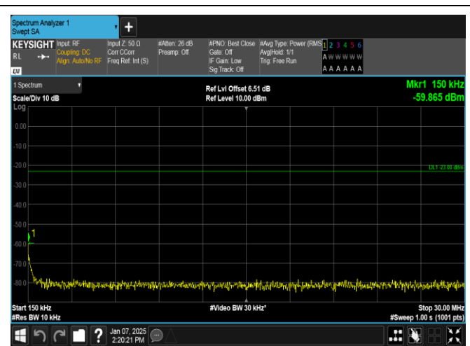
Band12-1.4MHz-16QAM-23017-1RB#5-0.15~30-PASS
