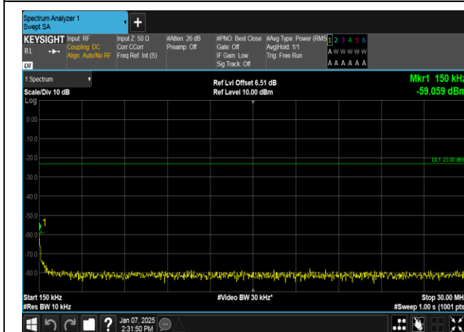
Band12-1.4MHz-QPSK-23173-1RB#5-0.15~30-PASS
