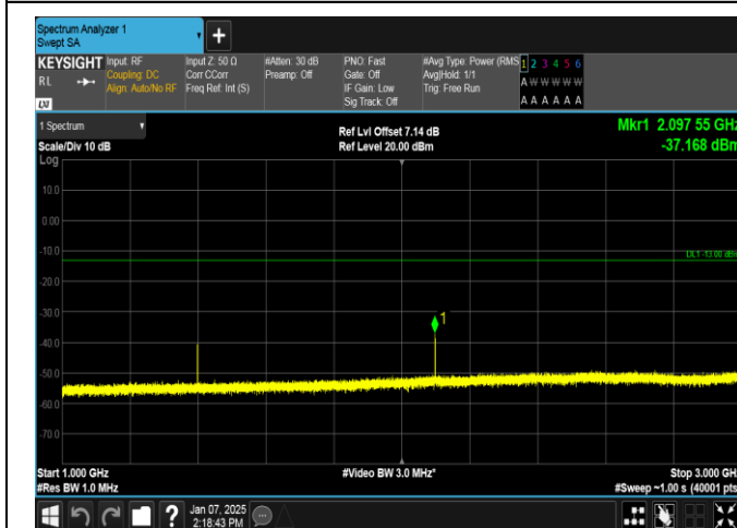
Band12-1.4MHz-16QAM-23017-1RB#0-1000~3000-PASS
