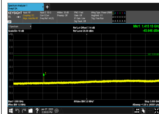
Band12-1.4MHz-QPSK-23095-6RB#0-1000~3000-PASS
