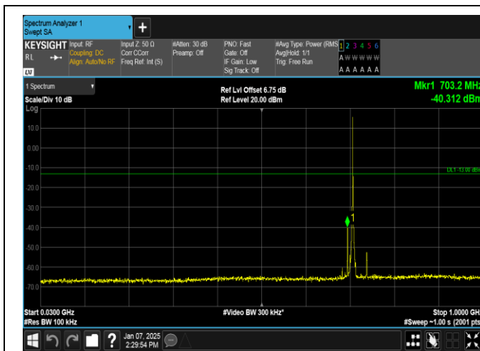
Band12-1.4MHz-QPSK-23173-1RB#0-30~1000-PASS
