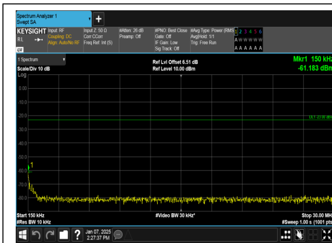
Band12-1.4MHz-QPSK-23095-6RB#0-0.15~30-PASS
