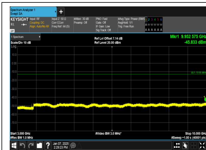
Band12-1.4MHz-16QAM-23095-6RB#0-3000~10000-PASS
