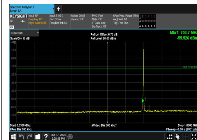
Band12-1.4MHz-16QAM-23095-6RB#0-30~1000-PASS
