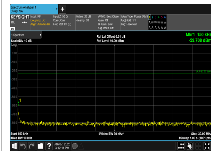
Band12-3MHz-QPSK-23095-1RB#0-0.15~30-PASS
