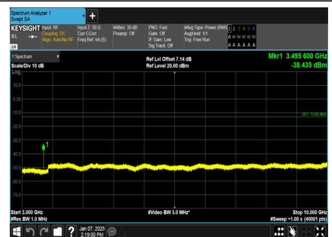
Band12-1.4MHz-16QAM-23017-1RB#0-3000~10000-PASS
