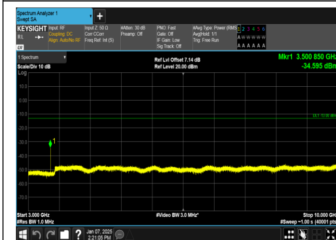
Band12-1.4MHz-16QAM-23017-1RB#5-3000~10000-PASS
