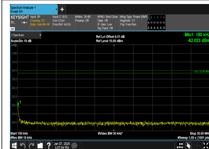
Band12-3MHz-QPSK-23025-1RB#14-0.15~30-PASS
