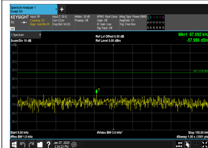
Band12-1.4MHz-16QAM-23095-1RB#0-0.009~0.15-PASS
