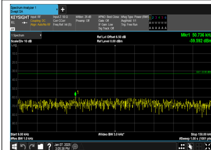
Band12-3MHz-QPSK-23025-1RB#0-0.009~0.15-PASS
