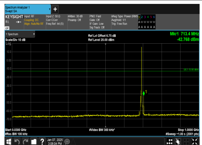
Band12-3MHz-QPSK-23025-1RB#14-30~1000-PASS
