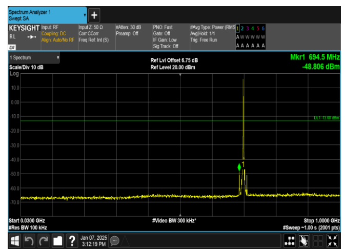
Band12-3MHz-QPSK-23095-1RB#0-30~1000-PASS
