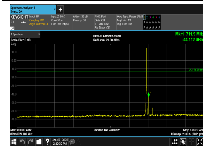
Band12-1.4MHz-16QAM-23017-1RB#5-30~1000-PASS
