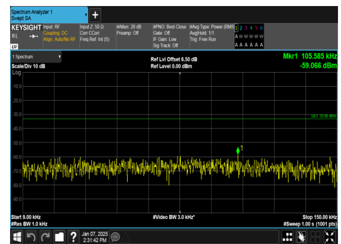
Band12-1.4MHz-QPSK-23173-1RB#5-0.009~0.15-PASS
