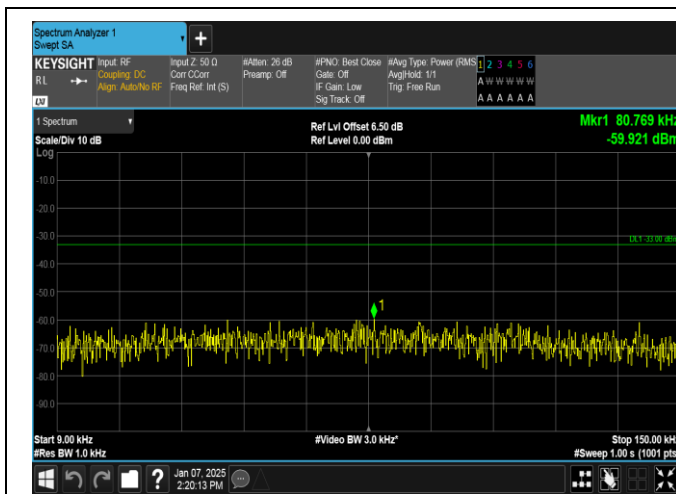
Band12-1.4MHz-16QAM-23017-1RB#5-0.009~0.15-PASS
