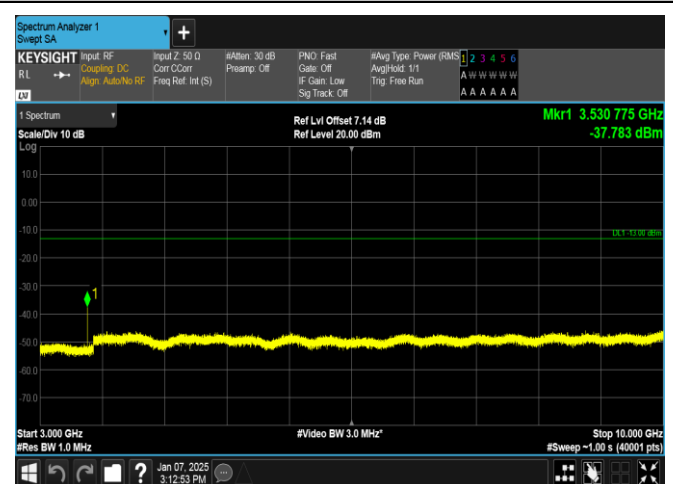
Band12-3MHz-QPSK-23095-1RB#0-3000~10000-PASS
