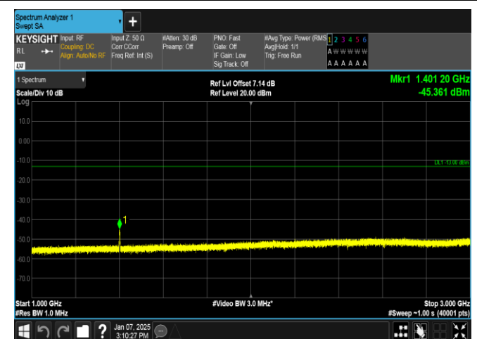
Band12-3MHz-QPSK-23025-15RB#0-1000~3000-PASS
