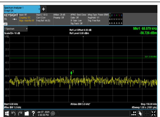
Band12-1.4MHz-16QAM-23173-1RB#0-0.009~0.15-PASS
