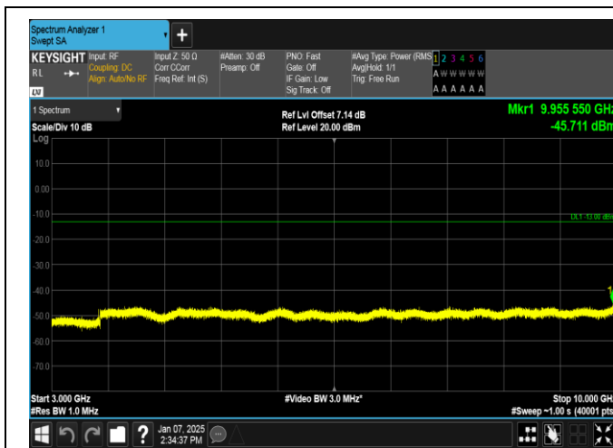
Band12-1.4MHz-QPSK-23173-6RB#0-3000~10000-PASS
