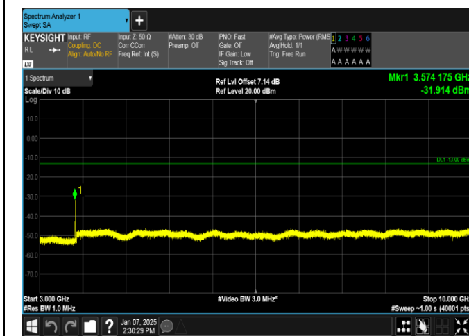
Band12-1.4MHz-QPSK-23173-1RB#0-3000~10000-PASS
