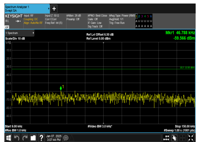
Band12-3MHz-QPSK-23025-1RB#14-0.009~0.15-PASS
