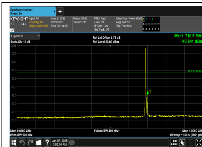
Band12-3MHz-QPSK-23025-1RB#0-30~1000-PASS
