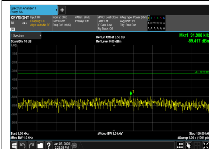
Band12-1.4MHz-QPSK-23173-1RB#0-0.009~0.15-PASS
