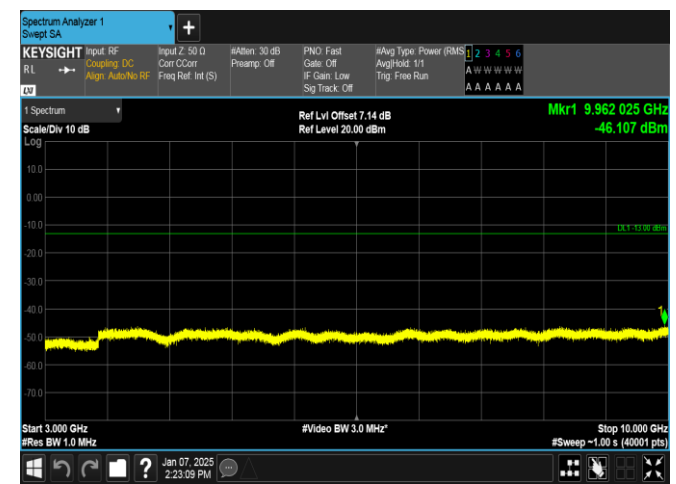
Band12-1.4MHz-16QAM-23017-6RB#0-3000~10000-PASS
