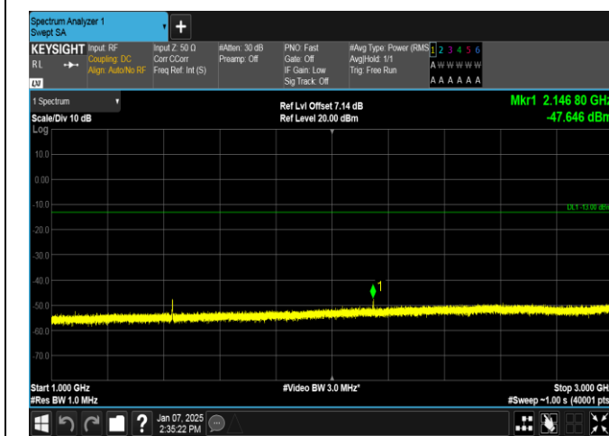
Band12-1.4MHz-16QAM-23173-6RB#0-1000~3000-PASS
