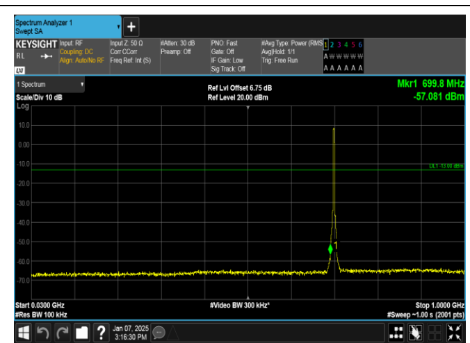
Band12-3MHz-QPSK-23095-15RB#0-30~1000-PASS
