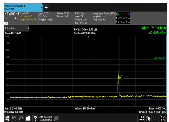
Band12-3MHz-16QAM-23025-1RB#0-30~1000-PASS
