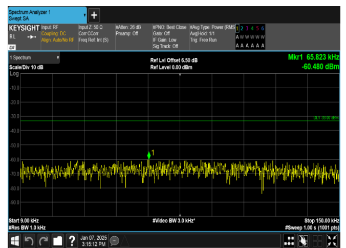
Band12-3MHz-16QAM-23095-1RB#14-0.009~0.15-PASS
