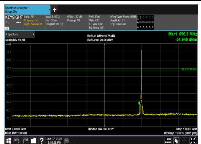
Band12-3MHz-16QAM-23095-1RB#14-30~1000-PASS
