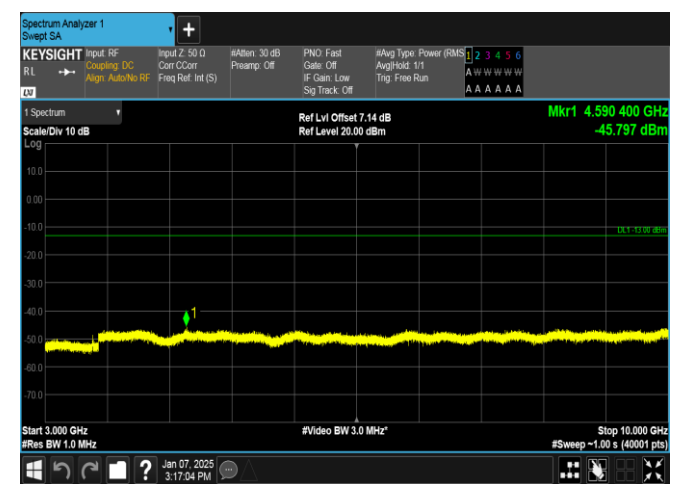
Band12-3MHz-QPSK-23095-15RB#0-3000~10000-PASS
