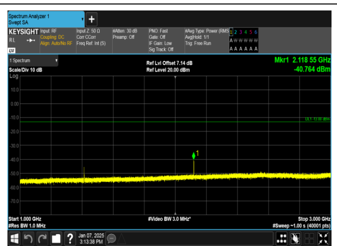
Band12-3MHz-16QAM-23095-1RB#0-1000~3000-PASS
