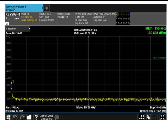
Band12-3MHz-QPSK-23165-1RB#0-0.15~30-PASS
