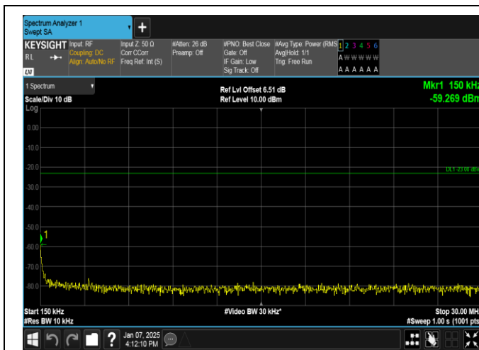
Band12-5MHz-16QAM-23155-25RB#0-0.15~30-PASS
