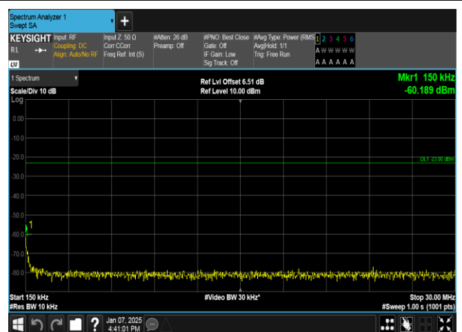
Band12-10MHz-QPSK-23060-1RB#0-0.15~30-PASS
