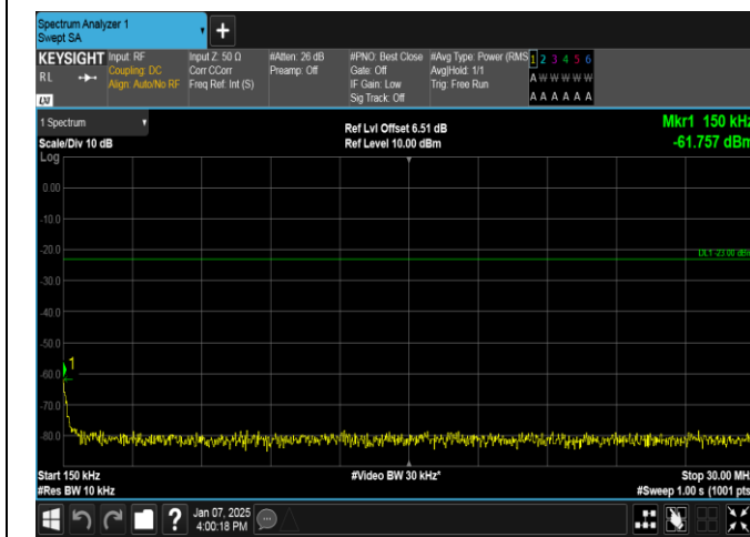
Band12-5MHz-QPSK-23095-1RB#0-0.15~30-PASS
