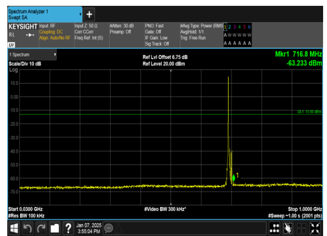
Band12-5MHz-16QAM-23035-1RB#0-30~1000-PASS
