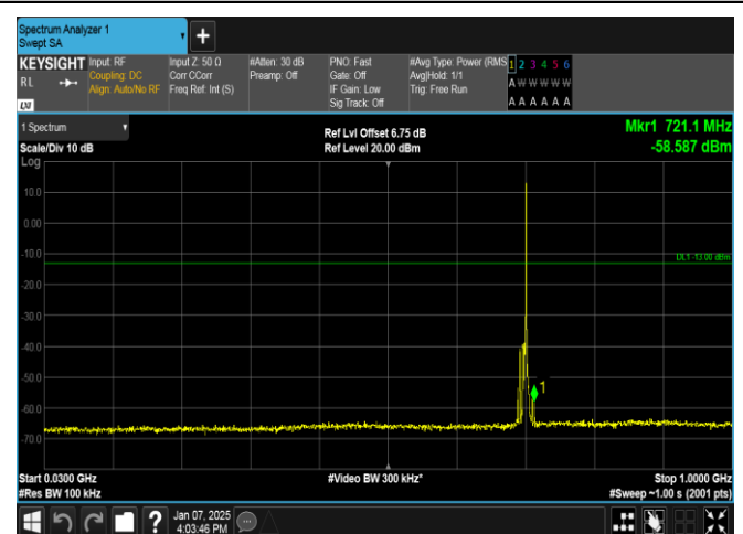
Band12-5MHz-16QAM-23095-1RB#24-30~1000-PASS
