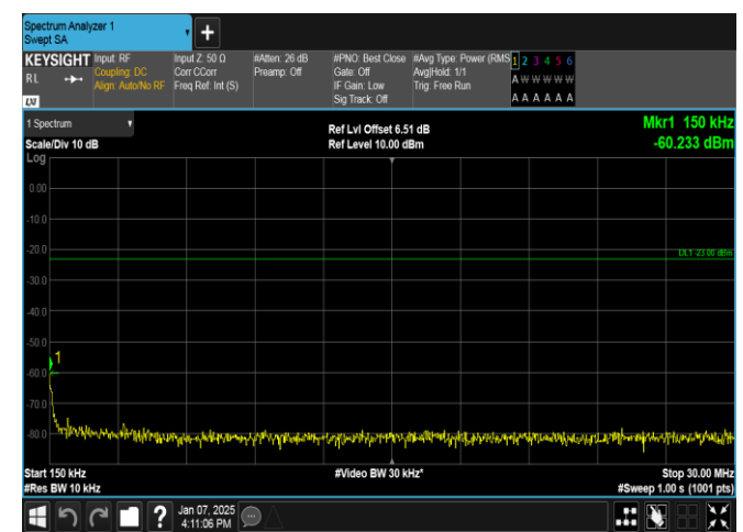
Band12-5MHz-QPSK-23155-25RB#0-0.15~30-PASS
