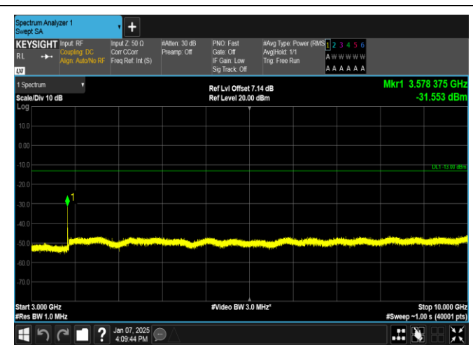
Band12-5MHz-QPSK-23155-1RB#24-3000~10000-PASS
