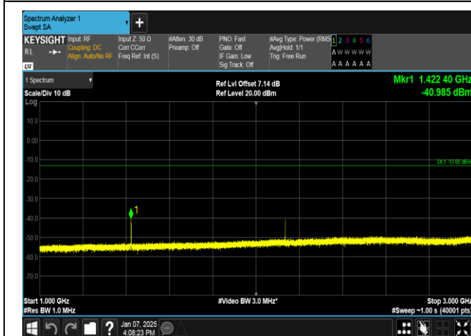
Band12-5MHz-16QAM-23155-1RB#0-1000~3000-PASS
