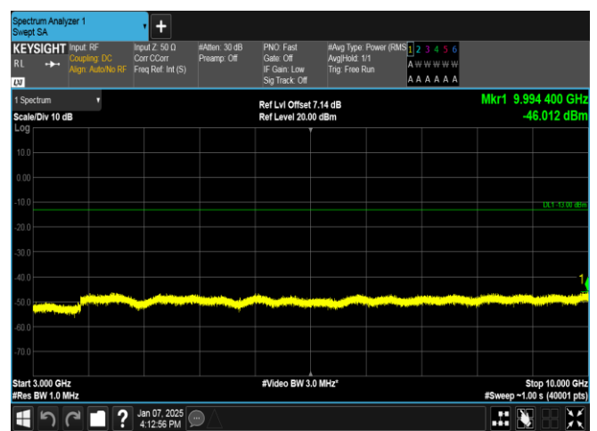
Band12-5MHz-16QAM-23155-25RB#0-3000~10000-PASS
