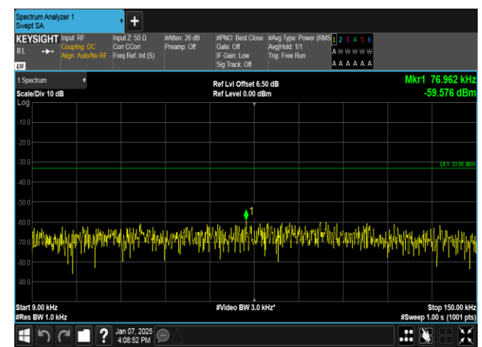
Band12-5MHz-QPSK-23155-1RB#24-0.009~0.15-PASS
