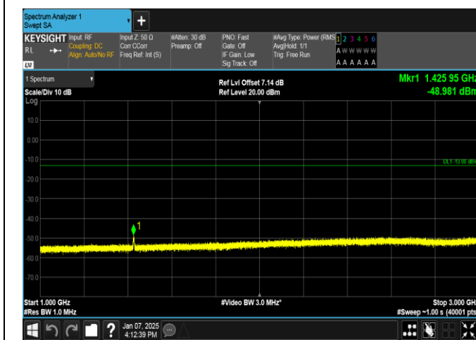
Band12-5MHz-16QAM-23155-25RB#0-1000~3000-PASS
