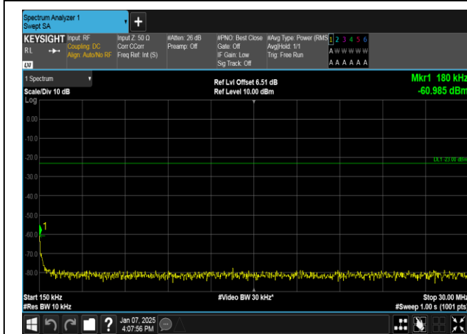
Band12-5MHz-16QAM-23155-1RB#0-0.15~30-PASS
