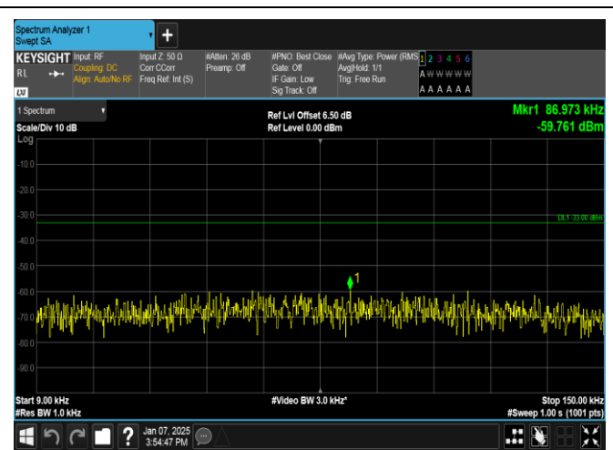
Band12-5MHz-16QAM-23035-1RB#0-0.009~0.15-PASS
