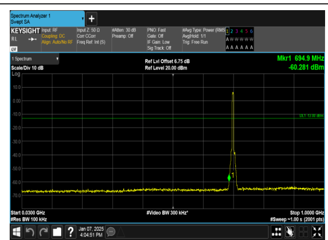
Band12-5MHz-QPSK-23095-25RB#0-30~1000-PASS
