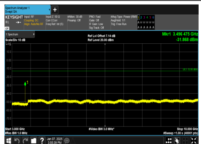
Band12-5MHz-16QAM-23035-1RB#0-3000~10000-PASS
