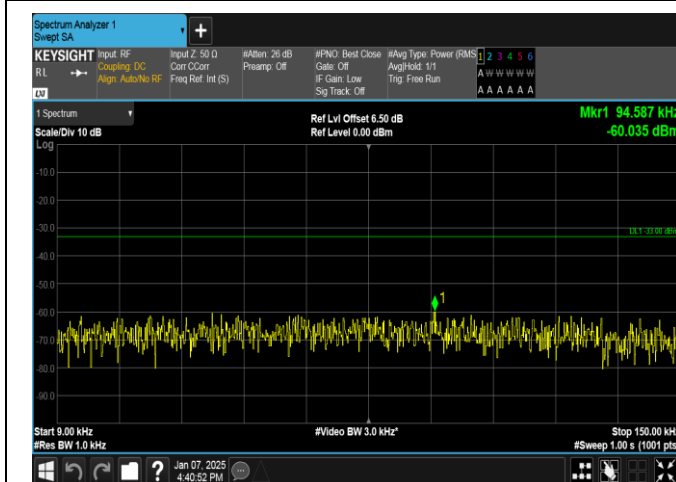
Band12-10MHz-QPSK-23060-1RB#0-0.009~0.15-PASS
