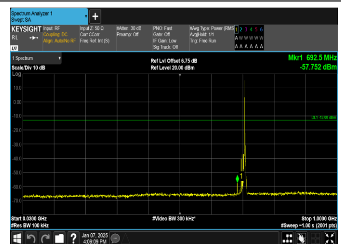
Band12-5MHz-QPSK-23155-1RB#24-30~1000-PASS
