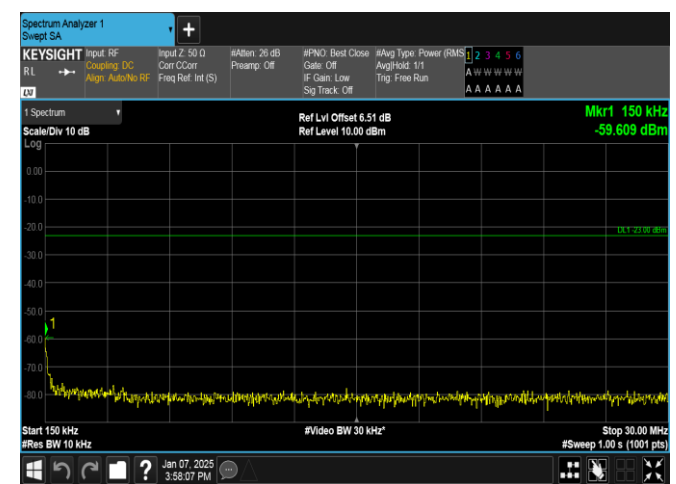
Band12-5MHz-QPSK-23035-25RB#0-0.15~30-PASS
