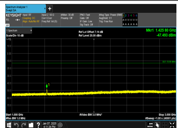
Band12-5MHz-QPSK-23155-25RB#0-1000~3000-PASS
