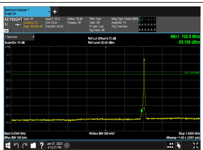
Band12-5MHz-16QAM-23155-25RB#0-30~1000-PASS
