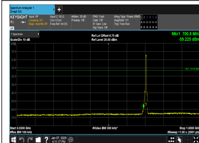
Band12-5MHz-QPSK-23155-25RB#0-30~1000-PASS
