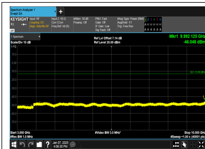
Band12-5MHz-16QAM-23095-25RB#0-3000~10000-PASS
