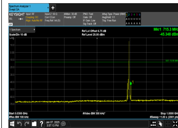
Band12-5MHz-16QAM-23035-1RB#24-30~1000-PASS
