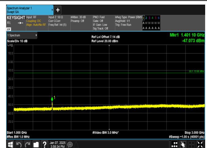
Band12-5MHz-QPSK-23035-25RB#0-1000~3000-PASS
