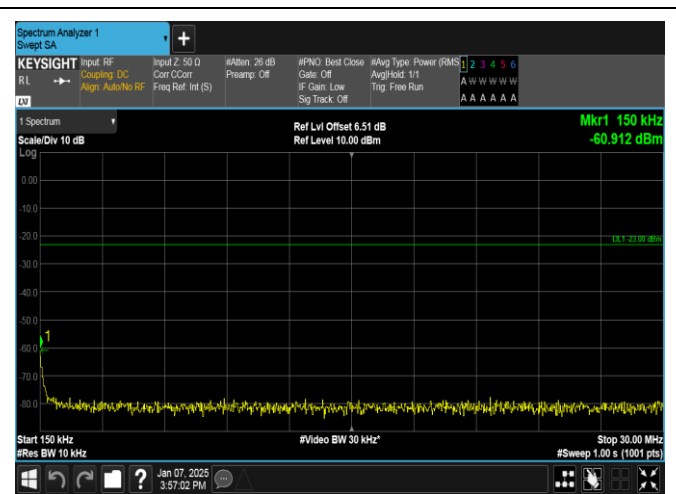
Band12-5MHz-16QAM-23035-1RB#24-0.15~30-PASS
