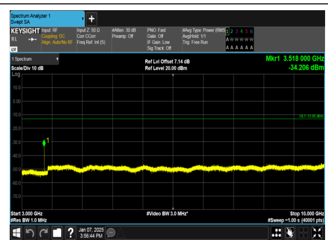
Band12-5MHz-QPSK-23035-1RB#24-3000~10000-PASS
