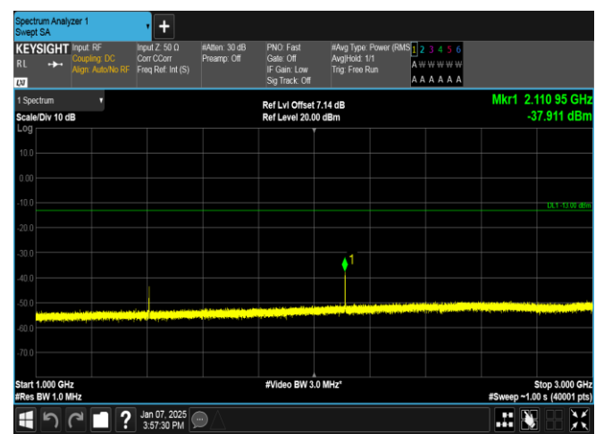
Band12-5MHz-16QAM-23035-1RB#24-1000~3000-PASS
