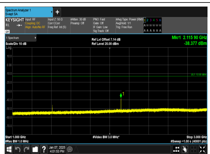
Band12-5MHz-16QAM-23095-1RB#0-1000~3000-PASS
