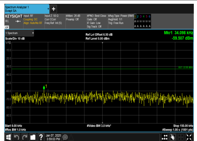
Band12-5MHz-16QAM-23035-25RB#0-0.009~0.15-PASS
