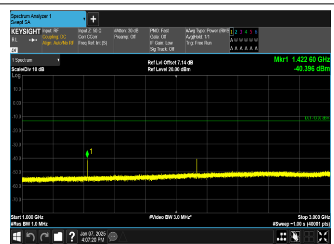
Band12-5MHz-QPSK-23155-1RB#0-1000~3000-PASS
