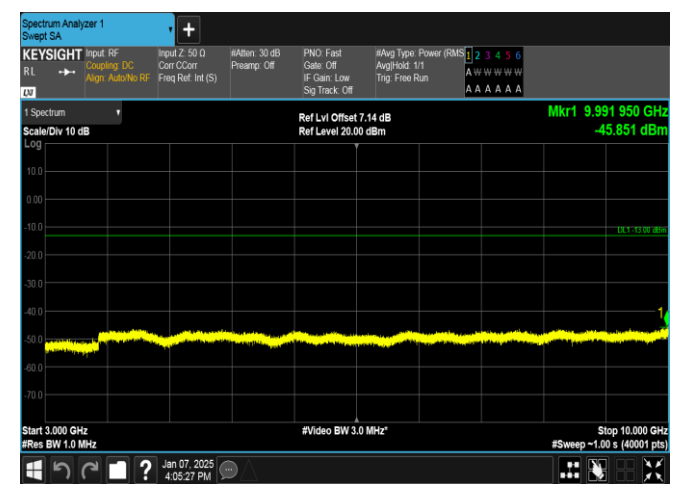
Band12-5MHz-QPSK-23095-25RB#0-3000~10000-PASS
