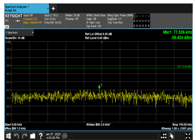
Band12-5MHz-16QAM-23095-1RB#24-0.009~0.15-PASS
