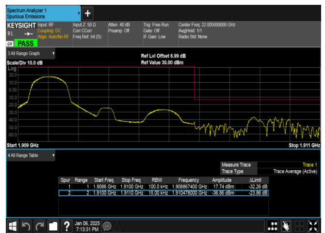
Band2-1.4MHz-16QAM-19193-1RB#0-PASS
