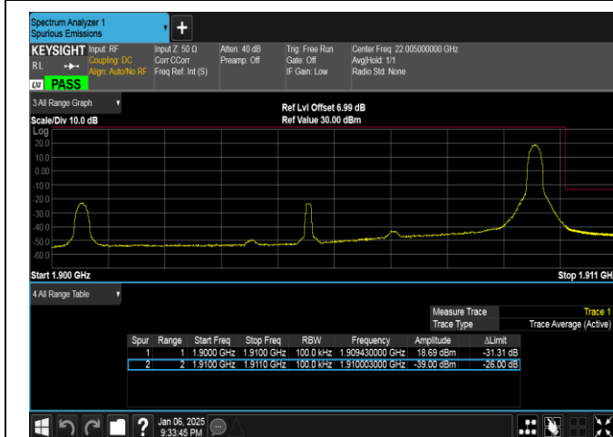
Band2-10MHz-QPSK-19150-1RB#49-PASS
