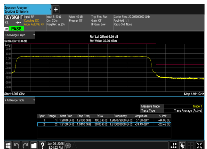
Band2-3MHz-QPSK-19185-15RB#0-PASS
