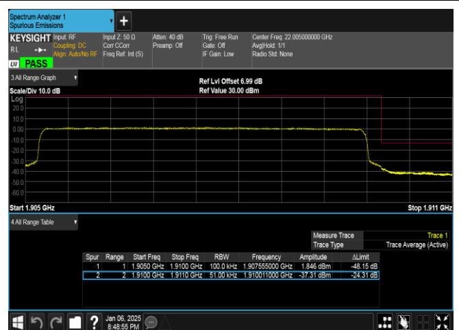
Band2-5MHz-16QAM-19175-25RB#0-PASS
