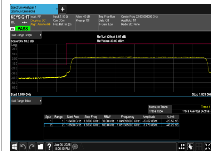
Band2-3MHz-16QAM-18615-15RB#0-PASS
