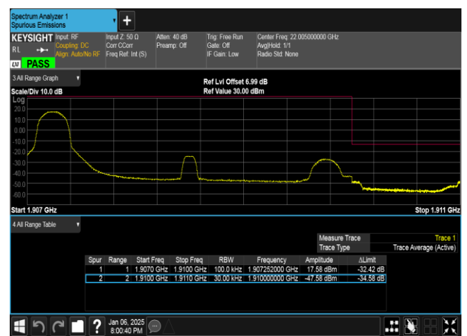
Band2-3MHz-16QAM-19185-1RB#0-PASS
