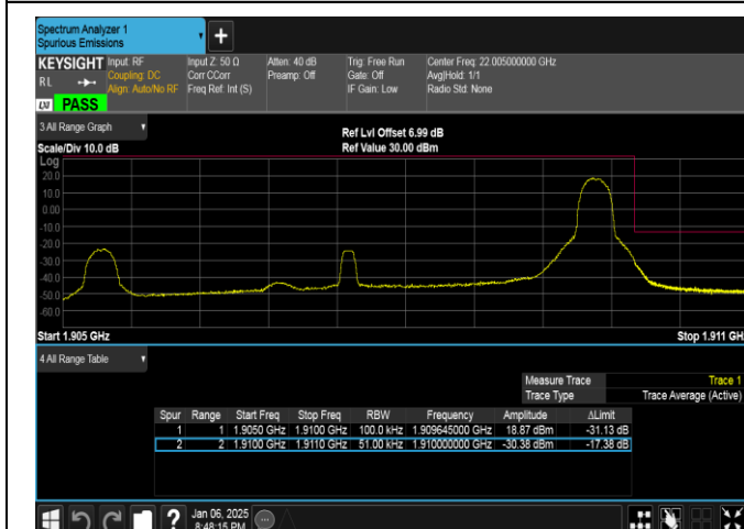
Band2-5MHz-QPSK-19175-1RB#24-PASS
