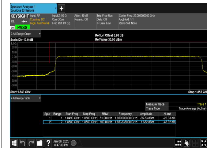
Band2-5MHz-16QAM-18625-25RB#0-PASS
