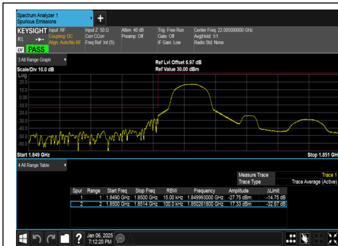
Band2-1.4MHz-16QAM-18607-1RB#0-PASS
