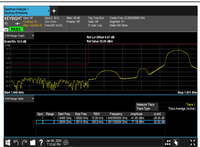
Band2-1.4MHz-16QAM-18607-1RB#5-PASS
