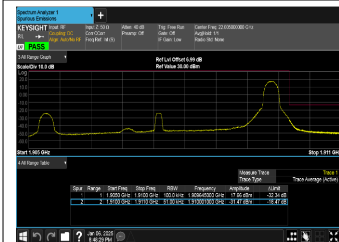
Band2-5MHz-16QAM-19175-1RB#24-PASS
