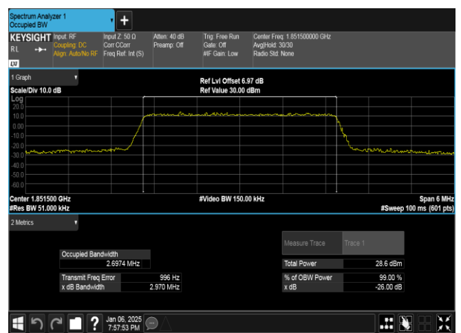
Band2-3MHz-16QAM-18615-15RB#0-PASS
