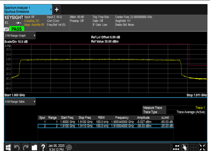
Band2-10MHz-QPSK-19150-50RB#0-PASS
