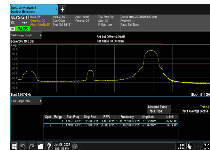
Band2-3MHz-16QAM-19185-1RB#14-PASS
