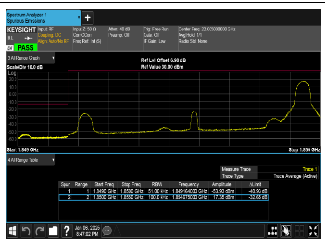
Band2-5MHz-16QAM-18625-1RB#24-PASS
