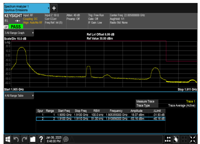
Band2-5MHz-16QAM-19175-1RB#0-PASS
