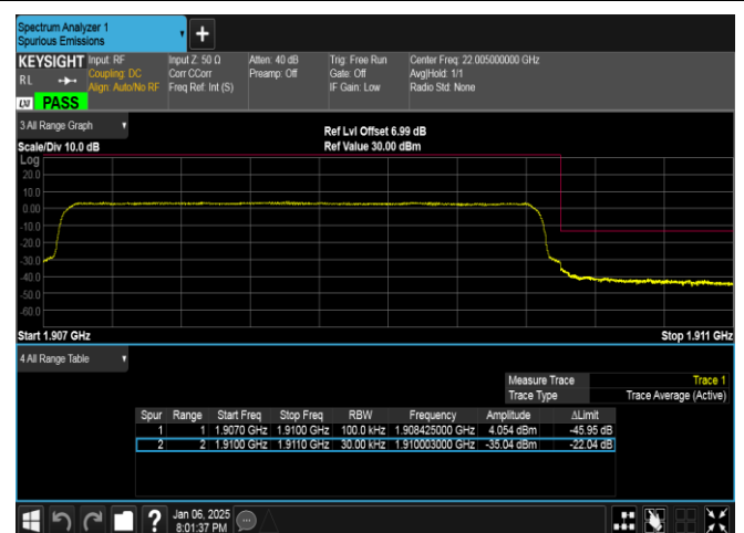
Band2-3MHz-16QAM-19185-15RB#0-PASS
