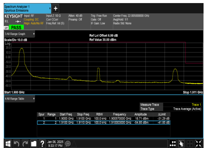
Band2-10MHz-QPSK-19150-1RB#0-PASS
