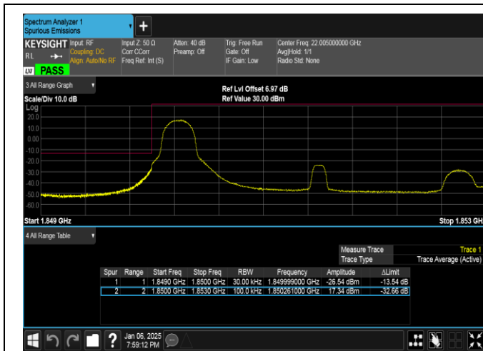
Band2-3MHz-16QAM-18615-1RB#0-PASS
