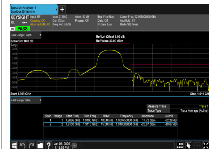
Band2-1.4MHz-16QAM-19193-1RB#5-PASS
