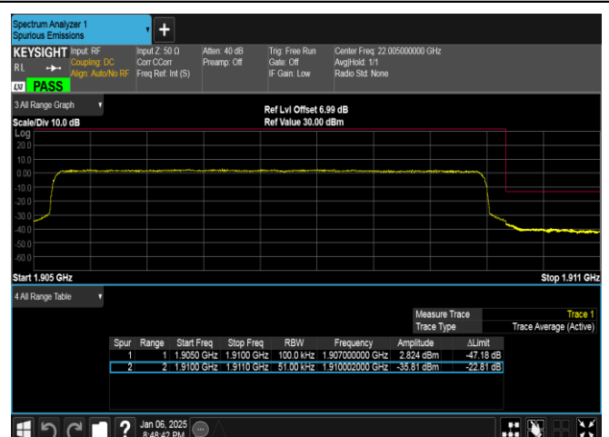
Band2-5MHz-QPSK-19175-25RB#0-PASS
