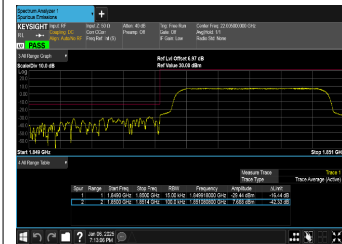
Band2-1.4MHz-16QAM-18607-6RB#0-PASS
