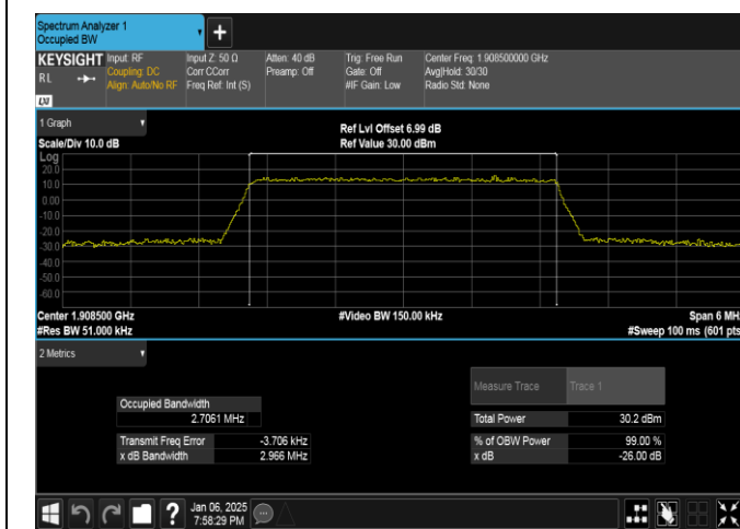
Band2-3MHz-QPSK-19185-15RB#0-PASS
