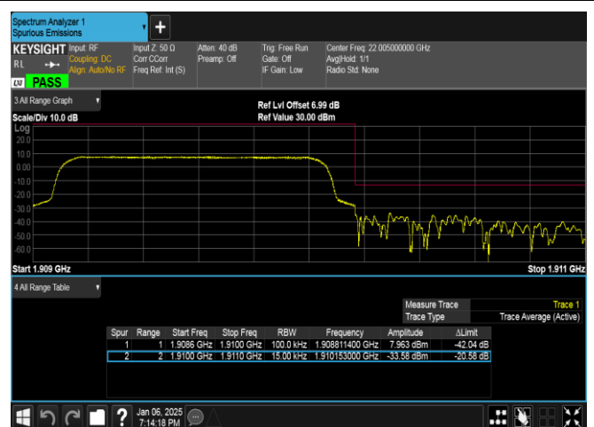
Band2-1.4MHz-16QAM-19193-6RB#0-PASS
