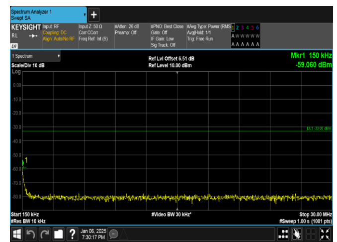
Band2-1.4MHz-16QAM-19193-1RB#5-0.15~30-PASS
