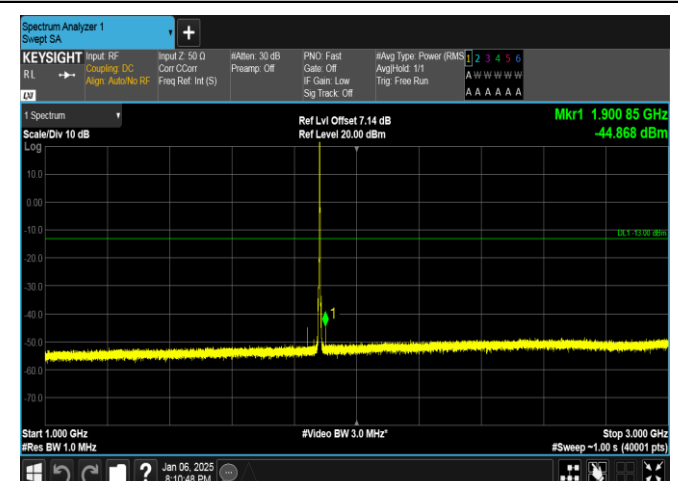
Band2-3MHz-QPSK-18900-1RB#14-1000~3000-PASS
