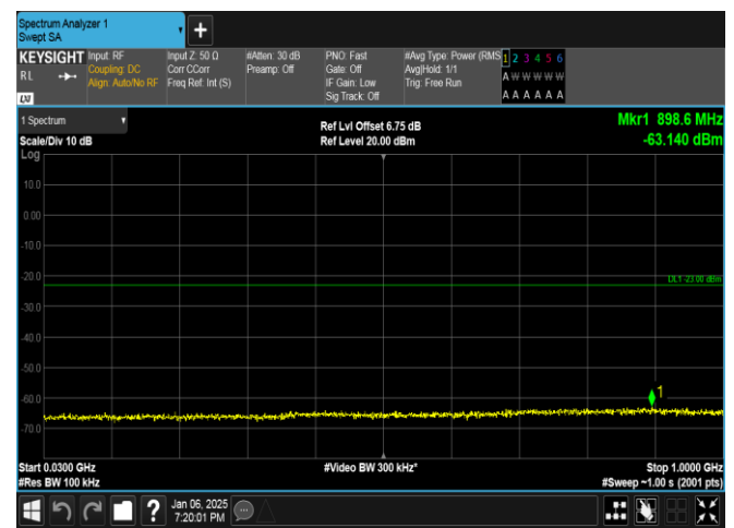
Band2-1.4MHz-16QAM-18607-6RB#0-30~1000-PASS
