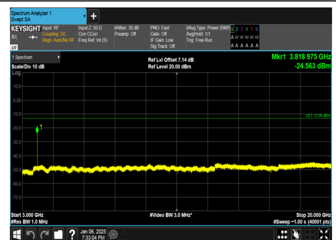
Band2-1.4MHz-16QAM-19193-6RB#0-3000~20000-PASS
