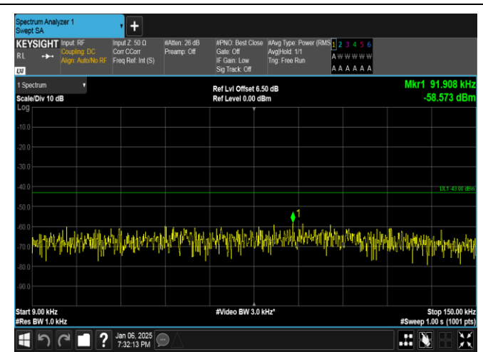
Band2-1.4MHz-16QAM-19193-6RB#0-0.009~0.15-PASS
