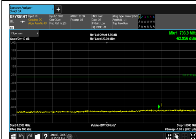
Band2-3MHz-QPSK-18900-1RB#14-30~1000-PASS
