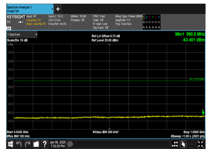
Band2-1.4MHz-16QAM-19193-6RB#0-30~1000-PASS
