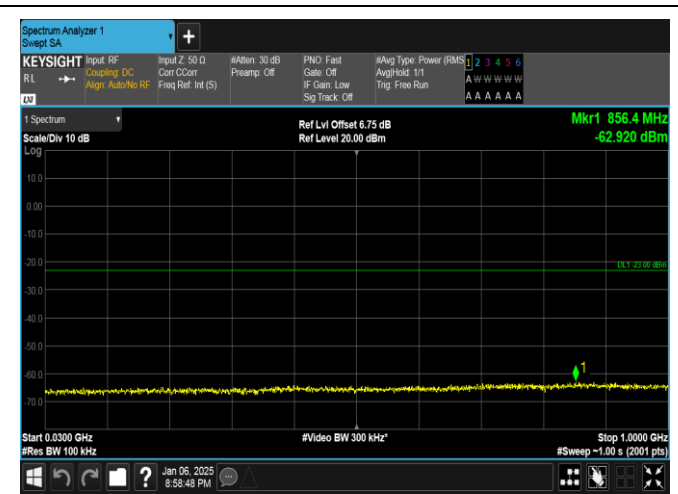
Band2-5MHz-16QAM-18900-1RB#24-30~1000-PASS
