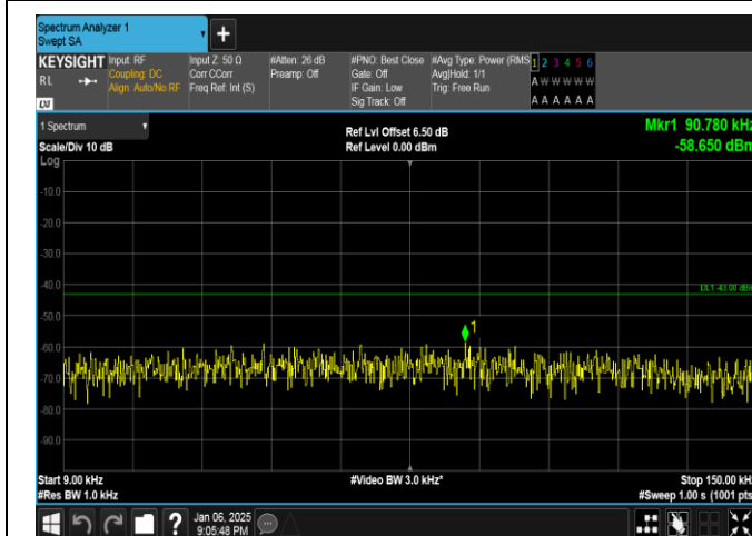
Band2-5MHz-QPSK-19175-25RB#0-0.009~0.15-PASS
