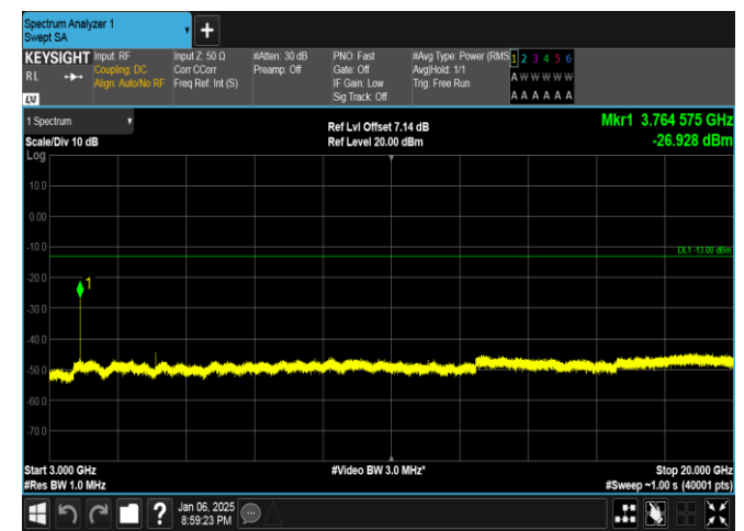
Band2-5MHz-16QAM-18900-1RB#24-3000~20000-PASS
