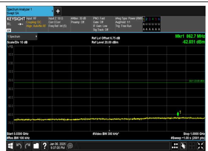
Band2-10MHz-QPSK-18650-1RB#49-30~1000-PASS
