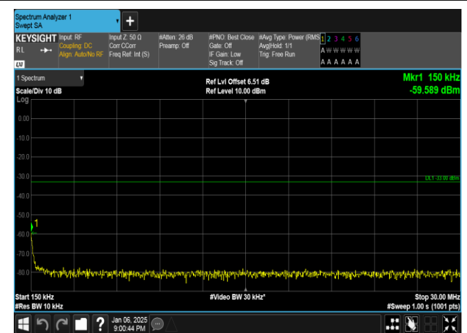
Band2-5MHz-16QAM-18900-25RB#0-0.15~30-PASS
