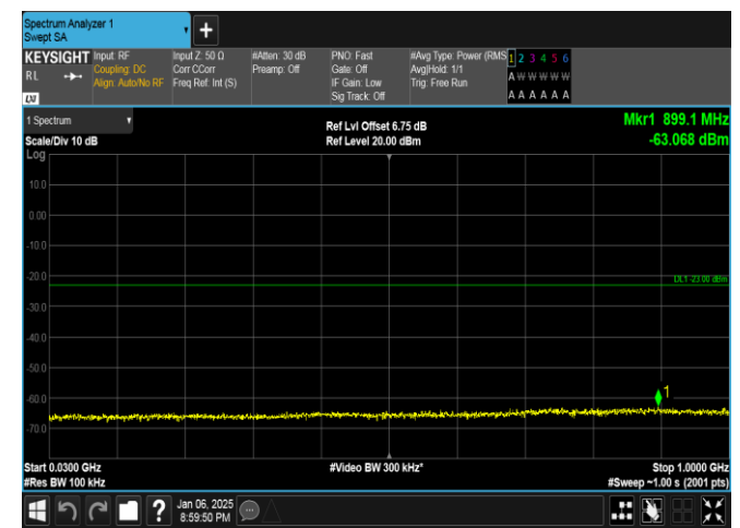
Band2-5MHz-QPSK-18900-25RB#0-30~1000-PASS
