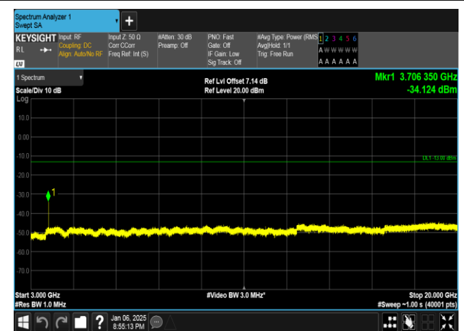
Band2-5MHz-16QAM-18625-25RB#0-3000~20000-PASS
