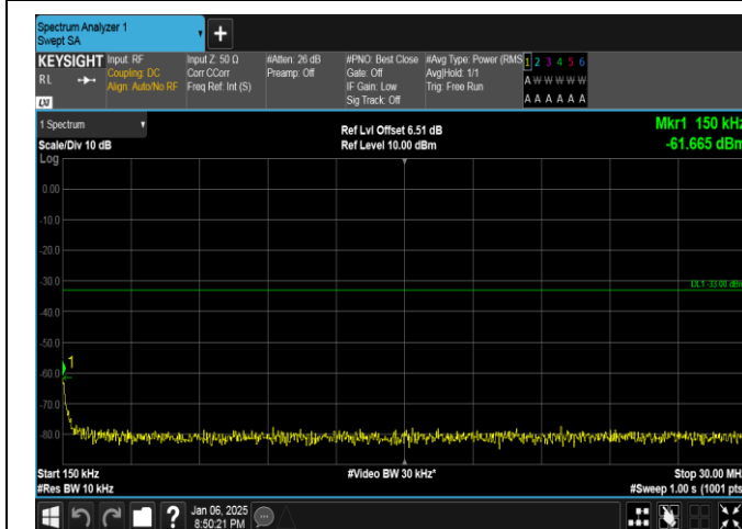
Band2-5MHz-16QAM-18625-1RB#0-0.15~30-PASS
