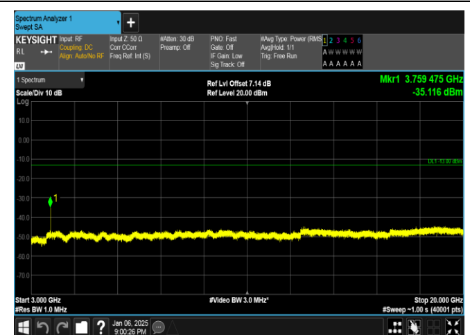
Band2-5MHz-QPSK-18900-25RB#0-3000~20000-PASS
