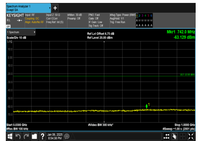
Band2-5MHz-16QAM-18625-25RB#0-30~1000-PASS
