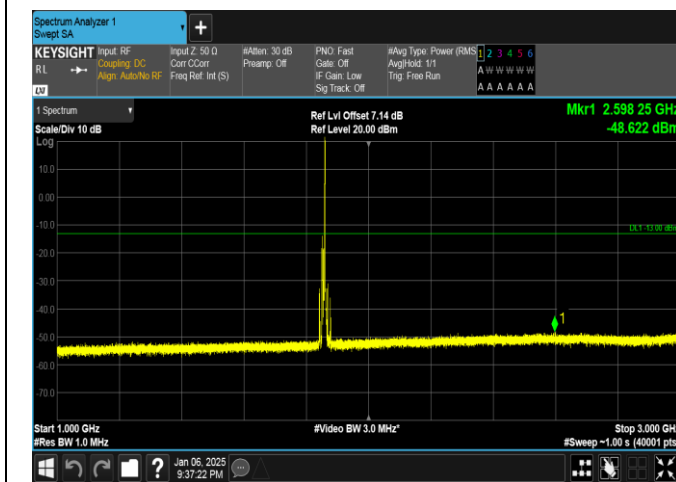
Band2-10MHz-QPSK-18650-1RB#49-1000~3000-PASS
