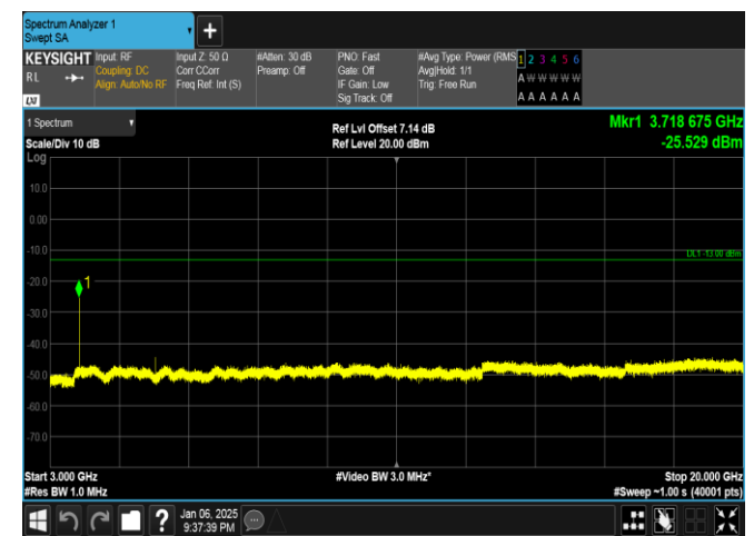
Band2-10MHz-QPSK-18650-1RB#49-3000~20000-PASS
