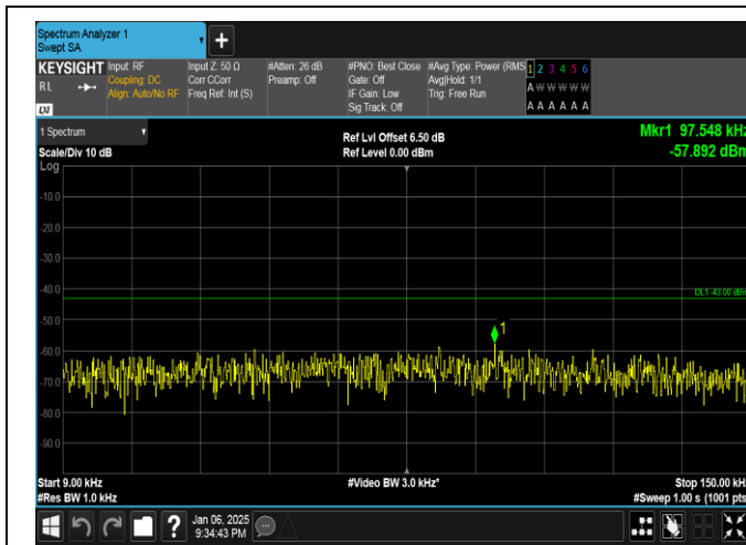
Band2-10MHz-QPSK-18650-1RB#0-0.009~0.15-PASS
