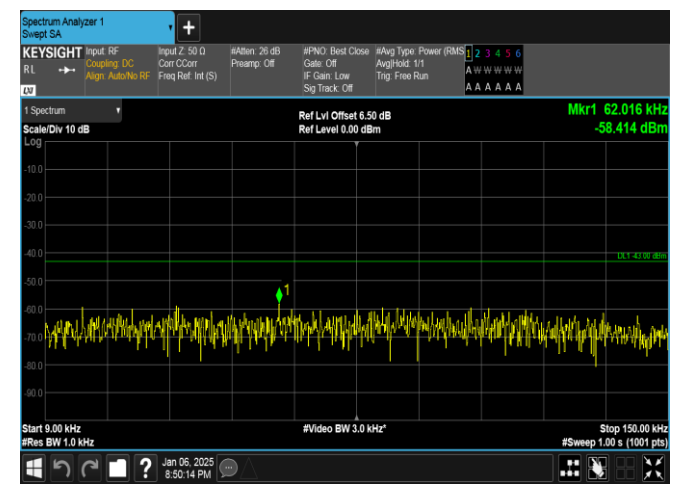
Band2-5MHz-16QAM-18625-1RB#0-0.009~0.15-PASS
