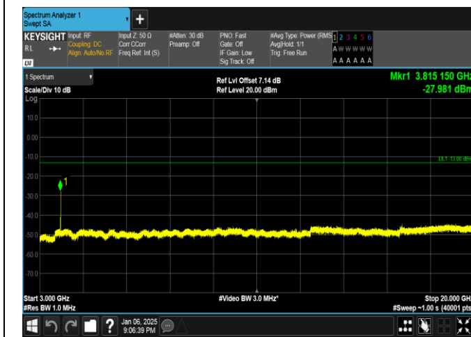
Band2-5MHz-QPSK-19175-25RB#0-3000~20000-PASS
