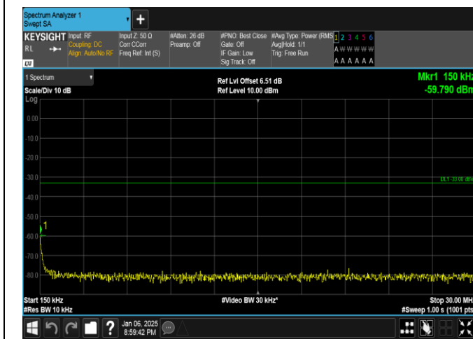
Band2-5MHz-QPSK-18900-25RB#0-0.15~30-PASS
