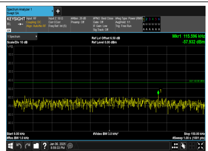
Band2-5MHz-QPSK-18900-25RB#0-0.009~0.15-PASS
