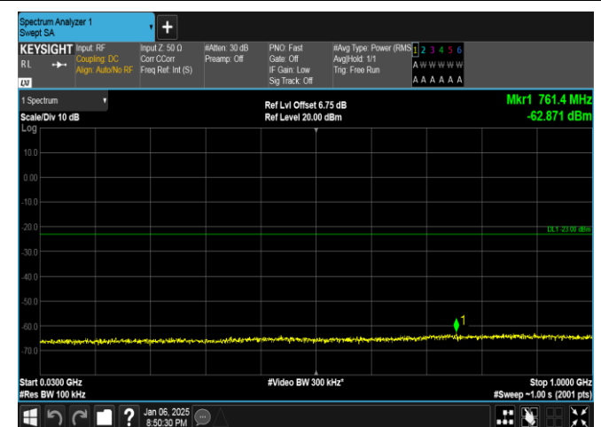
Band2-5MHz-16QAM-18625-1RB#0-30~1000-PASS
