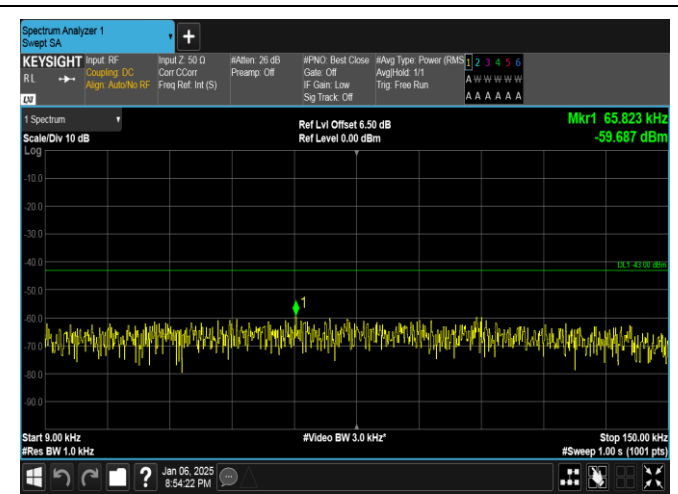
Band2-5MHz-16QAM-18625-25RB#0-0.009~0.15-PASS
