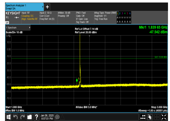
Band2-5MHz-16QAM-18900-1RB#0-1000~3000-PASS
