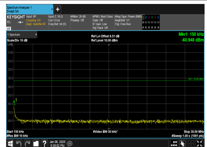
Band2-10MHz-QPSK-18650-50RB#0-0.15~30-PASS
