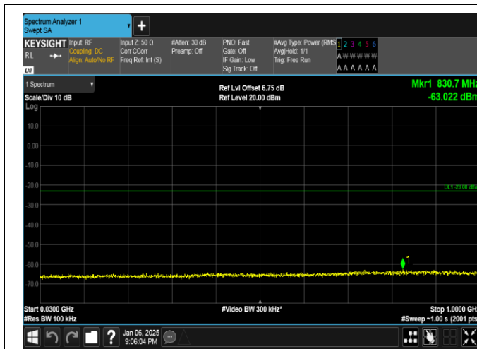
Band2-5MHz-QPSK-19175-25RB#0-30~1000-PASS
