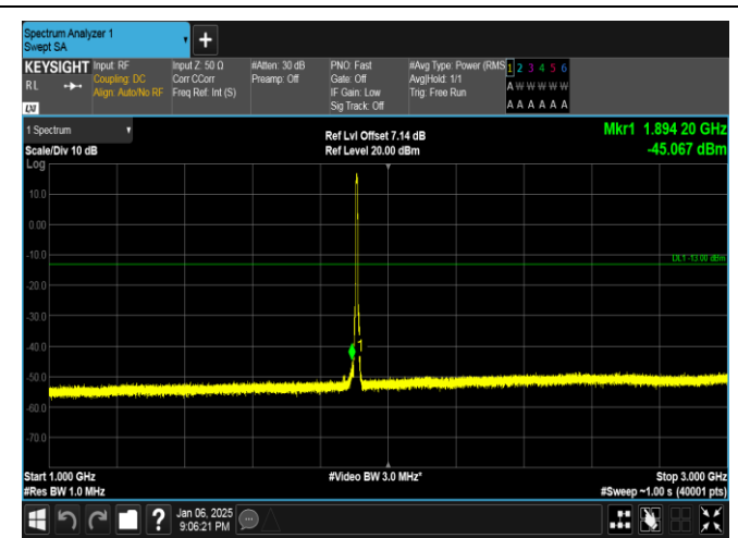
Band2-5MHz-QPSK-19175-25RB#0-1000~3000-PASS
