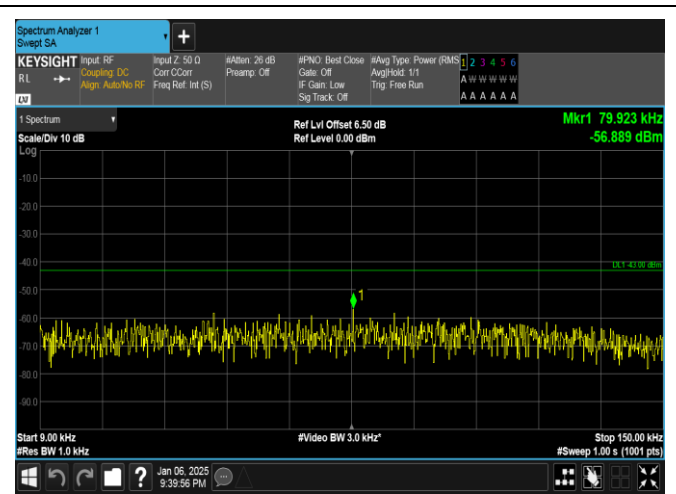
Band2-10MHz-16QAM-18650-50RB#0-0.009~0.15-PASS
