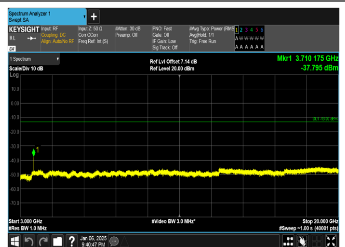
Band2-10MHz-16QAM-18650-50RB#0-3000~20000-PASS
