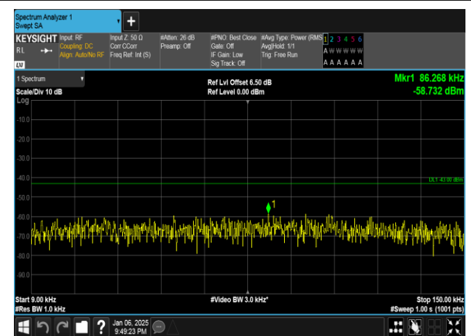
Band2-10MHz-QPSK-19150-1RB#49-0.009~0.15-PASS
