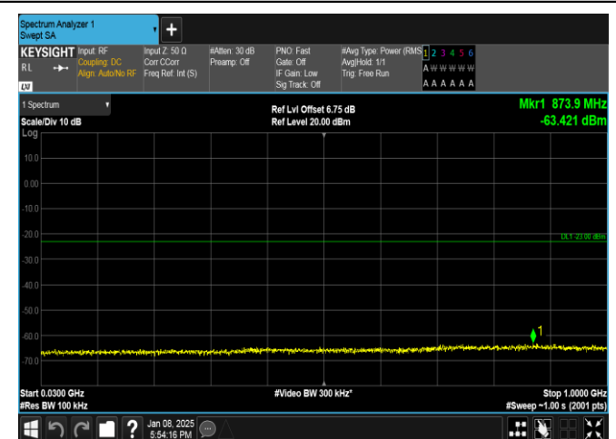
Band25-3MHz-16QAM-26675-1RB#0-30~1000-PASS
