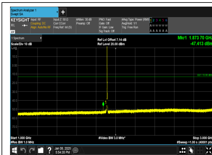
Band25-3MHz-16QAM-26675-1RB#0-1000~3000-PASS
