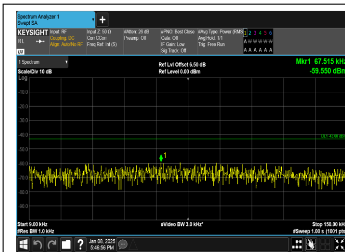
Band25-3MHz-16QAM-26365-1RB#0-0.009~0.15-PASS
