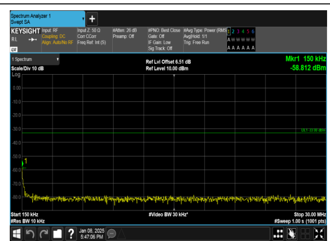
Band25-3MHz-16QAM-26365-1RB#0-0.15~30-PASS
