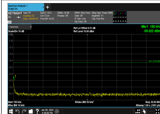
Band25-5MHz-QPSK-26365-1RB#0-0.15~30-PASS
