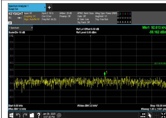
Band25-3MHz-QPSK-26675-15RB#0-0.009~0.15-PASS
