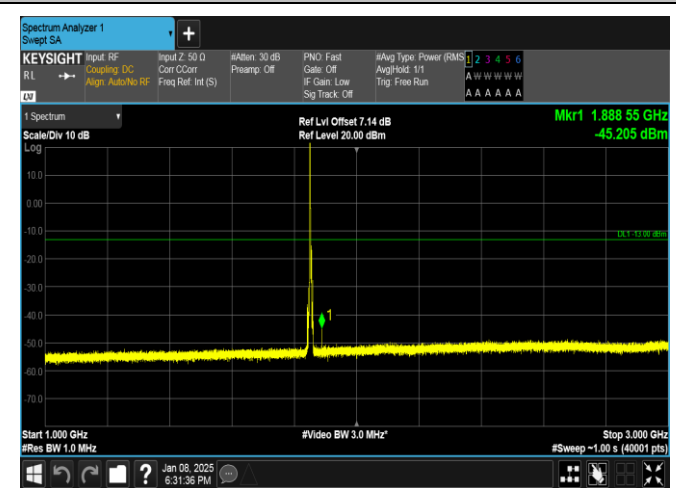
Band25-5MHz-QPSK-26065-1RB#0-1000~3000-PASS
