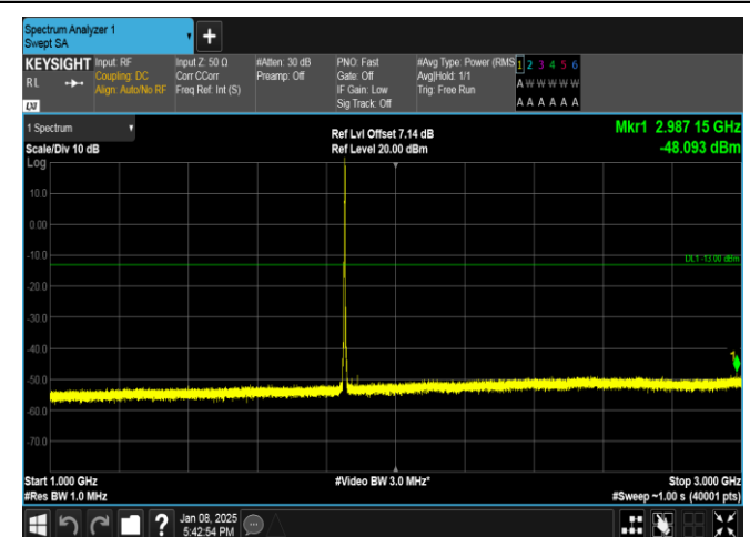
Band25-3MHz-16QAM-26055-1RB#14-1000~3000-PASS
