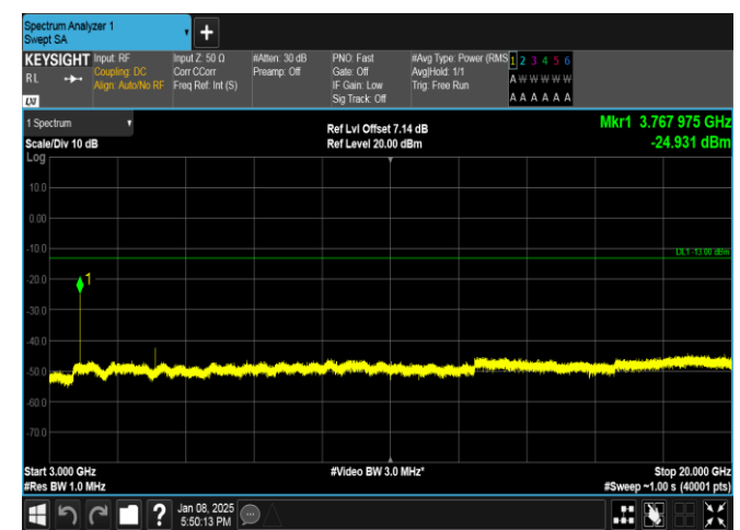
Band25-3MHz-16QAM-26365-1RB#14-3000~20000-PASS
