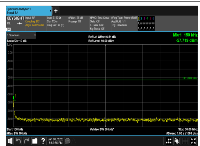
Band25-3MHz-QPSK-26675-1RB#0-0.15~30-PASS
