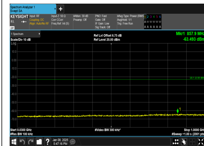
Band25-3MHz-16QAM-26365-1RB#0-30~1000-PASS
