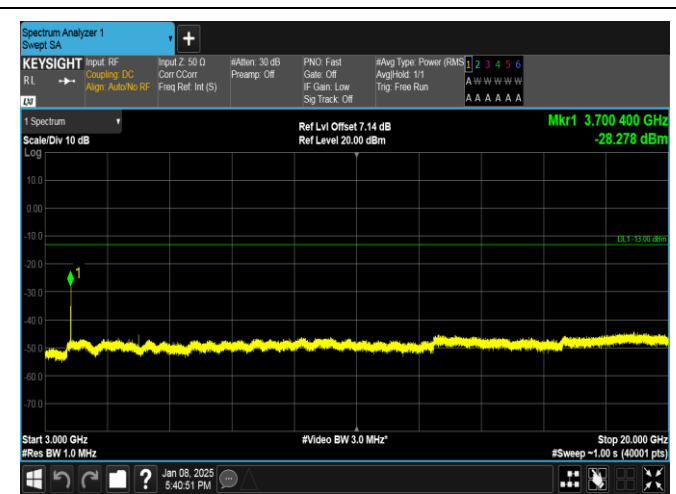
Band25-3MHz-16QAM-26055-1RB#0-3000~20000-PASS
