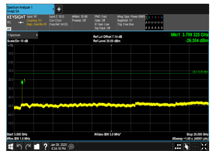
Band25-5MHz-QPSK-26065-1RB#24-3000~20000-PASS
