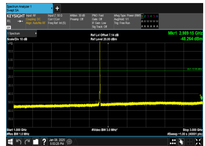
Band25-3MHz-QPSK-26675-1RB#0-1000~3000-PASS
