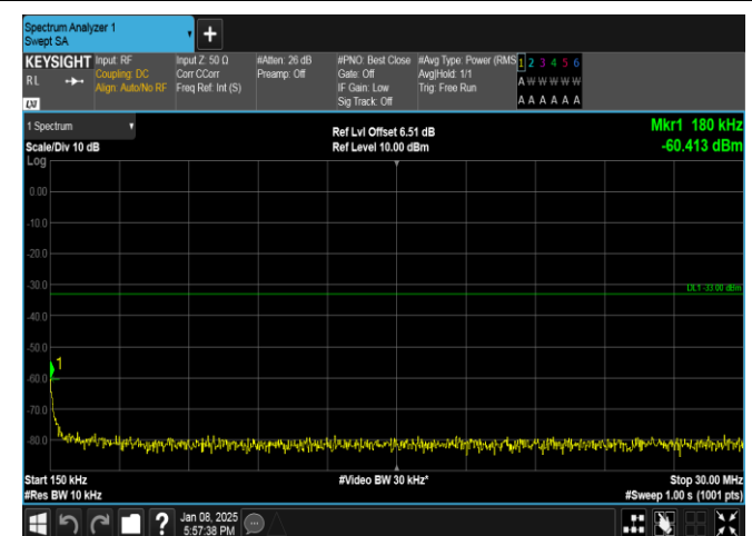
Band25-3MHz-QPSK-26675-15RB#0-0.15~30-PASS
