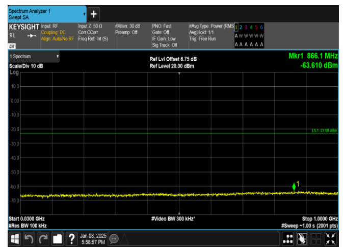
Band25-3MHz-16QAM-26675-15RB#0-30~1000-PASS
