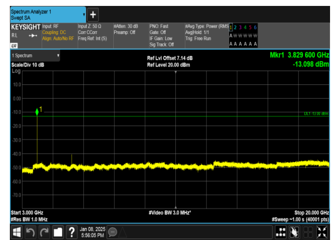
Band25-3MHz-QPSK-26675-1RB#14-3000~20000-PASS
