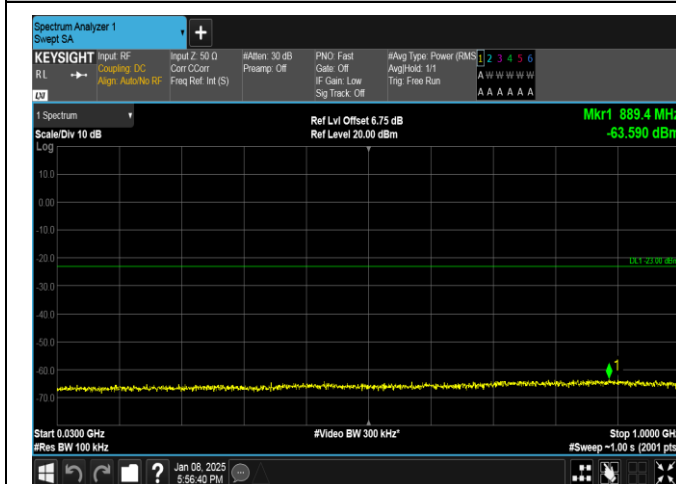
Band25-3MHz-16QAM-26675-1RB#14-30~1000-PASS
