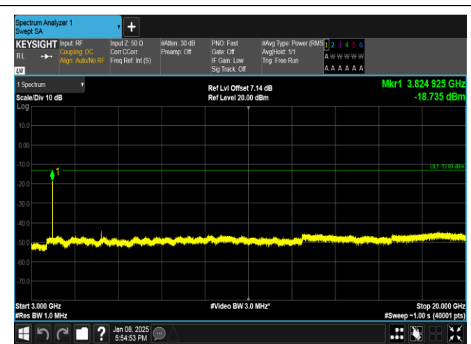
Band25-3MHz-16QAM-26675-1RB#0-3000~20000-PASS
