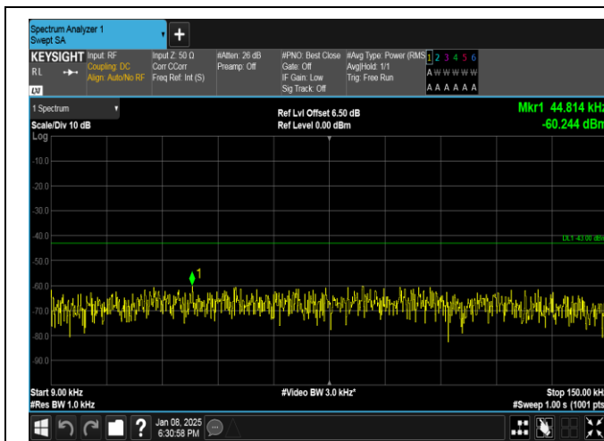
Band25-5MHz-QPSK-26065-1RB#0-0.009~0.15-PASS
