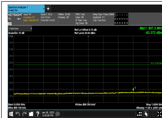
Band25-5MHz-QPSK-26065-25RB#0-30~1000-PASS
