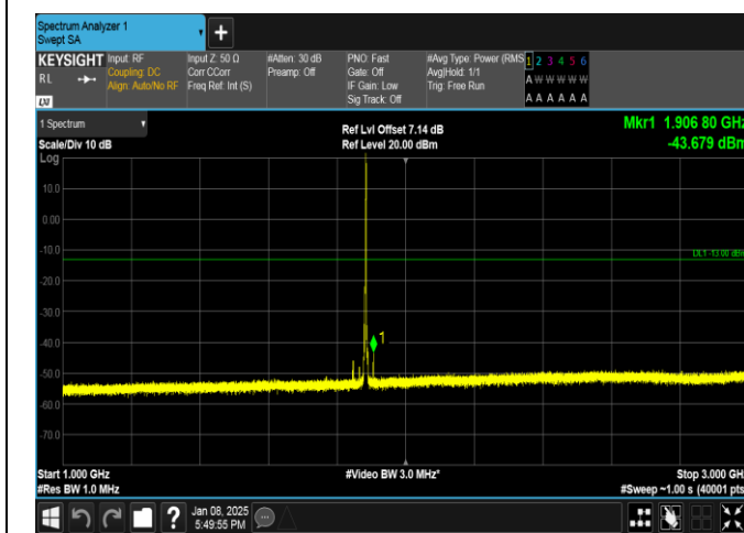
Band25-3MHz-16QAM-26365-1RB#14-1000~3000-PASS
