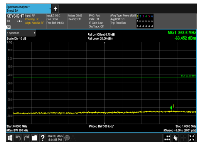
Band25-3MHz-16QAM-26055-15RB#0-30~1000-PASS
