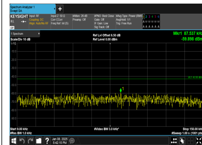
Band25-3MHz-16QAM-26055-1RB#14-0.009~0.15-PASS
