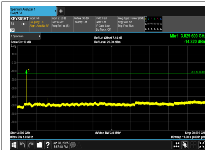
Band25-3MHz-16QAM-26675-1RB#14-3000~20000-PASS
