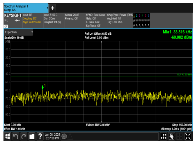
Band25-5MHz-QPSK-26365-1RB#0-0.009~0.15-PASS
