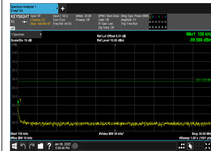
Band25-3MHz-16QAM-26675-15RB#0-0.15~30-PASS
