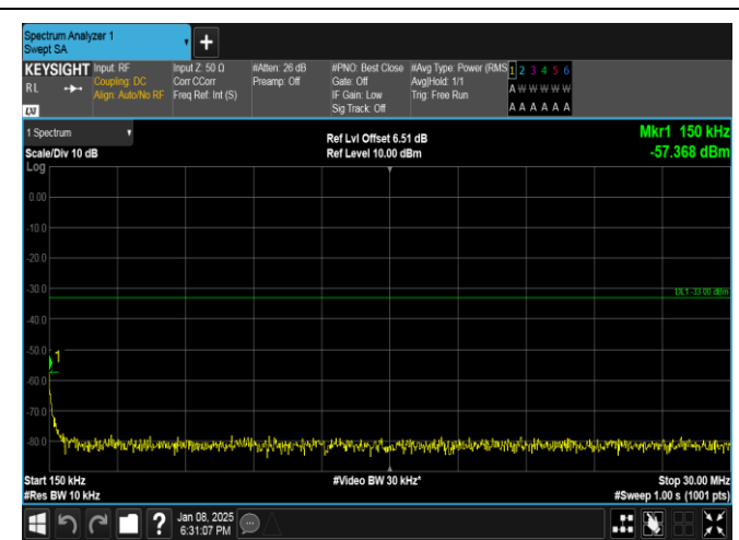
Band25-5MHz-QPSK-26065-1RB#0-0.15~30-PASS
