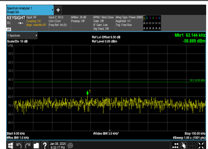
Band25-5MHz-QPSK-26065-1RB#24-0.009~0.15-PASS
