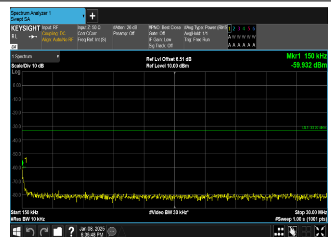
Band25-5MHz-QPSK-26065-25RB#0-0.15~30-PASS
