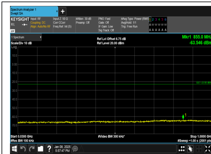
Band25-3MHz-QPSK-26675-15RB#0-30~1000-PASS
