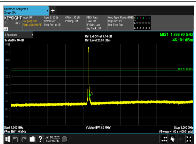
Band25-5MHz-QPSK-26065-25RB#0-1000~3000-PASS
