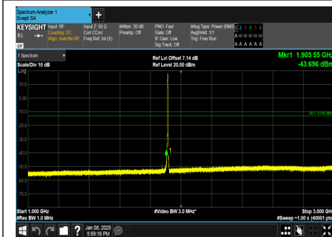
Band25-3MHz-16QAM-26675-15RB#0-1000~3000-PASS
