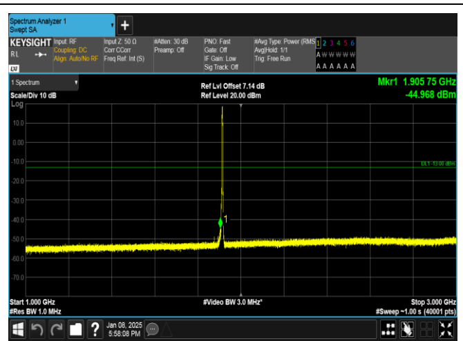
Band25-3MHz-QPSK-26675-15RB#0-1000~3000-PASS
