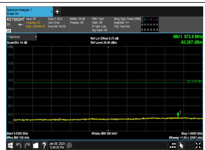
Band25-3MHz-16QAM-26365-1RB#14-30~1000-PASS
