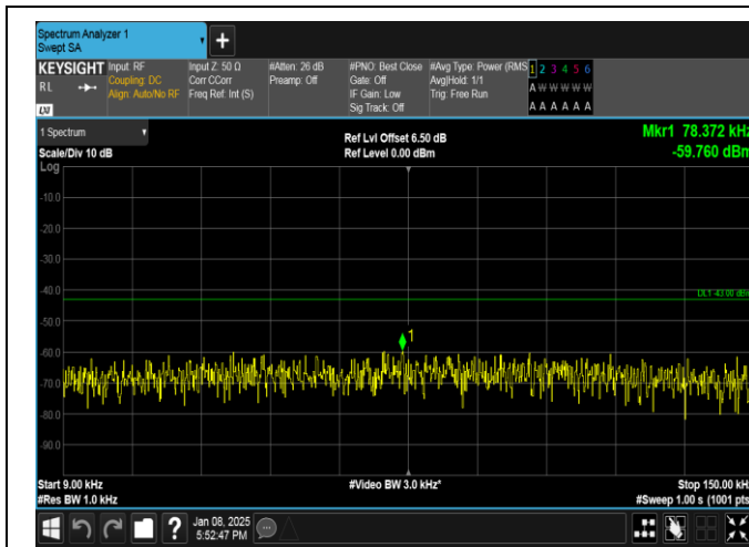
Band25-3MHz-QPSK-26675-1RB#0-0.009~0.15-PASS
