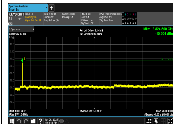
Band25-3MHz-QPSK-26675-1RB#0-3000~20000-PASS
