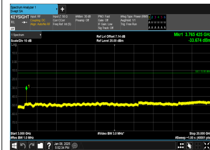
Band25-3MHz-16QAM-26365-15RB#0-3000~20000-PASS
