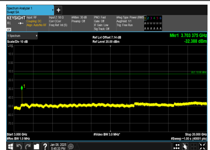
Band25-3MHz-16QAM-26055-15RB#0-3000~20000-PASS
