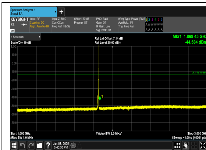
Band25-3MHz-16QAM-26055-1RB#0-1000~3000-PASS
