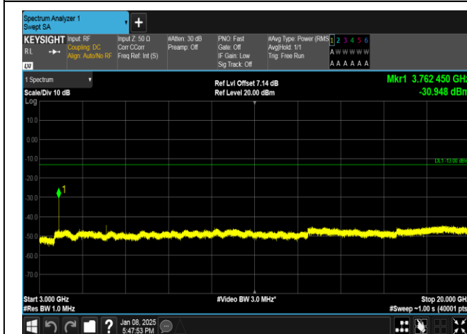
Band25-3MHz-16QAM-26365-1RB#0-3000~20000-PASS
