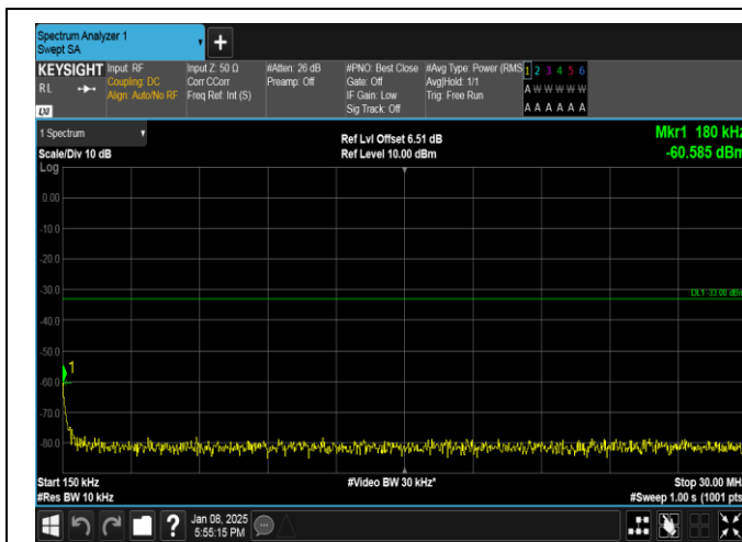
Band25-3MHz-QPSK-26675-1RB#14-0.15~30-PASS
