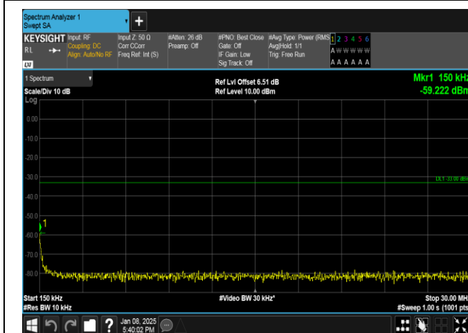
Band25-3MHz-16QAM-26055-1RB#0-0.15~30-PASS
