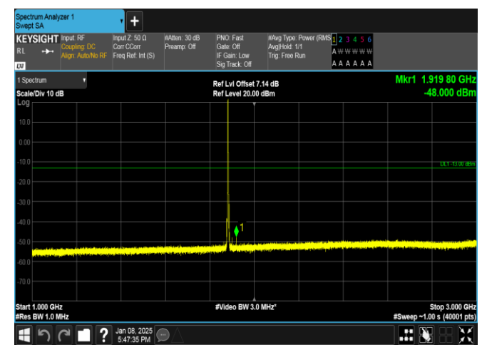
Band25-3MHz-16QAM-26365-1RB#0-1000~3000-PASS
