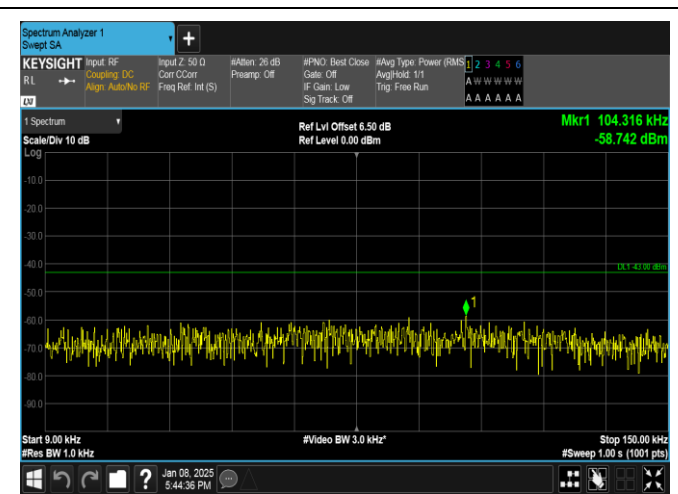
Band25-3MHz-16QAM-26055-15RB#0-0.009~0.15-PASS
