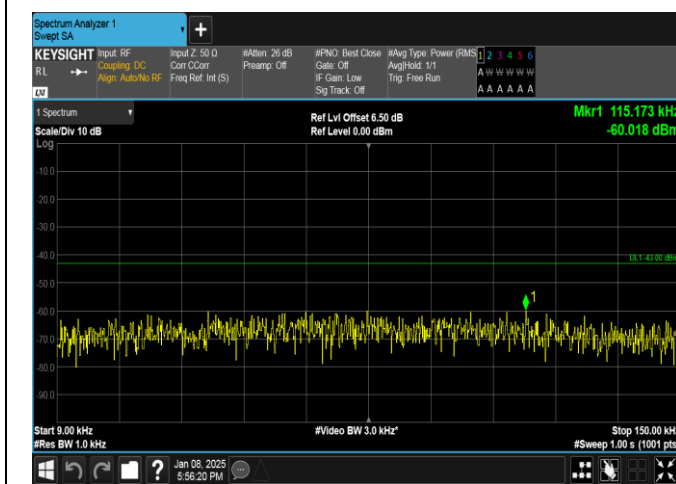
Band25-3MHz-16QAM-26675-1RB#14-0.009~0.15-PASS
