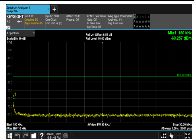
Band25-3MHz-16QAM-26365-15RB#0-0.15~30-PASS
