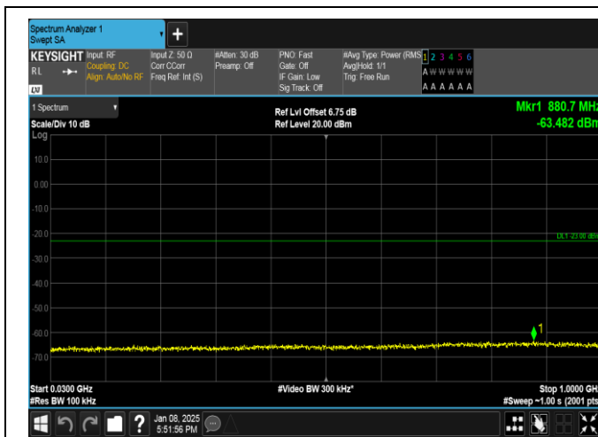
Band25-3MHz-16QAM-26365-15RB#0-30~1000-PASS
