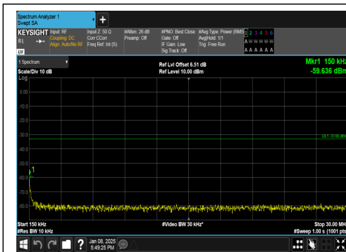
Band25-3MHz-16QAM-26365-1RB#14-0.15~30-PASS
