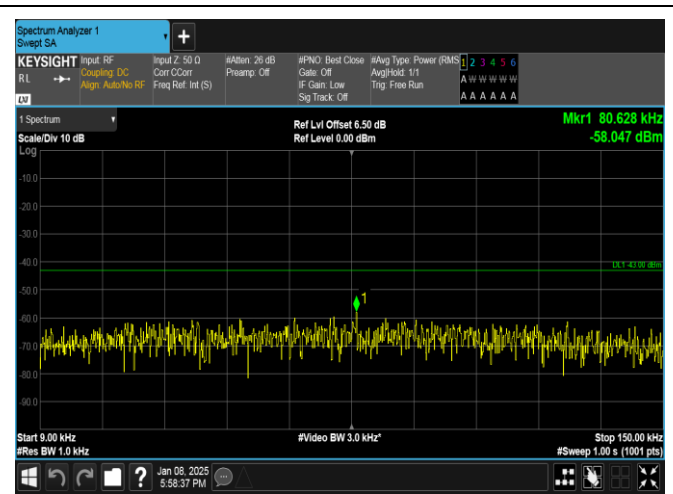
Band25-3MHz-16QAM-26675-15RB#0-0.009~0.15-PASS
