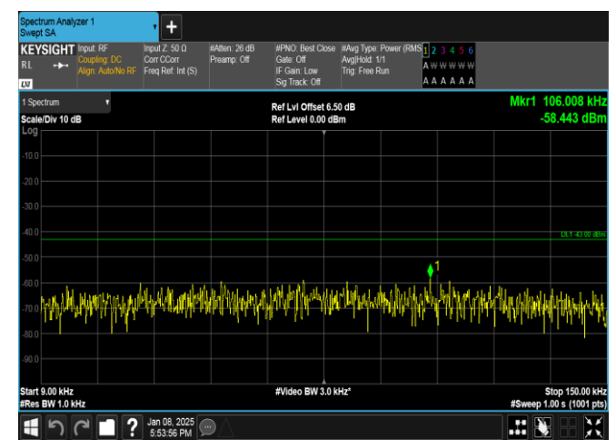
Band25-3MHz-16QAM-26675-1RB#0-0.009~0.15-PASS
