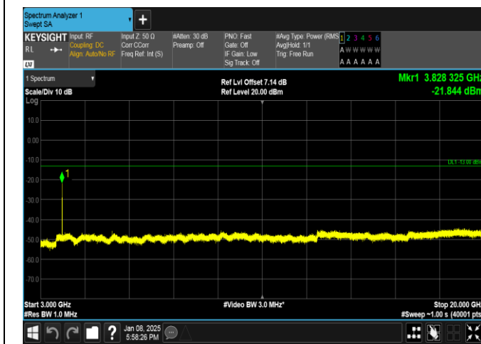
Band25-3MHz-QPSK-26675-15RB#0-3000~20000-PASS
