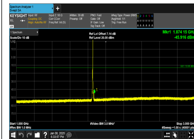
Band25-5MHz-QPSK-26065-1RB#24-1000~3000-PASS
