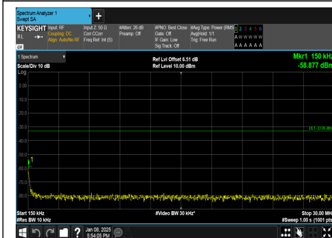
Band25-3MHz-16QAM-26675-1RB#0-0.15~30-PASS
