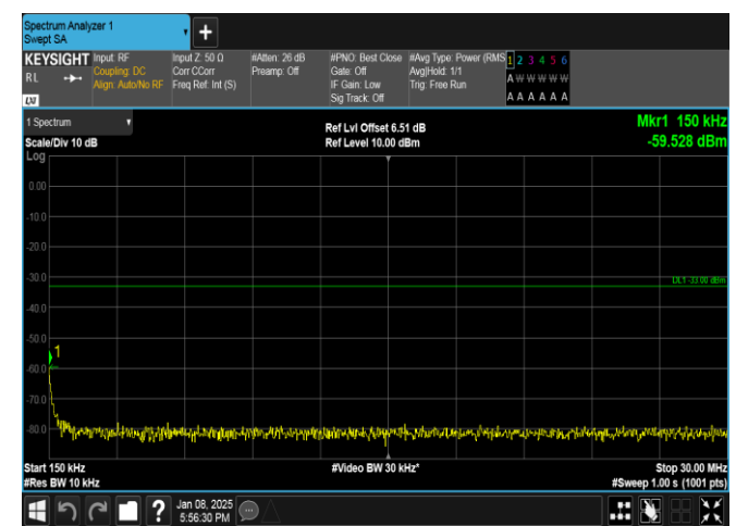
Band25-3MHz-16QAM-26675-1RB#14-0.15~30-PASS
