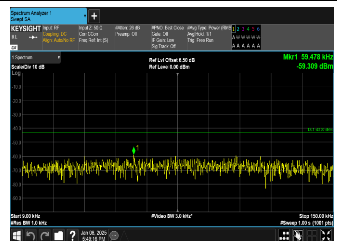
Band25-3MHz-16QAM-26365-1RB#14-0.009~0.15-PASS
