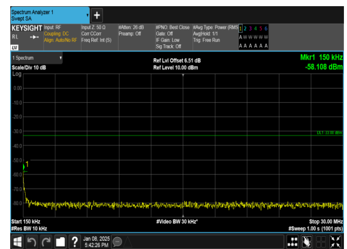
Band25-3MHz-16QAM-26055-1RB#14-0.15~30-PASS
