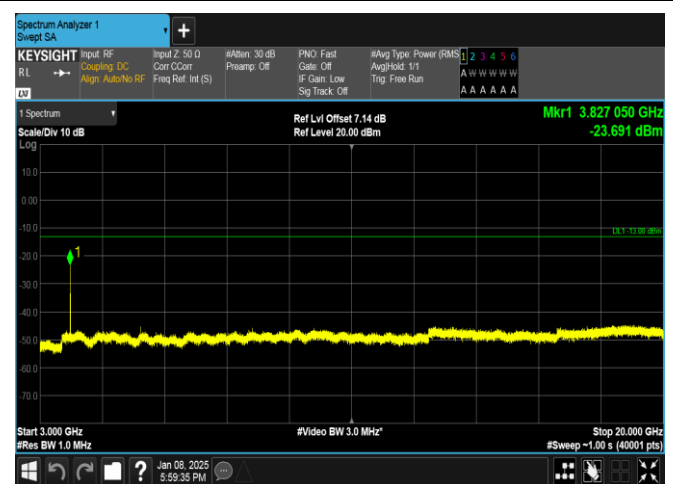
Band25-3MHz-16QAM-26675-15RB#0-3000~20000-PASS
