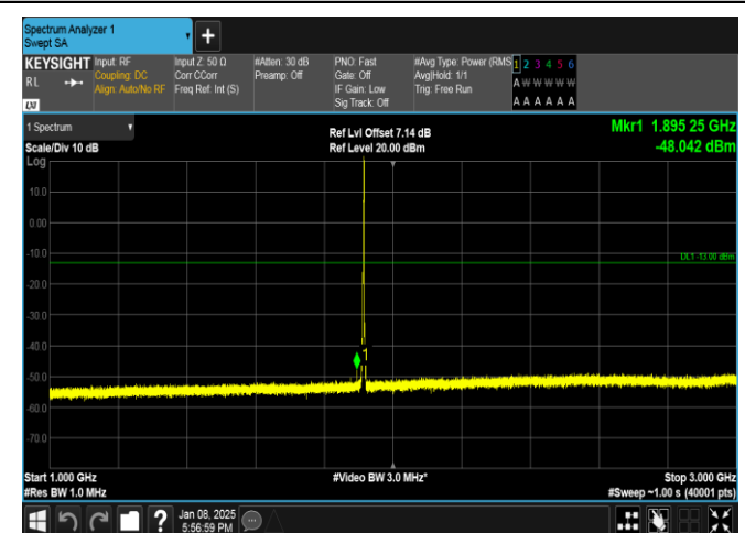
Band25-3MHz-16QAM-26675-1RB#14-1000~3000-PASS
