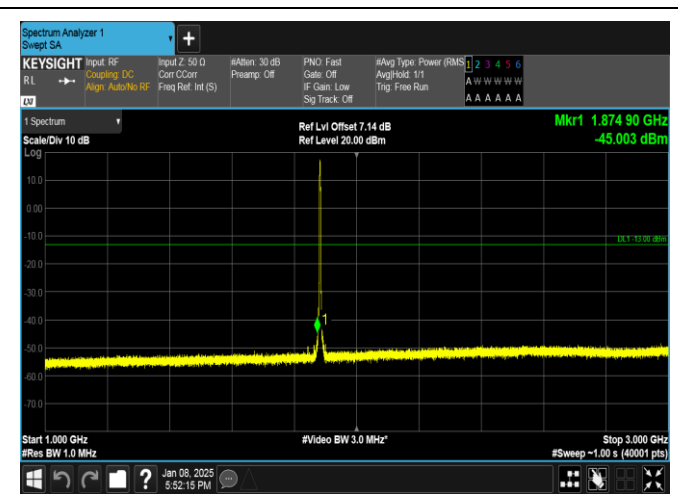
Band25-3MHz-16QAM-26365-15RB#0-1000~3000-PASS
