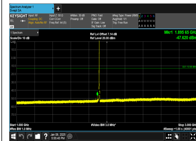
Band25-3MHz-QPSK-26675-1RB#14-1000~3000-PASS
