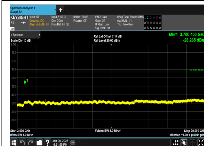
Band25-5MHz-QPSK-26065-1RB#0-3000~20000-PASS
