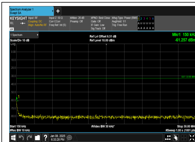
Band25-5MHz-QPSK-26065-1RB#24-0.15~30-PASS
