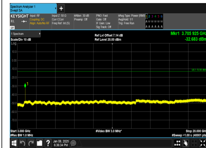
Band25-5MHz-QPSK-26065-25RB#0-3000~20000-PASS
