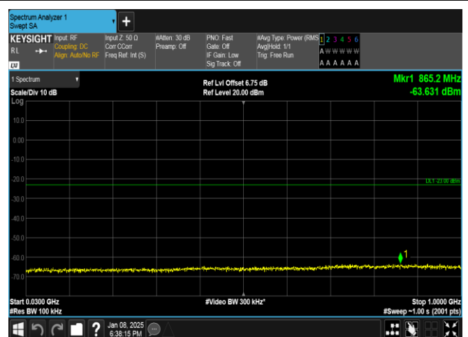
Band25-5MHz-QPSK-26365-1RB#0-30~1000-PASS
