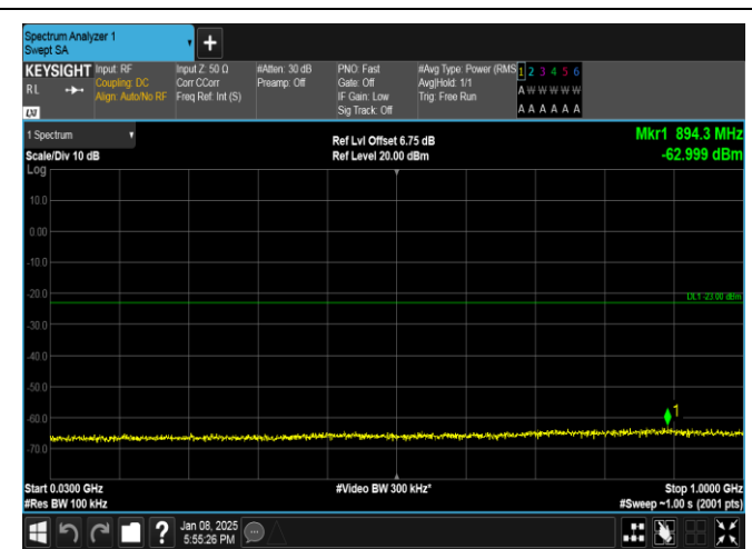
Band25-3MHz-QPSK-26675-1RB#14-30~1000-PASS
