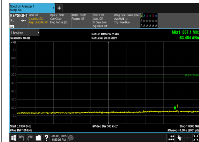
Band25-3MHz-QPSK-26675-1RB#0-30~1000-PASS
