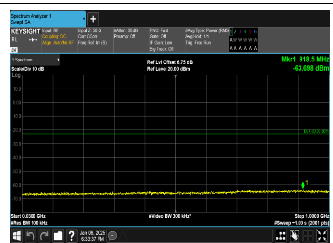
Band25-5MHz-QPSK-26065-1RB#24-30~1000-PASS
