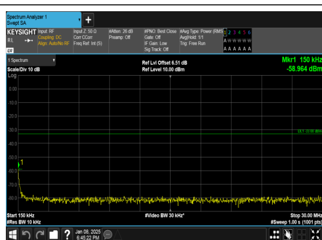
Band25-5MHz-OPSK-26665-1RB#0-0.15~30-PASS
