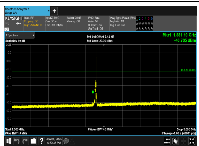
Band25-5MHz-QPSK-26665-25RB#0-1000~3000-PASS
