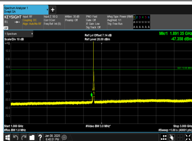
Band25-5MHz-QPSK-26665-1RB#0-1000~3000-PASS
