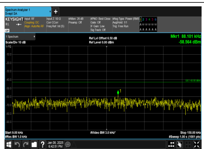
Band25-5MHz-QPSK-26365-25RB#0-0.009~0.15-PASS
