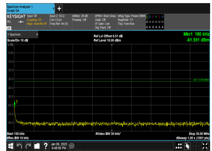
Band25-5MHz-16QAM-26665-1RB#24-0.15~30-PASS
