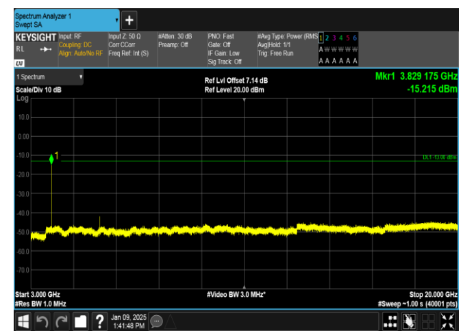
Band25-5MHz-QPSK-26665-1RB#24-3000~20000-PASS
