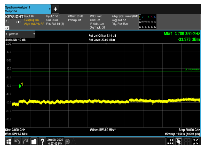
Band25-5MHz-16QAM-26065-25RB#0-3000~20000-PASS
