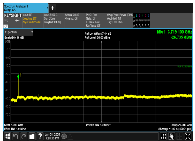
Band25-10MHz-QPSK-26090-1RB#49-3000~20000-PASS
