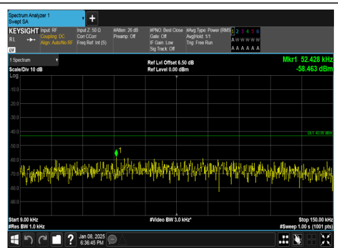
Band25-5MHz-16QAM-26065-25RB#0-0.009~0.15-PASS
