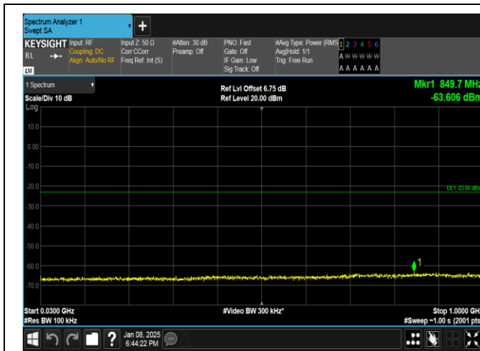
Band25-5MHz-16QAM-26365-25RB#0-30~1000-PASS
