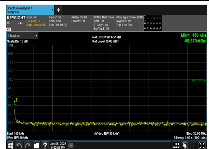
Band25-5MHz-QPSK-26665-25RB#0-0.15~30-PASS
