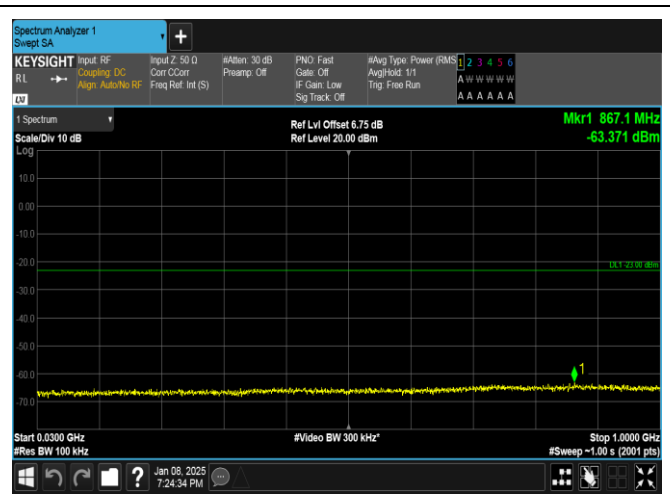
Band25-10MHz-QPSK-26090-1RB#49-30~1000-PASS
