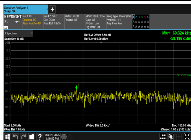
Band25-5MHz-QPSK-26665-1RB#24-0.009~0.15-PASS
