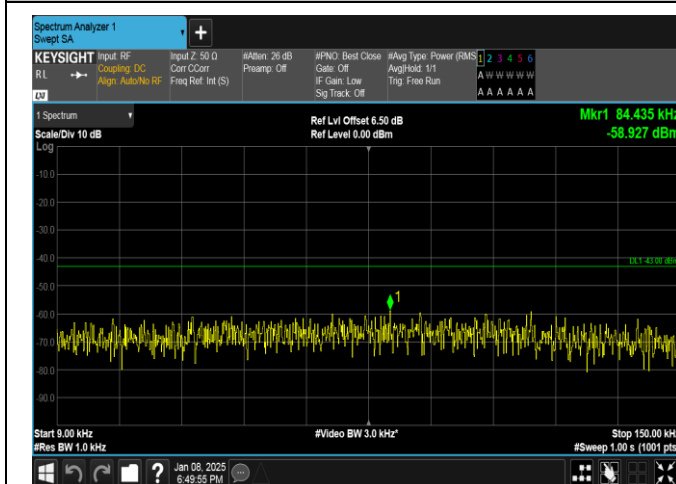
Band25-5MHz-QPSK-26665-25RB#0-0.009~0.15-PASS
