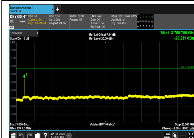
Band25-5MHz-16QAM-26365-1RB#0-3000~20000-PASS
