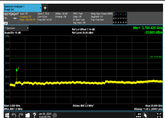
Band25-5MHz-QPSK-26365-25RB#0-3000~20000-PASS
