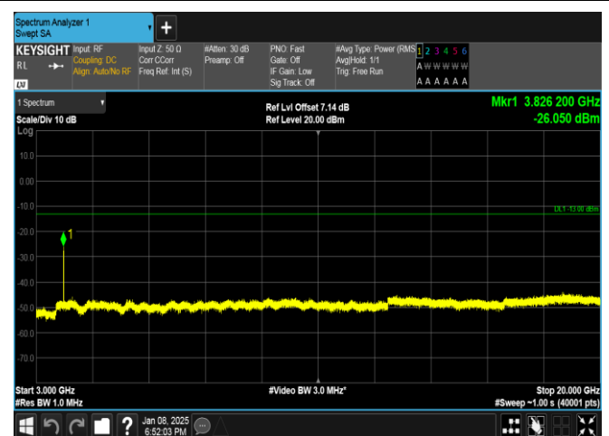
Band25-5MHz-16QAM-26665-25RB#0-3000~20000-PASS
