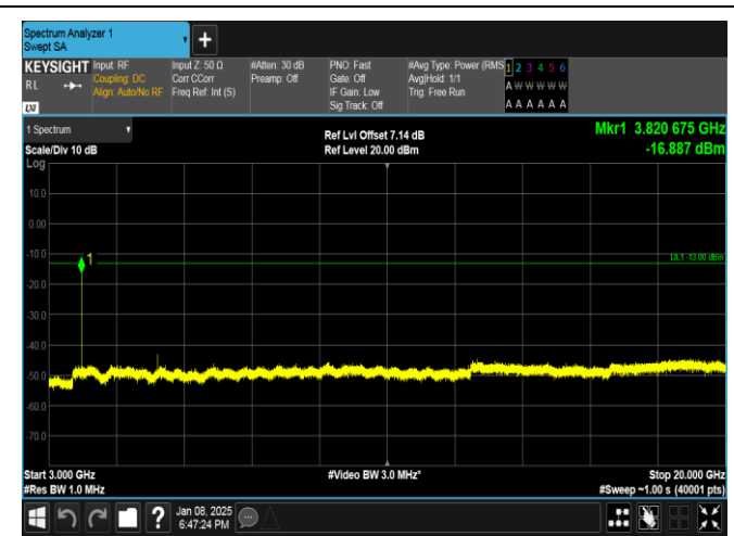
Band25-5MHz-16QAM-26665-1RB#0-3000~20000-PASS
