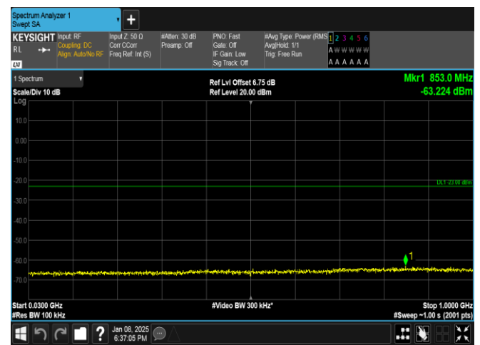
Band25-5MHz-16QAM-26065-25RB#0-30~1000-PASS
