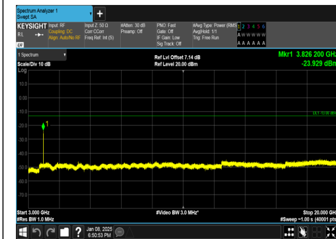
Band25-5MHz-QPSK-26665-25RB#0-3000~20000-PASS
