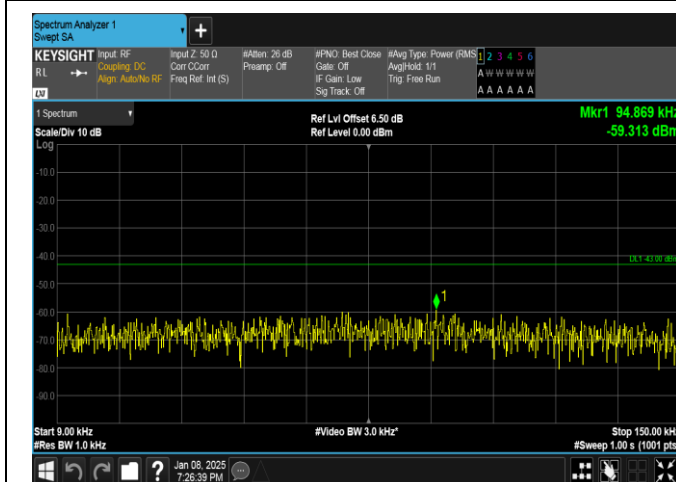
Band25-10MHz-QPSK-26090-50RB#0-0.009~0.15-PASS
