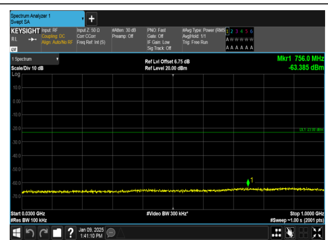
Band25-5MHz-QPSK-26665-1RB#24-30~1000-PASS
