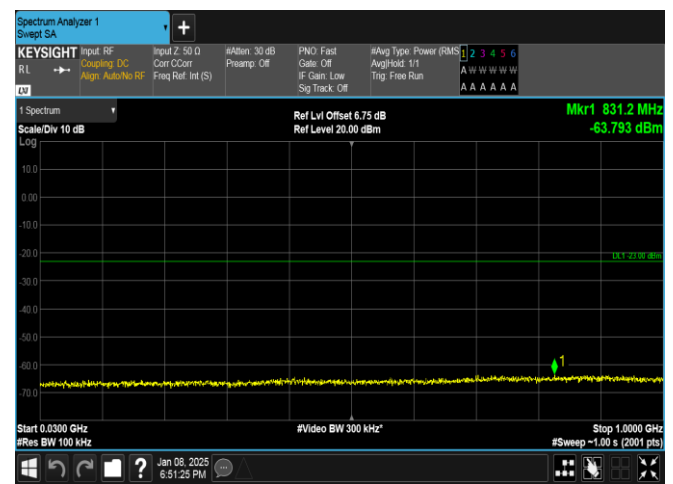
Band25-5MHz-16QAM-26665-25RB#0-30~1000-PASS
