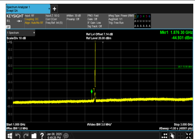
Band25-5MHz-16QAM-26665-1RB#24-1000~3000-PASS
