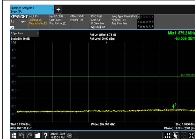
Band25-5MHz-QPSK-26665-1RB#0-30~1000-PASS
