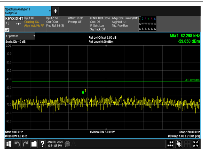
Band25-5MHz-16QAM-26665-25RB#0-0.009~0.15-PASS
