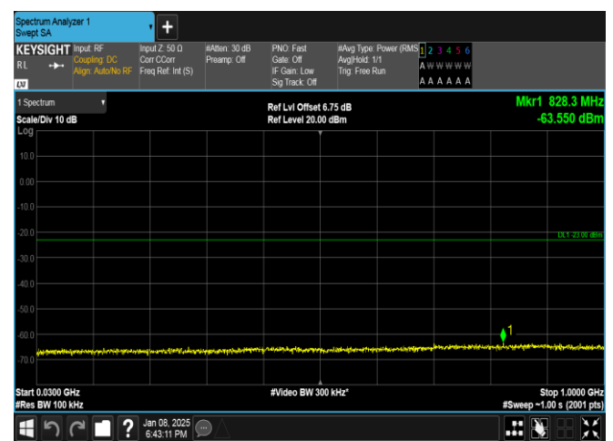
Band25-5MHz-QPSK-26365-25RB#0-30~1000-PASS
