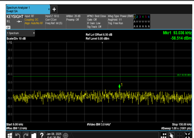
Band25-5MHz-16QAM-26365-1RB#24-0.009~0.15-PASS
