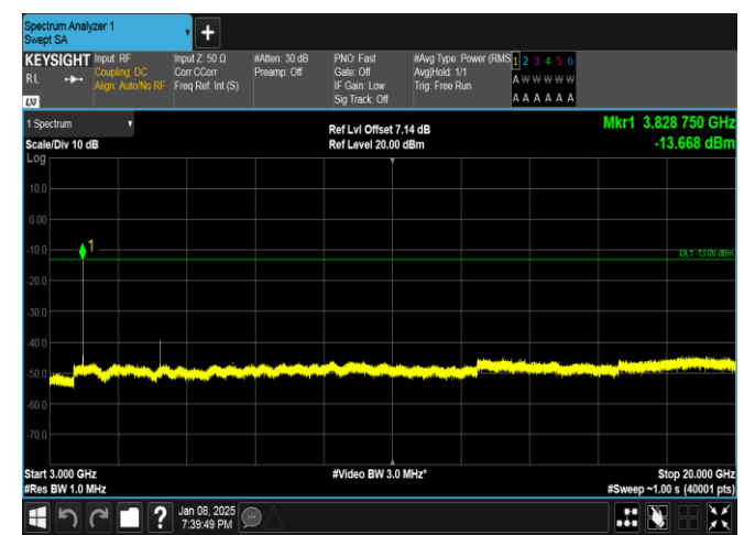
Band25-10MHz-QPSK-26640-1RB#49-3000~20000-PASS
