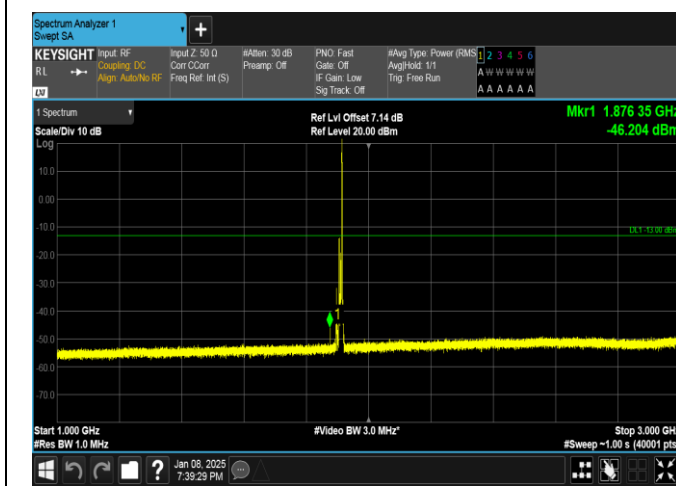
Band25-10MHz-QPSK-26640-1RB#49-1000~3000-PASS
