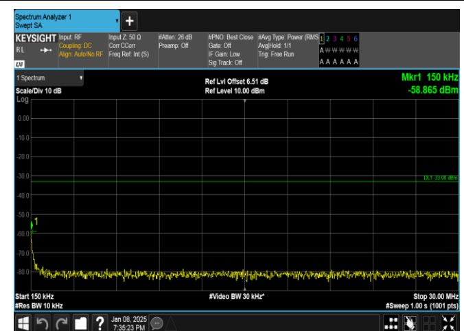
Band25-10MHz-16QAM-26365-50RB#0-0.15~30-PASS
