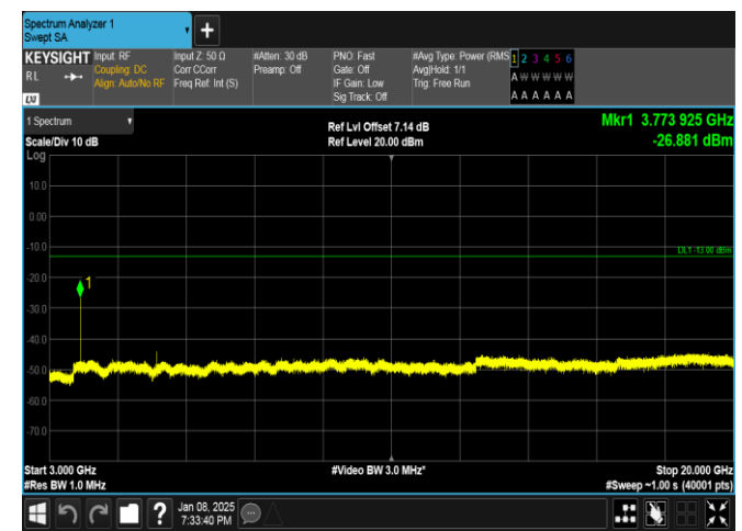
Band25-10MHz-16QAM-26365-1RB#49-3000~20000-PASS
