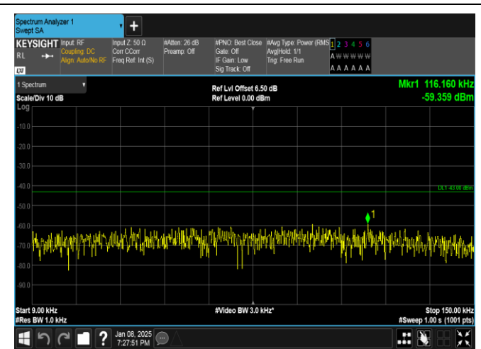
Band25-10MHz-16QAM-26090-50RB#0-0.009~0.15-PASS
