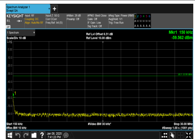
Band25-10MHz-QPSK-26640-50RB#0-0.15~30-PASS
