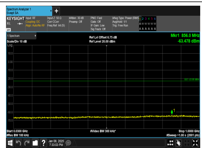
Band25-10MHz-16QAM-26365-1RB#49-30~1000-PASS
