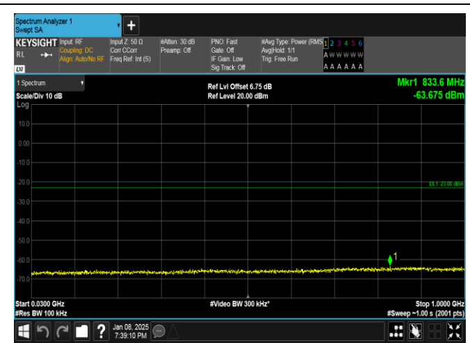
Band25-10MHz-QPSK-26640-1RB#49-30~1000-PASS
