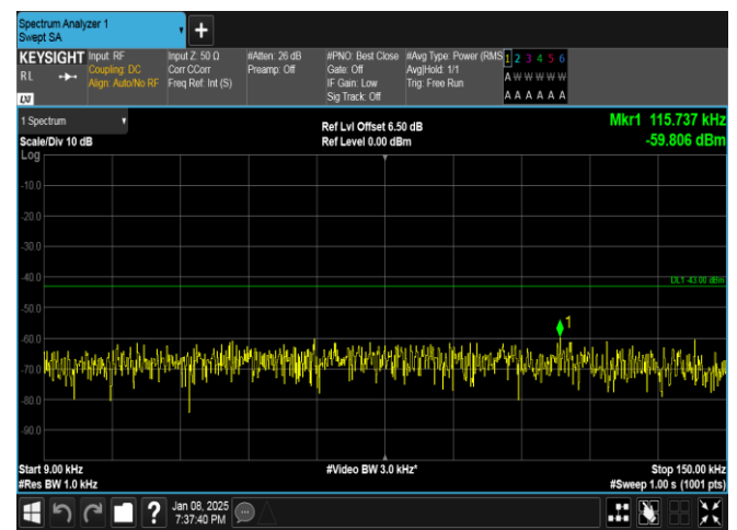
Band25-10MHz-16QAM-26640-1RB#0-0.009~0.15-PASS
