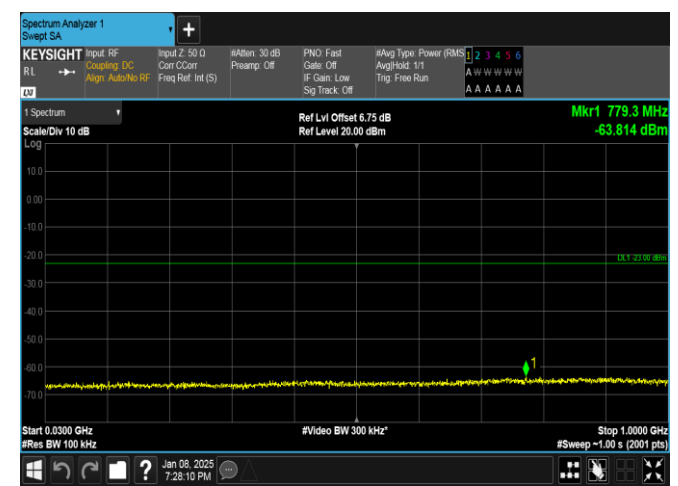
Band25-10MHz-16QAM-26090-50RB#0-30~1000-PASS
