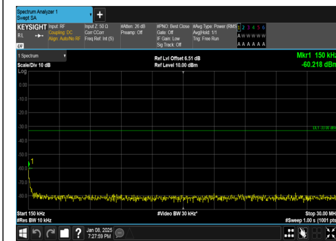
Band25-10MHz-16QAM-26090-50RB#0-0.15~30-PASS
