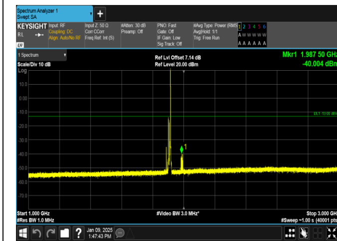
Band25-15MHz-QPSK-26615-1RB#74-1000~3000-PASS
