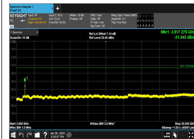
Band25-15MHz-QPSK-26615-75RB#0-3000~20000-PASS
