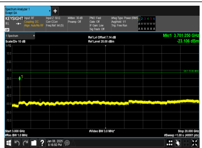
Band25-15MHz-16QAM-26115-1RB#0-3000~20000-PASS
