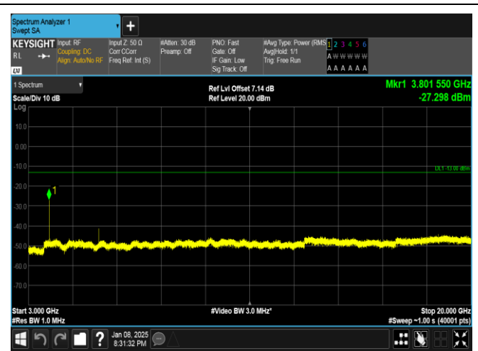
Band25-15MHz-16QAM-26615-1RB#0-3000~20000-PASS
