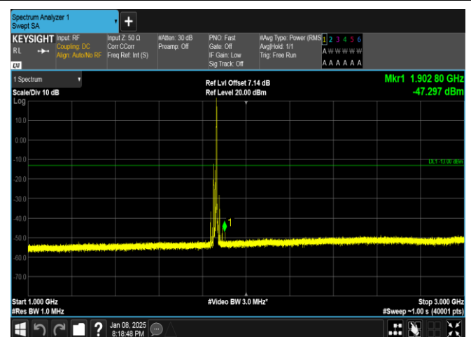
Band25-15MHz-16QAM-26115-1RB#74-1000~3000-PASS
