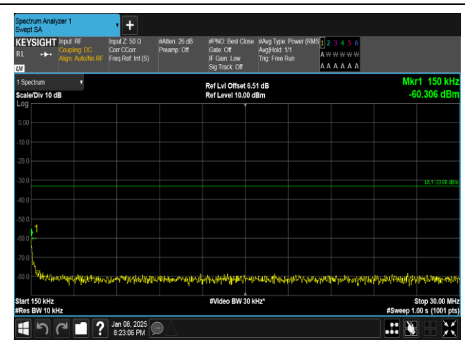
Band25-15MHz-16QAM-26365-1RB#0-0.15~30-PASS
