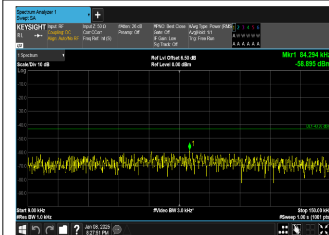
Band25-15MHz-16QAM-26365-75RB#0-0.009~0.15-PASS
