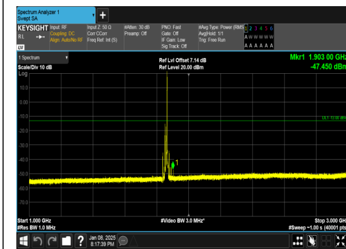
Band25-15MHz-QPSK-26115-1RB#74-1000~3000-PASS
