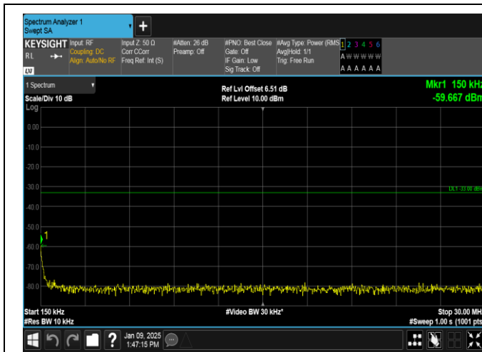
Band25-15MHz-QPSK-26615-1RB#74-0.15~30-PASS
