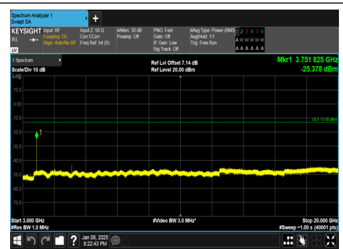
Band25-15MHz-QPSK-26365-1RB#0-3000~20000-PASS
