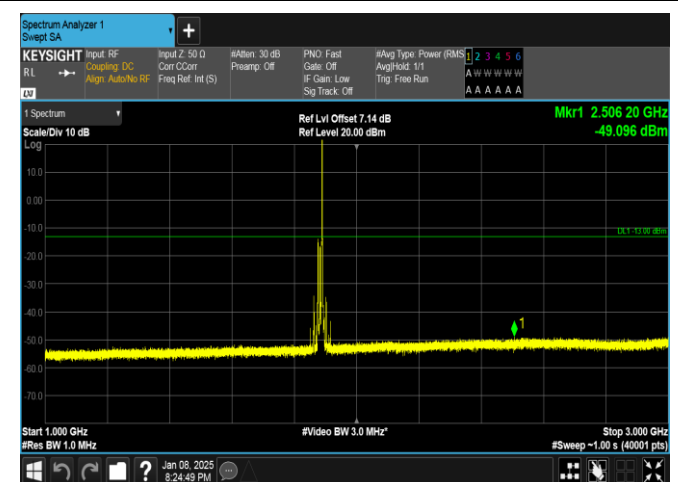
Band25-15MHz-QPSK-26365-1RB#74-1000~3000-PASS
