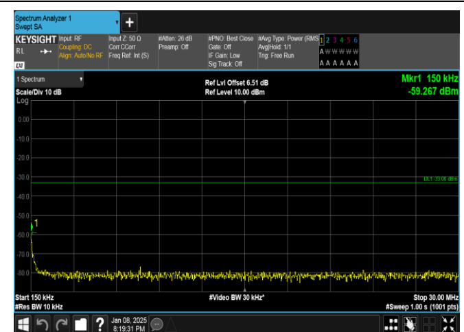
Band25-15MHz-QPSK-26115-75RB#0-0.15~30-PASS
