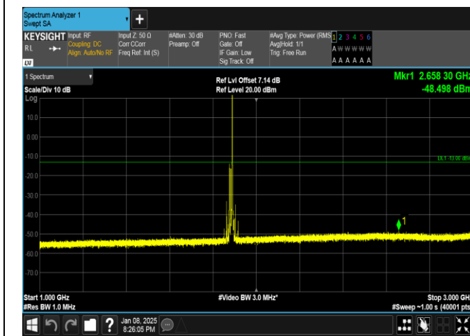
Band25-15MHz-16QAM-26365-1RB#74-1000~3000-PASS
