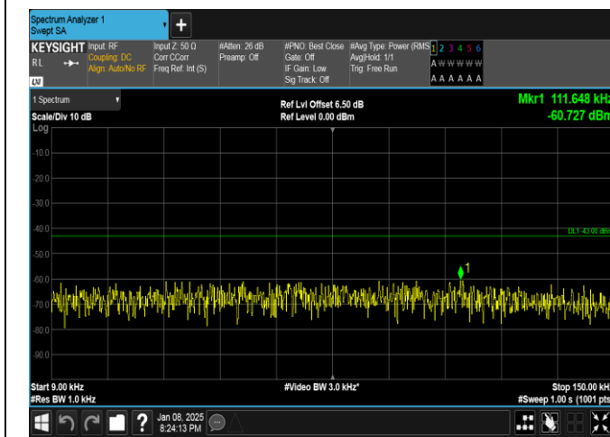
Band25-15MHz-QPSK-26365-1RB#74-0.009~0.15-PASS
