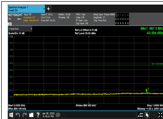
Band25-15MHz-QPSK-26115-75RB#0-30~1000-PASS
