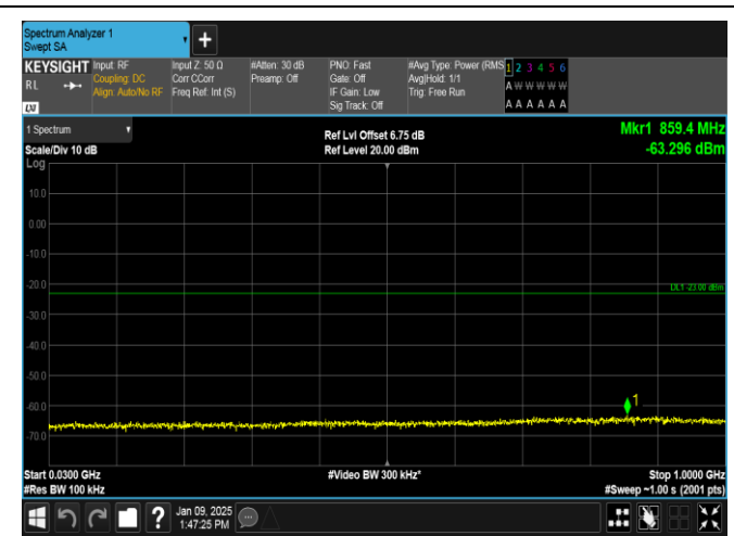
Band25-15MHz-QPSK-26615-1RB#74-30~1000-PASS
