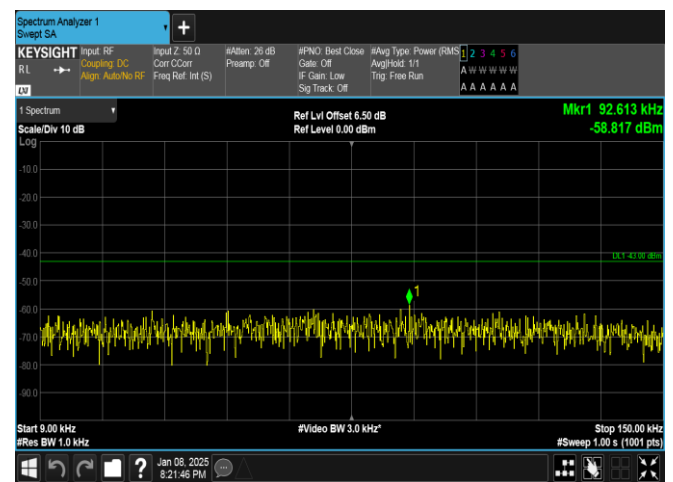
Band25-15MHz-QPSK-26365-1RB#0-0.009~0.15-PASS
