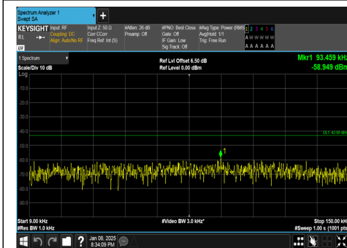
Band25-15MHz-QPSK-26615-75RB#0-0.009~0.15-PASS
