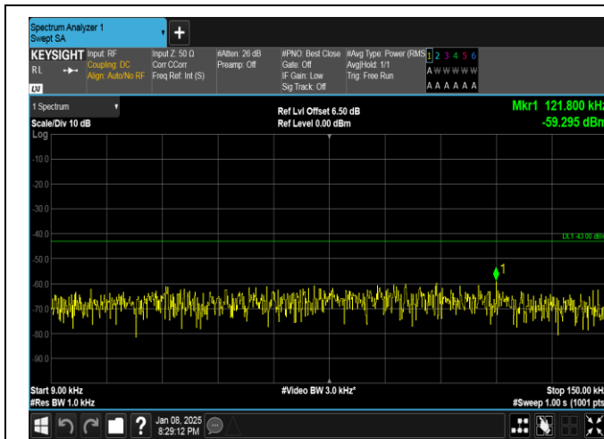
Band25-15MHz-QPSK-26615-1RB#0-0.009~0.15-PASS
