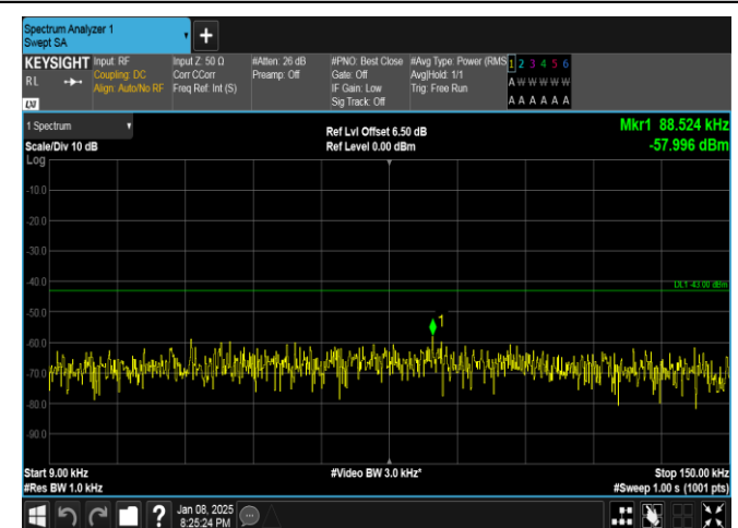
Band25-15MHz-16QAM-26365-1RB#74-0.009~0.15-PASS
