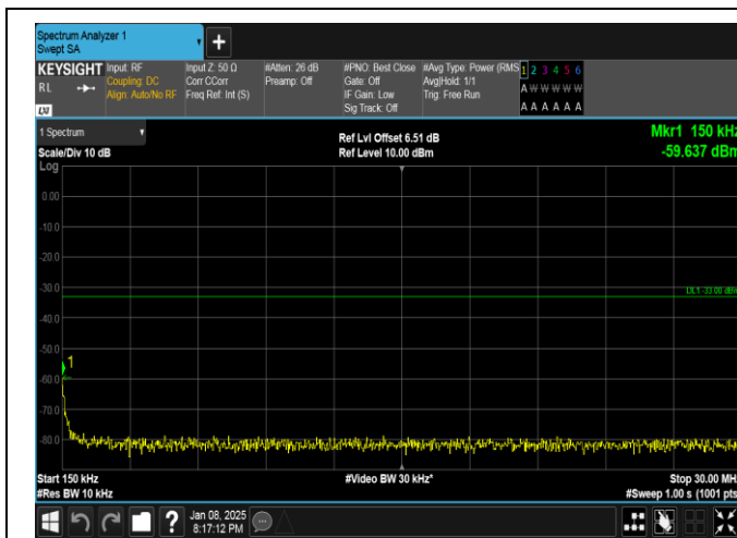
Band25-15MHz-QPSK-26115-1RB#74-0.15~30-PASS
