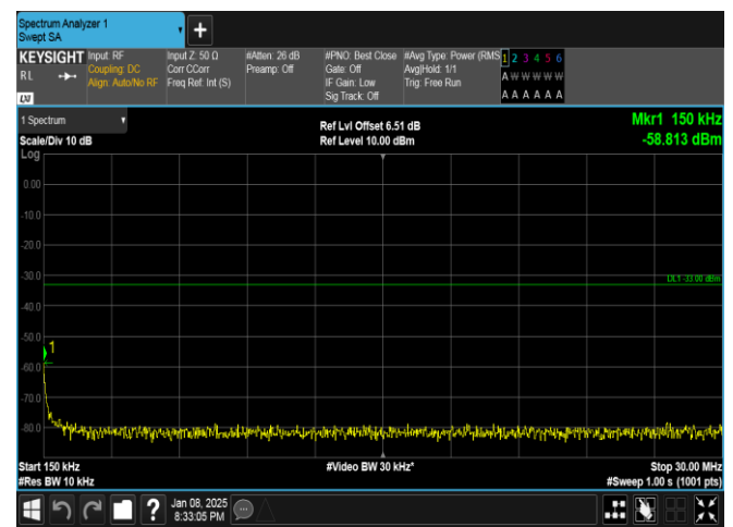
Band25-15MHz-16QAM-26615-1RB#74-0.15~30-PASS
