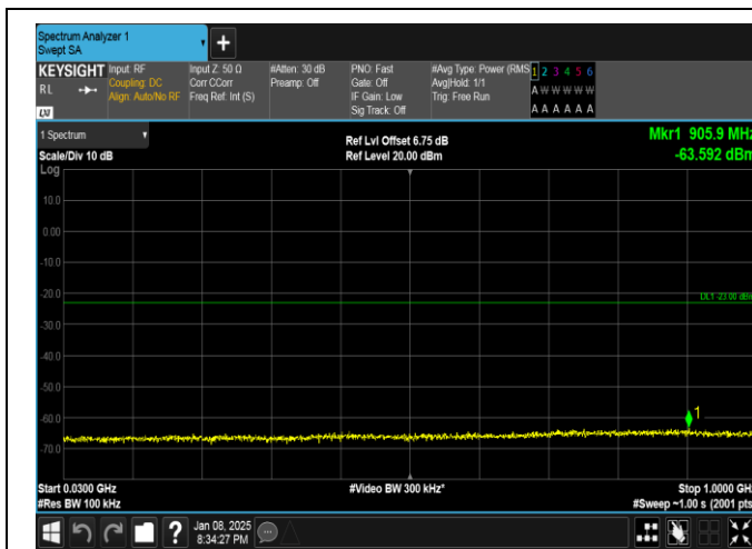
Band25-15MHz-QPSK-26615-75RB#0-30~1000-PASS
