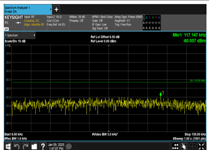
Band25-15MHz-QPSK-26615-1RB#74-0.009~0.15-PASS
