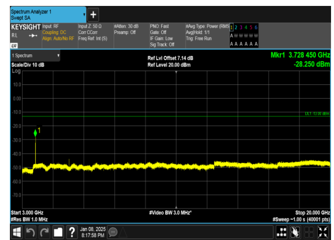
Band25-15MHz-QPSK-26115-1RB#74-3000~20000-PASS
