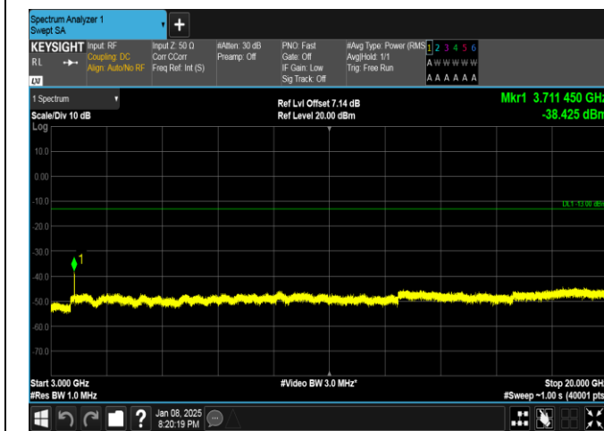
Band25-15MHz-QPSK-26115-75RB#0-3000~20000-PASS
