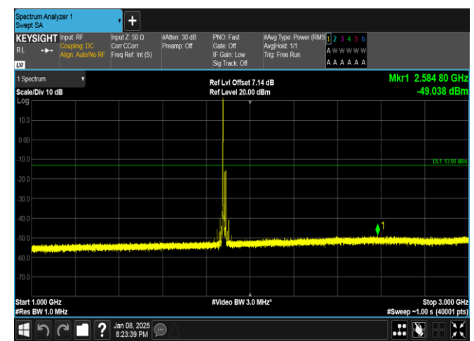
Band25-15MHz-16QAM-26365-1RB#0-1000~3000-PASS
