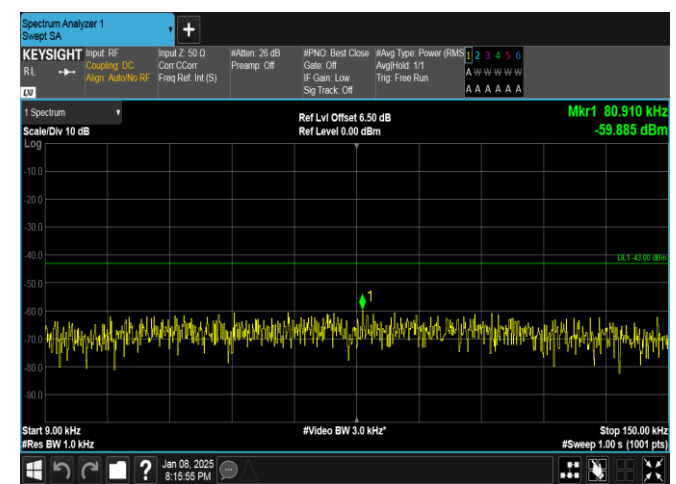
Band25-15MHz-16QAM-26115-1RB#0-0.009~0.15-PASS
