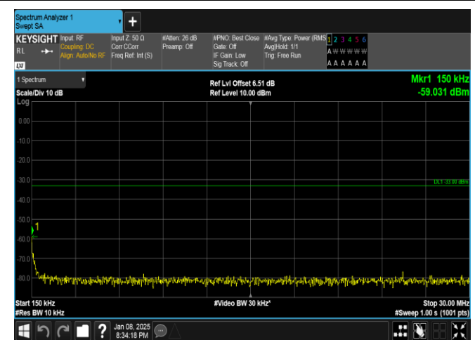
Band25-15MHz-QPSK-26615-75RB#0-0.15~30-PASS
