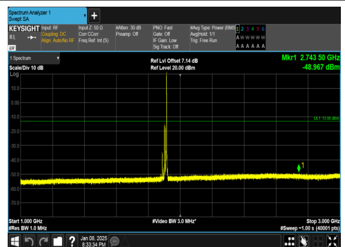
Band25-15MHz-16QAM-26615-1RB#74-1000~3000-PASS
