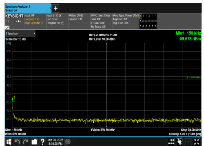
Band25-15MHz-16QAM-26115-1RB#74-0.15~30-PASS
