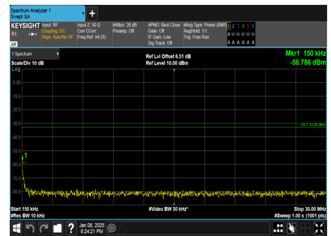
Band25-15MHz-QPSK-26365-1RB#74-0.15~30-PASS
