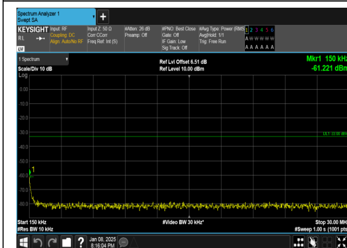
Band25-15MHz-16QAM-26115-1RB#0-0.15~30-PASS
