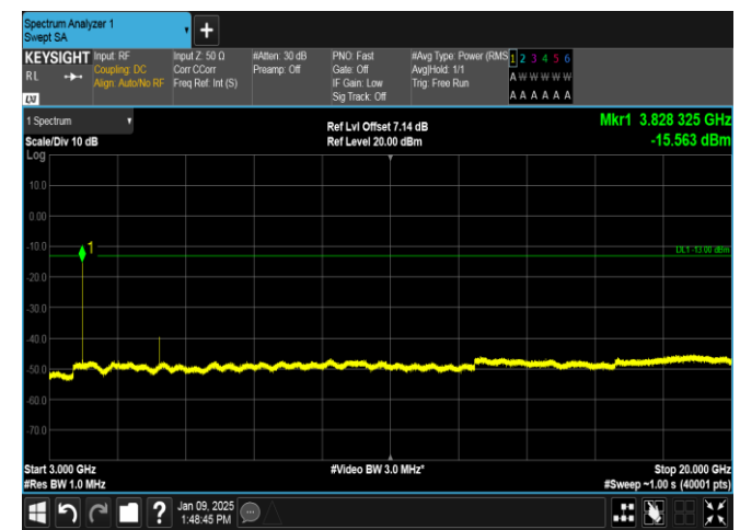
Band25-15MHz-QPSK-26615-1RB#74-3000~20000-PASS
