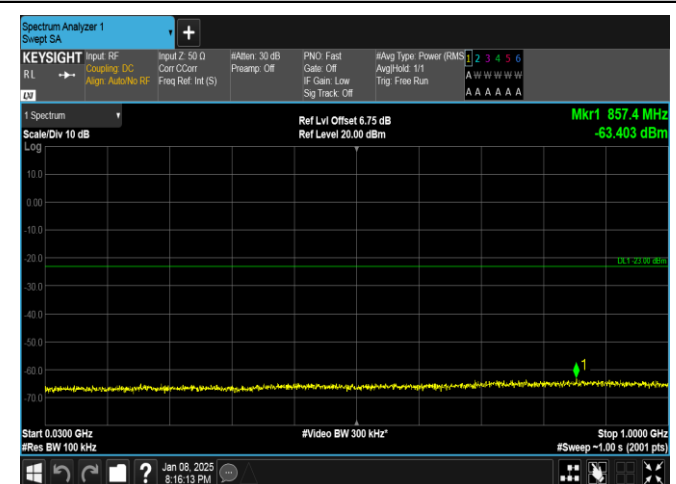
Band25-15MHz-16QAM-26115-1RB#0-30~1000-PASS
