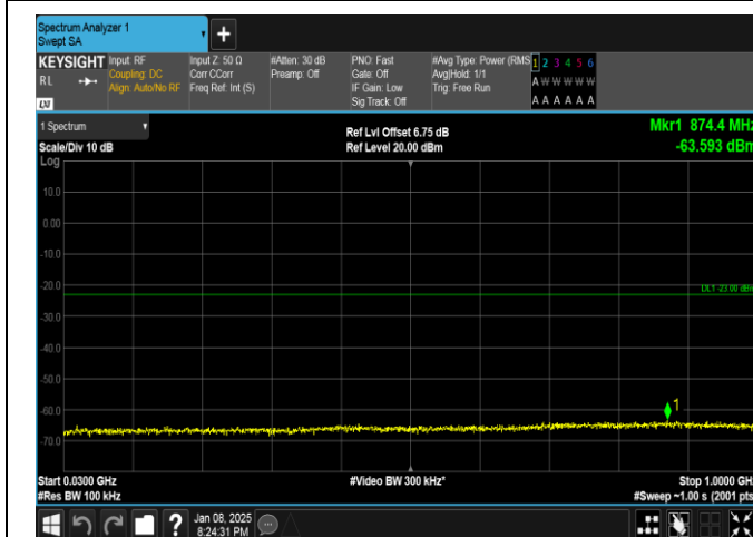
Band25-15MHz-QPSK-26365-1RB#74-30~1000-PASS
