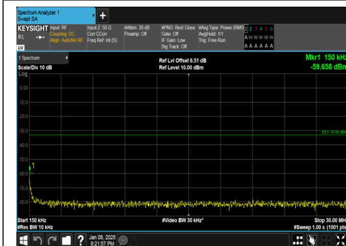
Band25-15MHz-QPSK-26365-1RB#0-0.15~30-PASS
