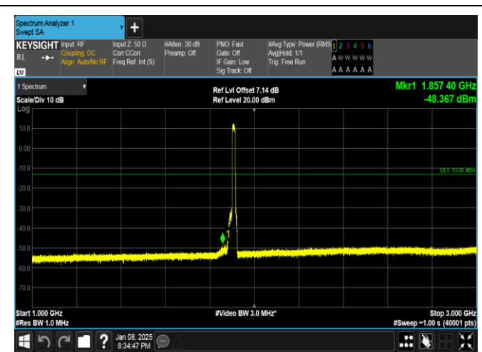
Band25-15MHz-QPSK-26615-75RB#0-1000~3000-PASS
