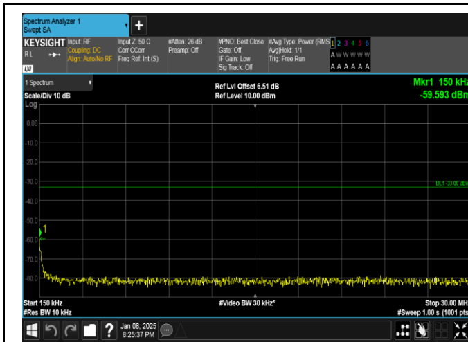
Band25-15MHz-16QAM-26365-1RB#74-0.15~30-PASS
